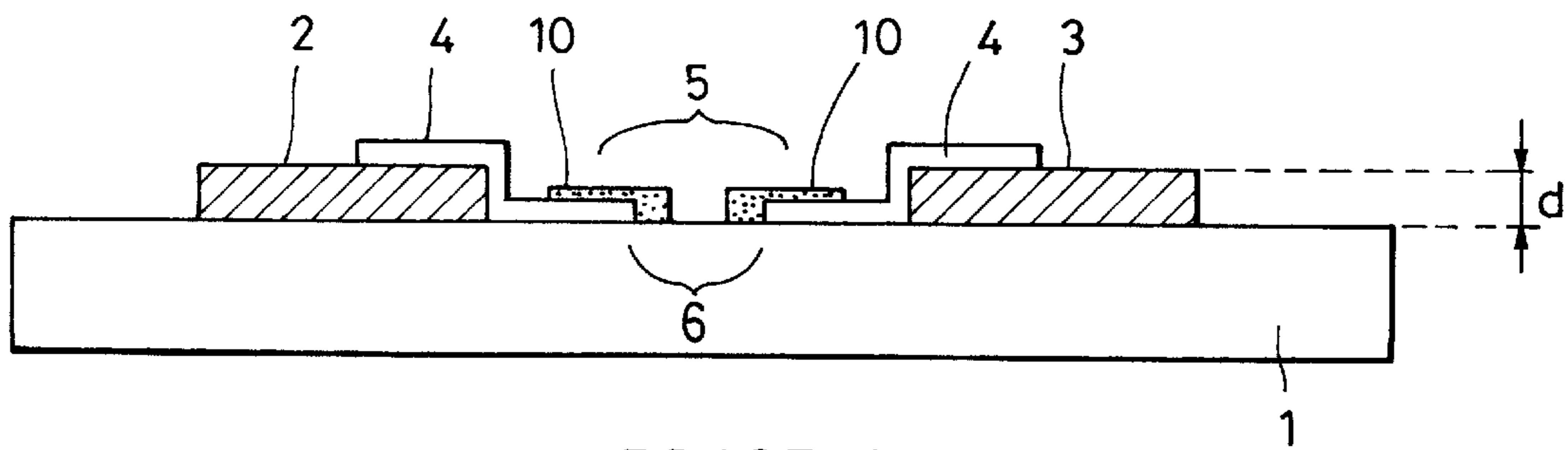
PRIOR ART
