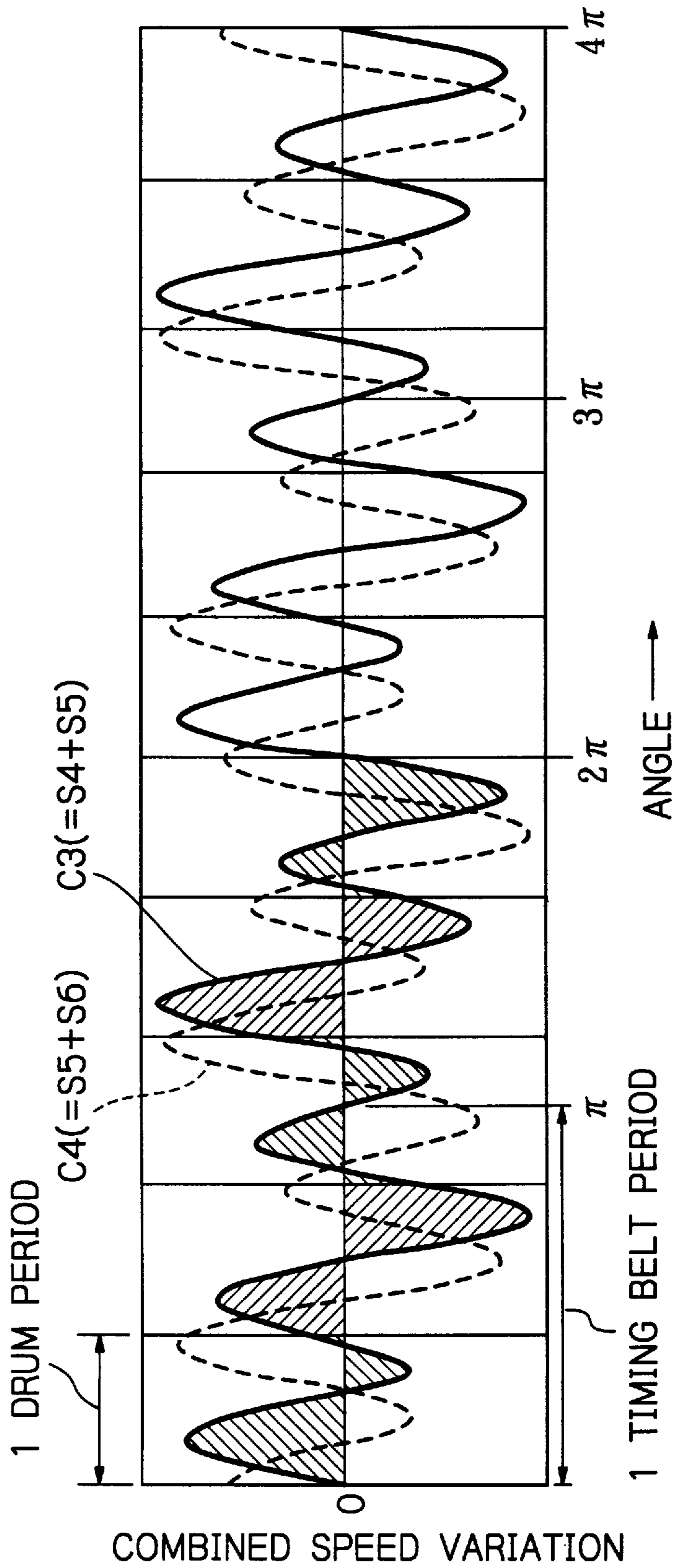
Fig. 5 PRIOR ART
