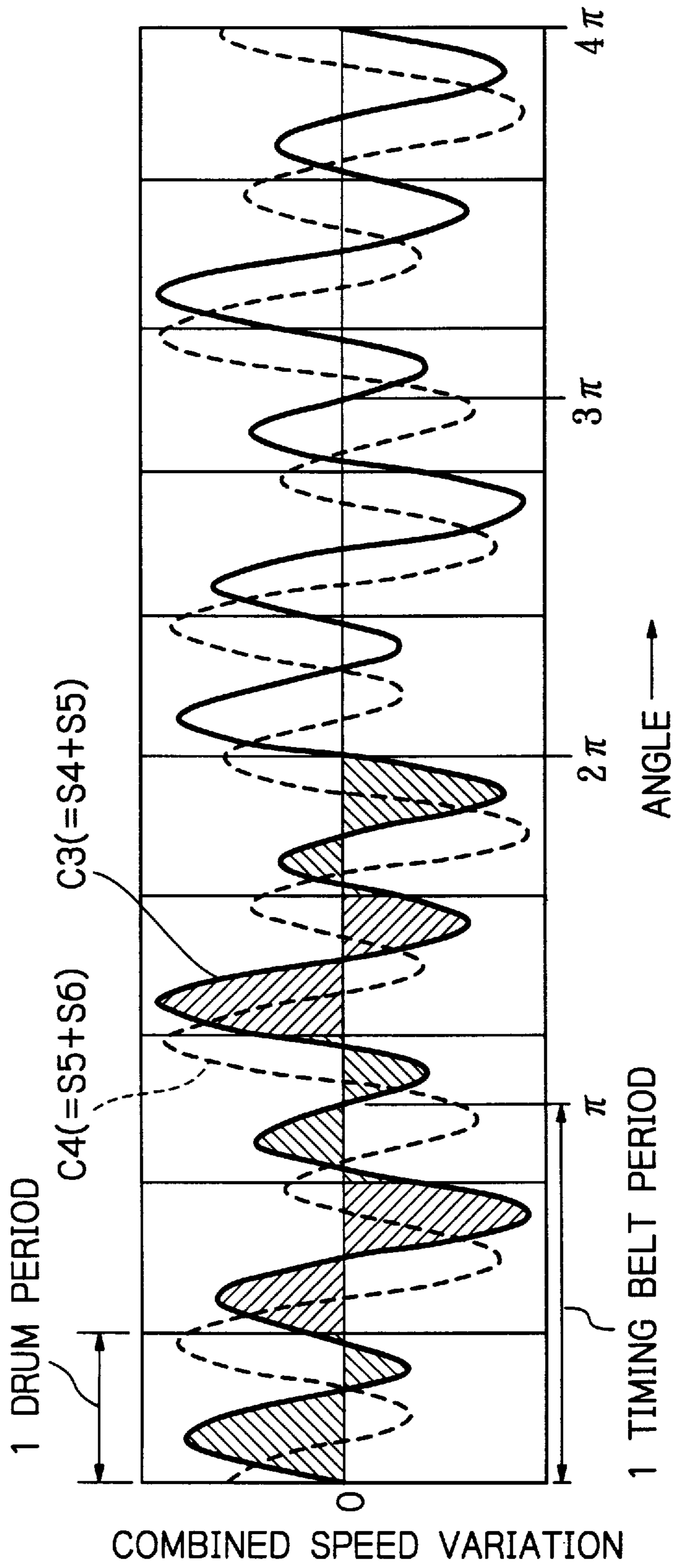
Fig. 5 PRIOR ART
