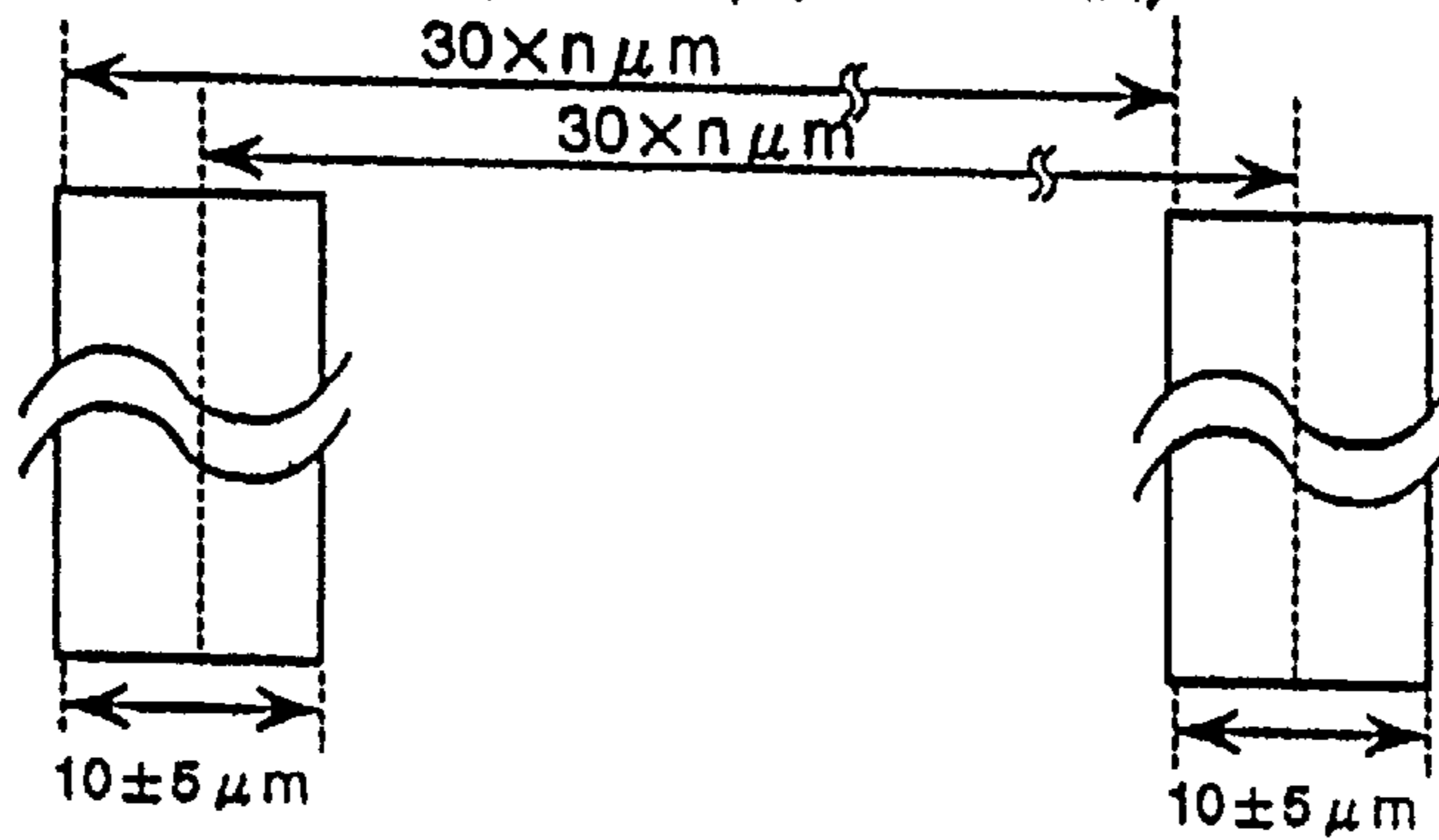
Fig. 5b Silt Dimension Accuracy (Precision) ( at r=22.2mm )
