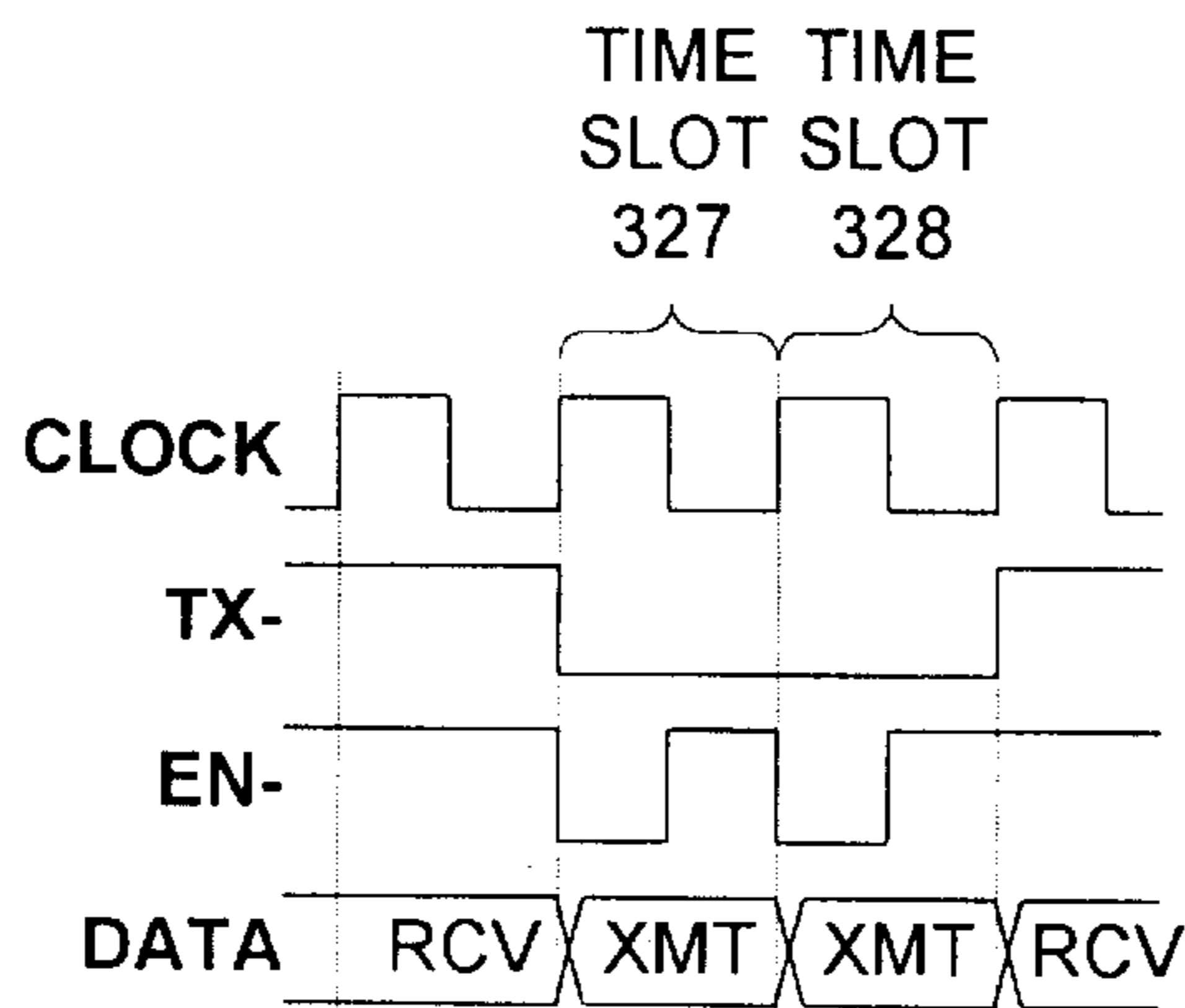
Figure 3b -- TDM TIMING
