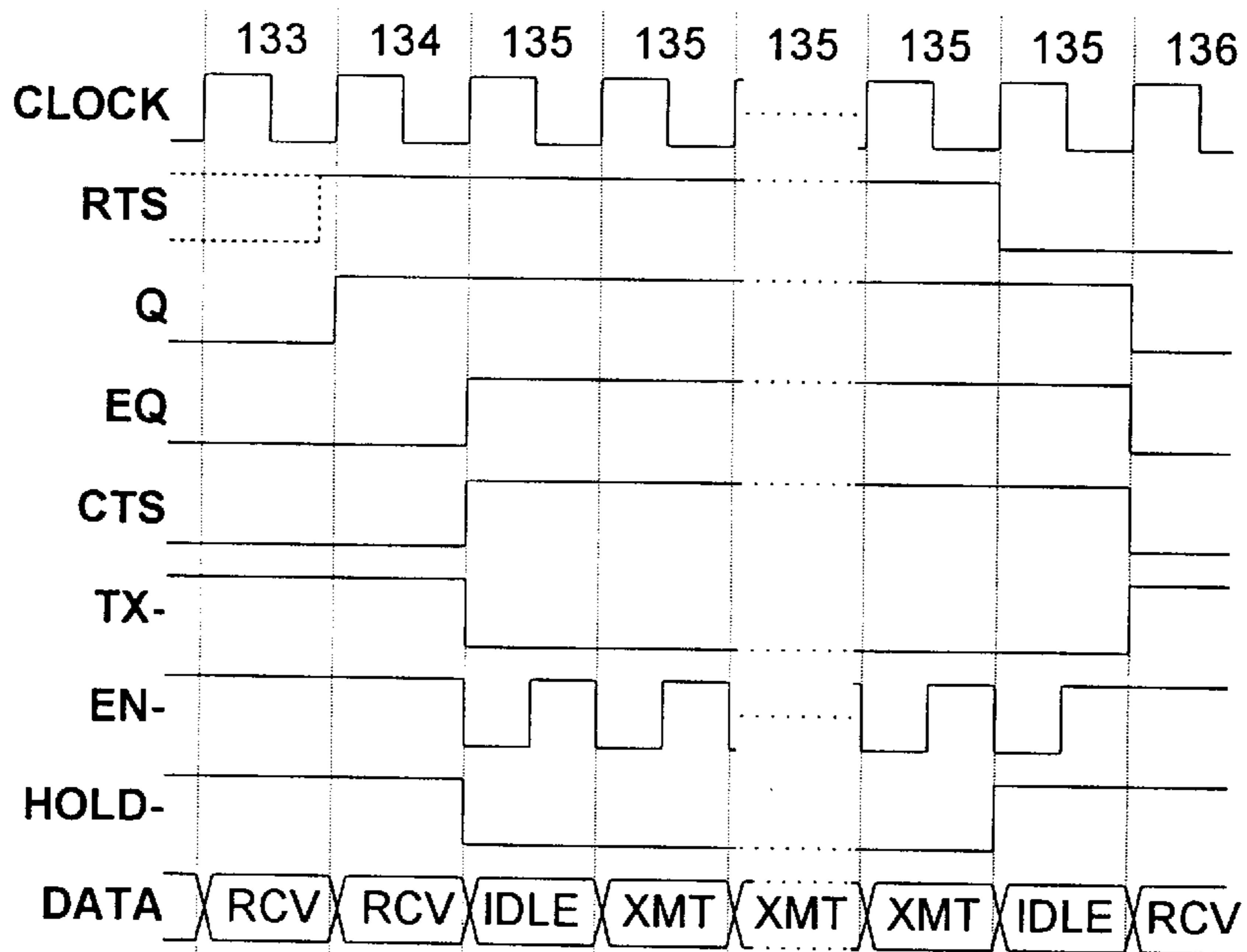
Figure 4b -- MESSAGE TIMING
