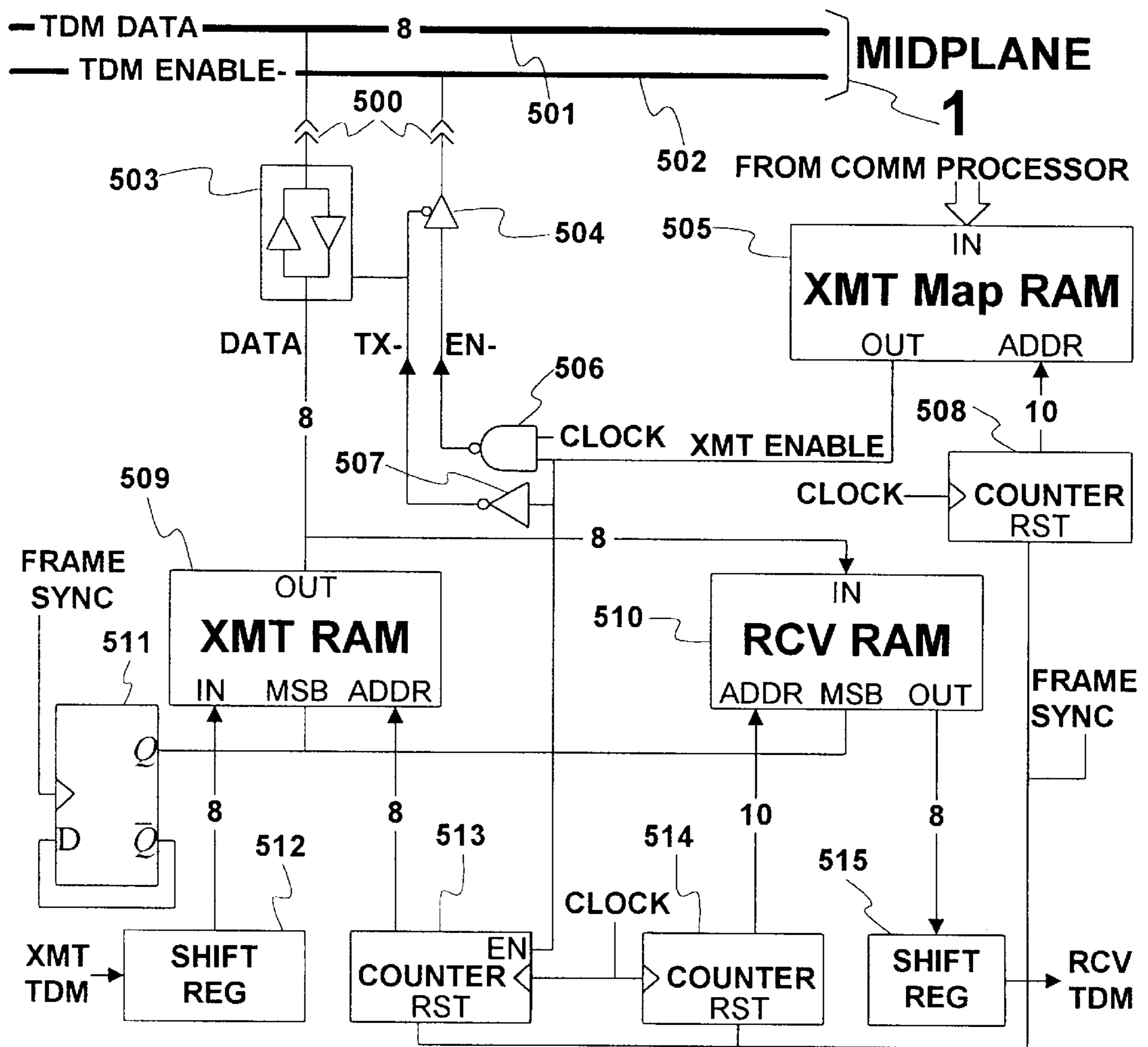
Figure 3a -- TDM ACCESS
