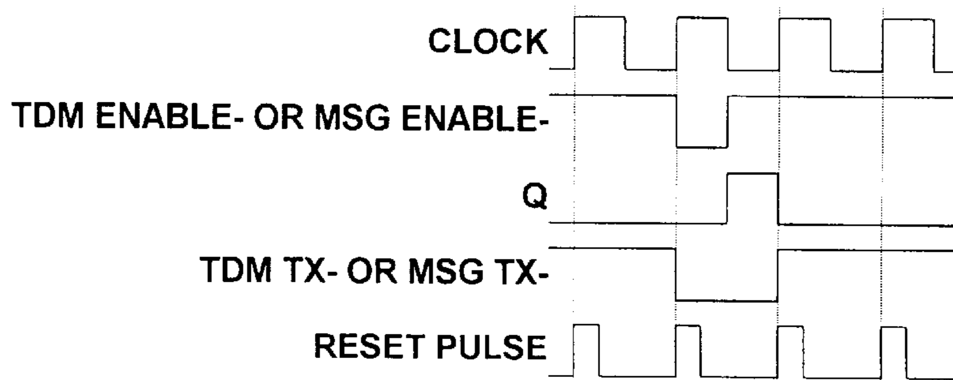
Figure 5b -- BUS REPEATER TIMING
