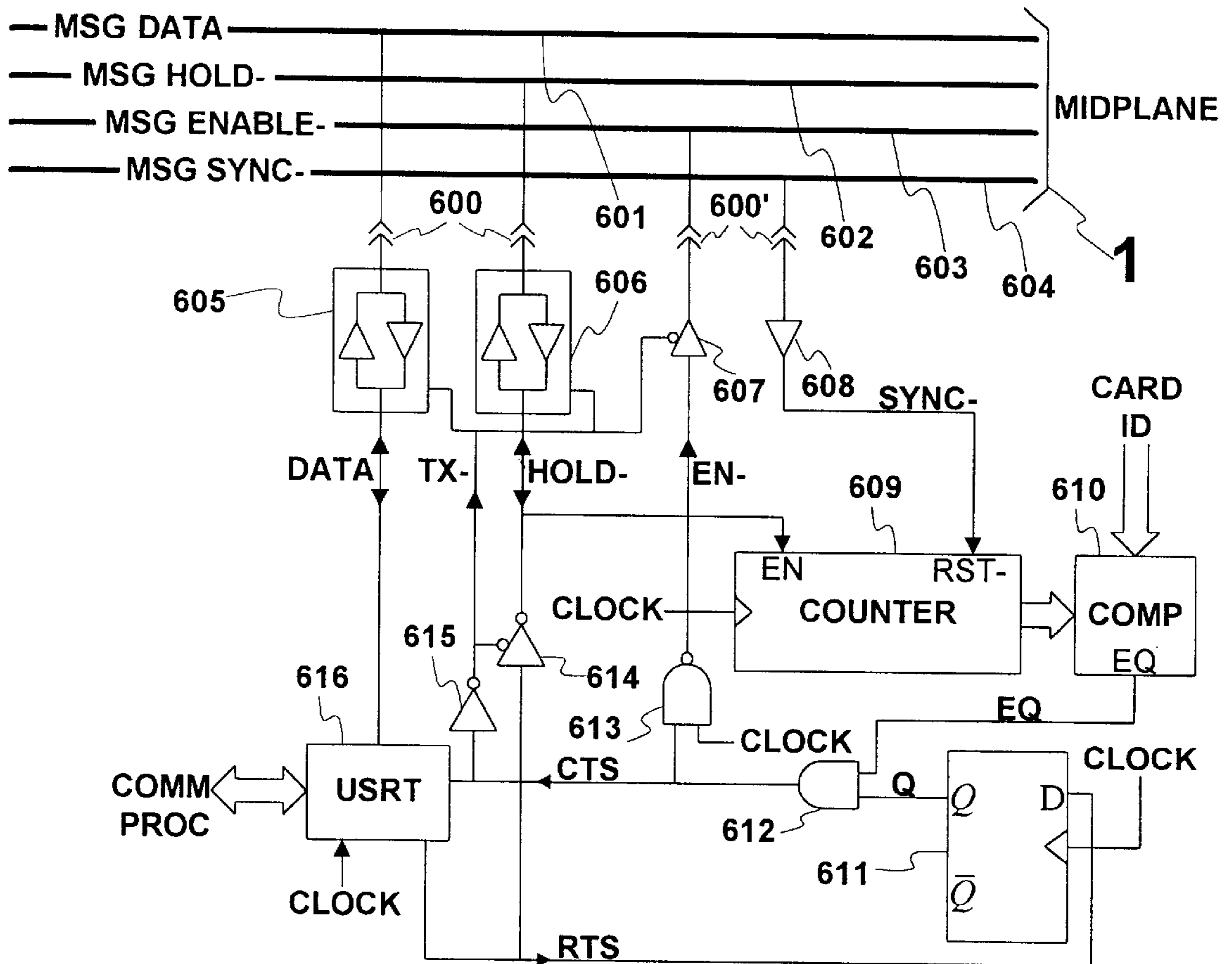
Figure 4a -- MESSAGE ACCESS
