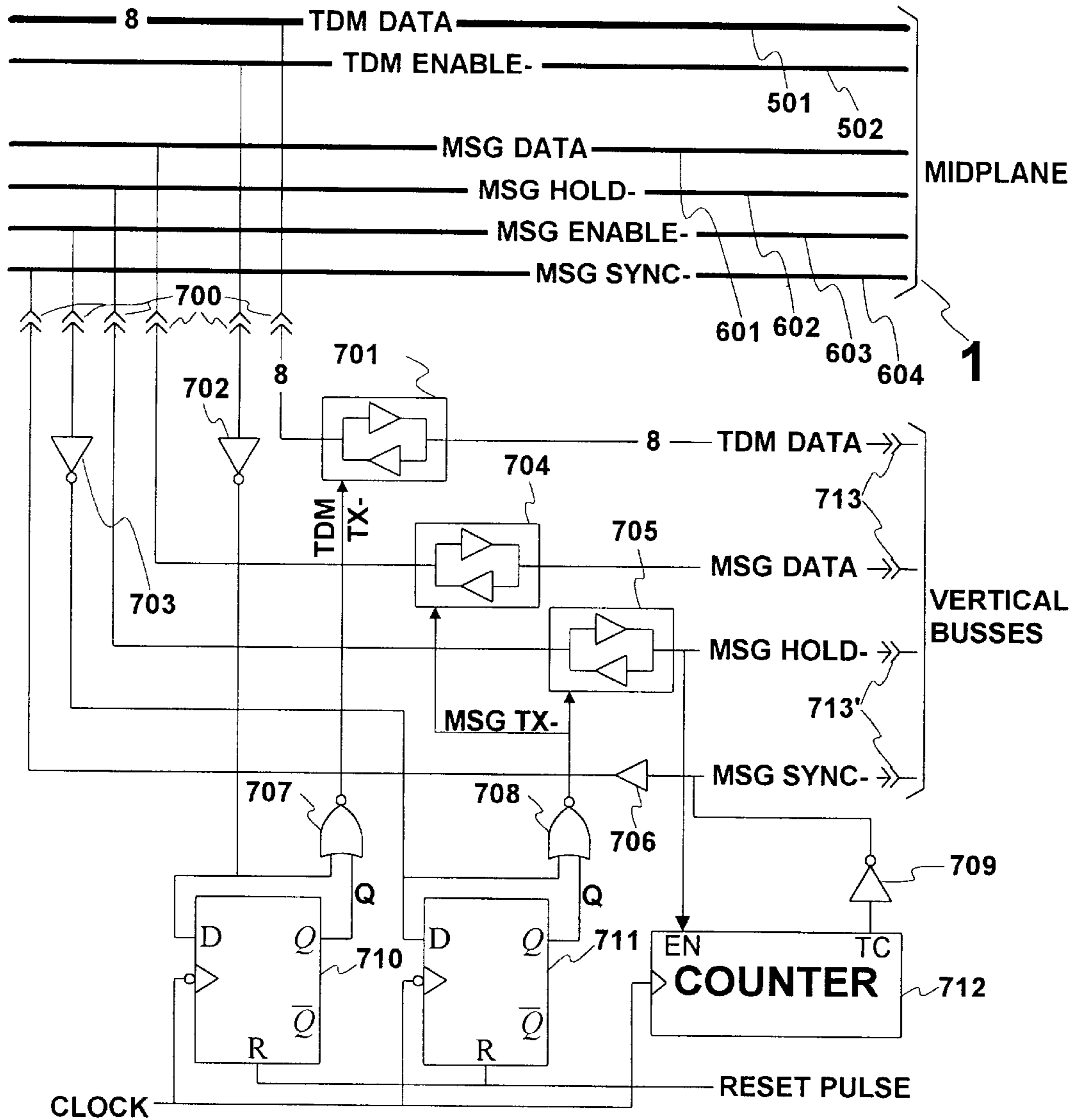
Figure 5a -- BUS REPEATER
