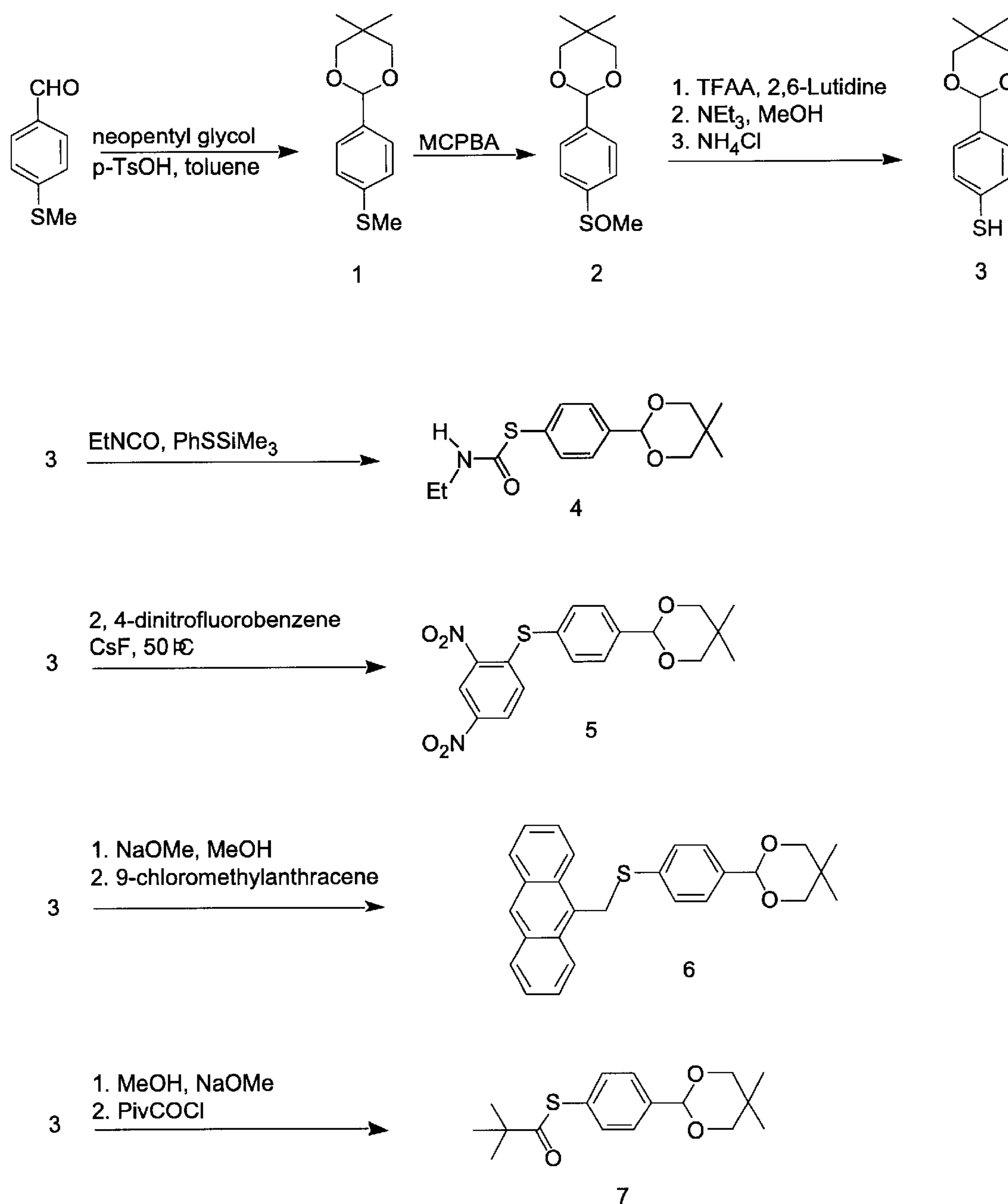
Scheme 1
