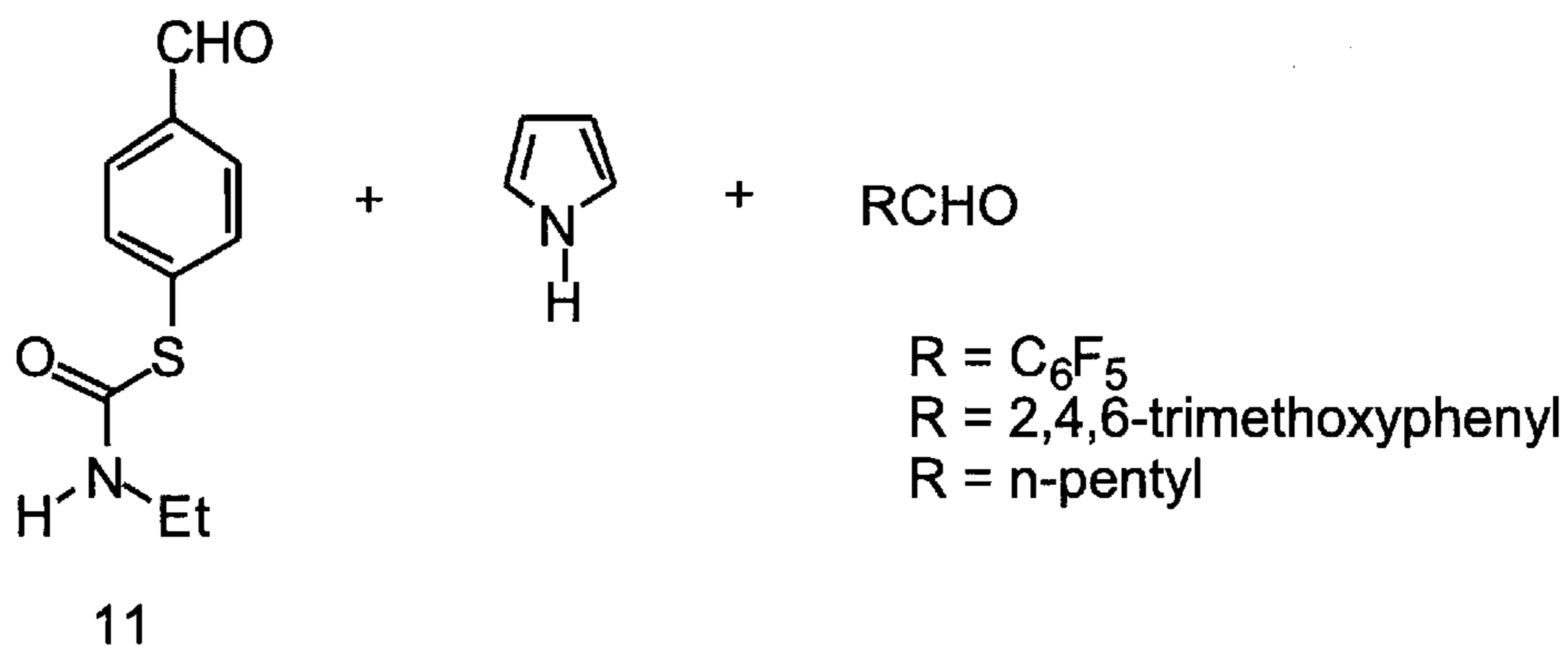
Scheme 6
