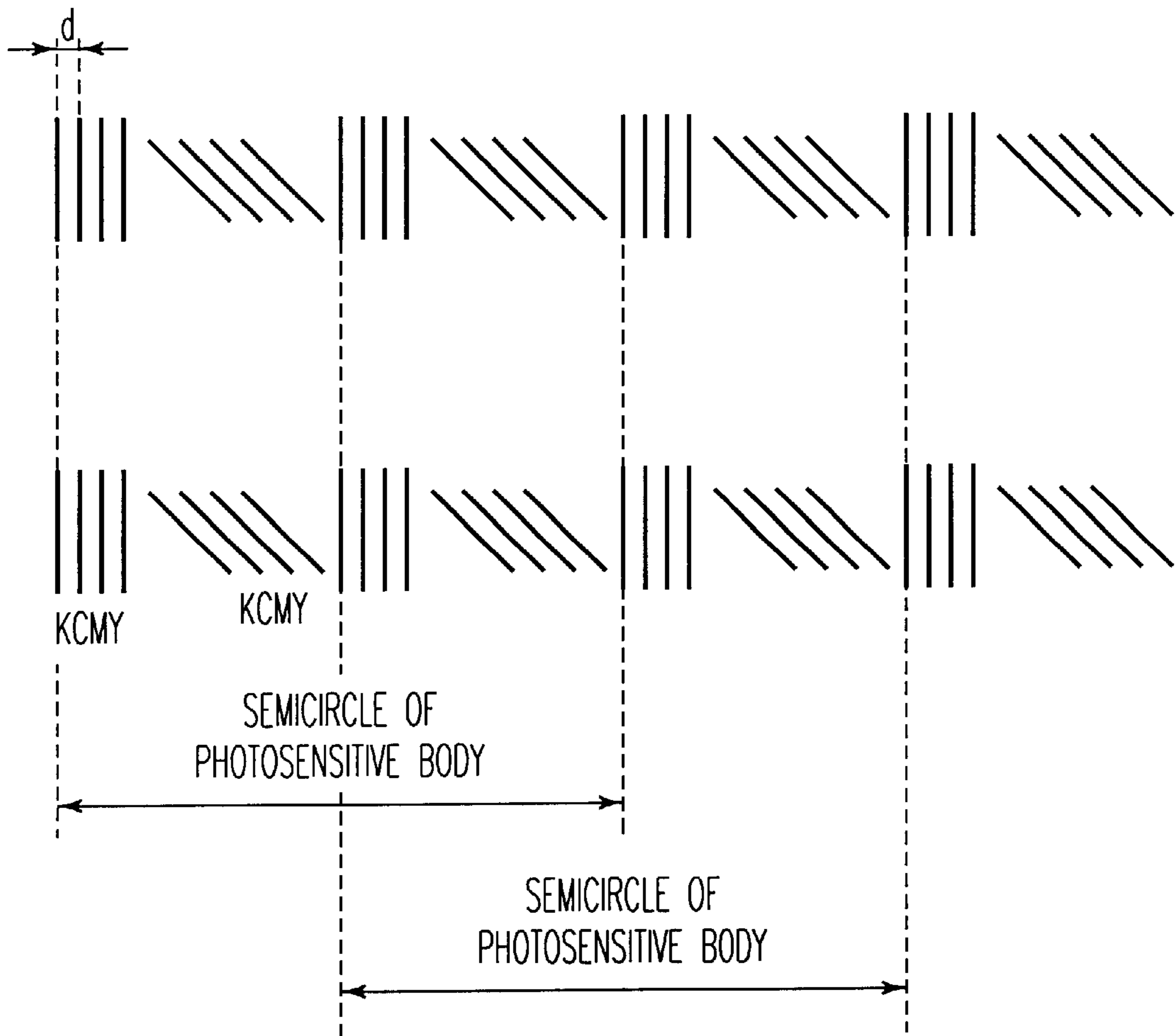
FIG. 15 PRIOR ART
