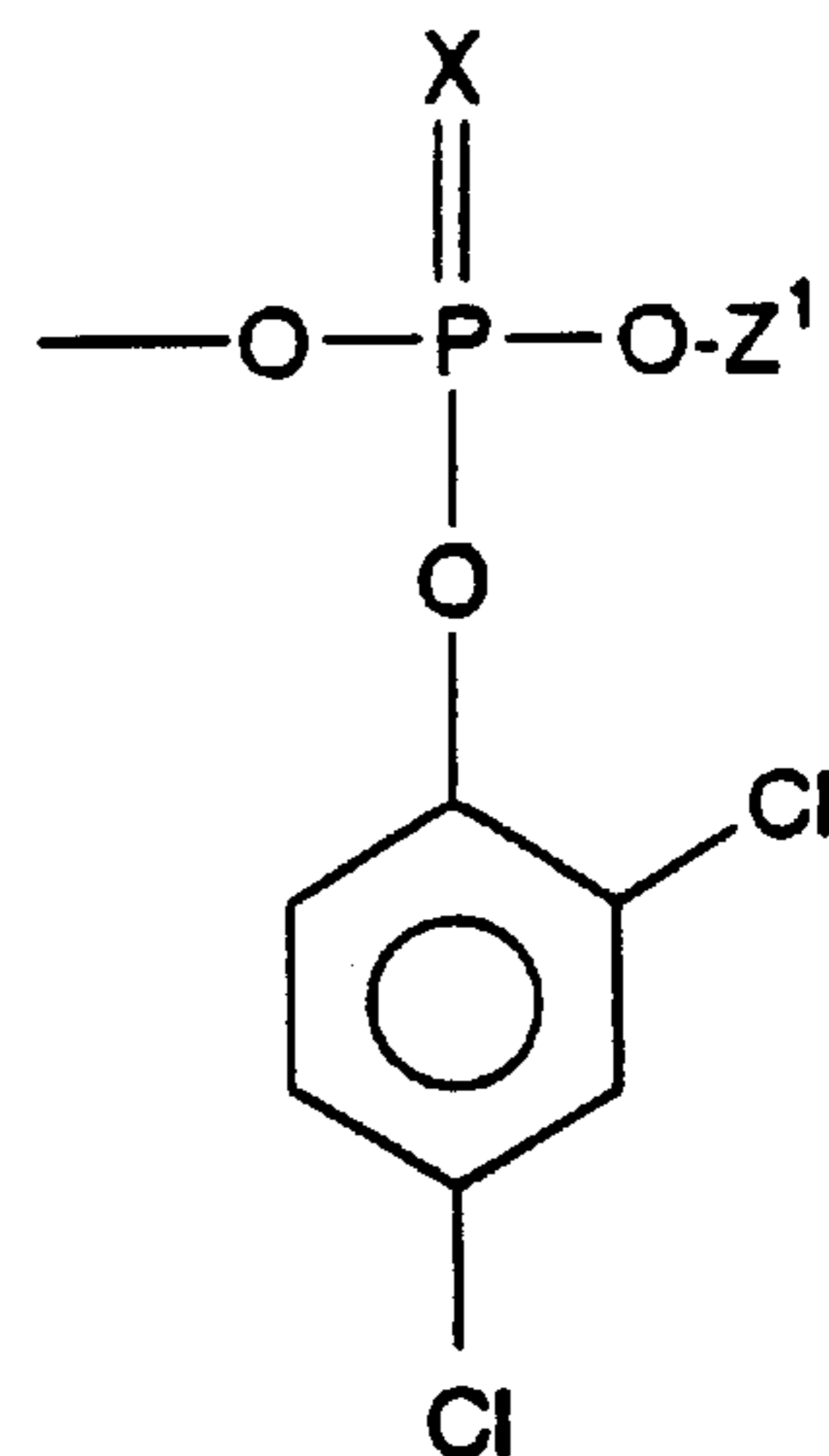
2,4-dichlorophenyl phosphate
