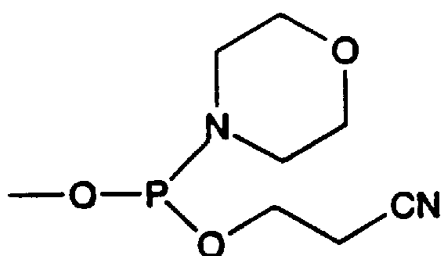
N-morpholino-β-cyanoethoxyphosphine
