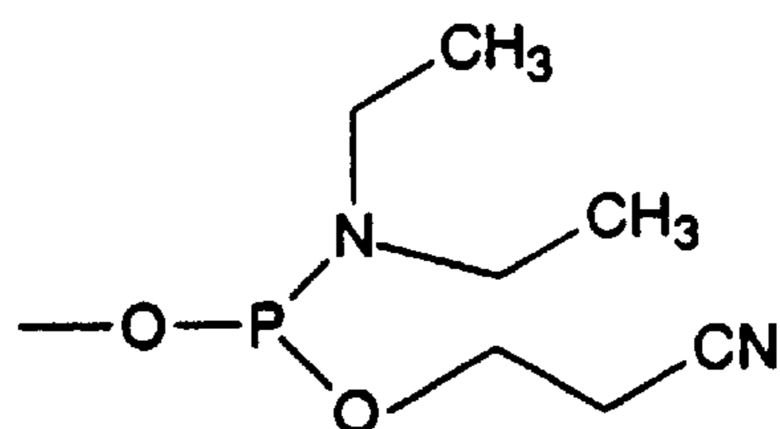
N,N-diethylamino-β-cyanoethoxyphosphine
