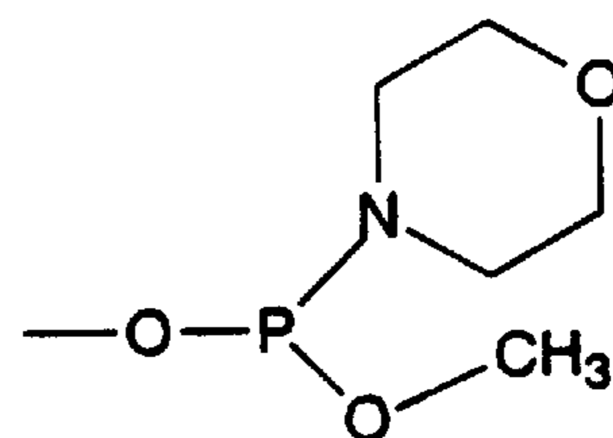
N-morpholino methoxyphosphine
