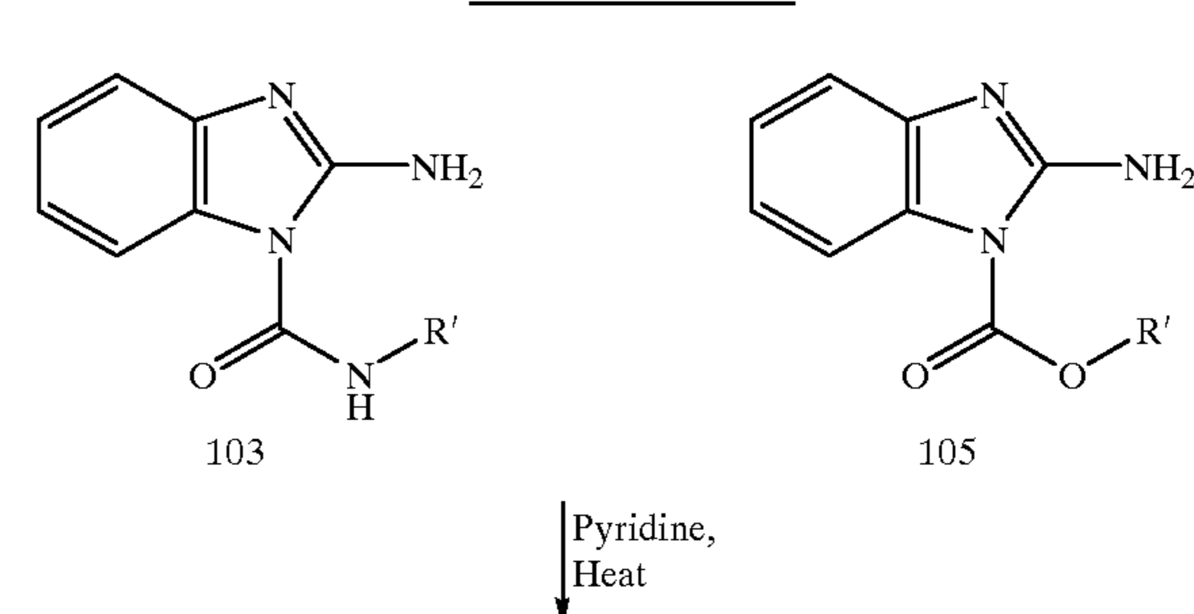
Reaction Scheme 2:
