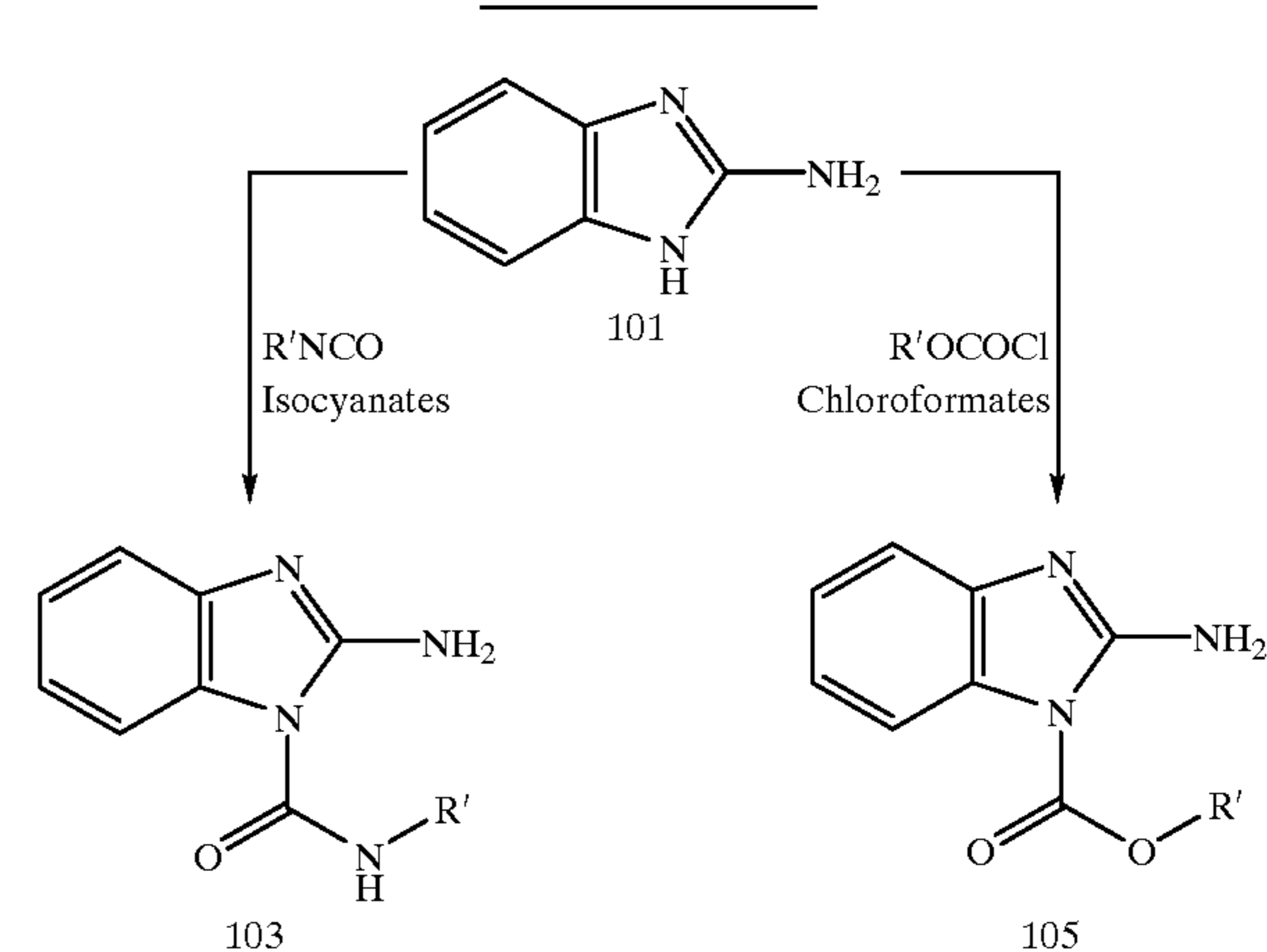
Reaction Scheme 1:
