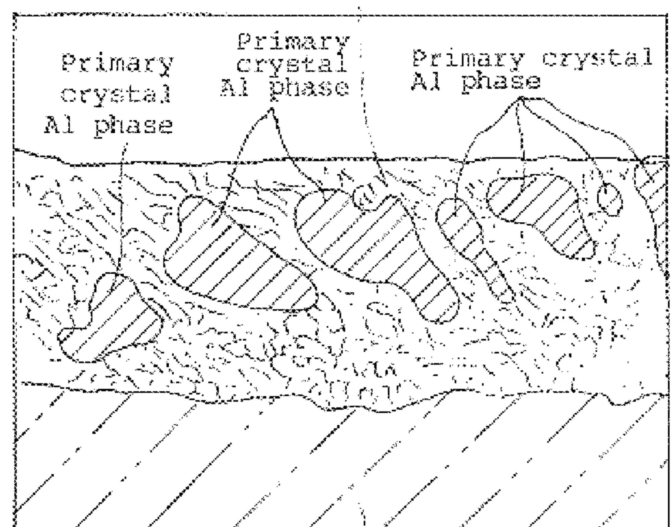
[Al/Zn/Zn 2 Mg ternary eutectic structure]
