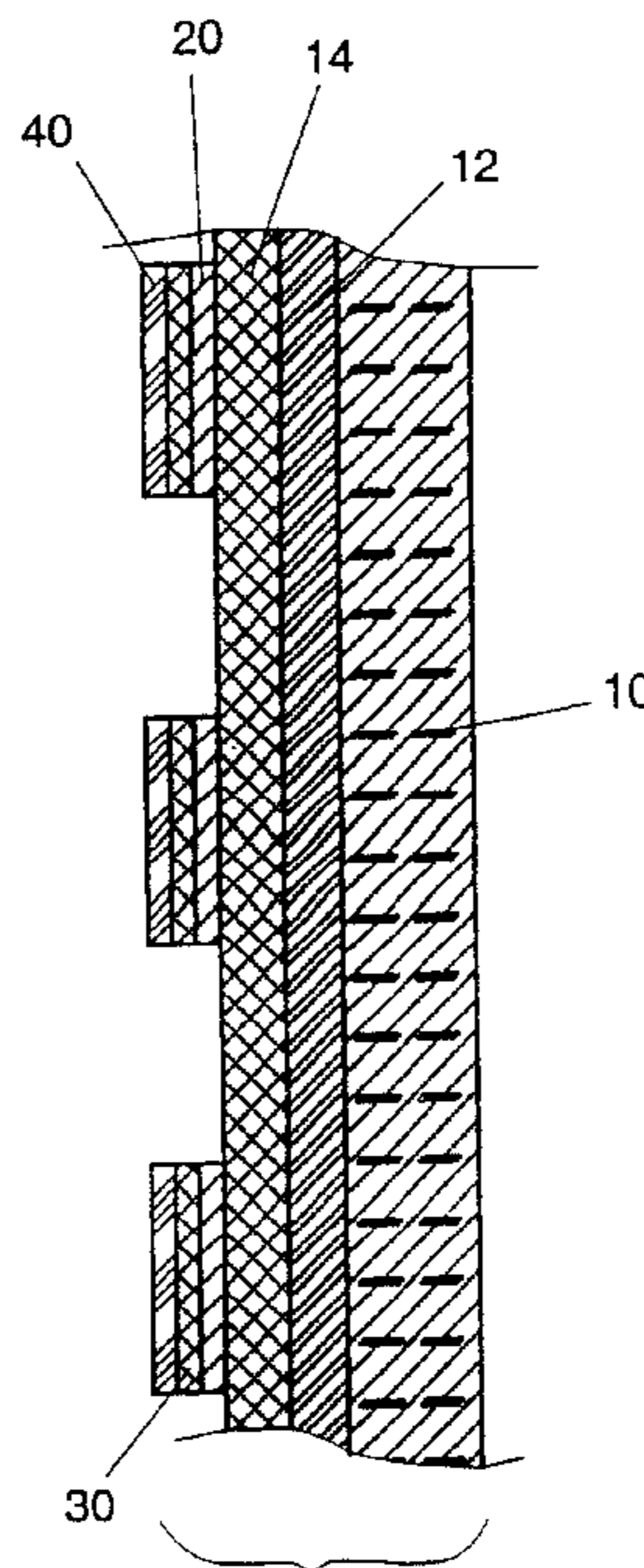
LABEL & SUBSTRATE EXPLODED VIEW
