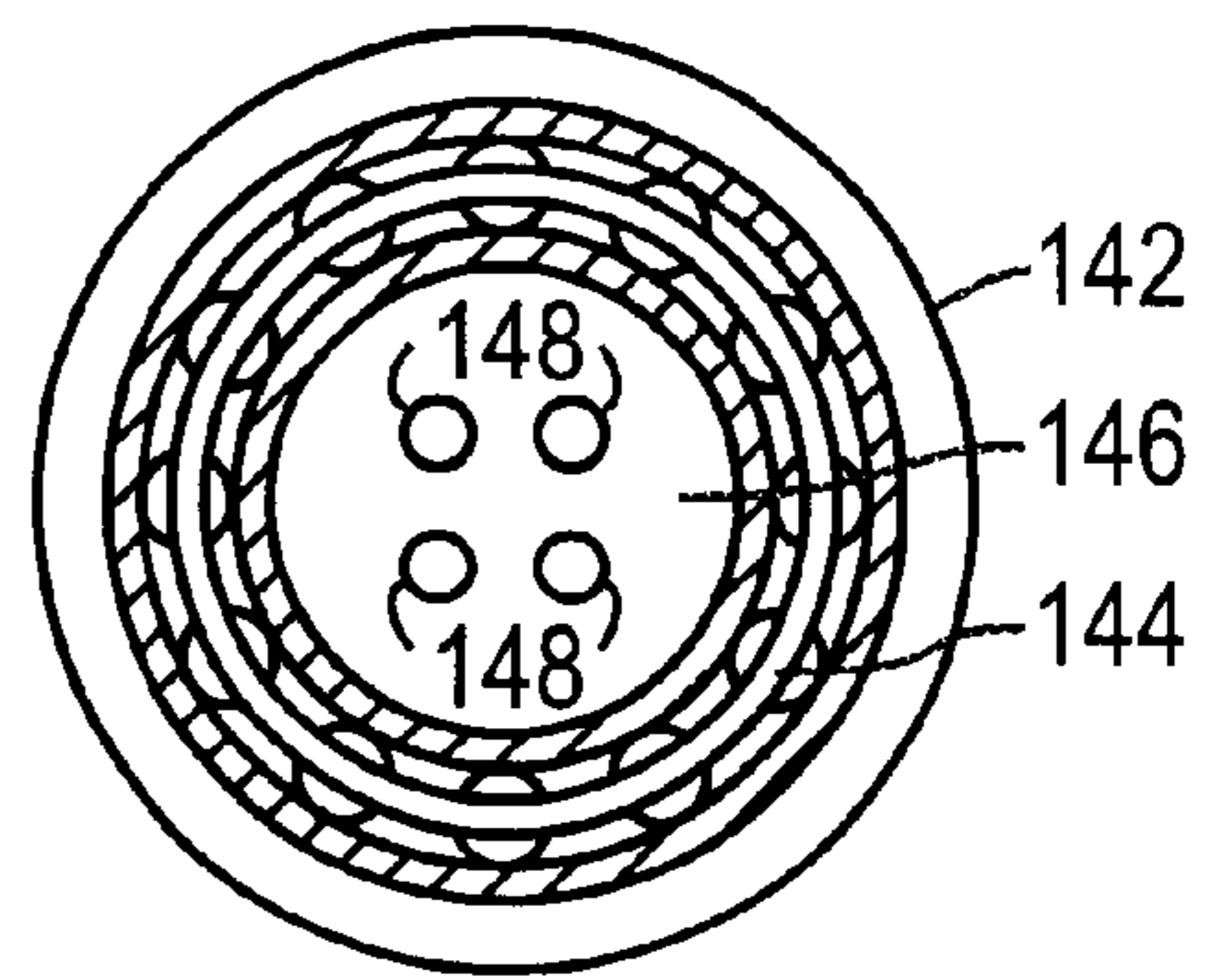
SECTION B-B FIG. 2D
