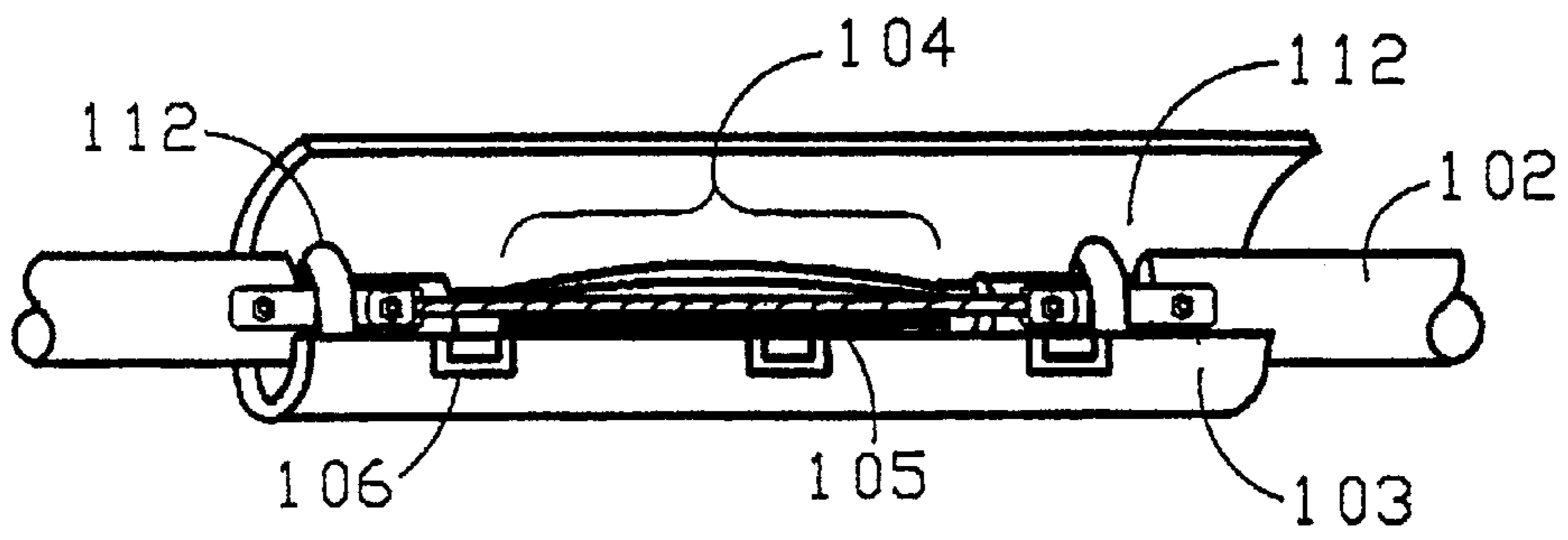
Fig. 3 PRIOR ART
