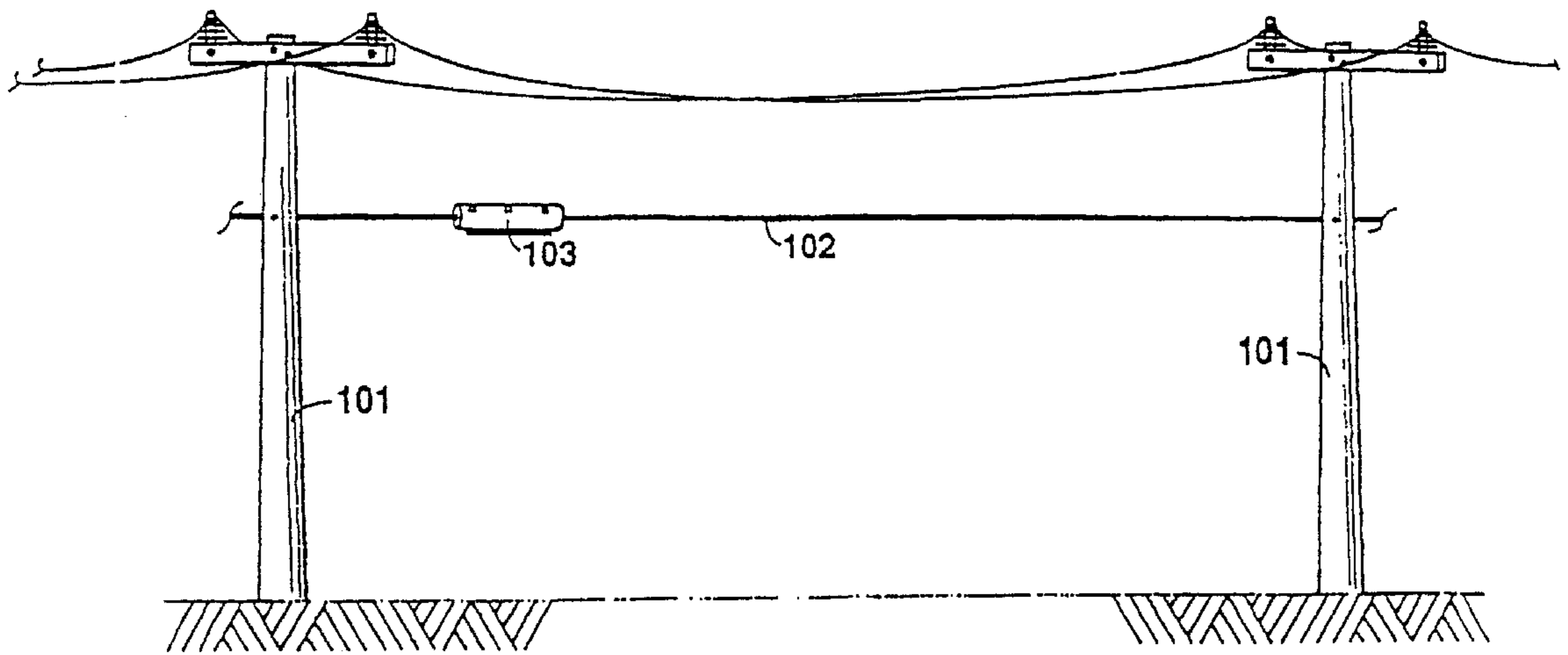
Fig. 1 PRIOR ART
