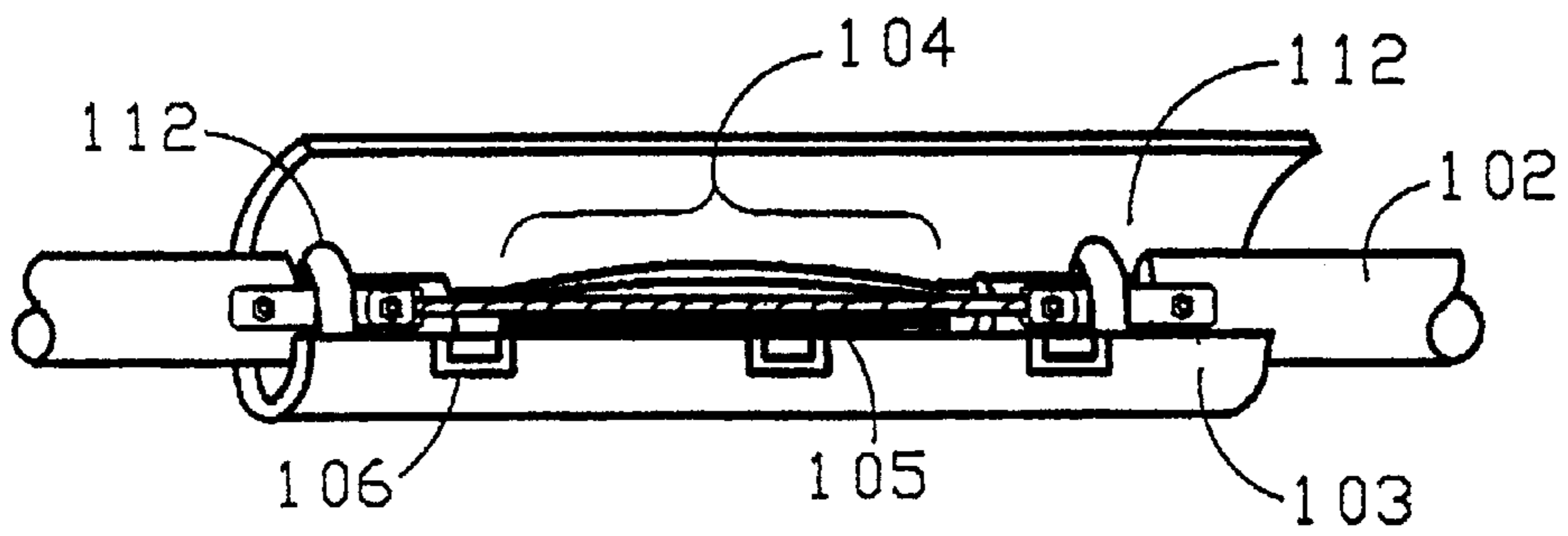
Fig. 3 PRIOR ART
