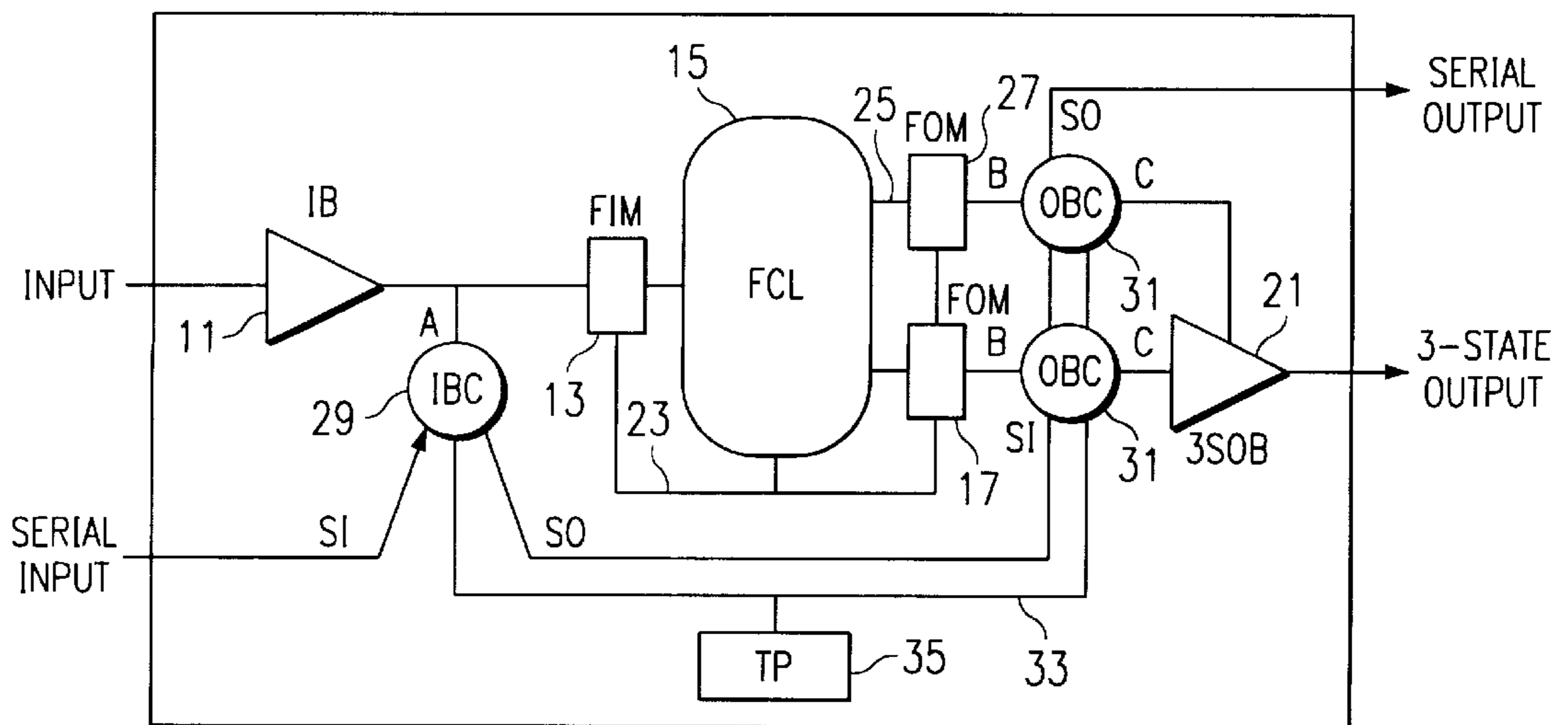
FIG. 4 (PRIOR ART)
