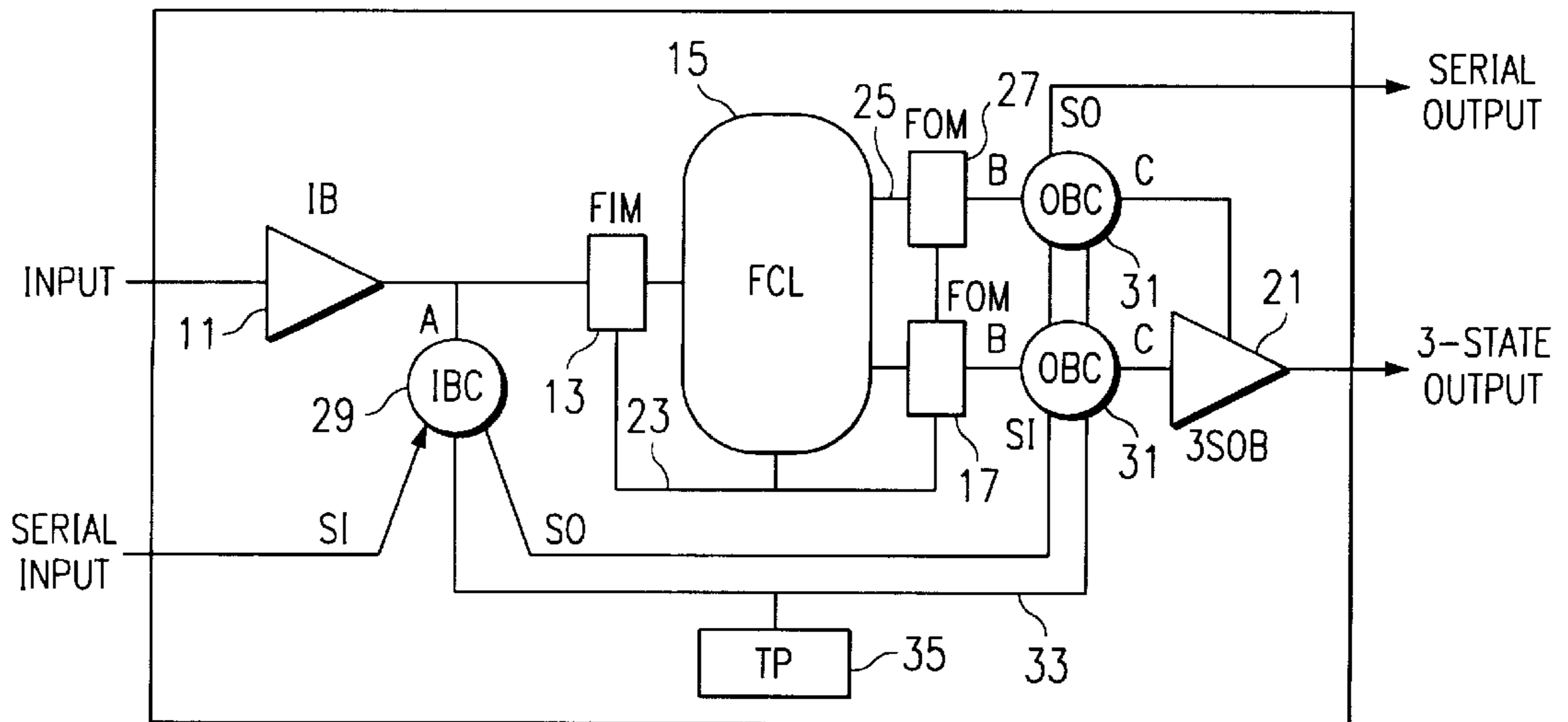
FIG. 4 (PRIOR ART)
