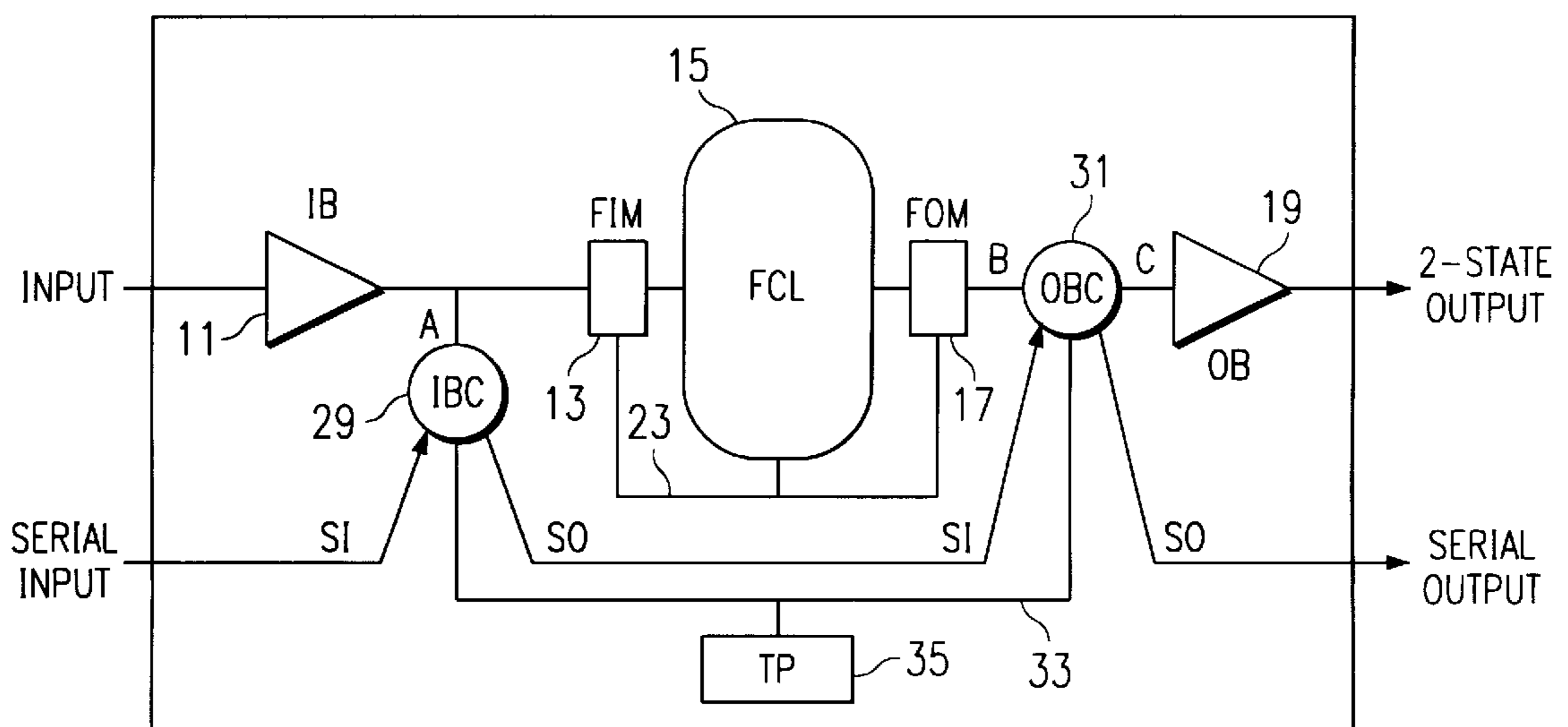
FIG. 3 (PRIOR ART)
