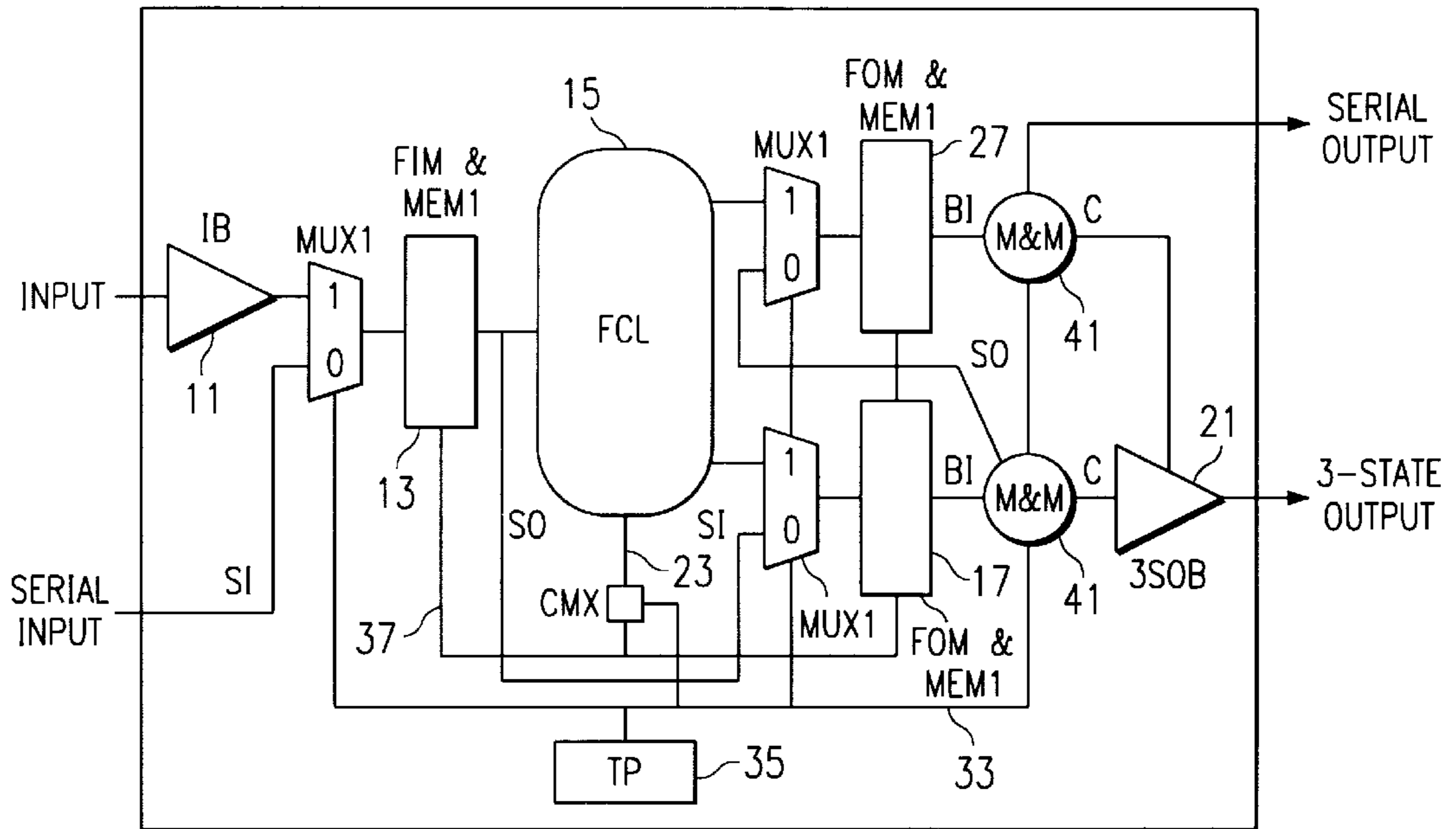
FIG. 6 (PRIOR ART)
