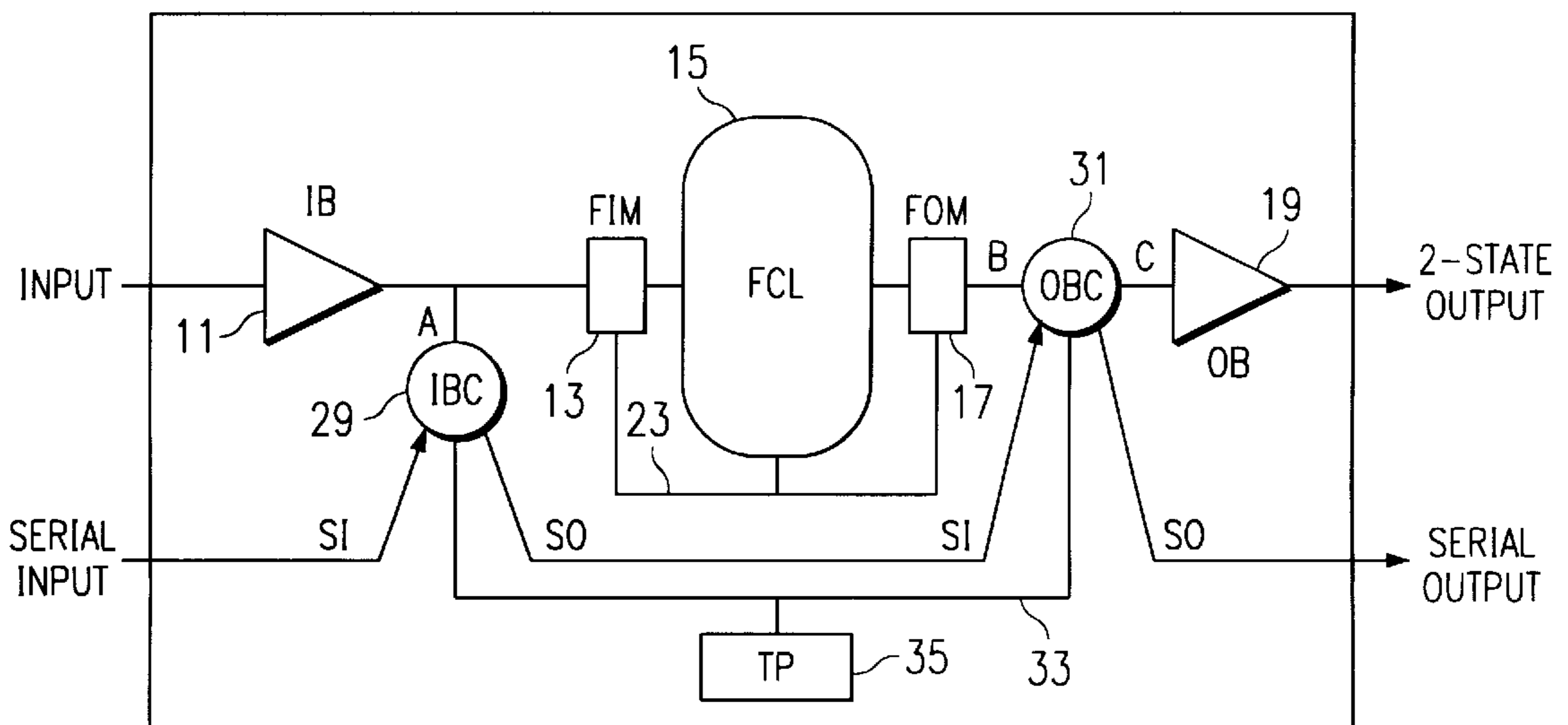
FIG. 3 (PRIOR ART)
