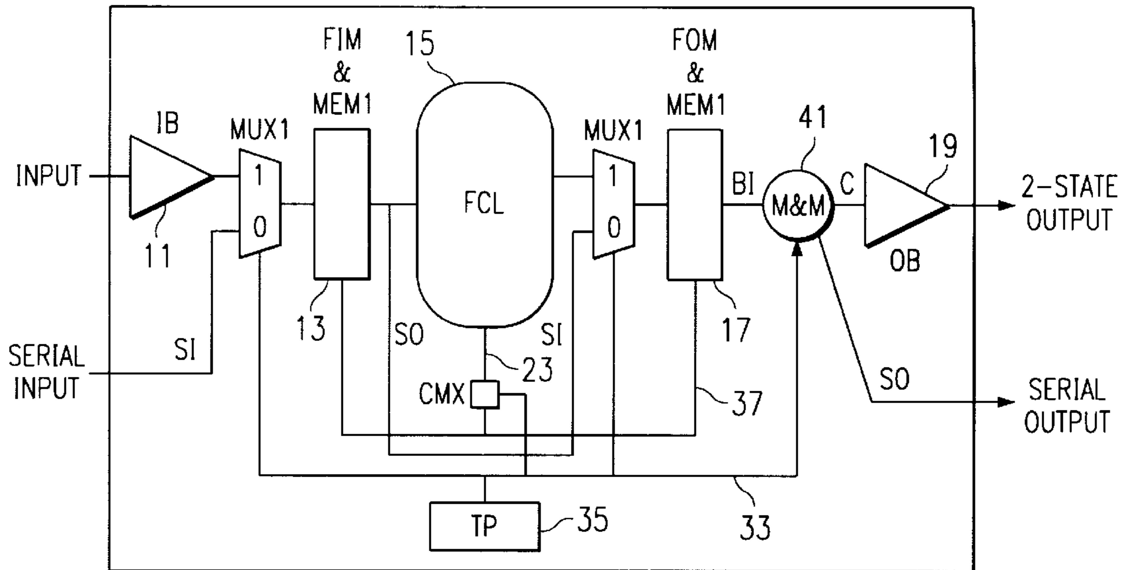
FIG. 5 (PRIOR ART)
