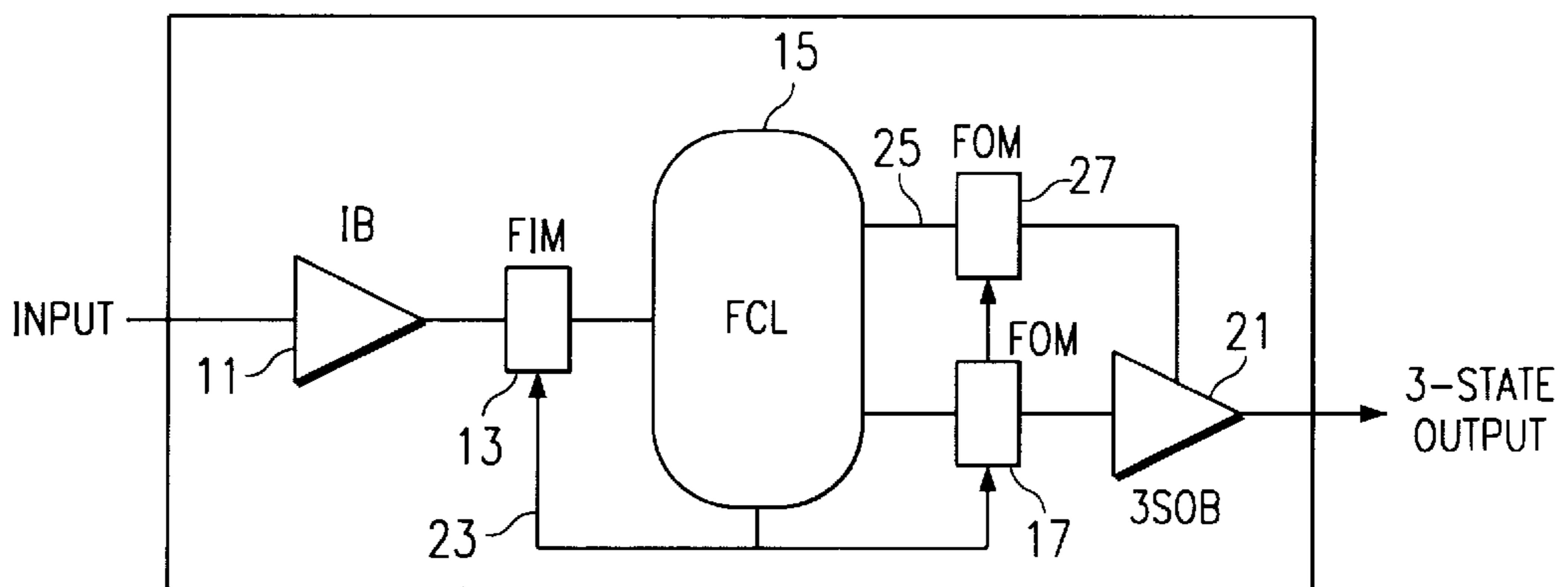
FIG. 2 (PRIOR ART)
