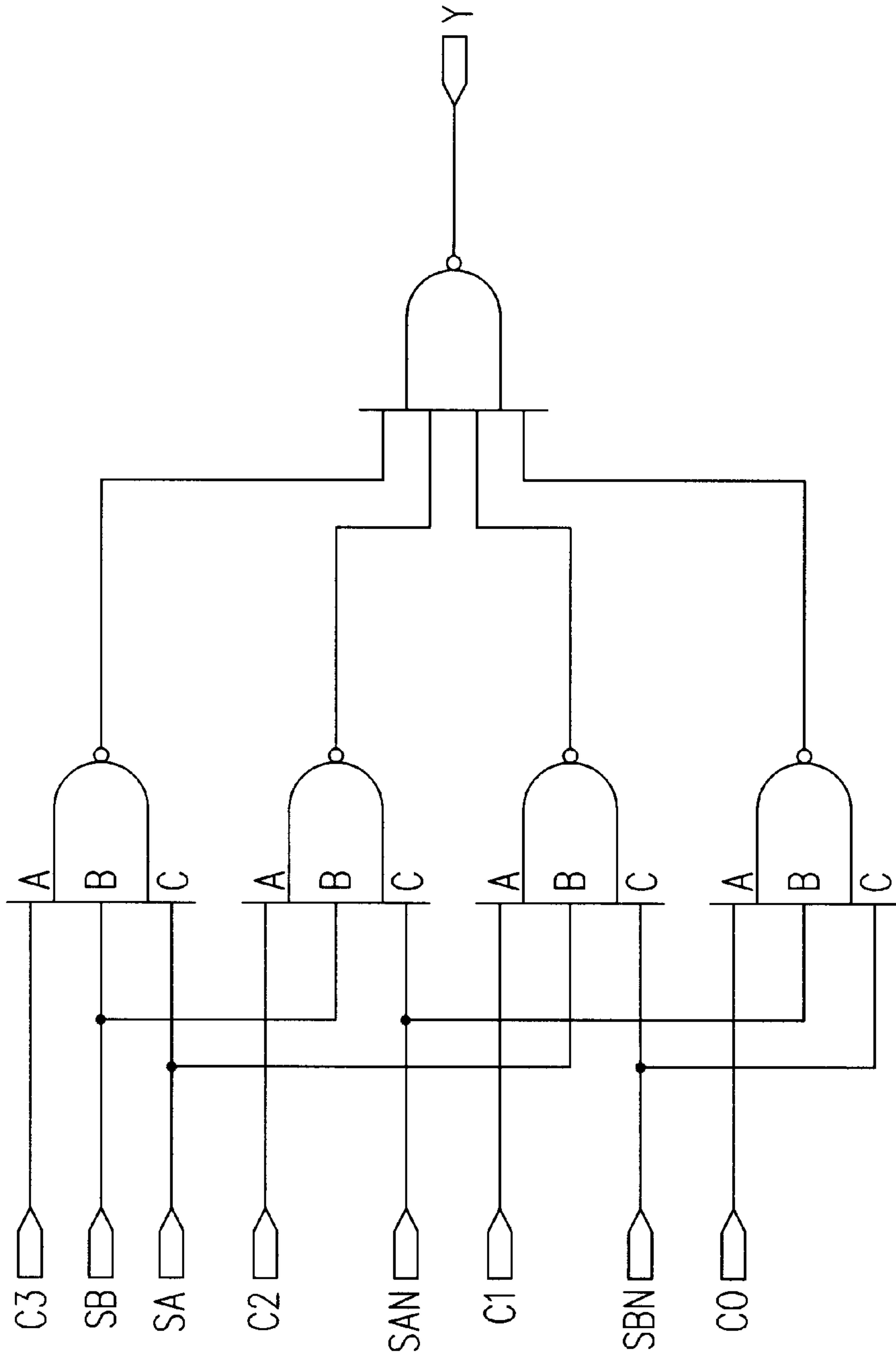
4:1 SELECTOR
