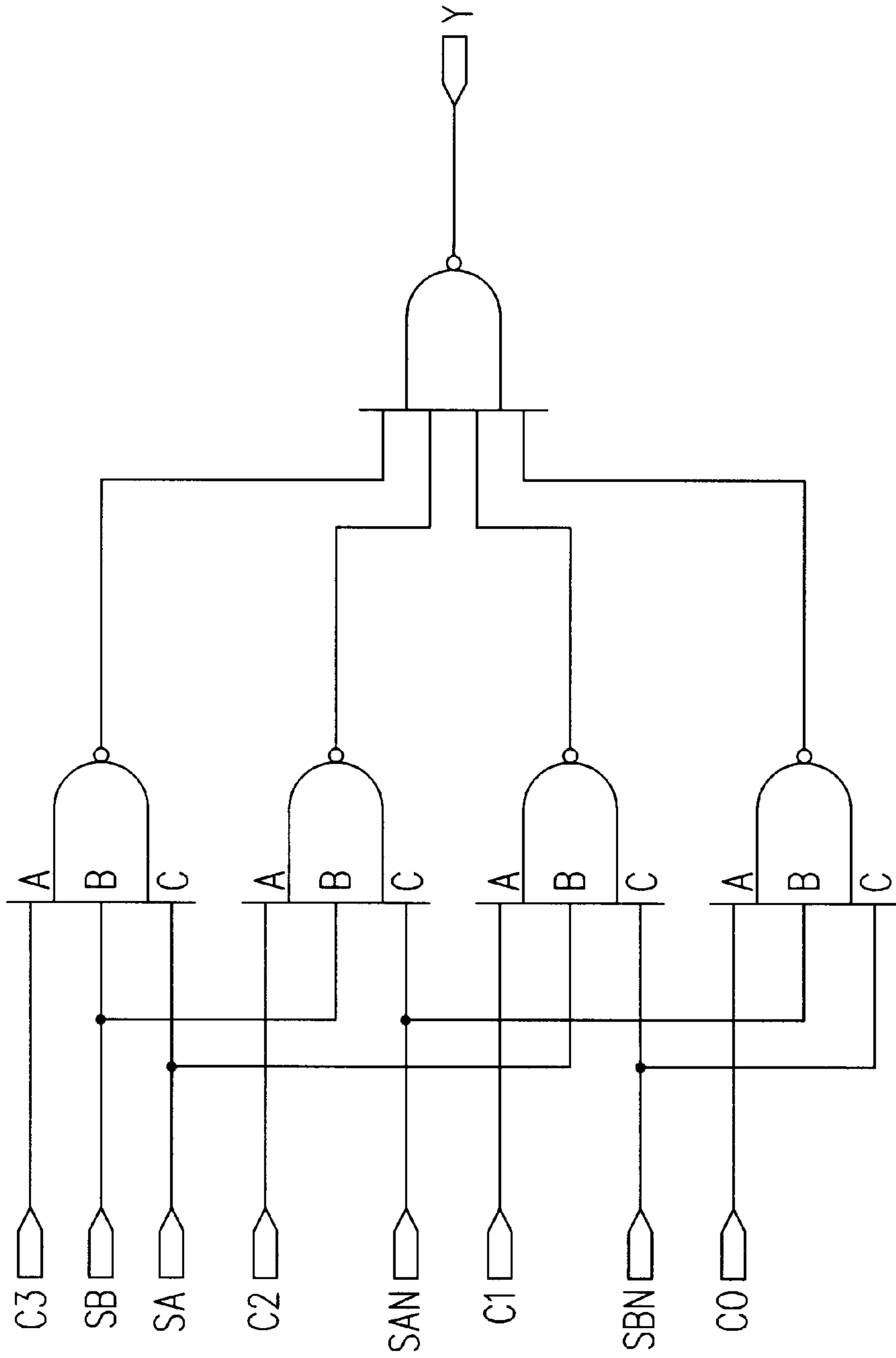
4:1 SELECTOR
