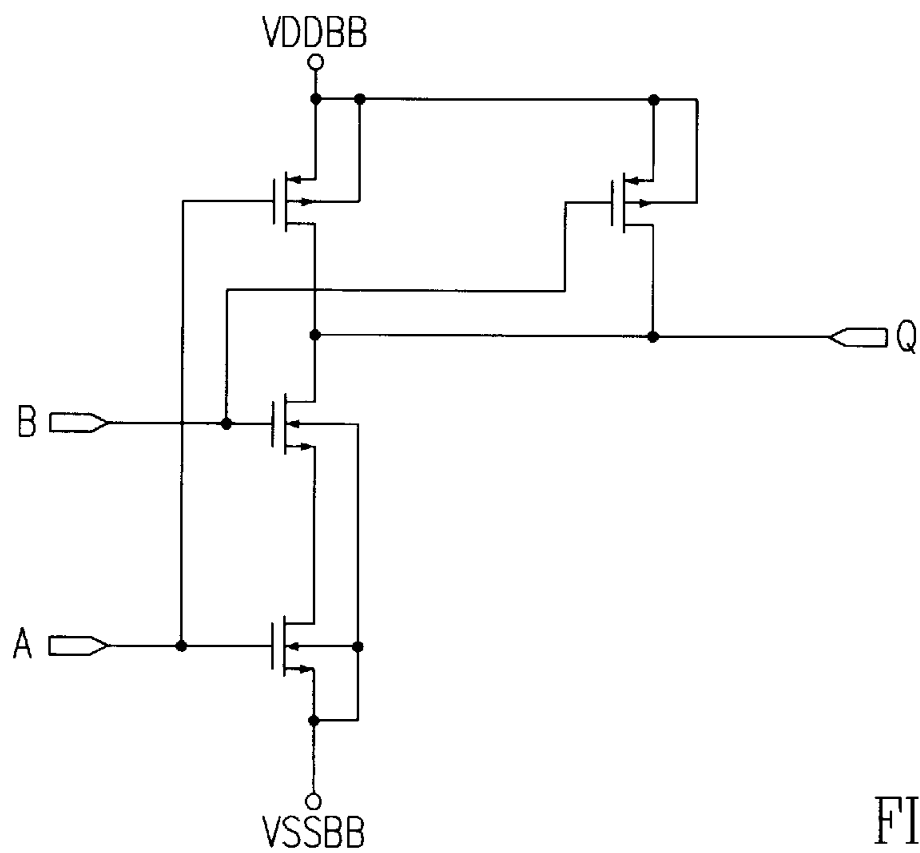
NAND2
