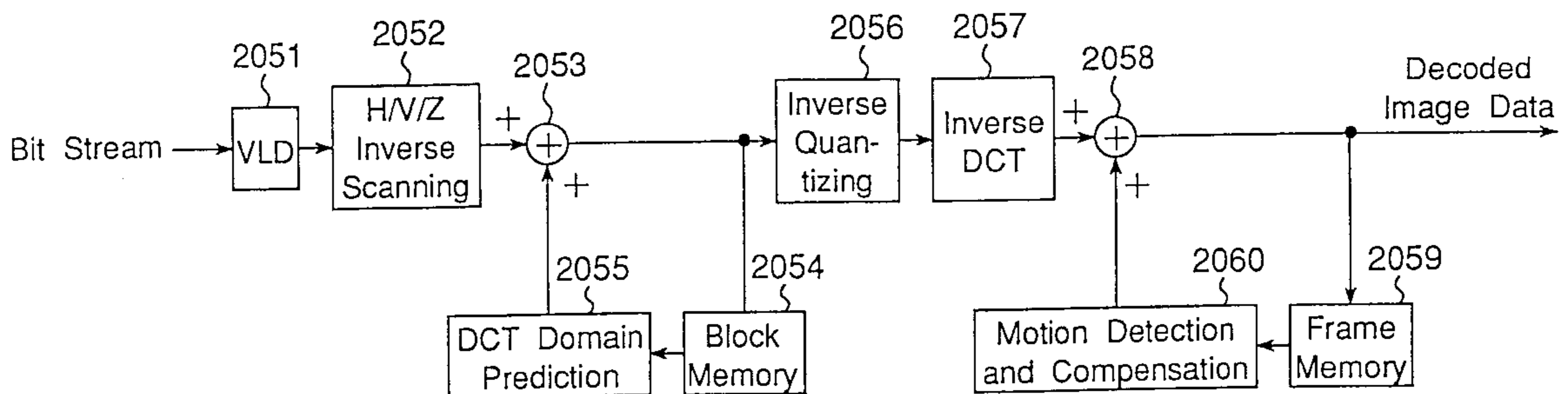
Eighth Preferred Embodiment Image Predictive Decoding Apparatus
