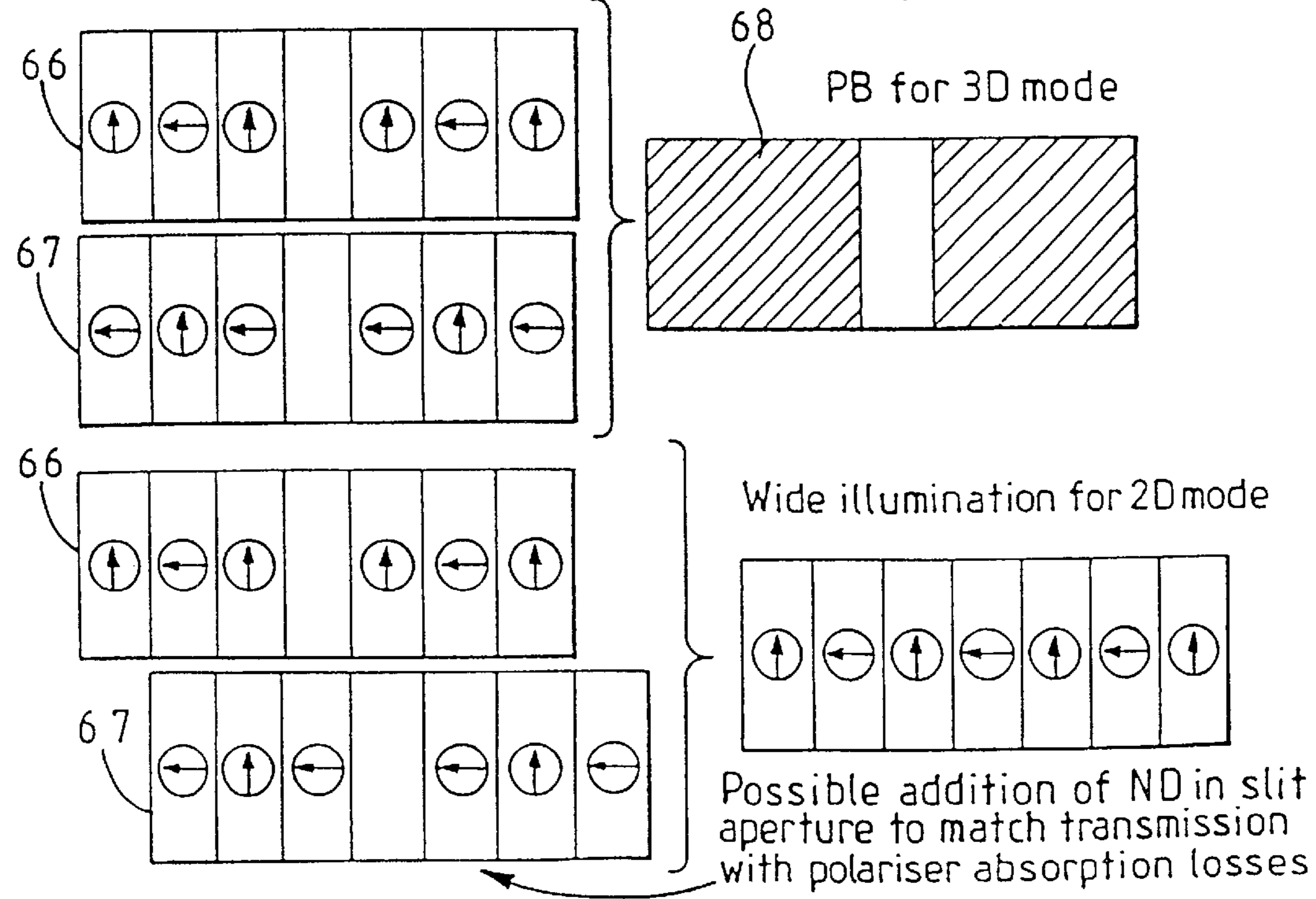
FIG 15 Two moving masks/polarisers approach
