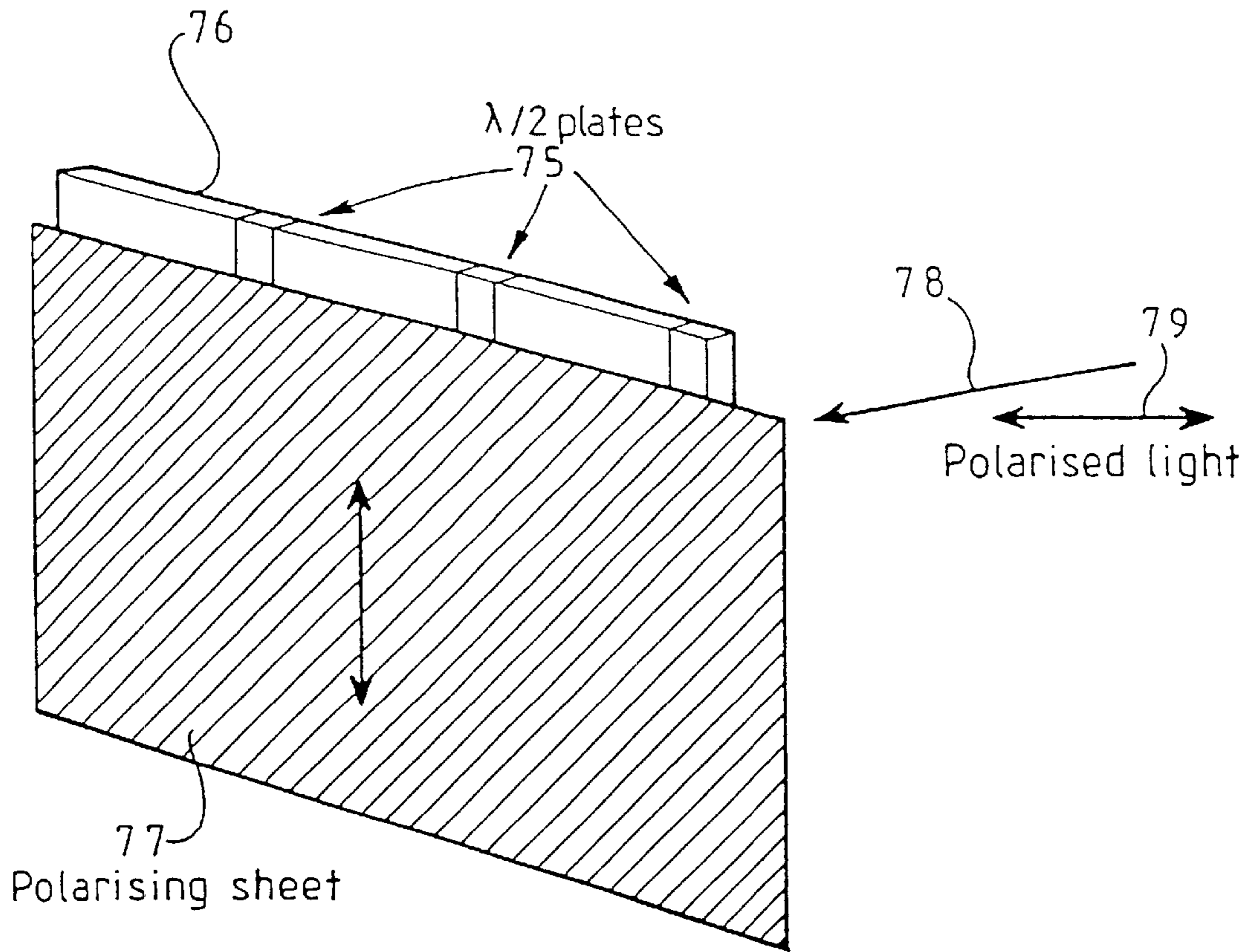
FIG 16 Basic two-element reversible parallax barrier element
