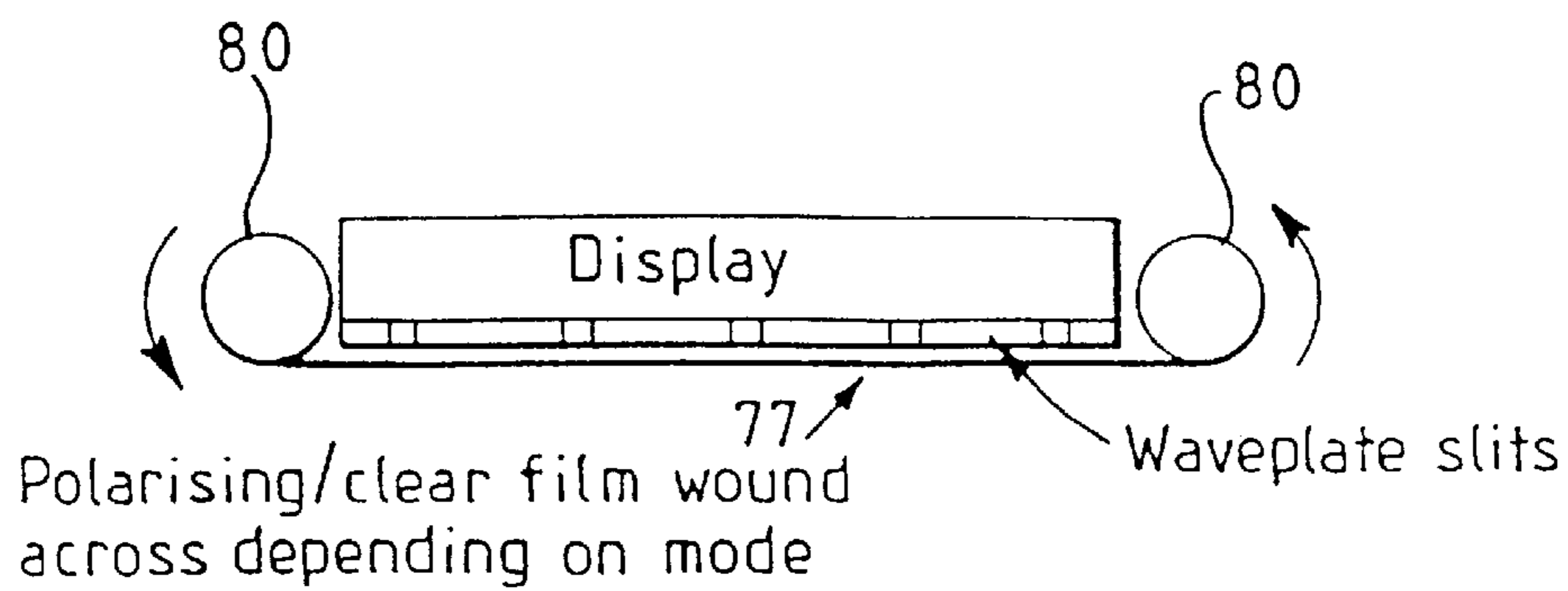
FIG 17 Embodiment with polarising film
