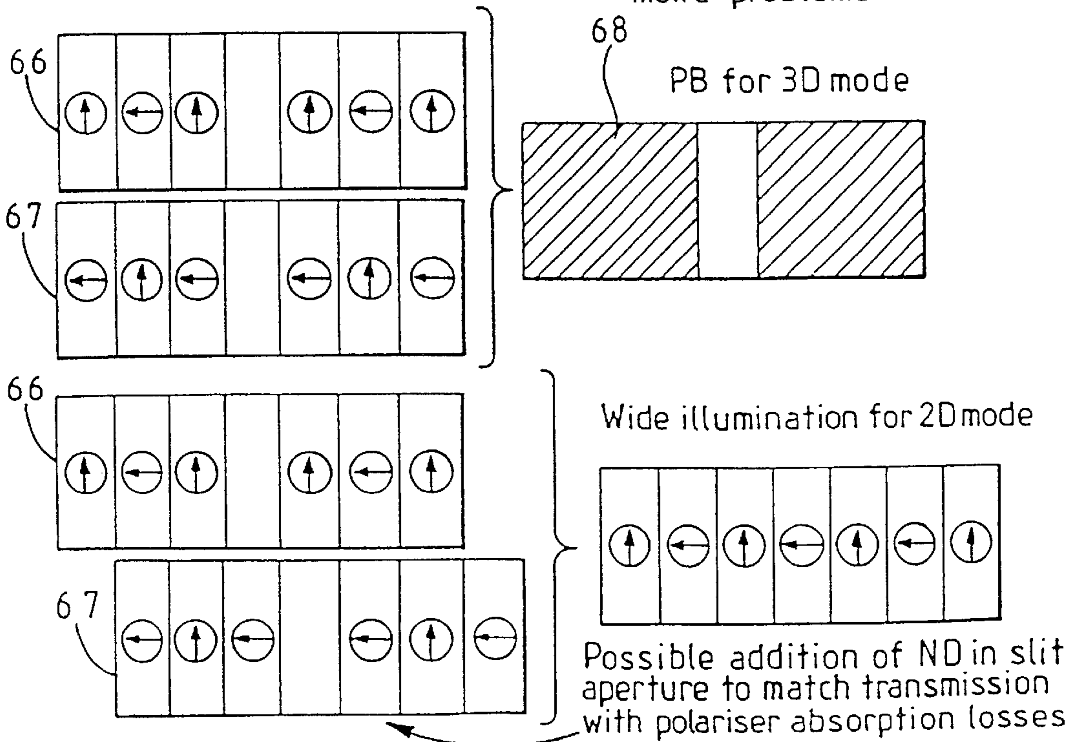
FIG 15 Two moving masks/polarisers approach
