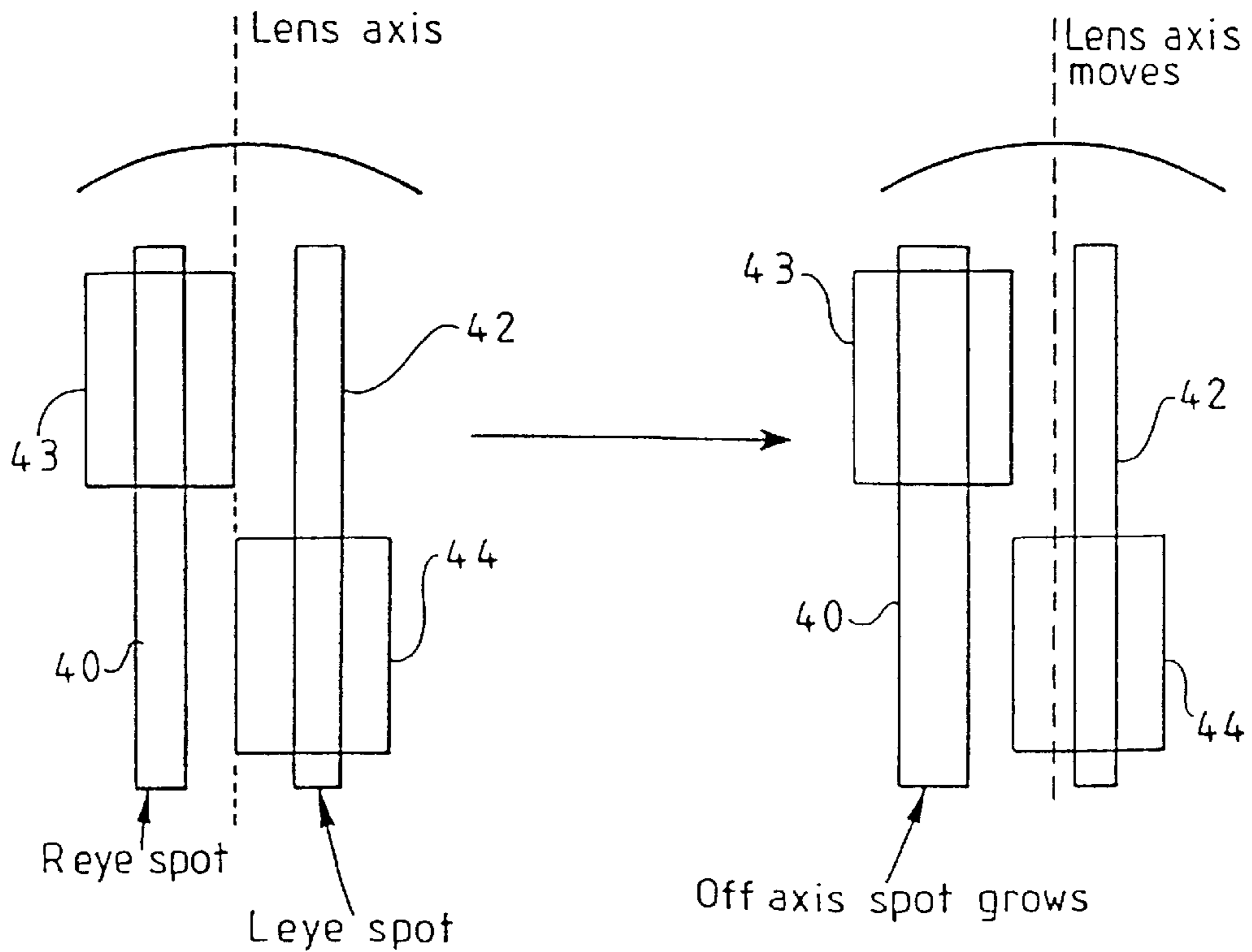
FIG 8 Effect of lateral tracking
