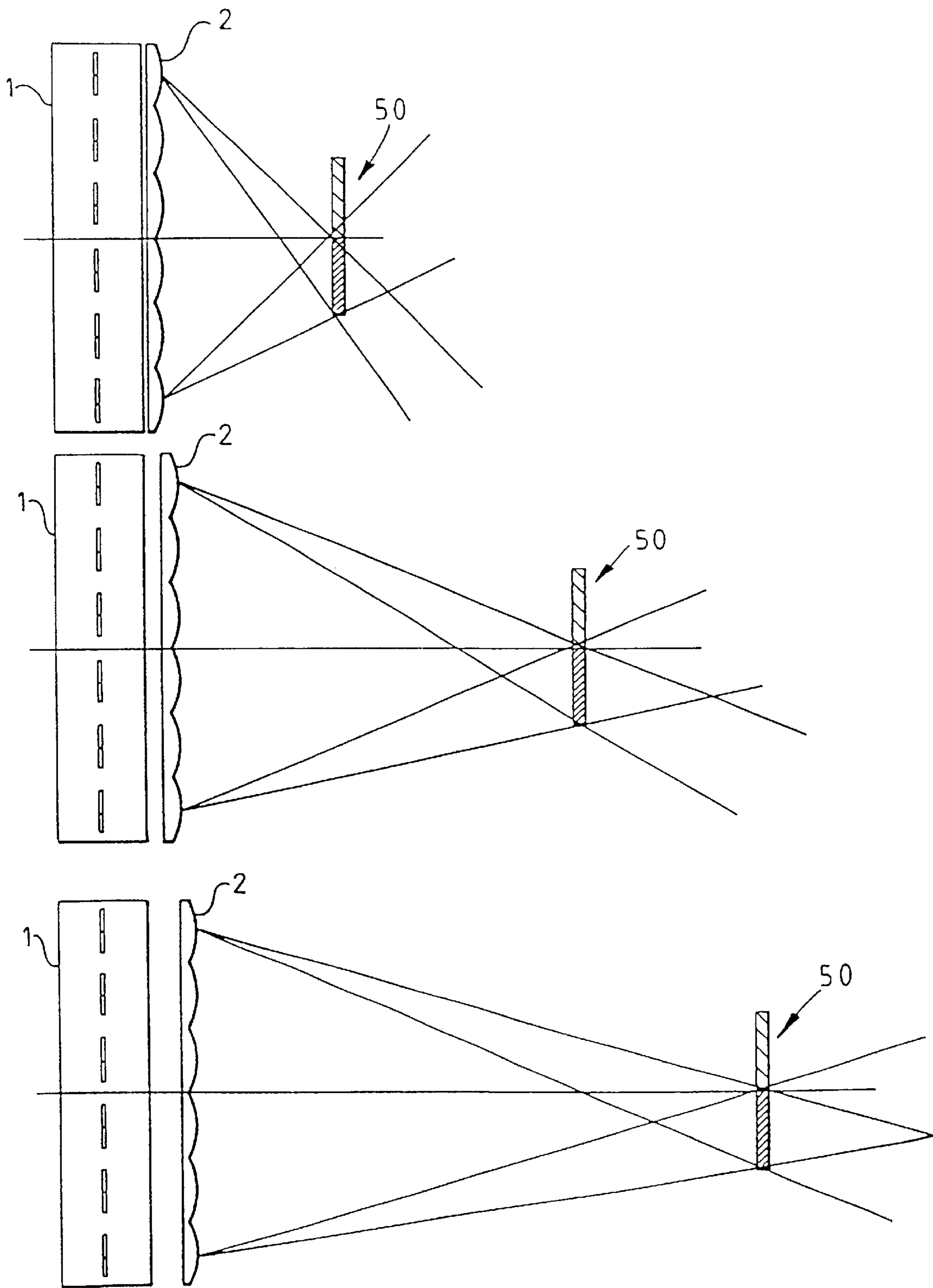
FIG 11 Quantised longitudinal tracking in mechanically tracked 3D displays
