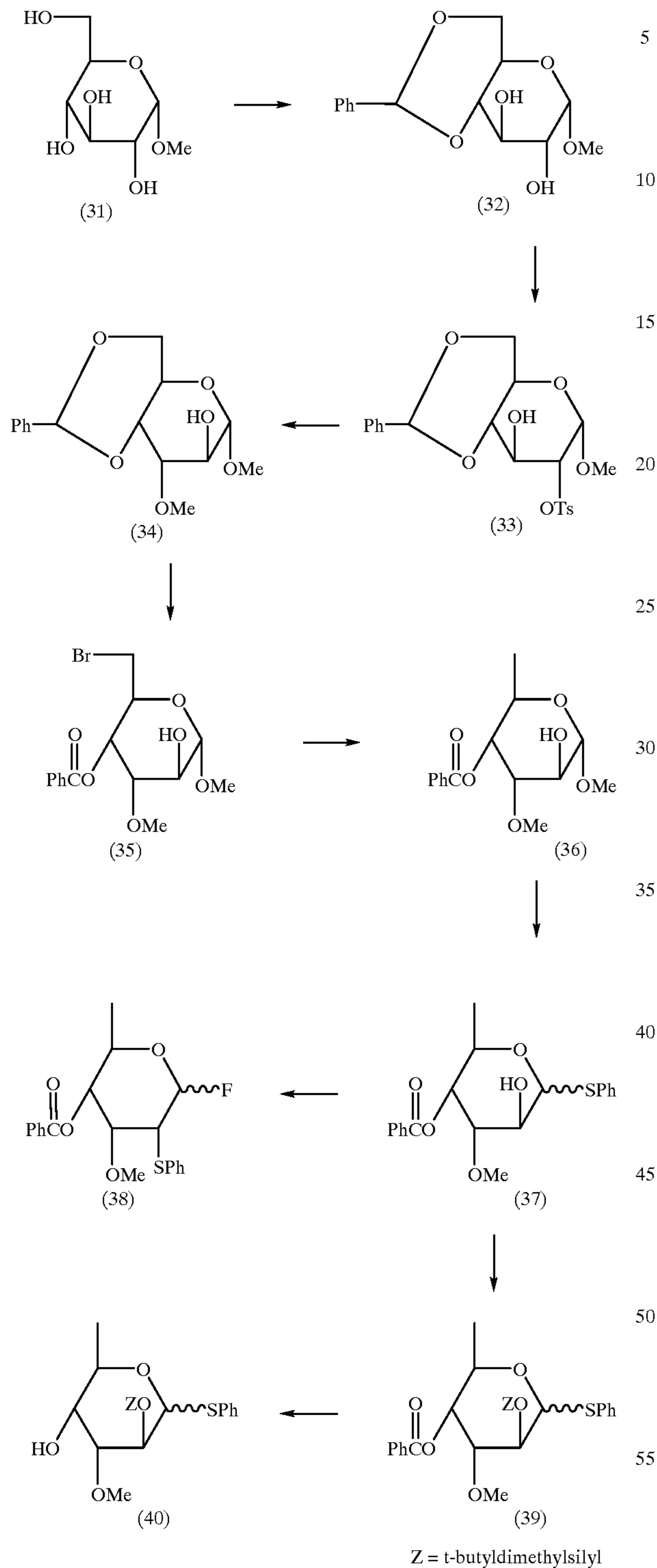
Reaction Scheme C
