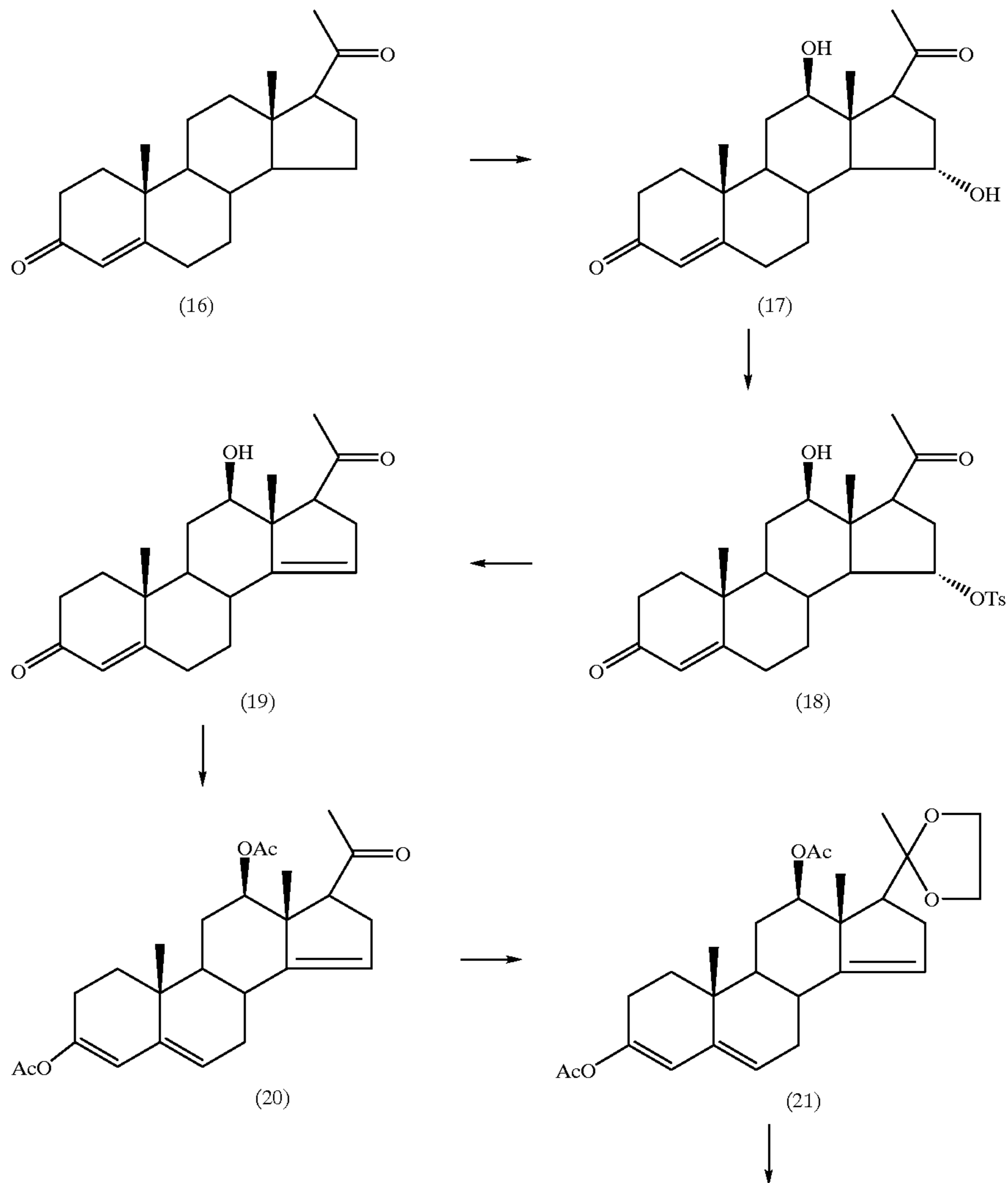
Reaction Scheme A
