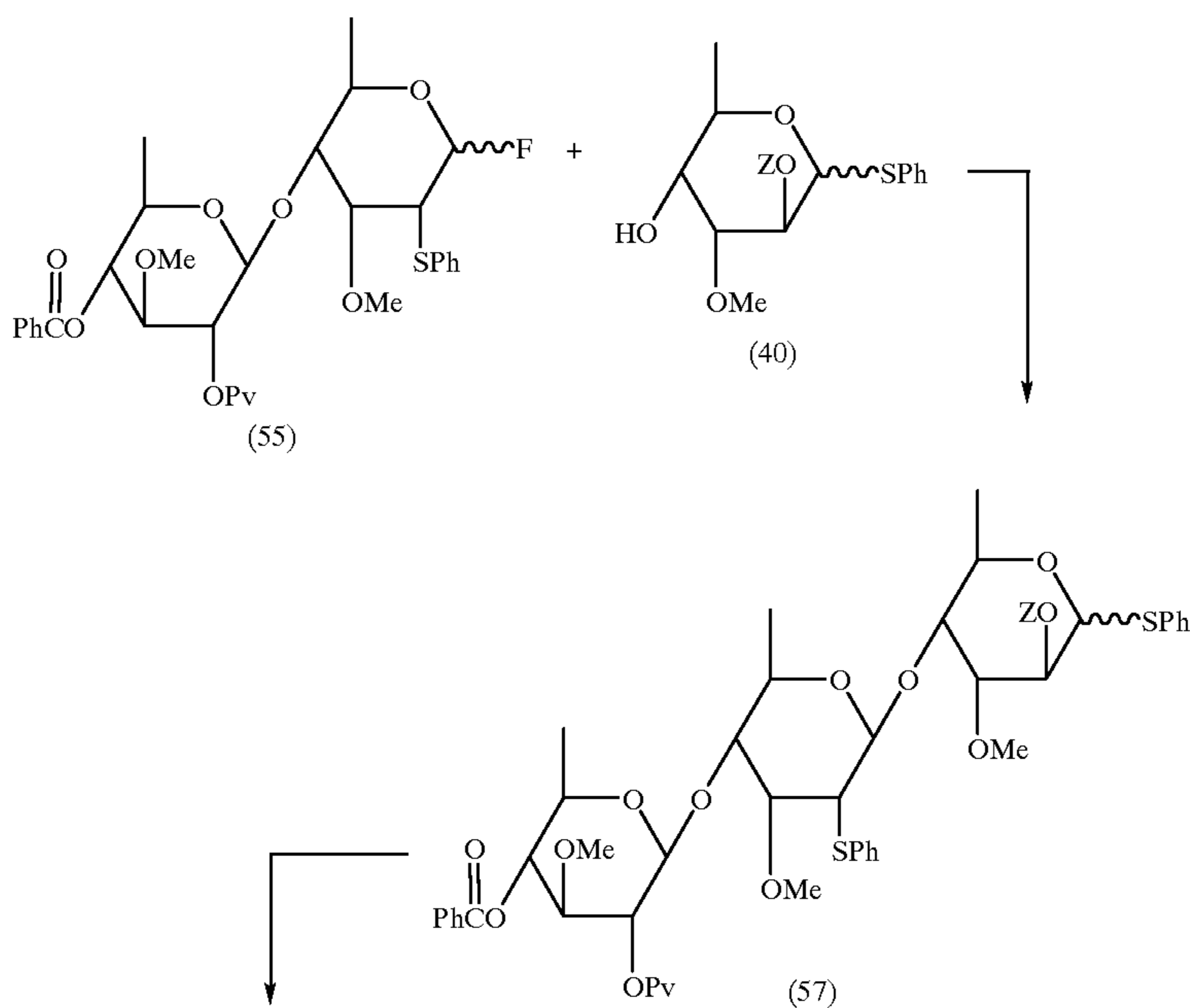
Reaction Scheme F
