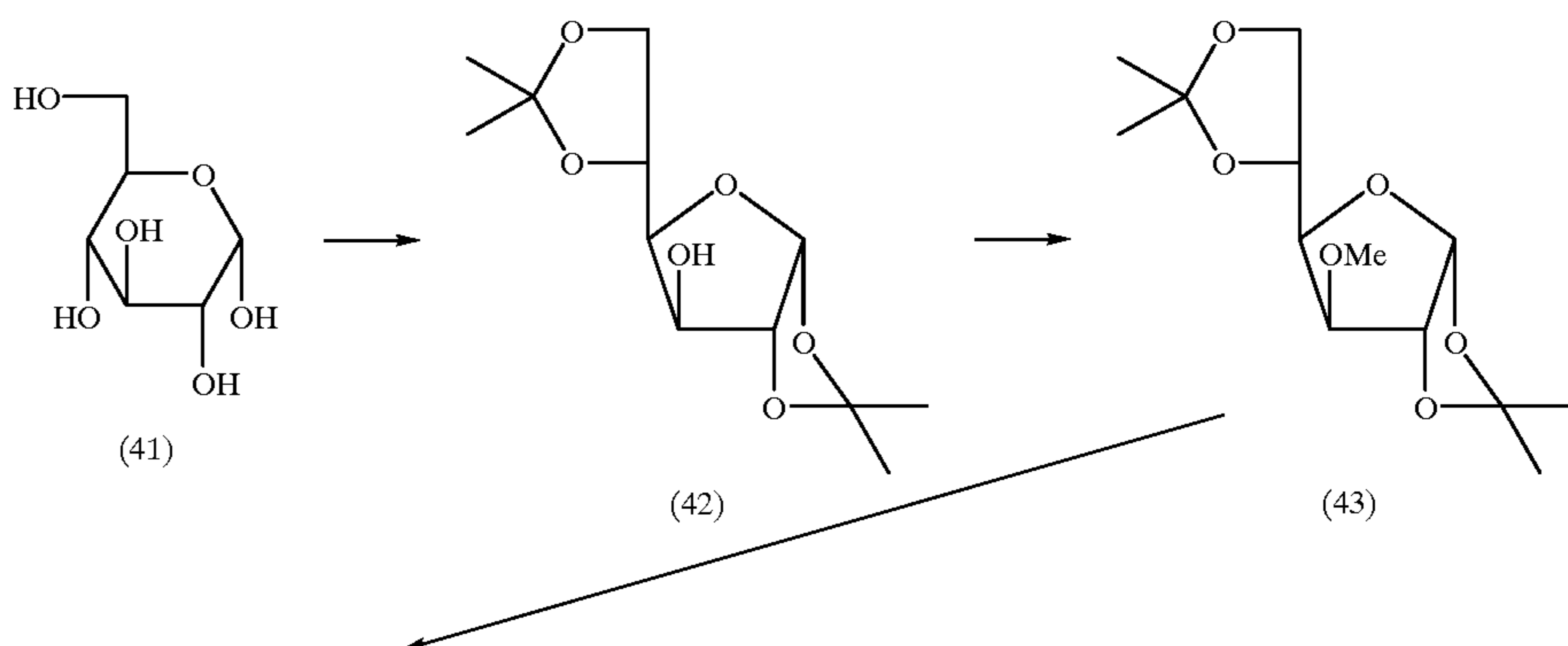
Reaction Scheme D
