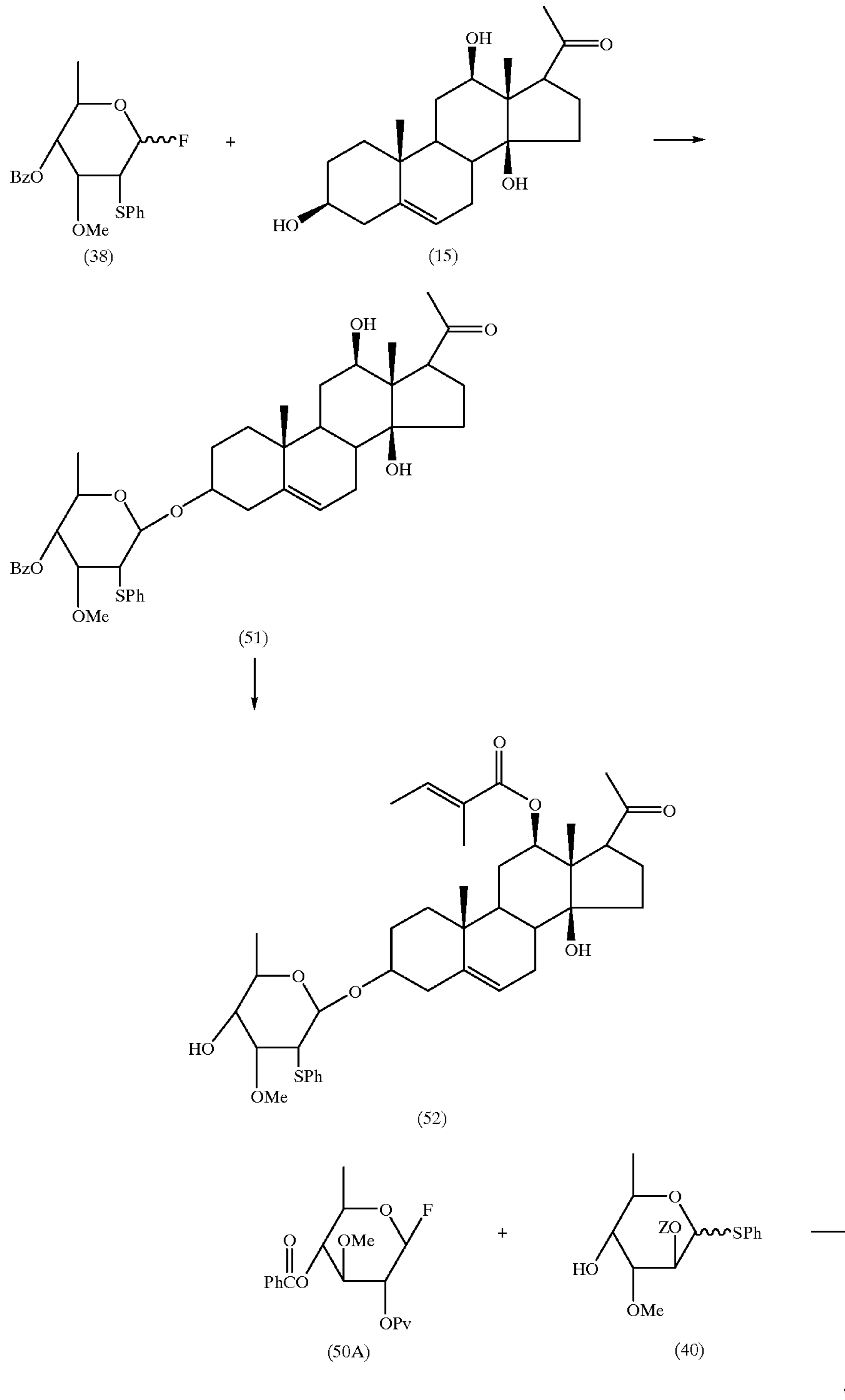
Reaction Scheme E
