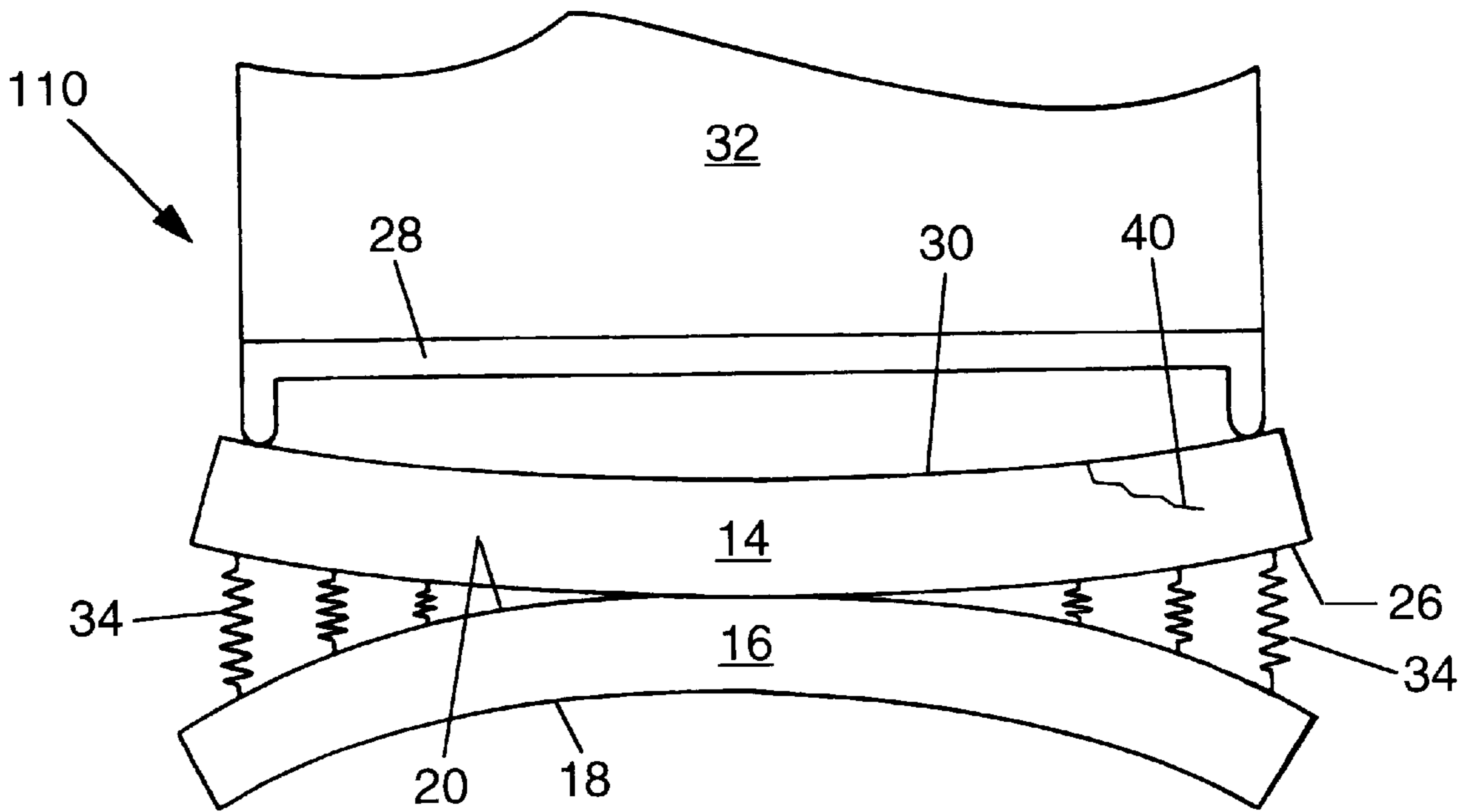
FIG. 2 PRIOR ART
