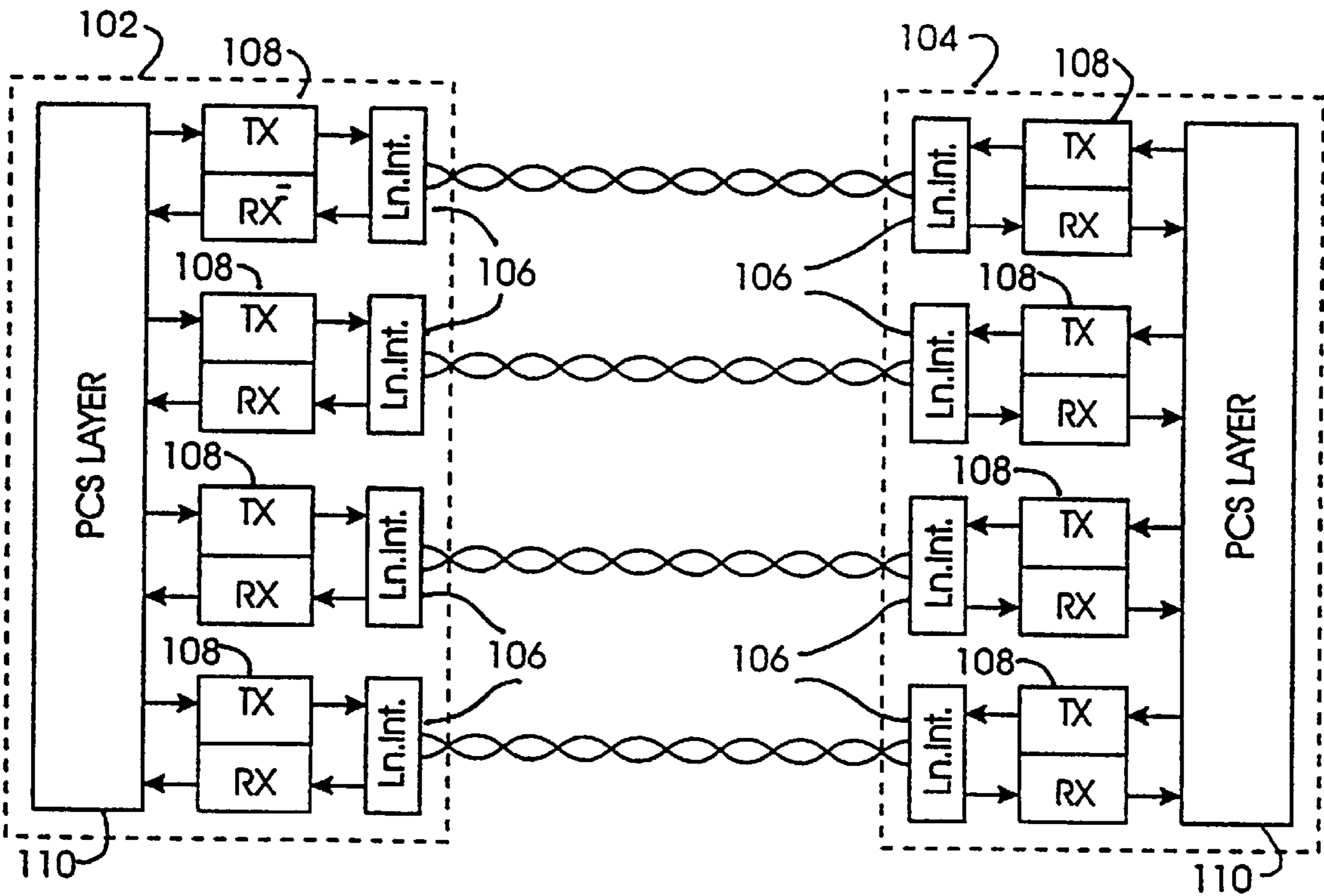
FIG. 1 PRIOR ART
