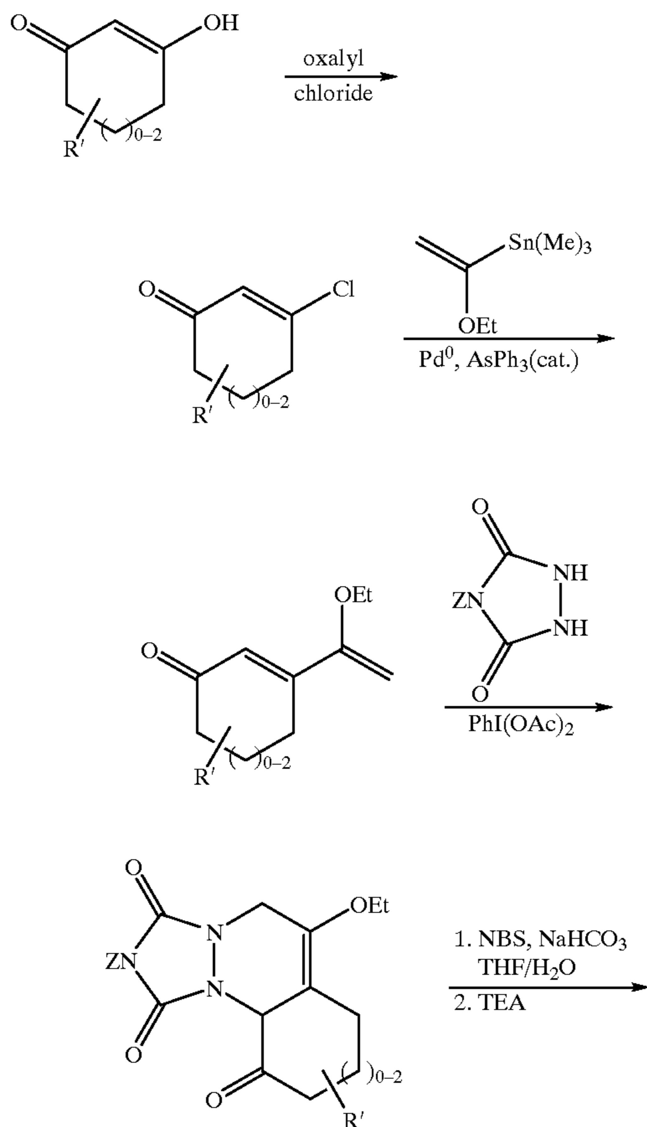
Reaction Scheme (30)
