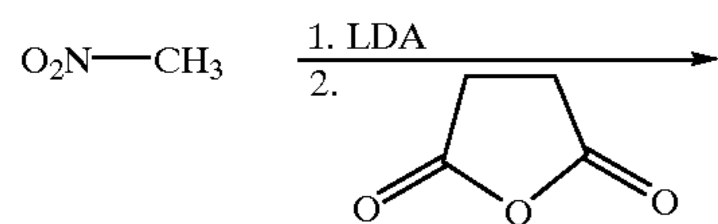
Reaction Scheme (26)
