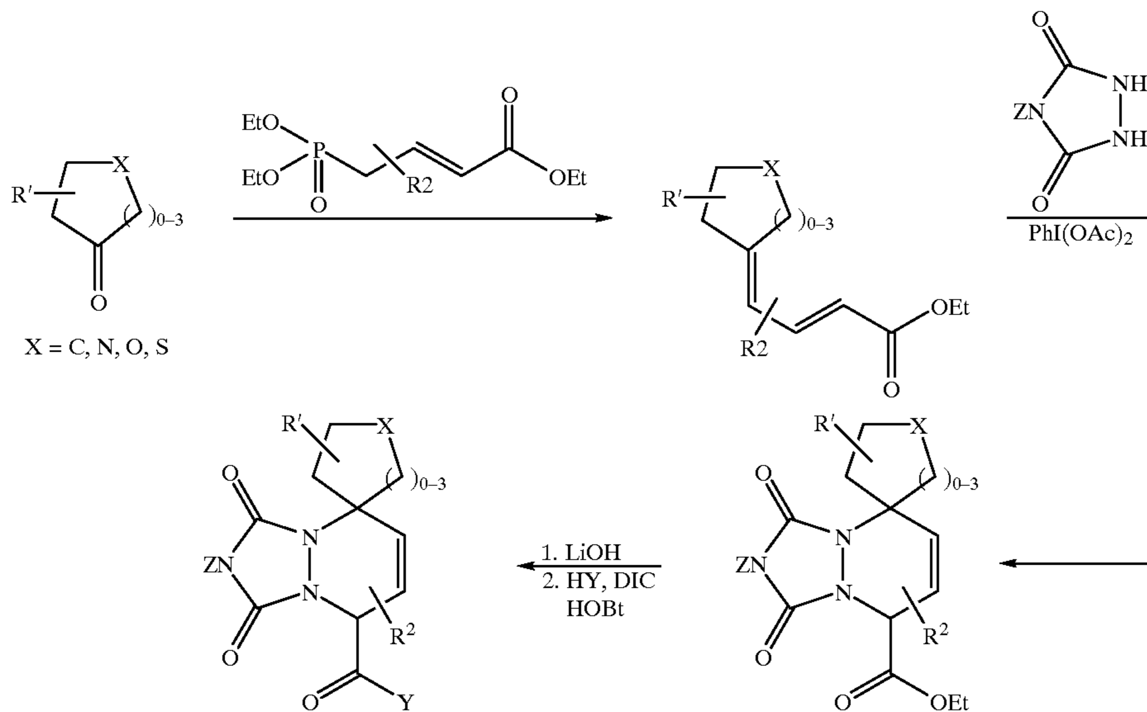
Reaction Scheme (29)
