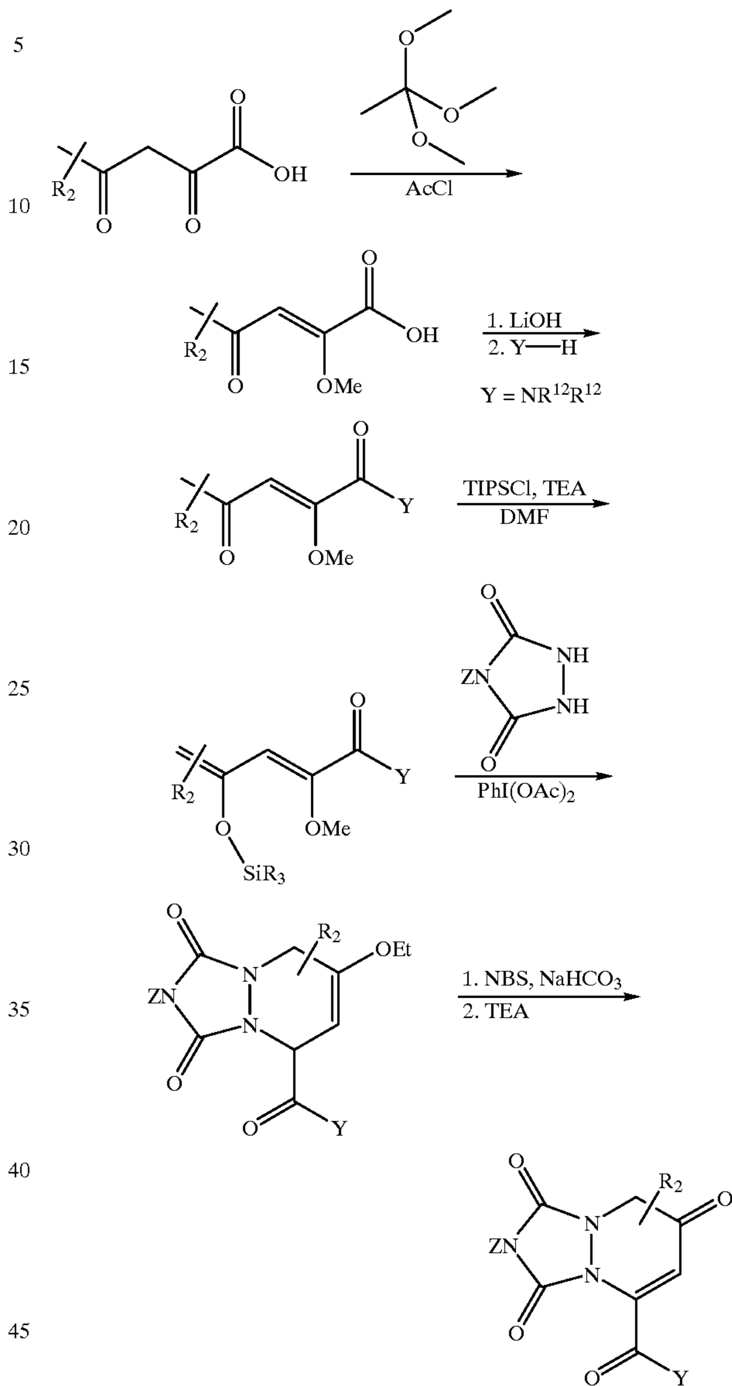
Reaction Scheme (33)
