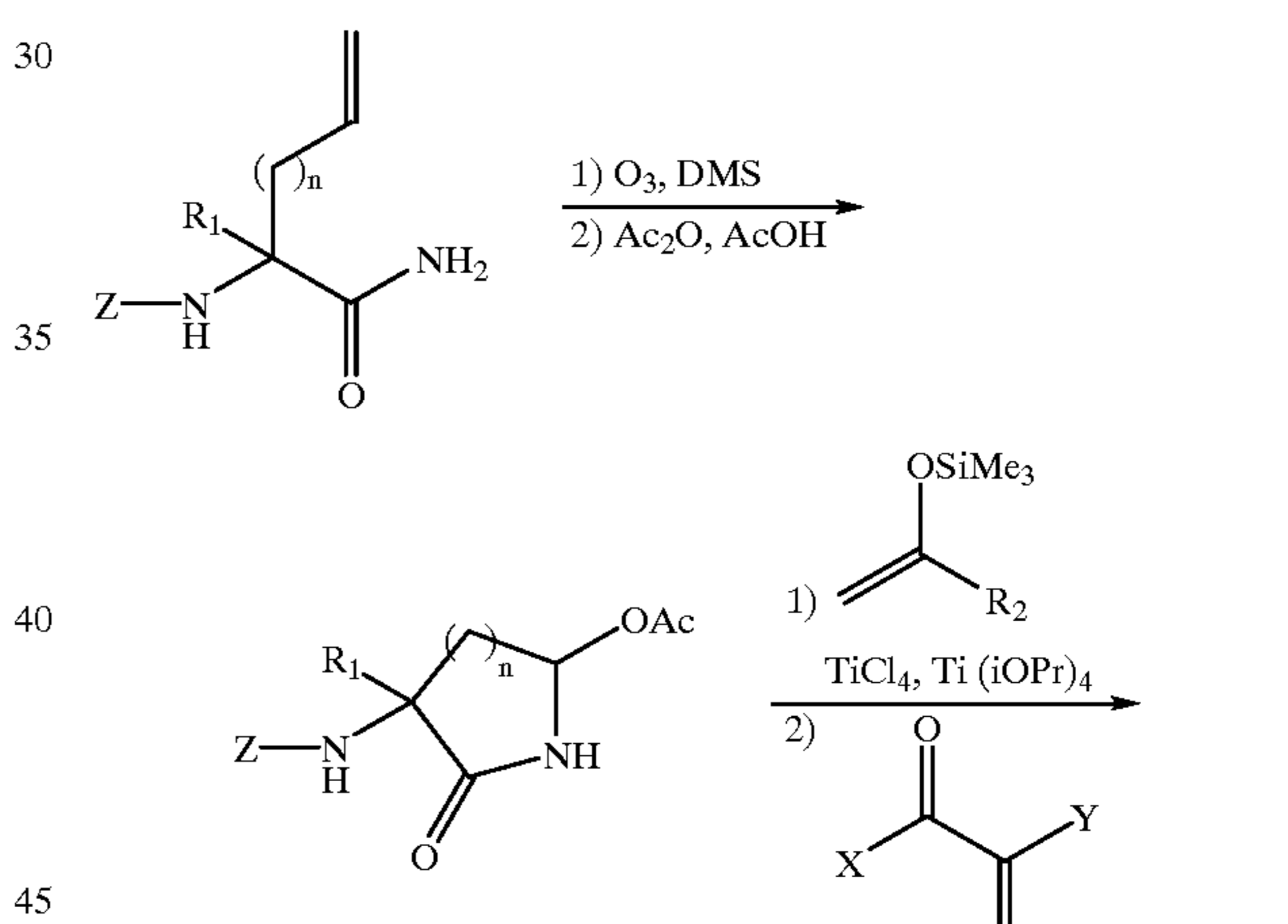
Reaction Scheme (17)
