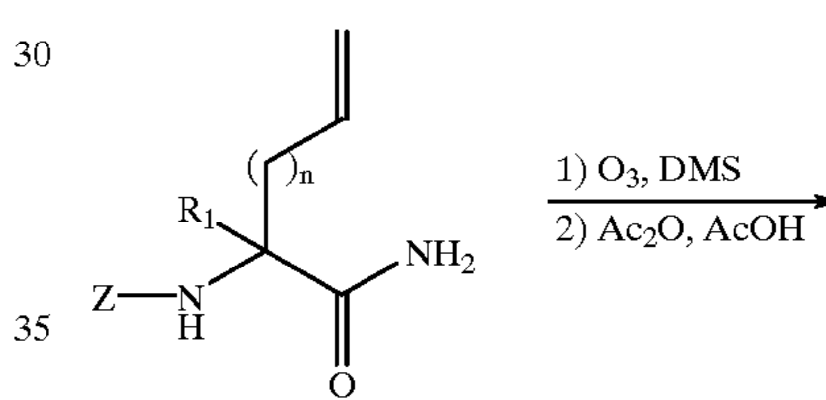
Reaction Scheme (17)
