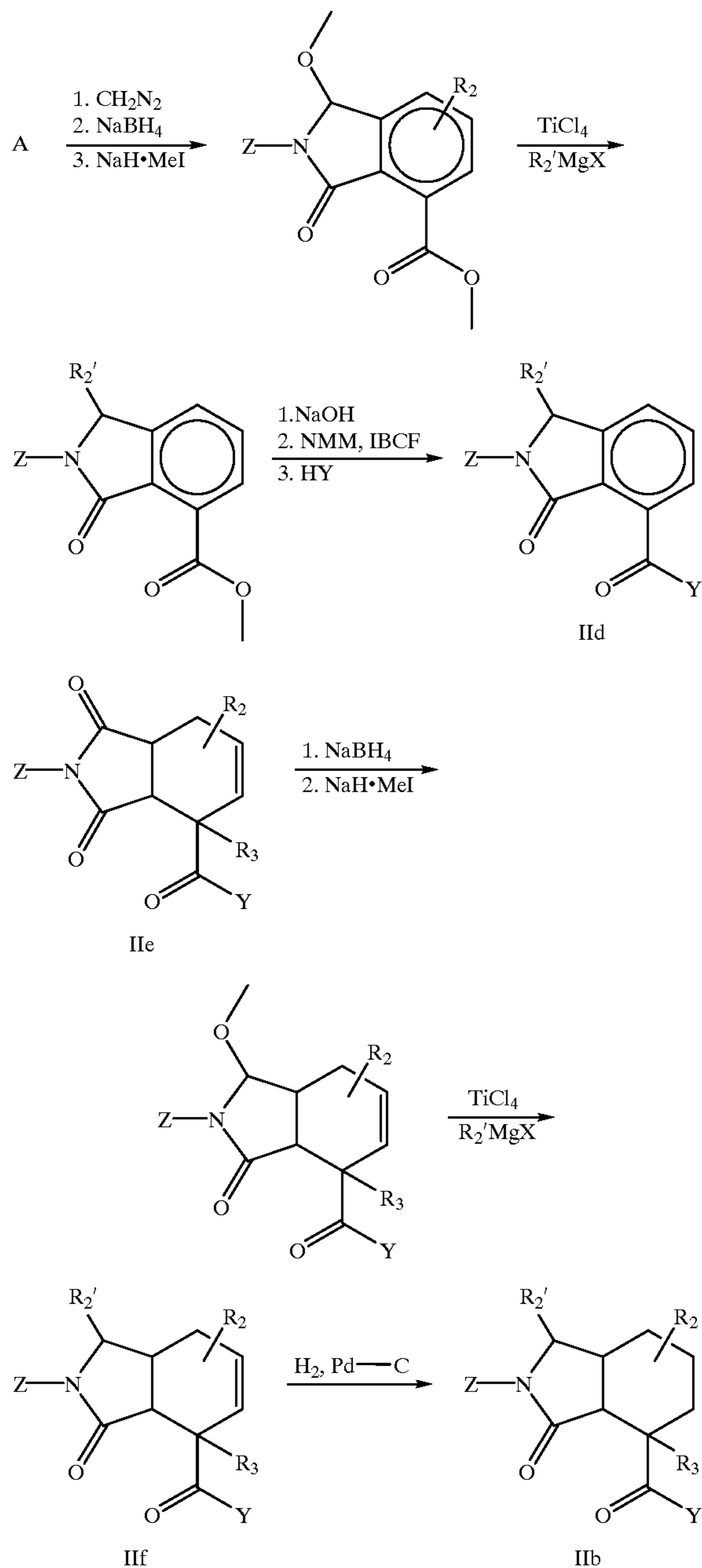
Reaction Scheme (25)
