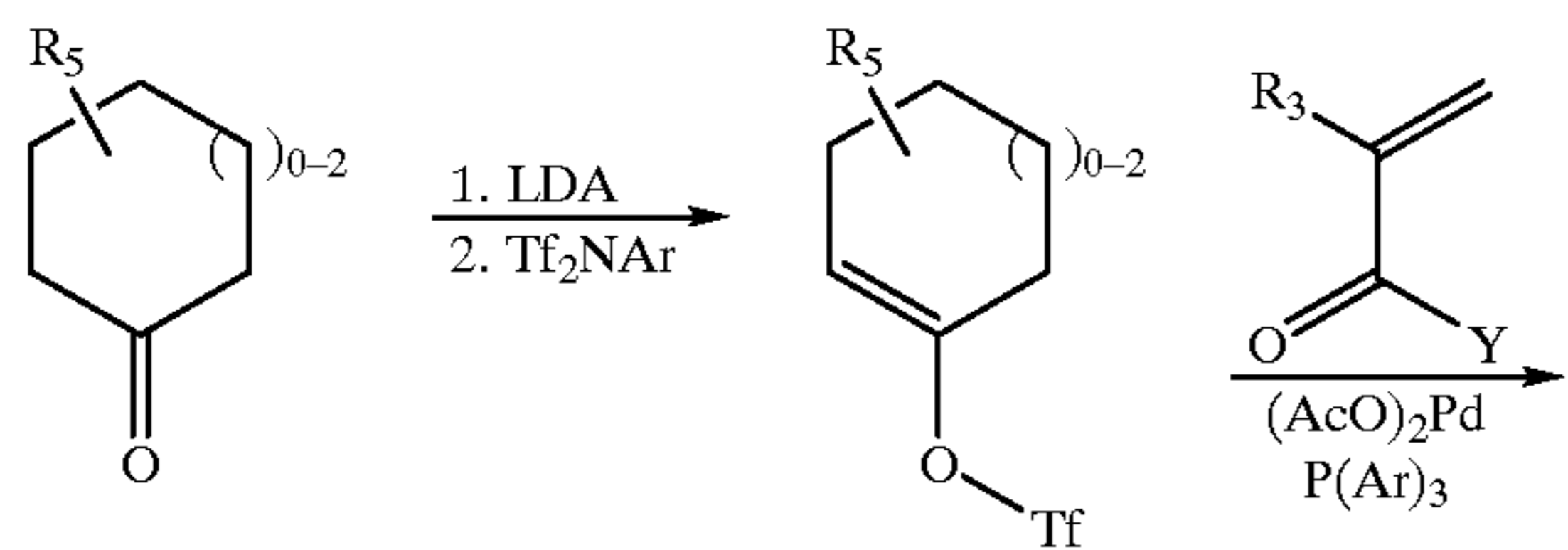
Reaction Scheme (27)
