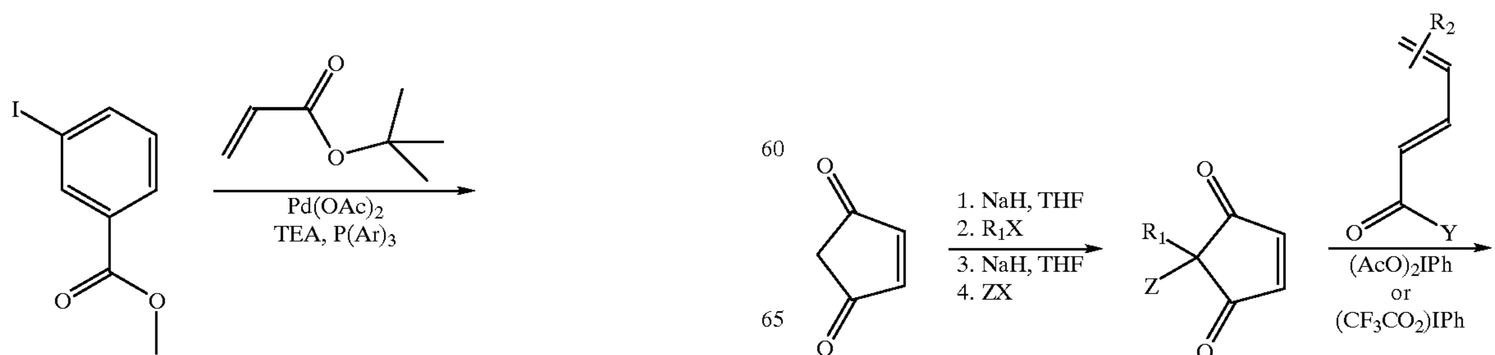
Reaction Scheme (19-1)
