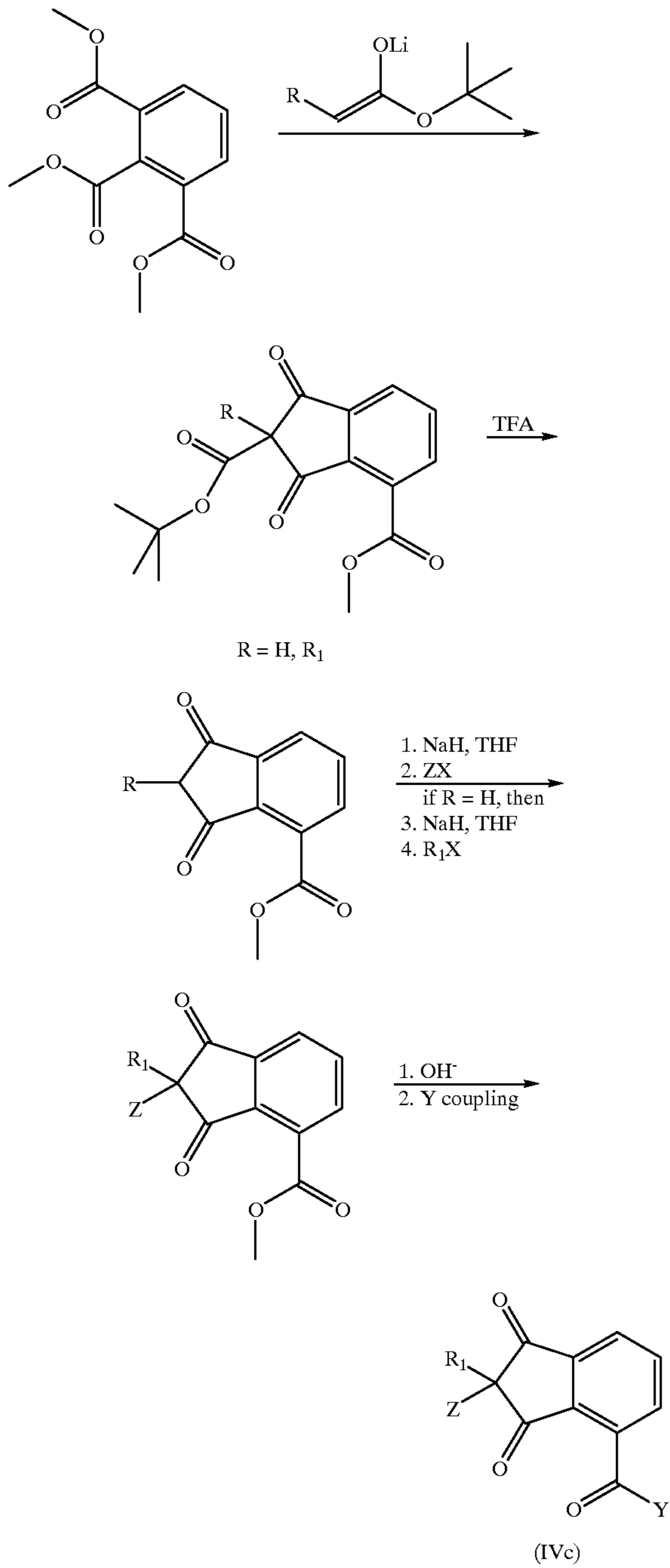
Reaction Scheme (18)
