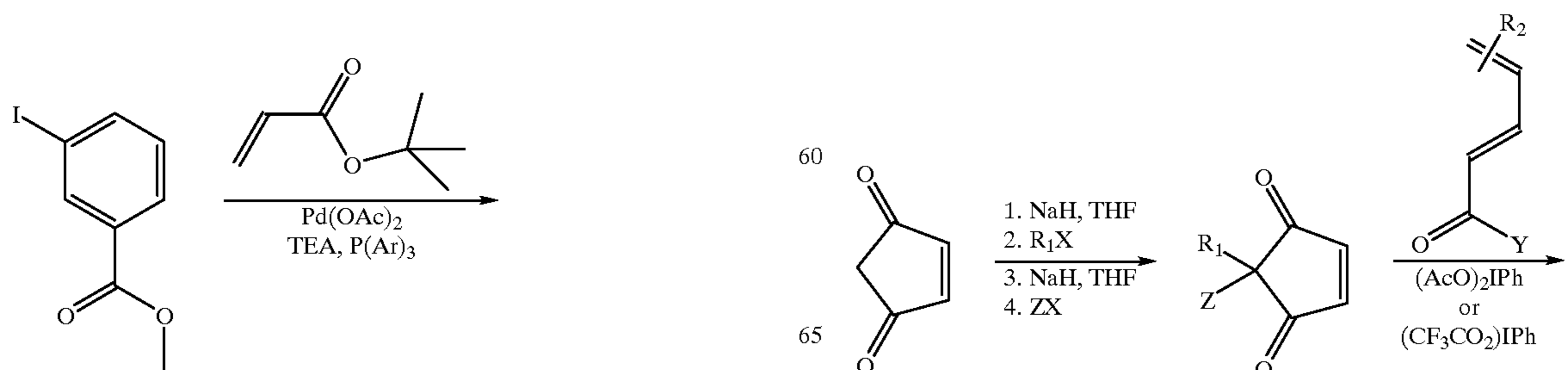
Reaction Scheme (19-1)
