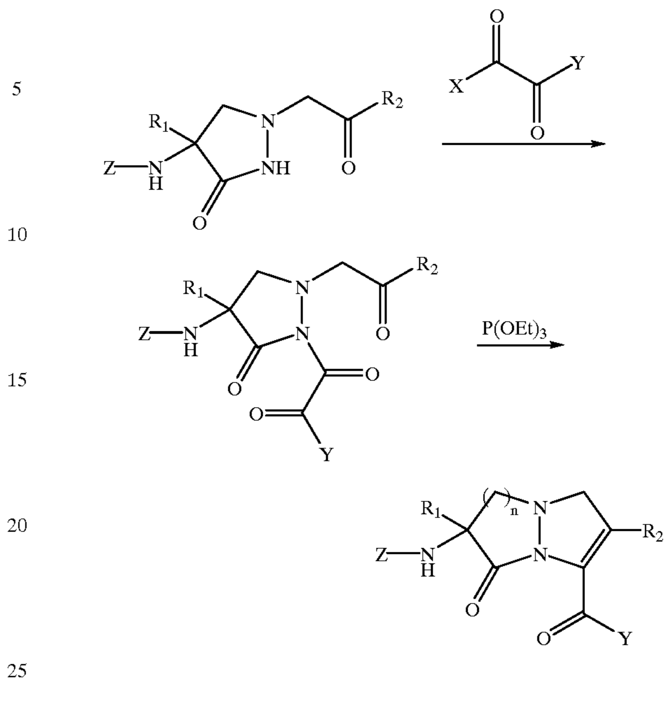
Reaction Scheme (17)
