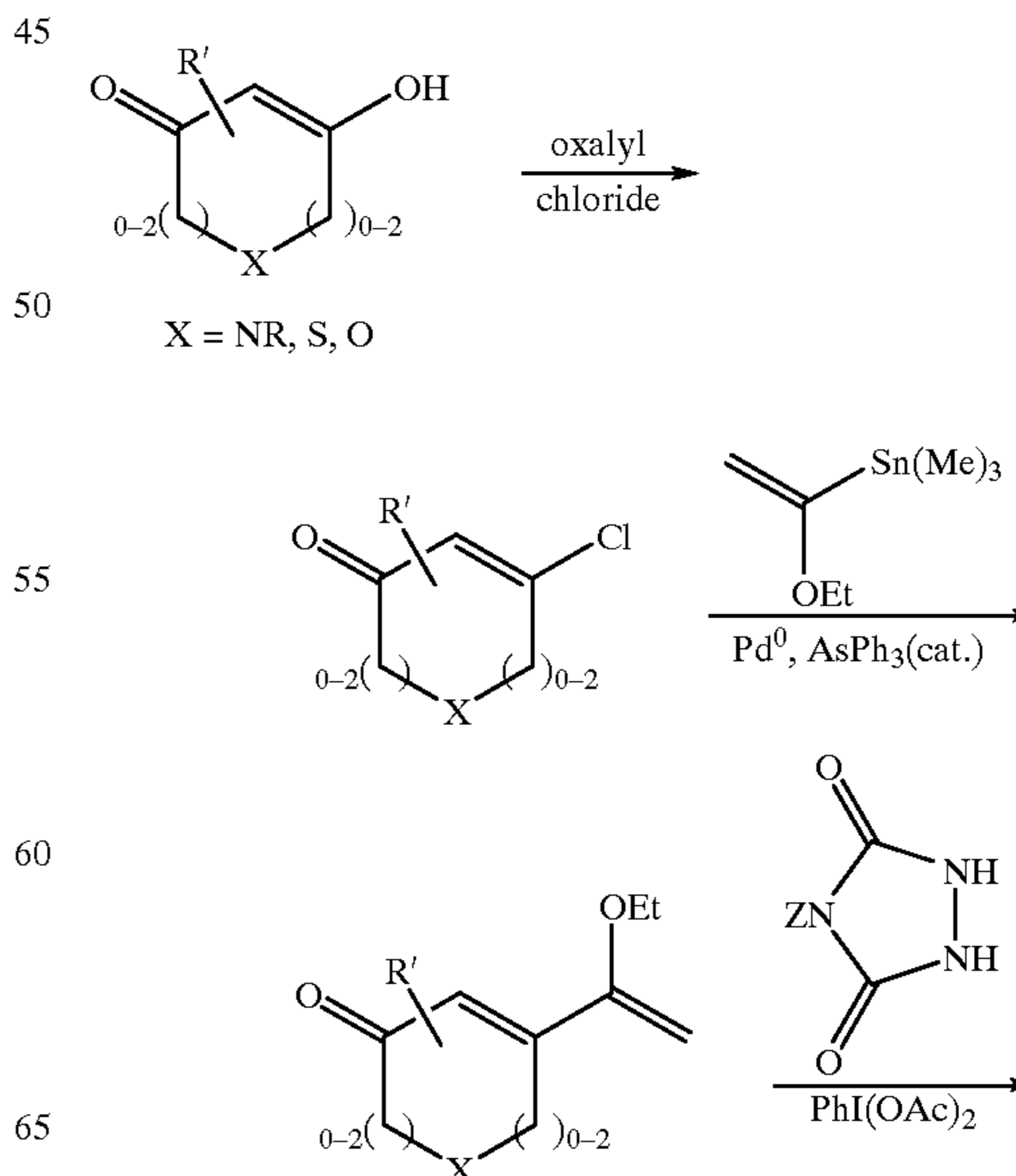
Reaction Scheme (31)
