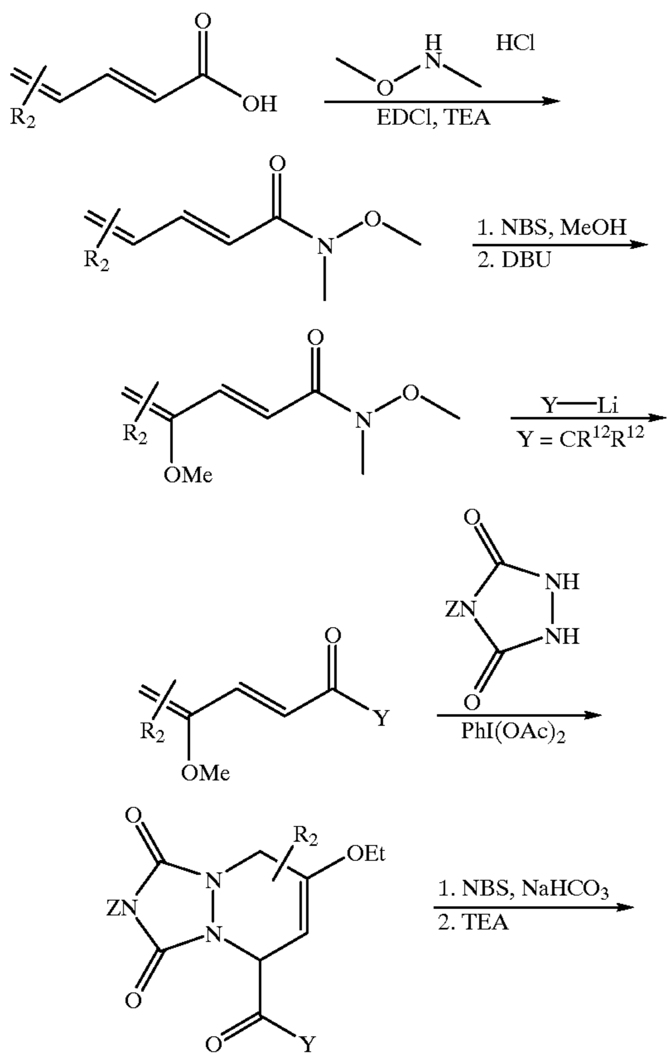
Reaction Scheme (32)
