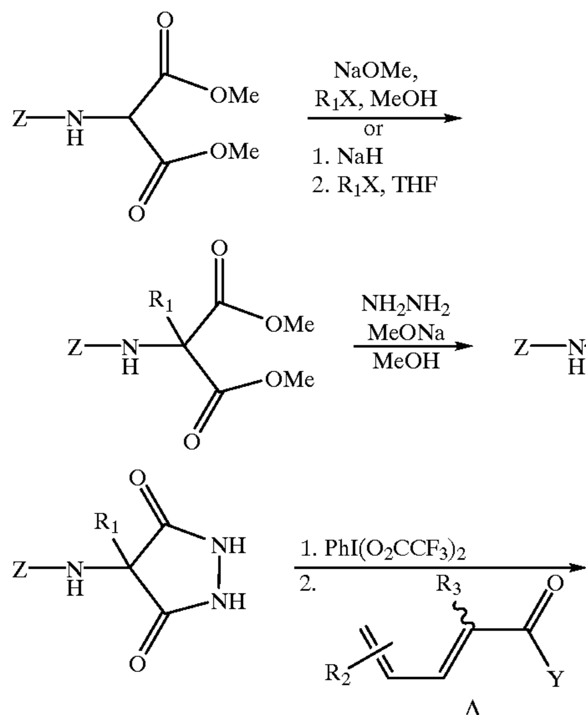
Reaction Scheme (15)
