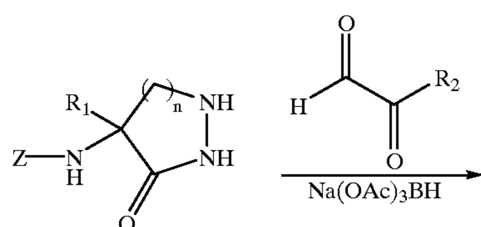
Reaction Scheme (16)
