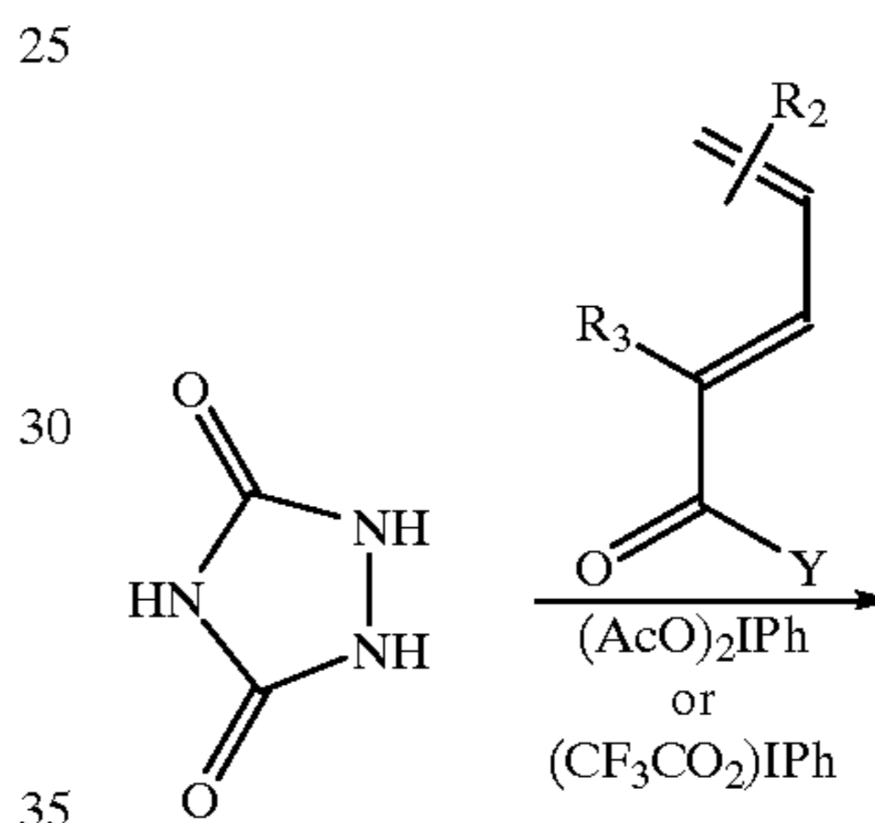
Reaction Scheme (28)
