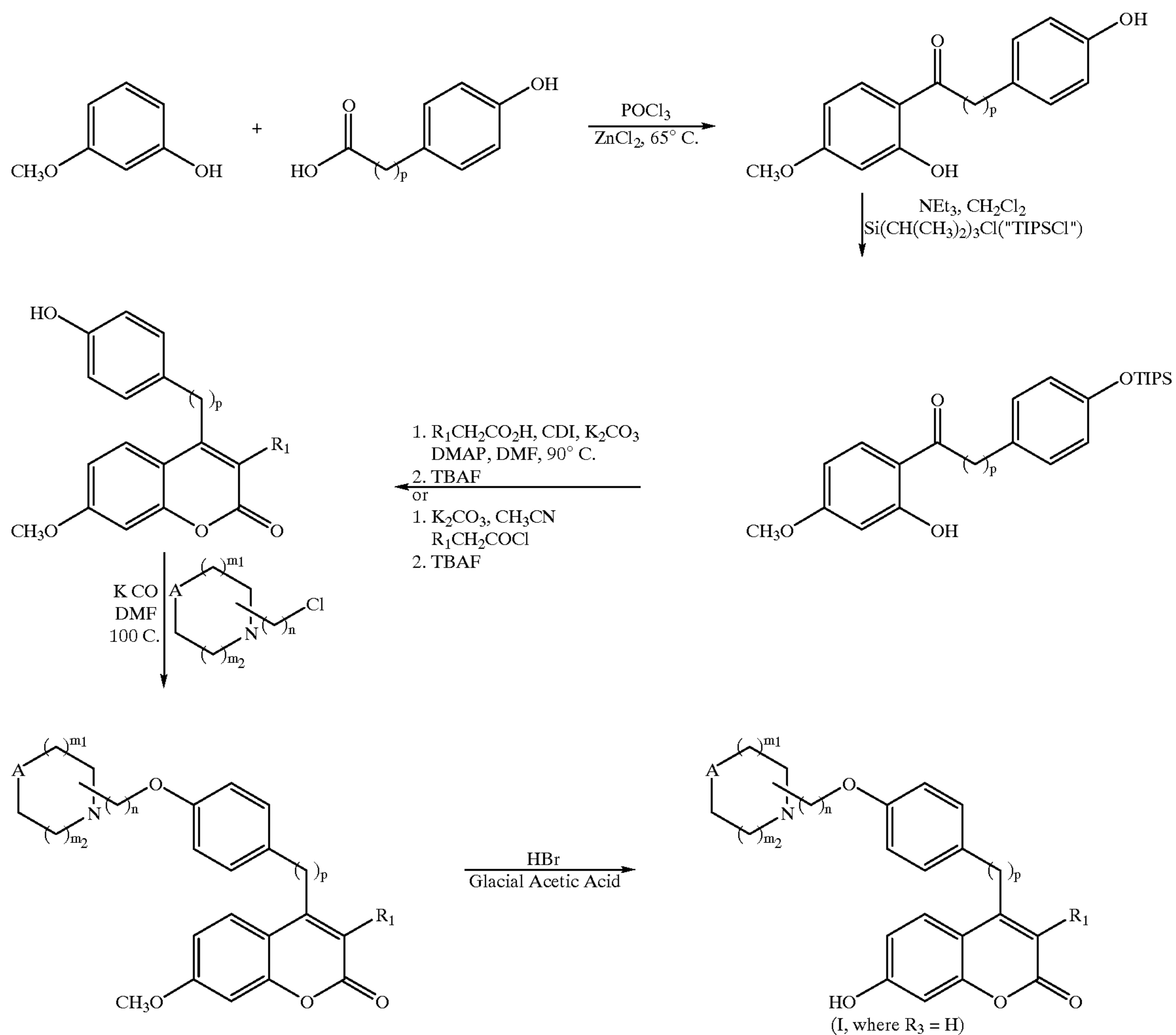
Reaction Scheme 1
