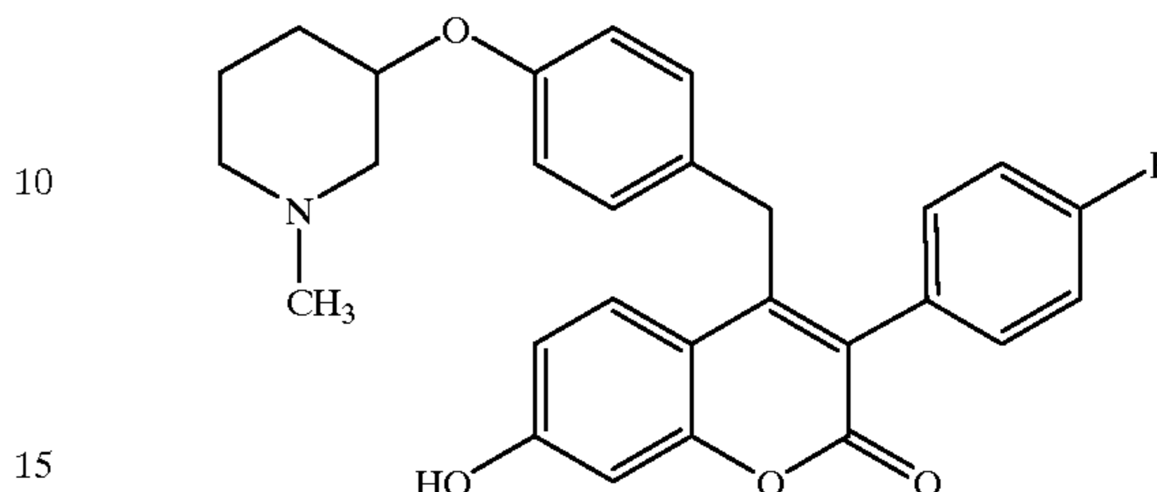
3-(4-Fluorophenyl)-4-[4-(1-methylpiperidyl-3-oxy)]-benzyl-7-hydroxycoumarin
