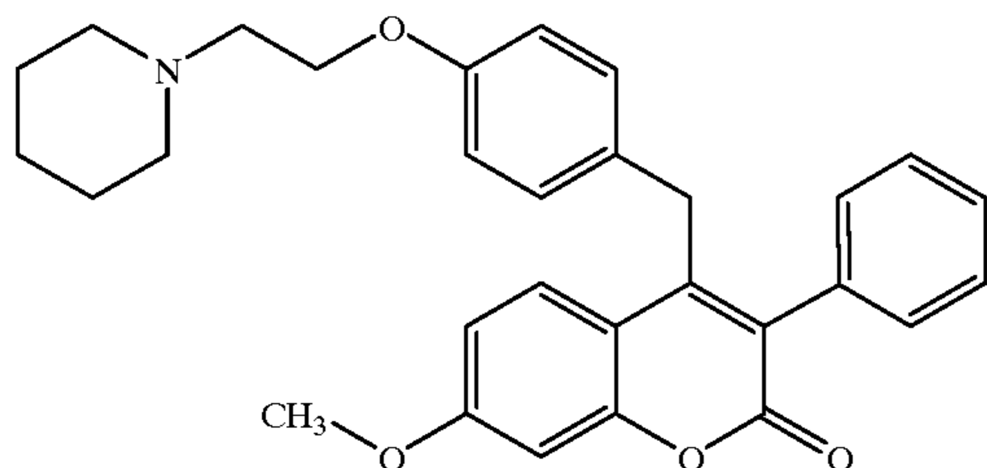
3-Phenyl-4-[4-(2-{piperin-1-yl})ethoxy]-benzyl-7-methoxycoumarin
