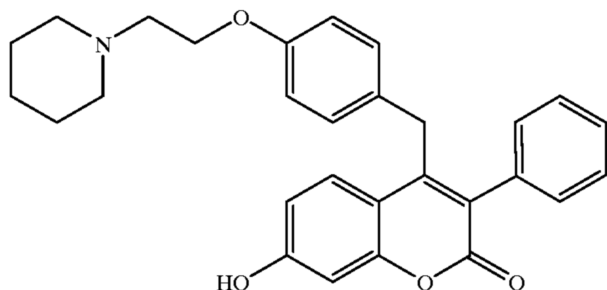
3-Phenyl-4-[4-(2-{piperidin-1-yl})ethoxy]-benzyl-7-hydroxycoumarin
