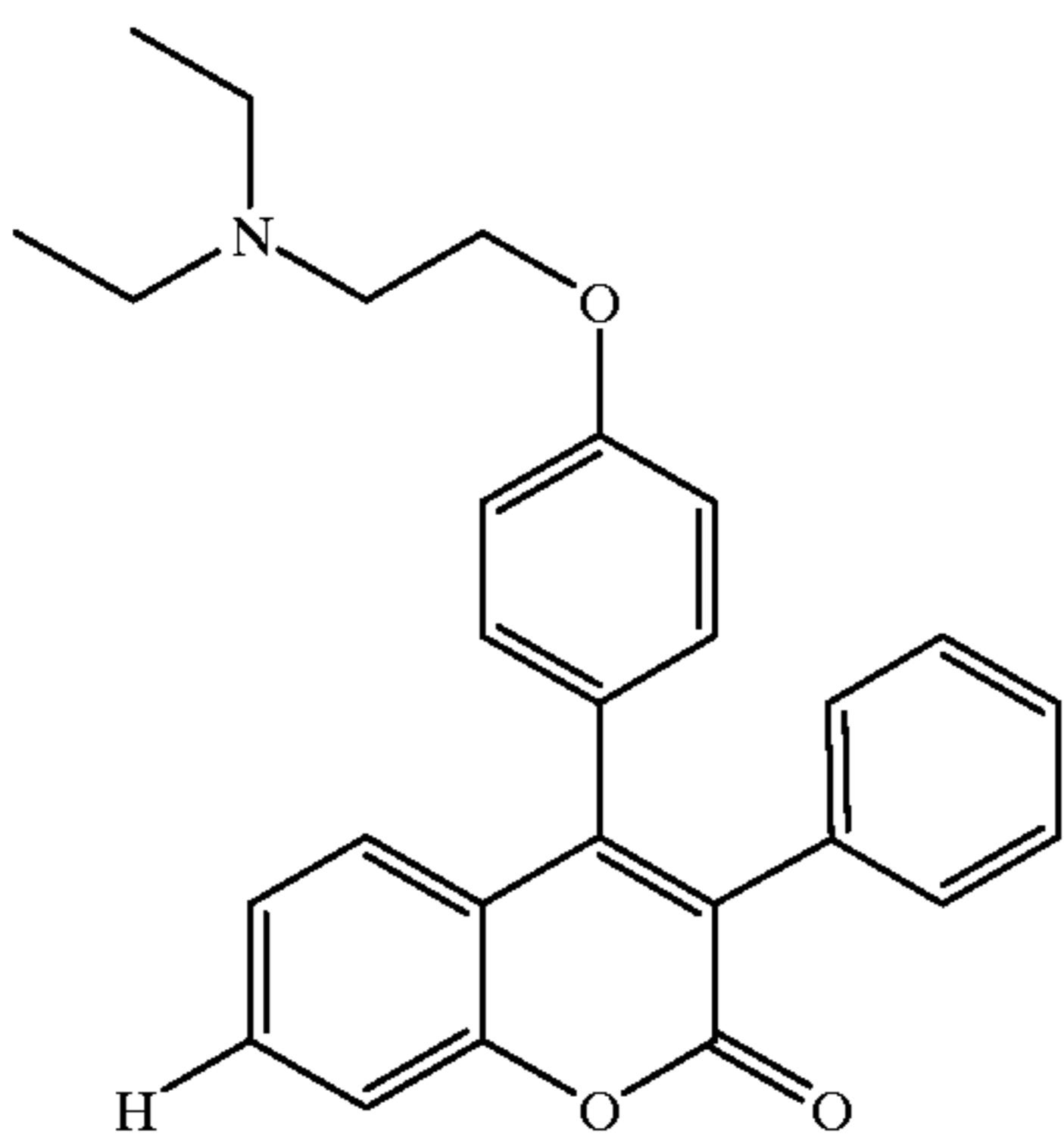
Compound "L-20"
