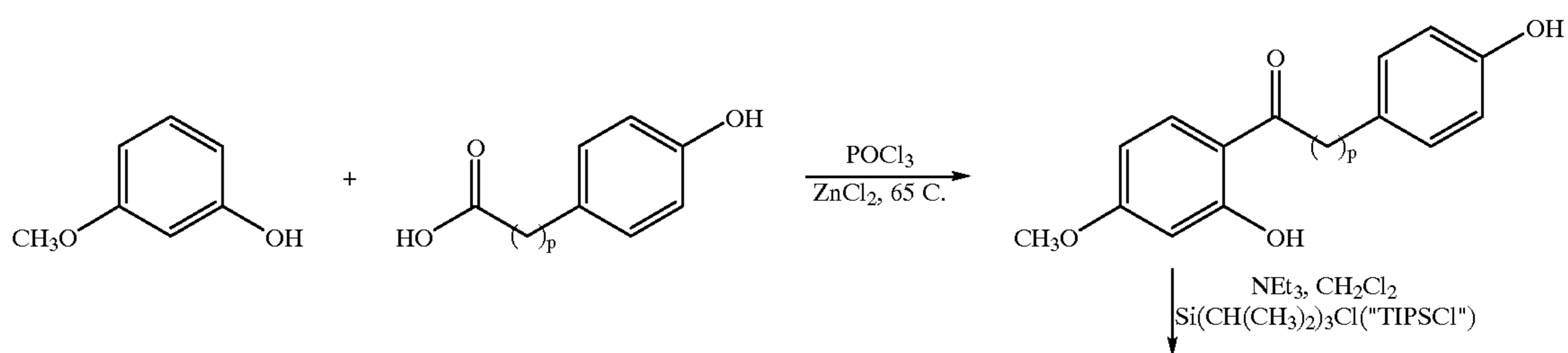
Reaction Scheme 2
