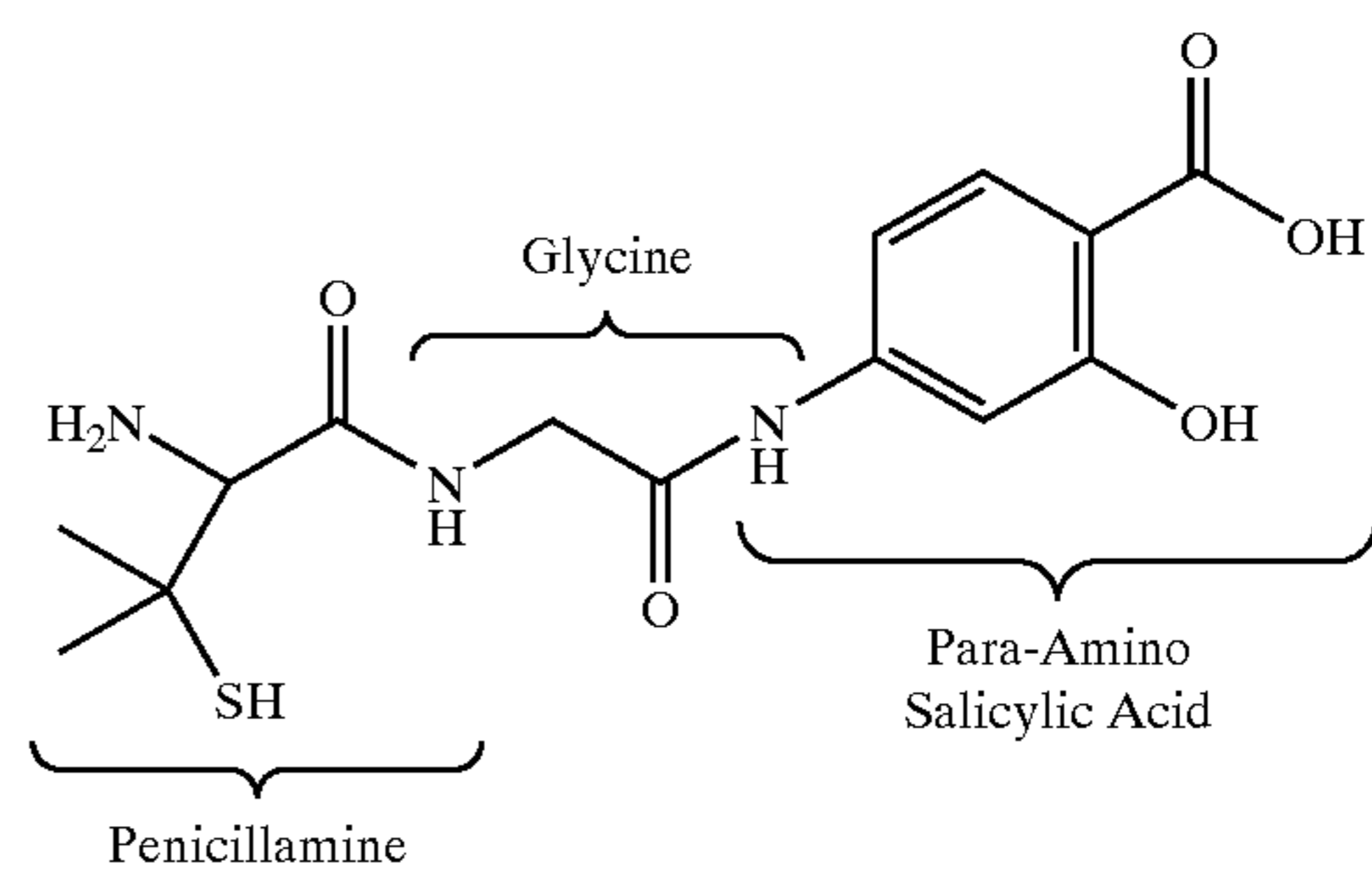
Structure of Heterodimeric Compound 1
