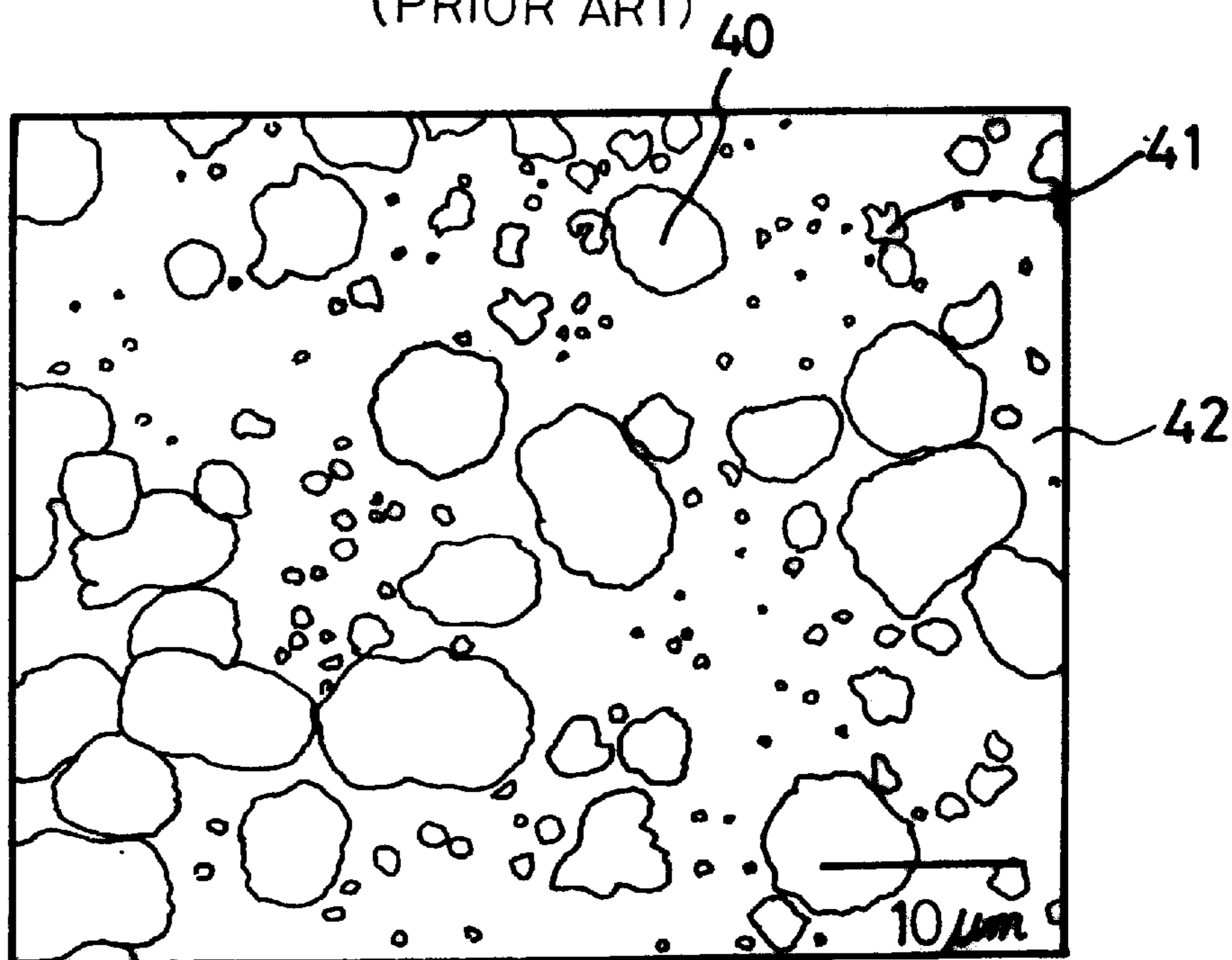
FIG. 4 (PRIOR ART)
