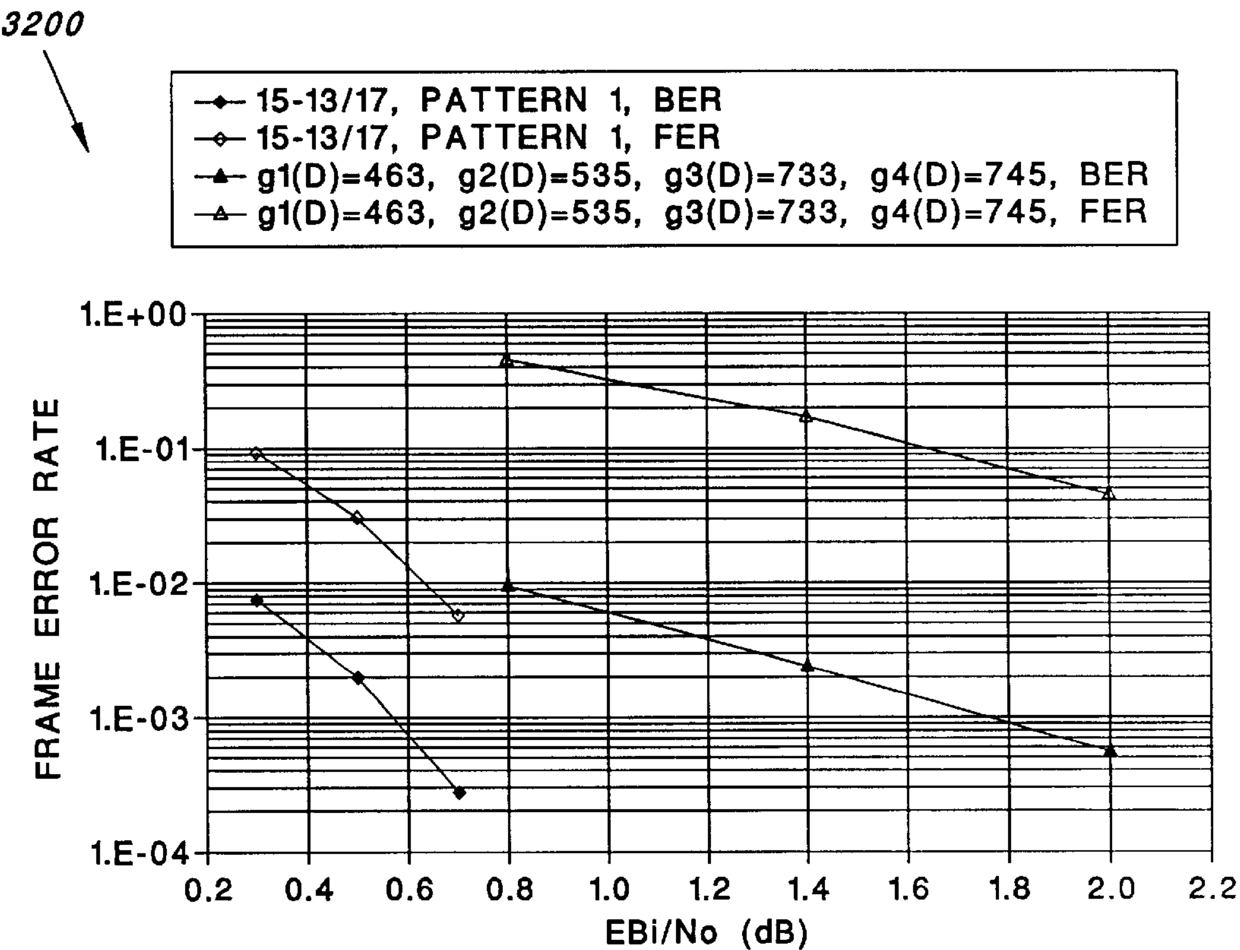
FIG. 32 COMPARISON OF RATE 1/4 FER-OPTIMIZED TURBO CODE VS CONVOLUTIONAL CODE, FRAME SIZE=512
