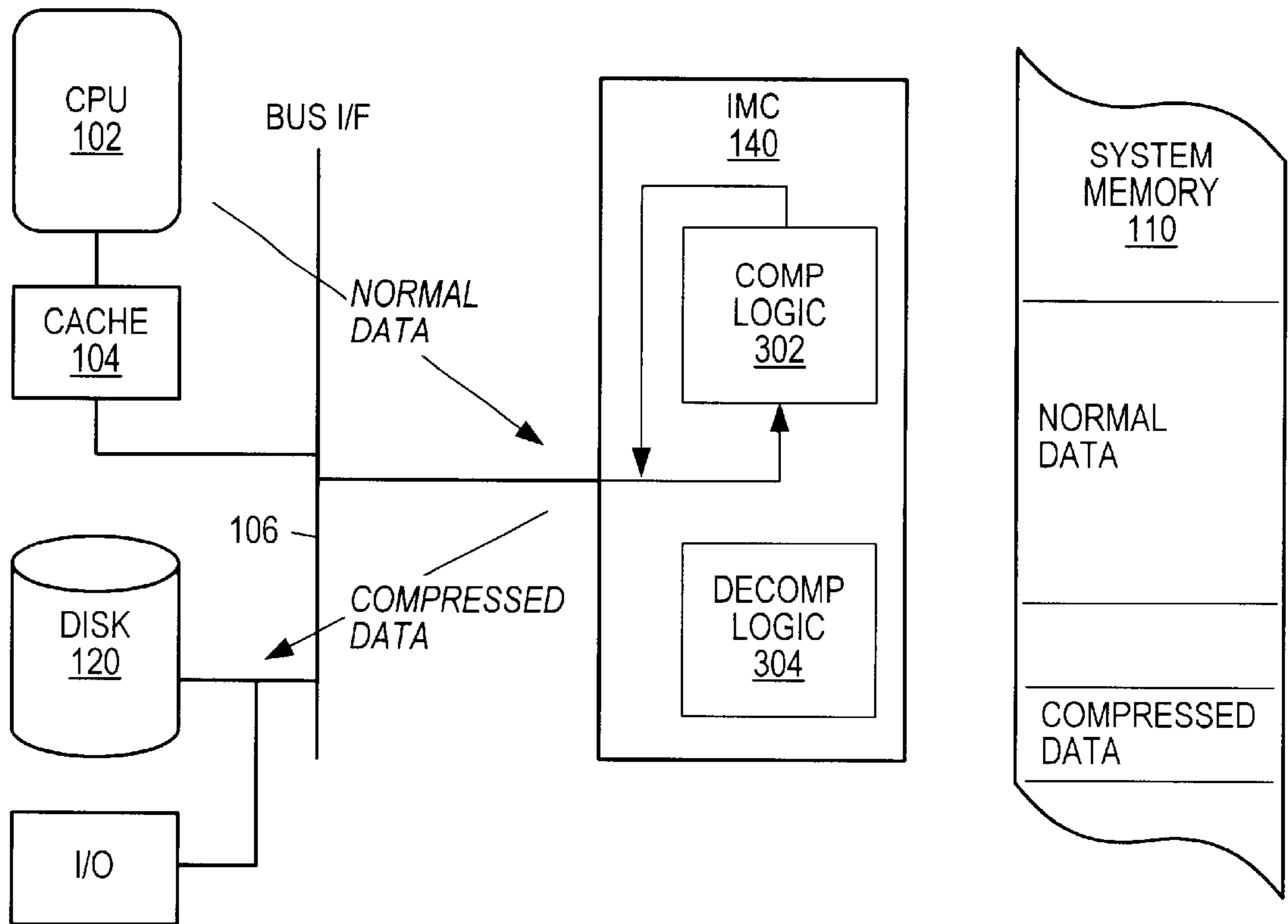
Compression of CPU data to Disk or I/O subsystem
