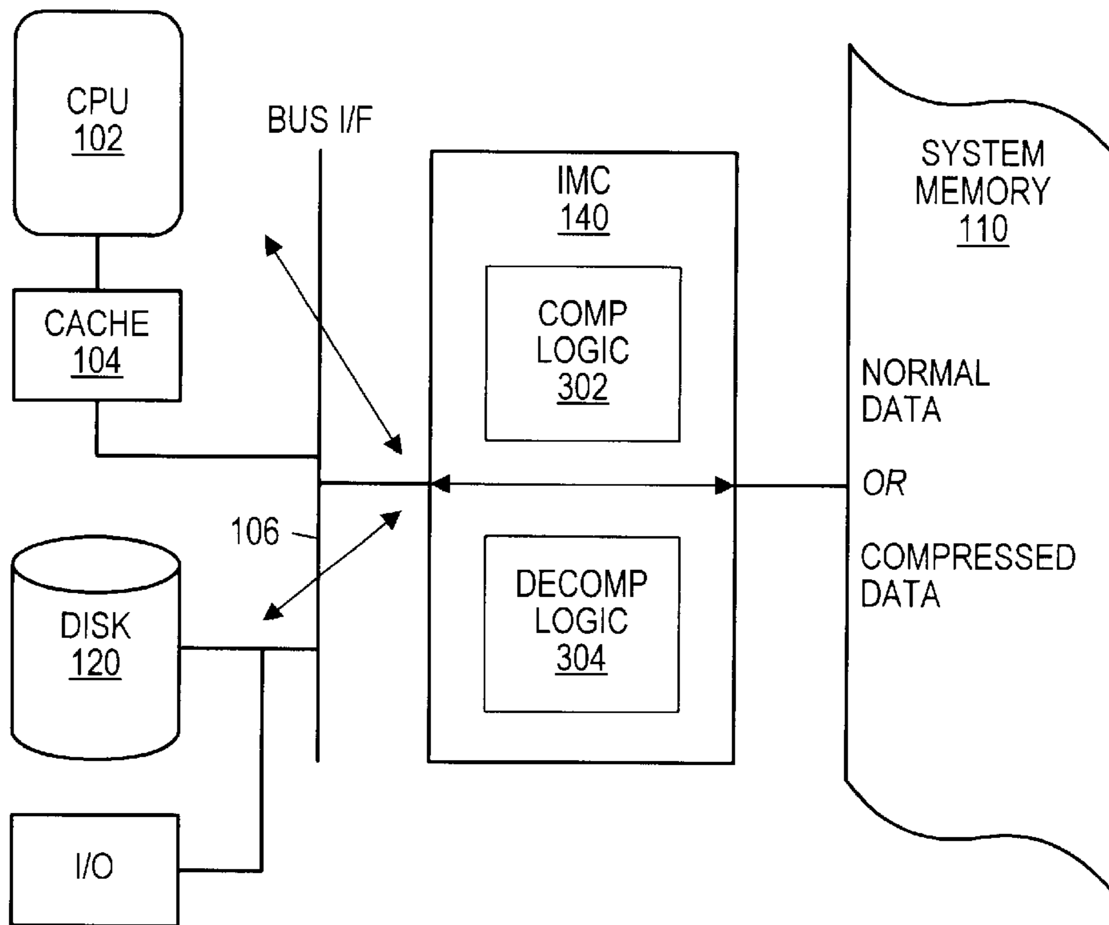
Normal or compressed data transfer, No modification by IMC
