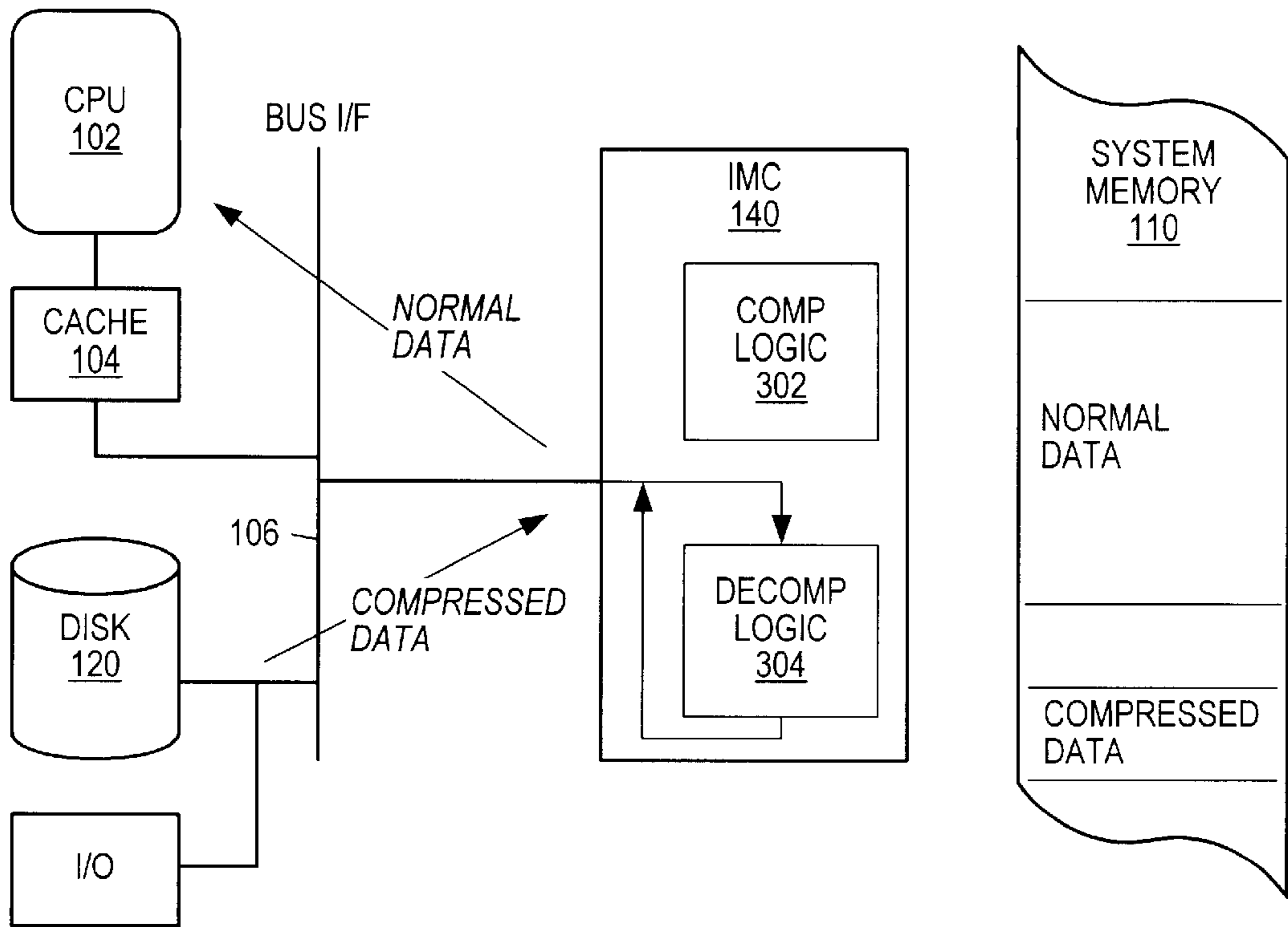
Decompression of disk to CPU
