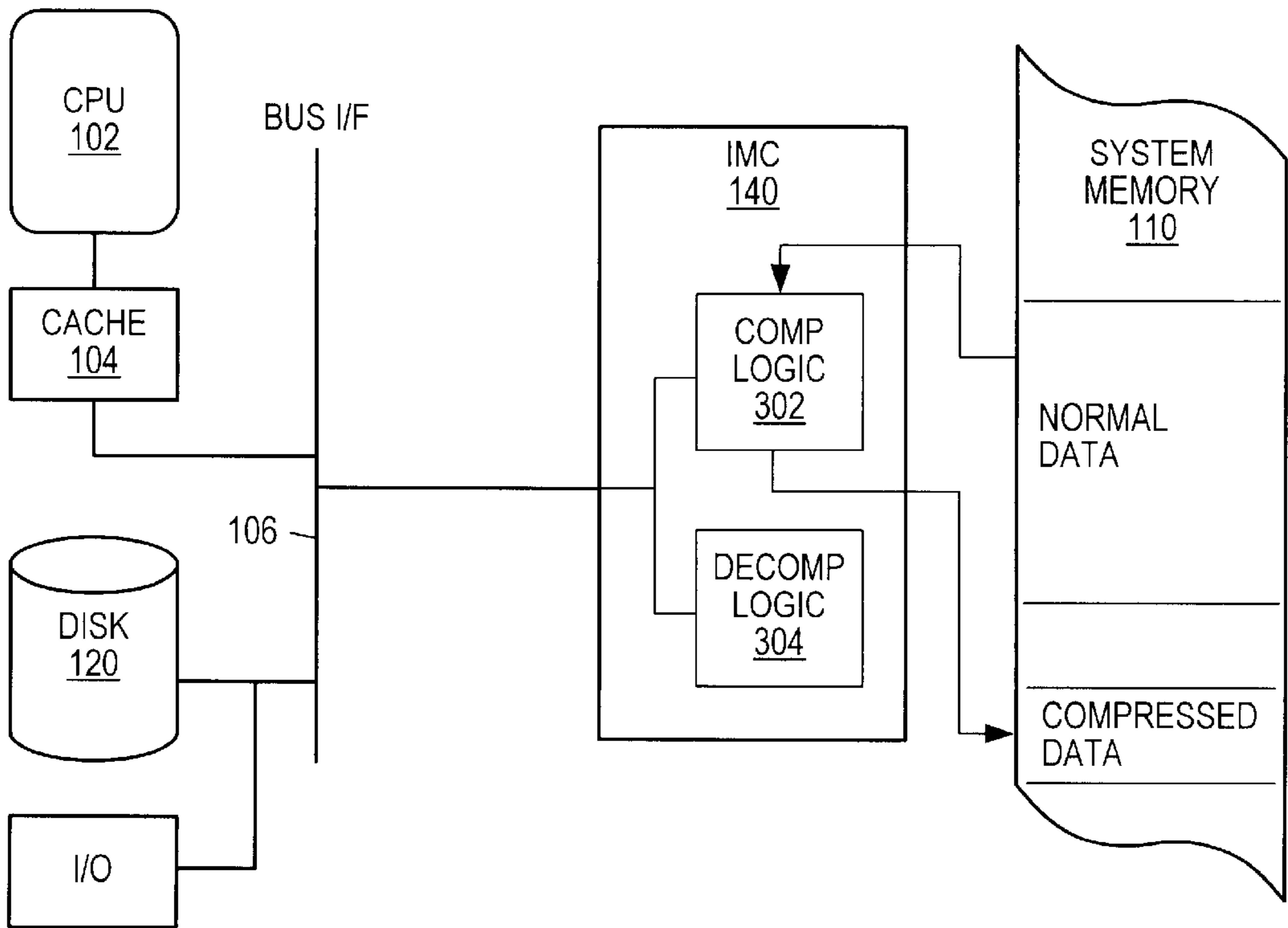
Memory to memory Compression
