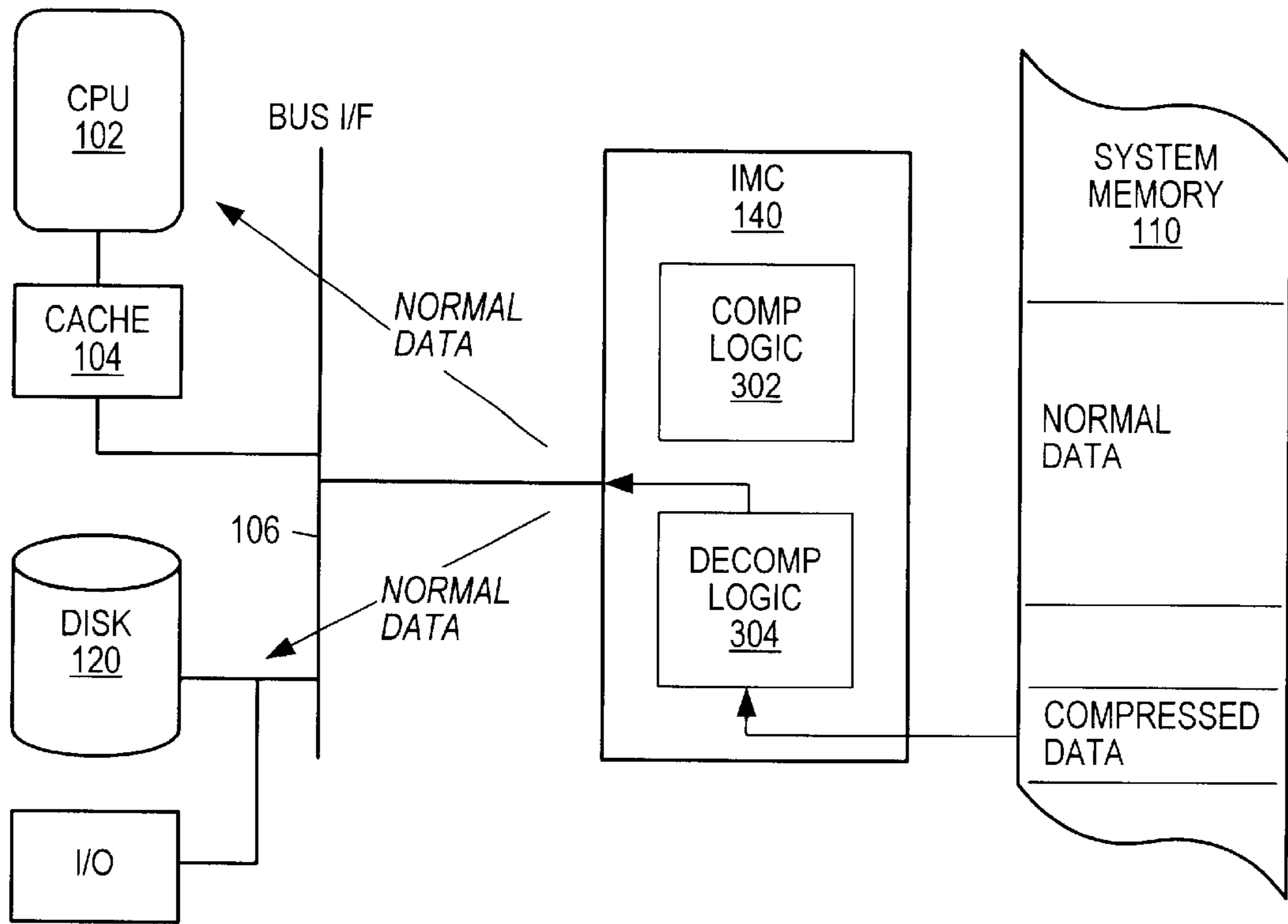
Memory decompression to CPU or DISK
