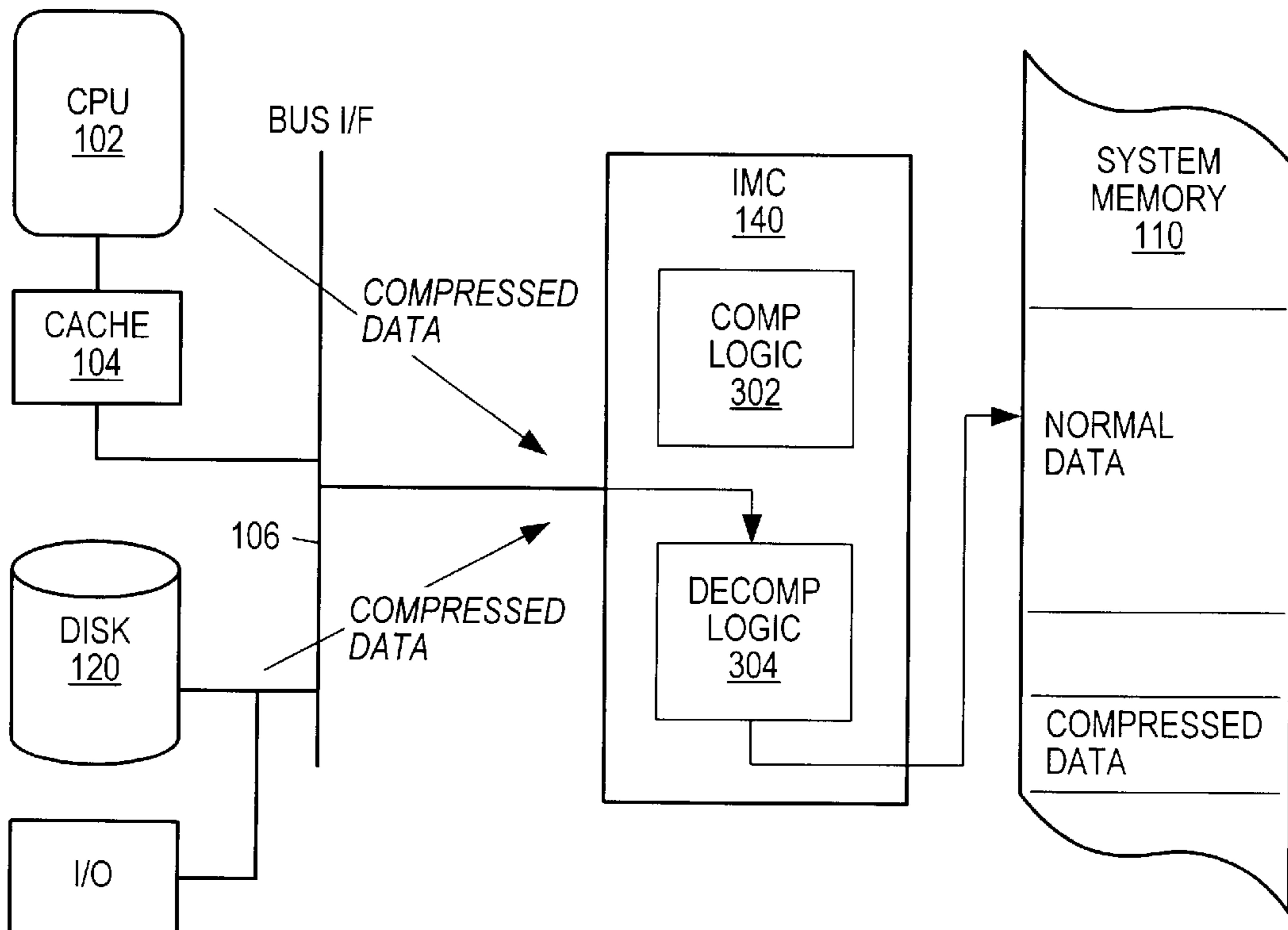
Decompression from Disk or CPU to memory
