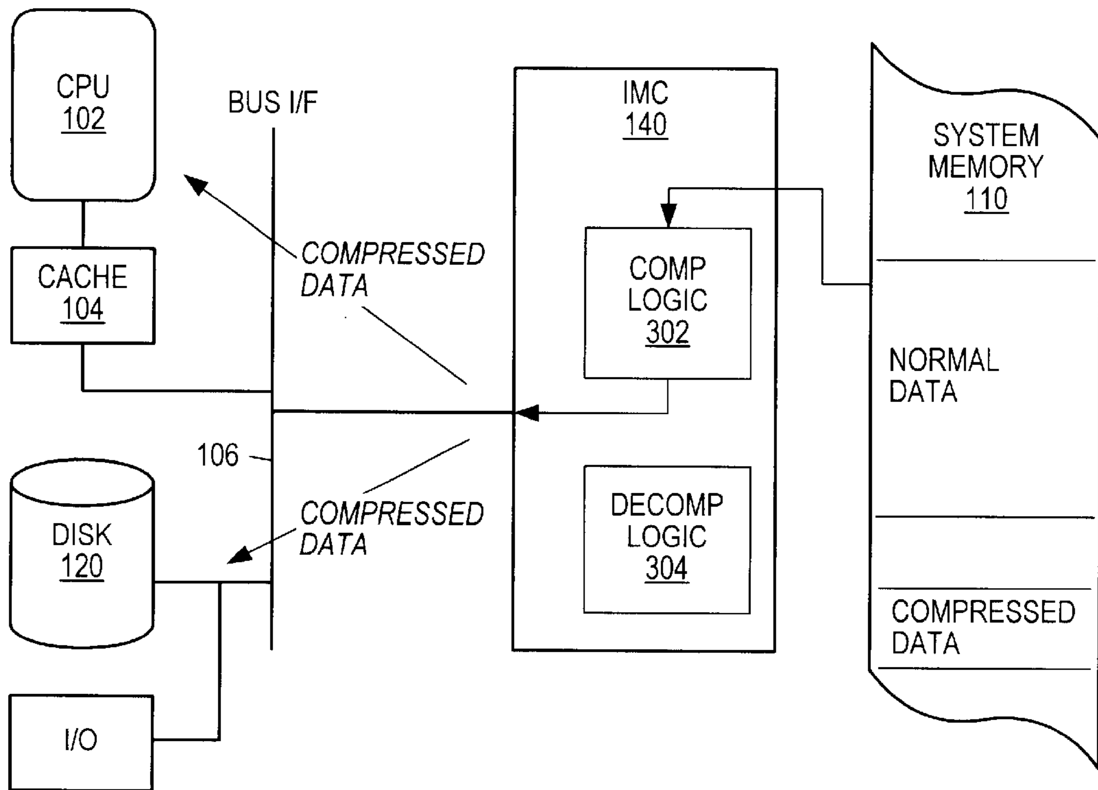
Compression from memory to CPU or Disk
