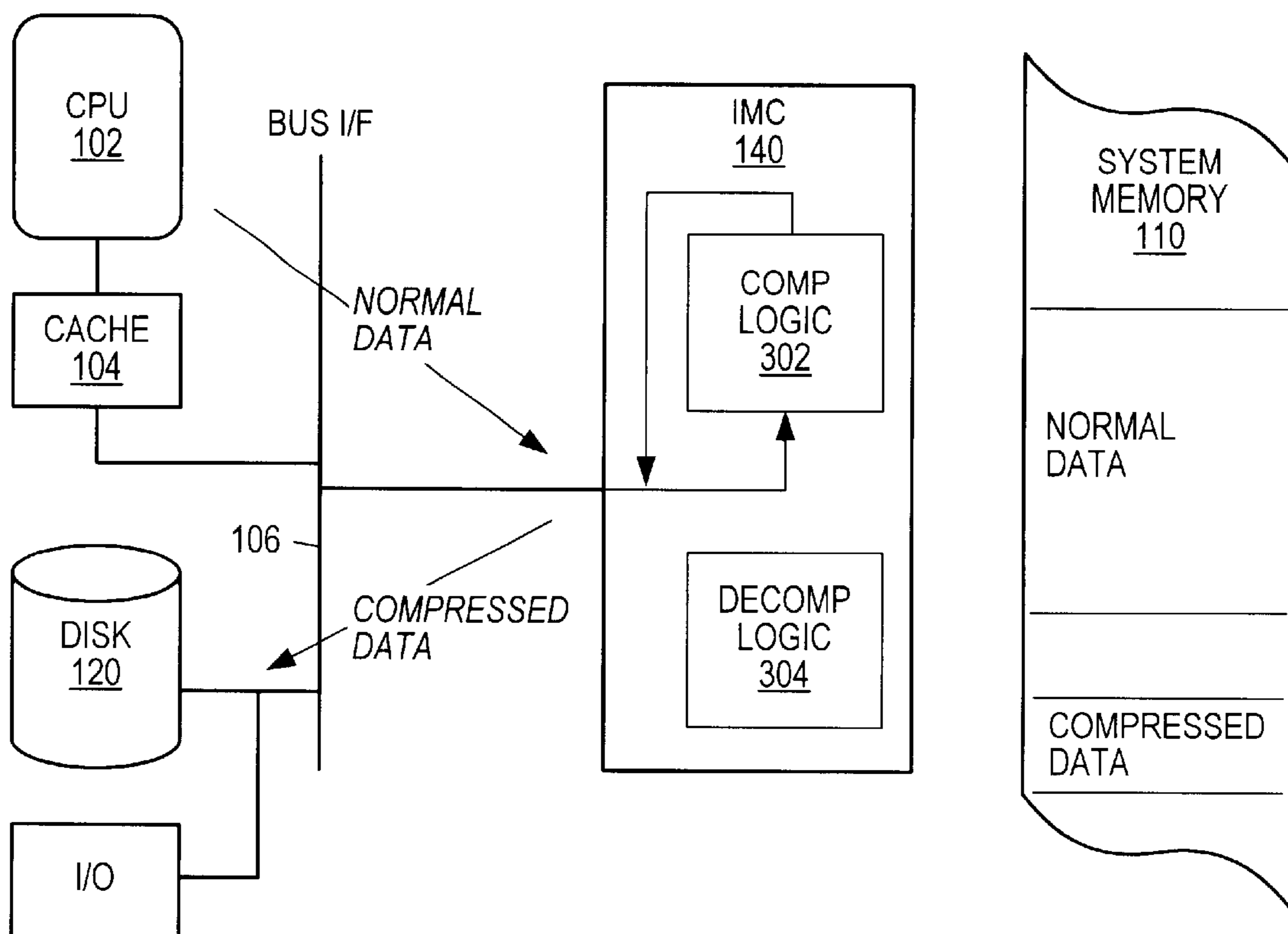
Compression of CPU data to Disk or I/O subsystem
