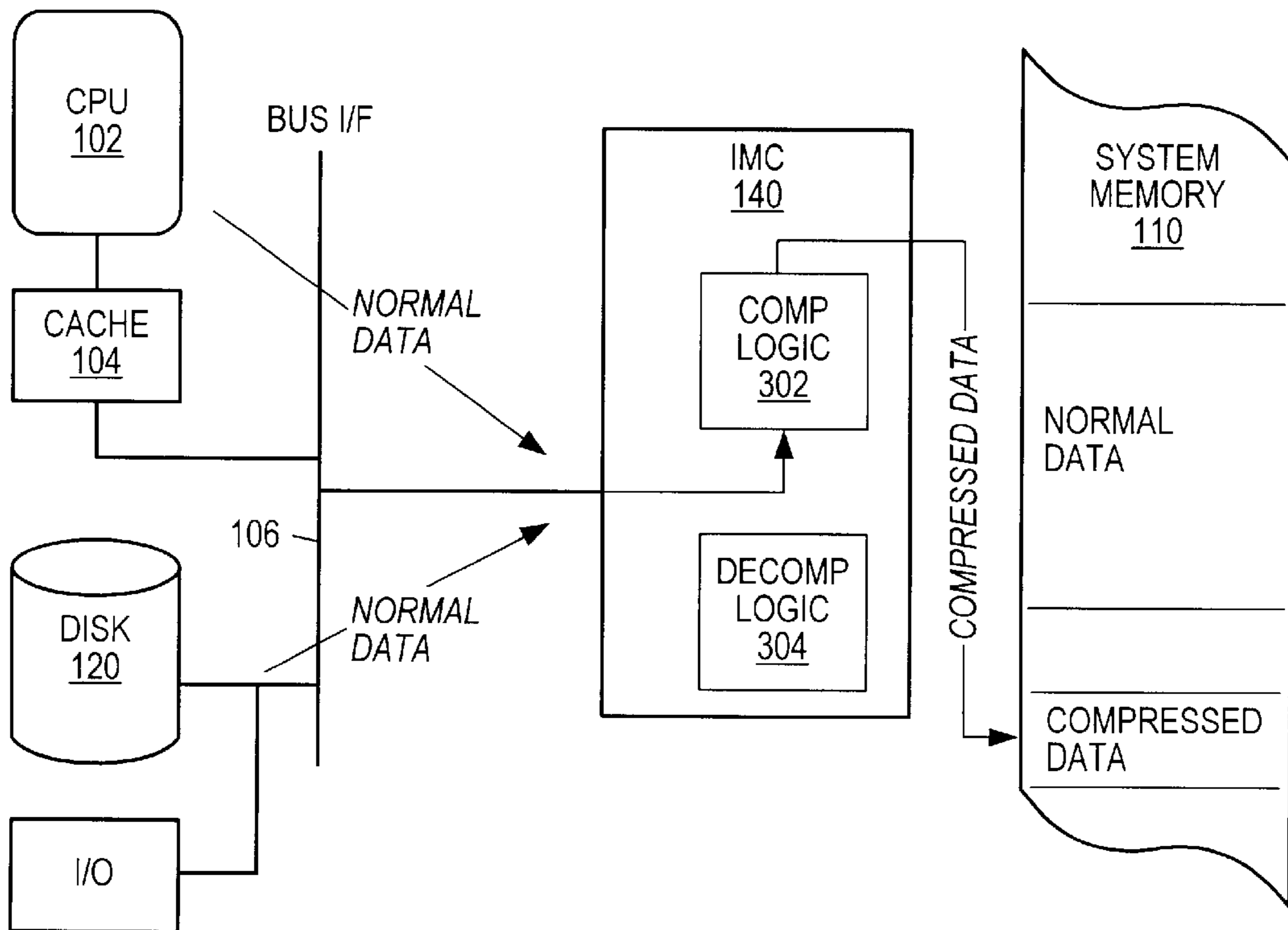
Compression from CPU or disk to memory
