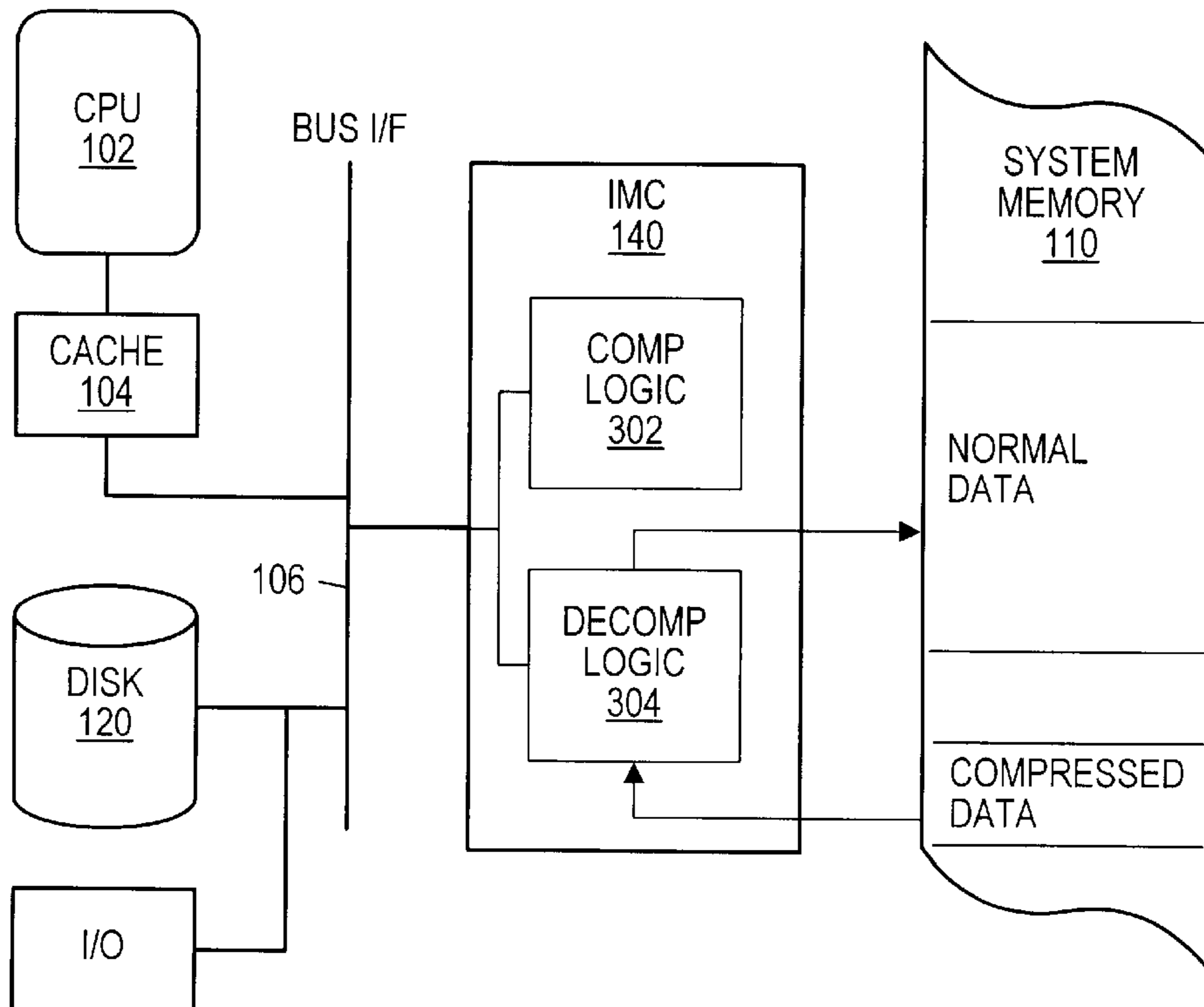
Memory to memory decompression
