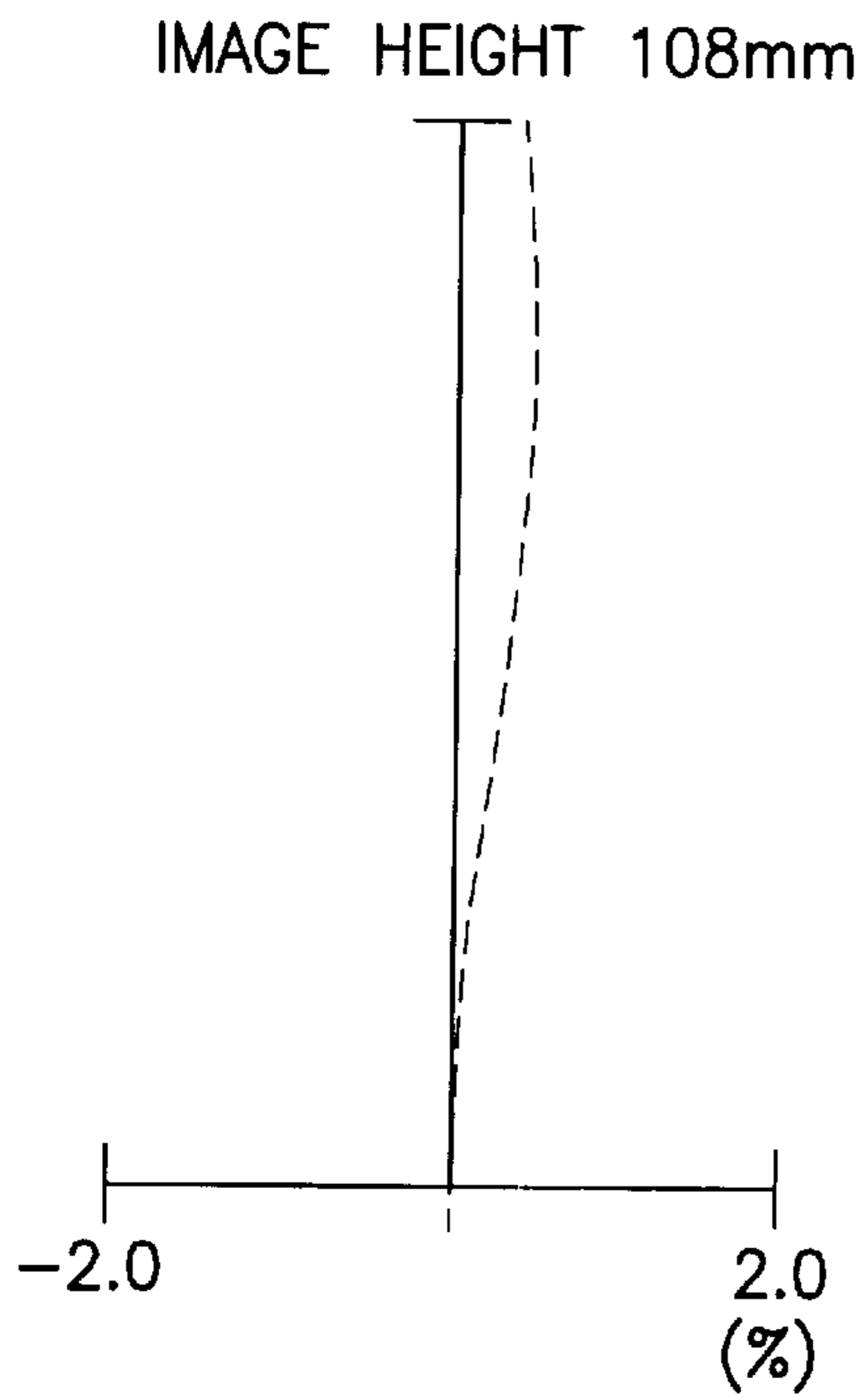
CONSTANT VELOCITY CHARACTERISTICS
