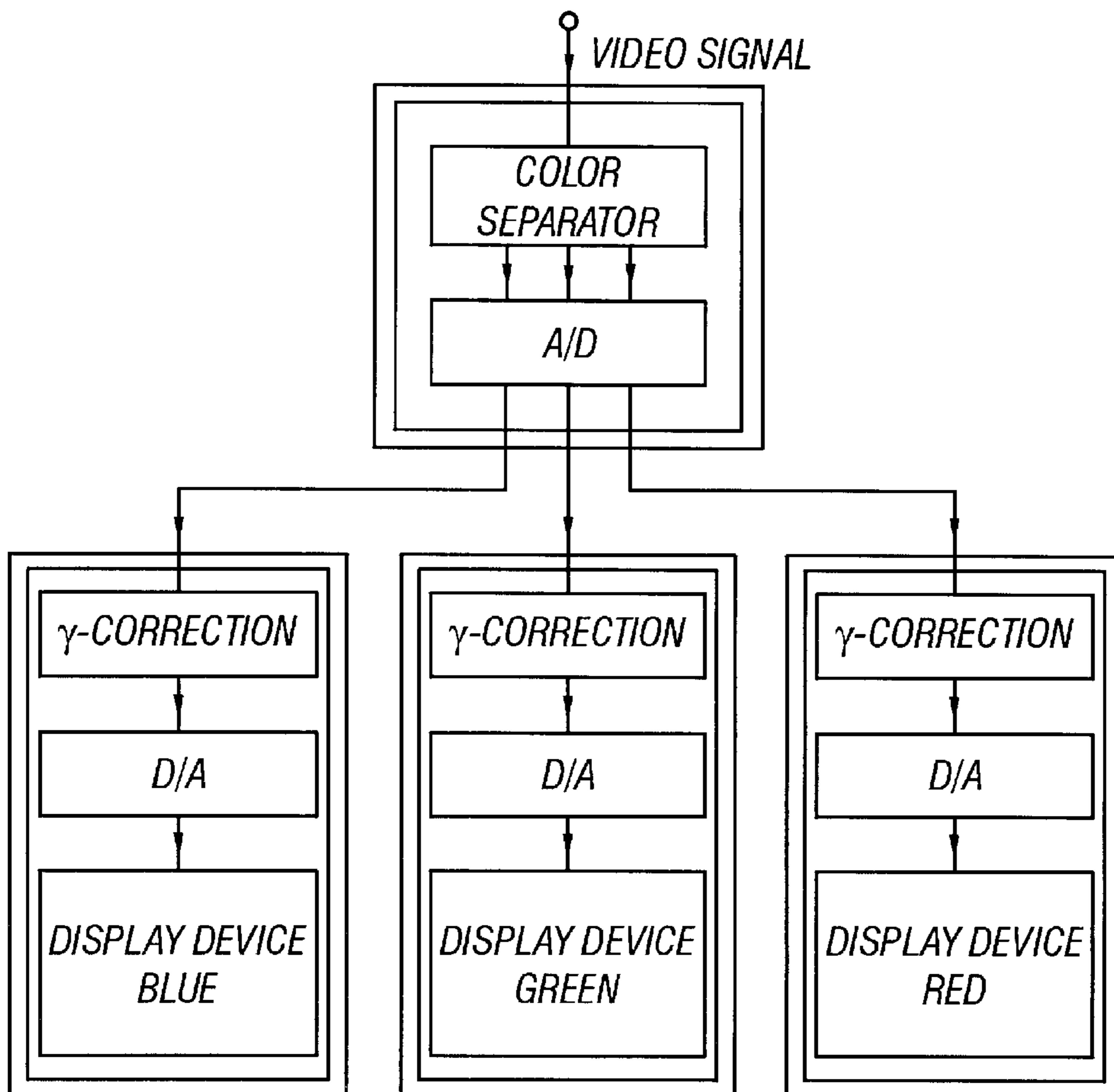
FIG. 4 (Prior Art)
