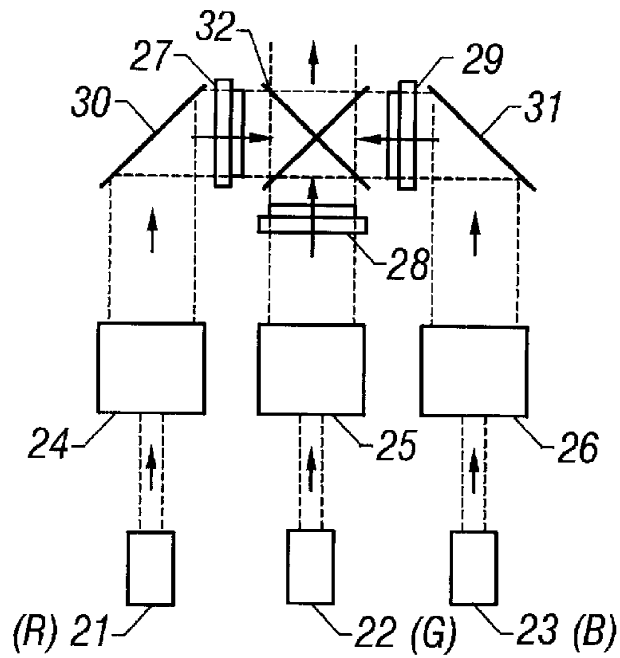
FIG. 3 (Prior Art)
