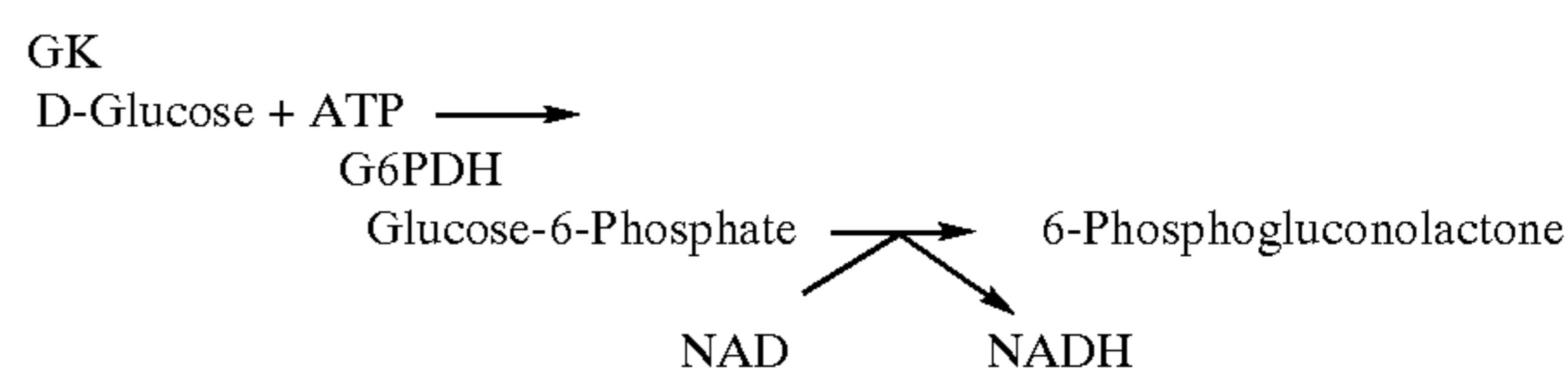
Scheme 2
