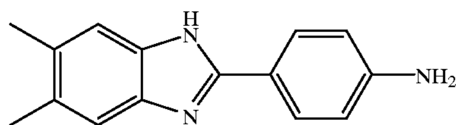
2-(4-aminophenyl)-5,6-dimethylbenzimidazole
