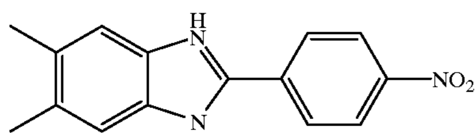
2-(4-nitrophenyl)-5,6-dimethylbenzimidazole
