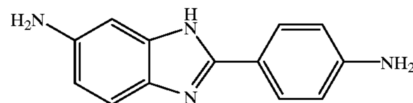
2-(4-aminophenyl)-5-aminobenzimidazole
