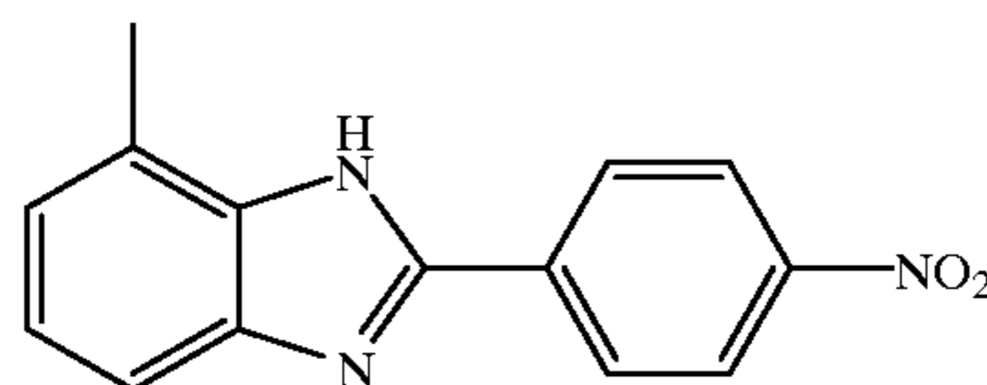
2-(4-nitrophenyl)-7-methyl benzimidazole
