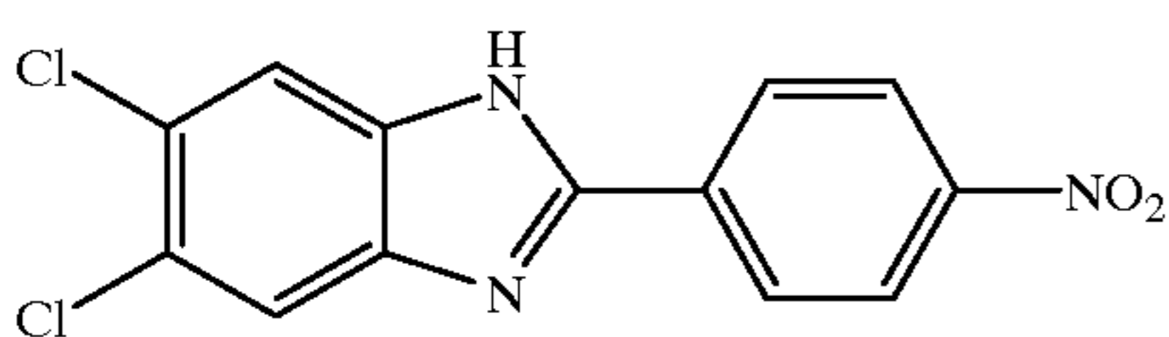
2-(4-nitrophenyl)-5,6-dichloro benzimidazole
