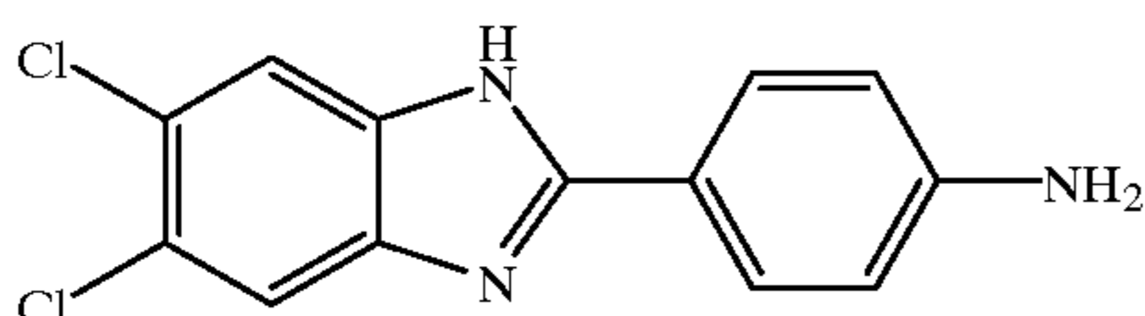
2-(4-Aminophenyl)-5,6-dichloro benzimidazole
