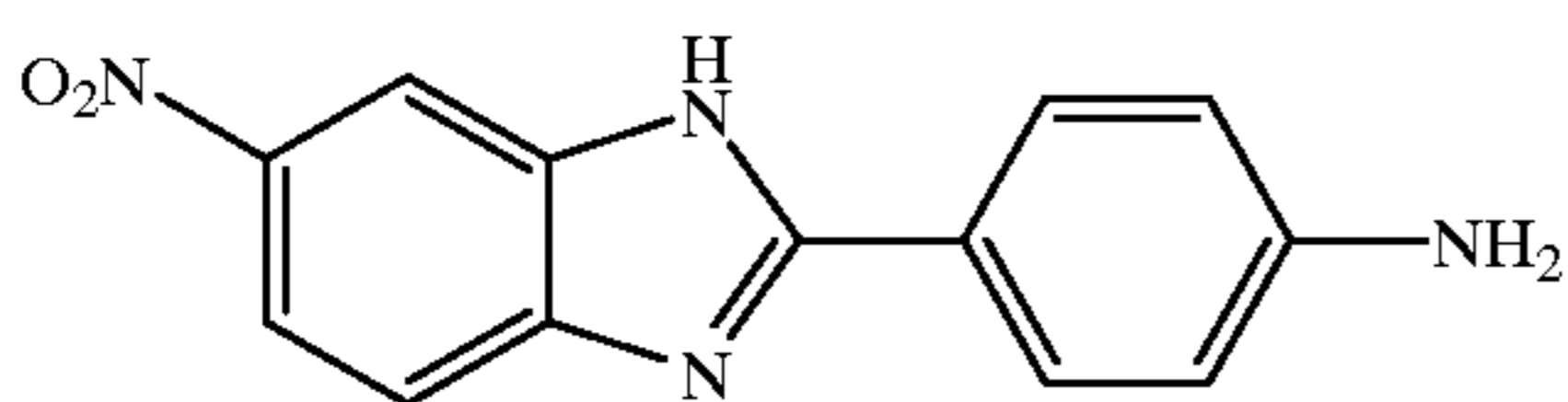
2-(4-aminophenyl)-5-methoxy benzimidazole
