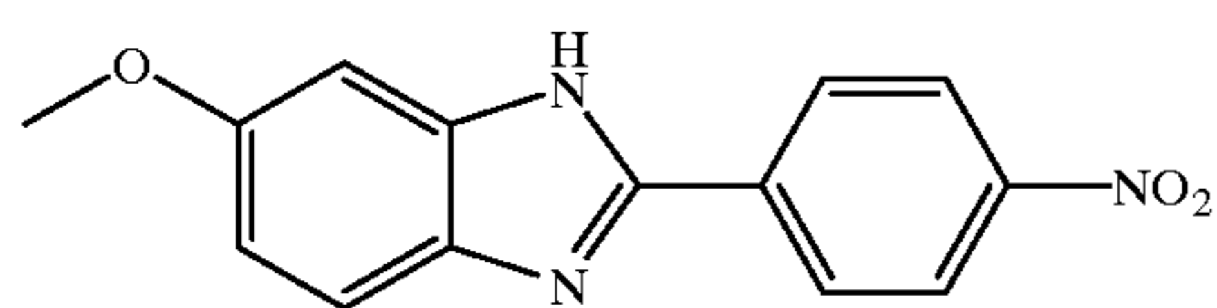
2-(4-nitrophenyl)-5-methoxy benzimidazole
