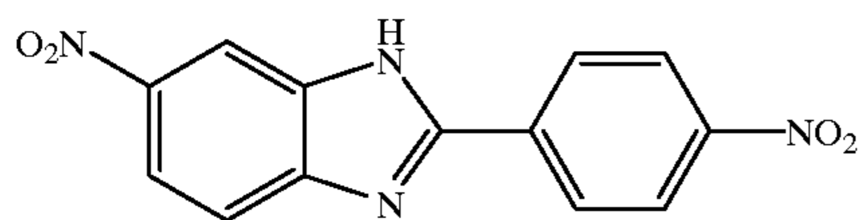
2-(4-nitrophenyl)-6-nitrobenzimidazole
