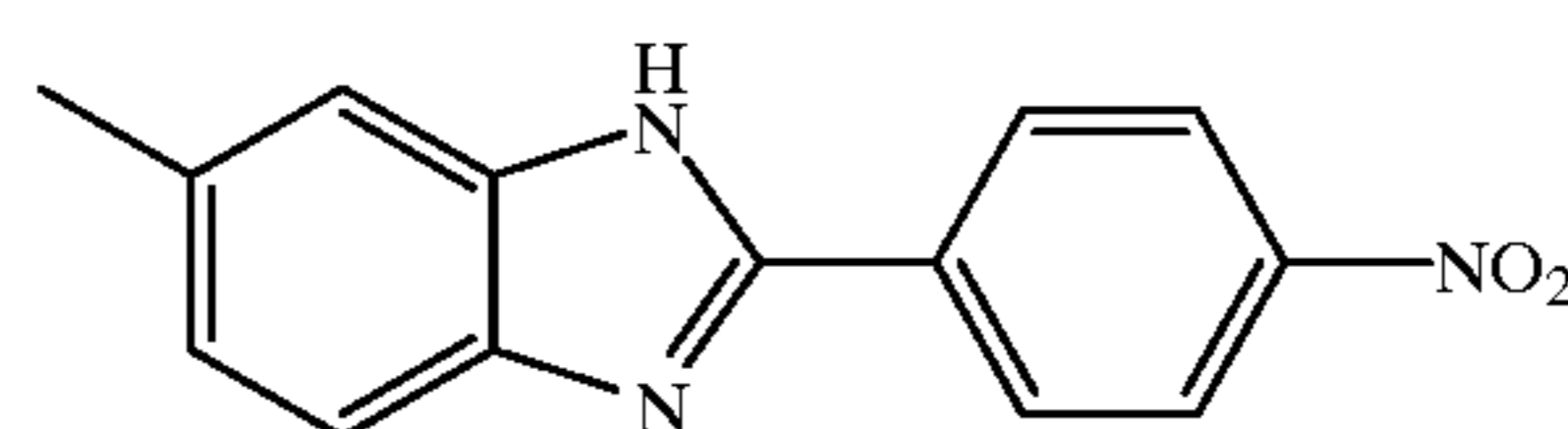
2-(4-nitrophenyl)-6-methylbenzimidazole
