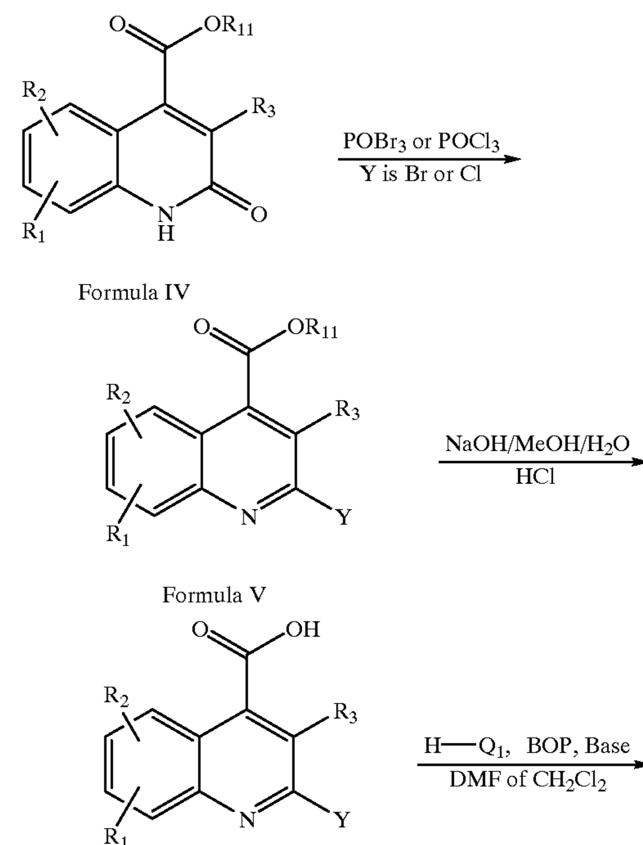
Scheme I
