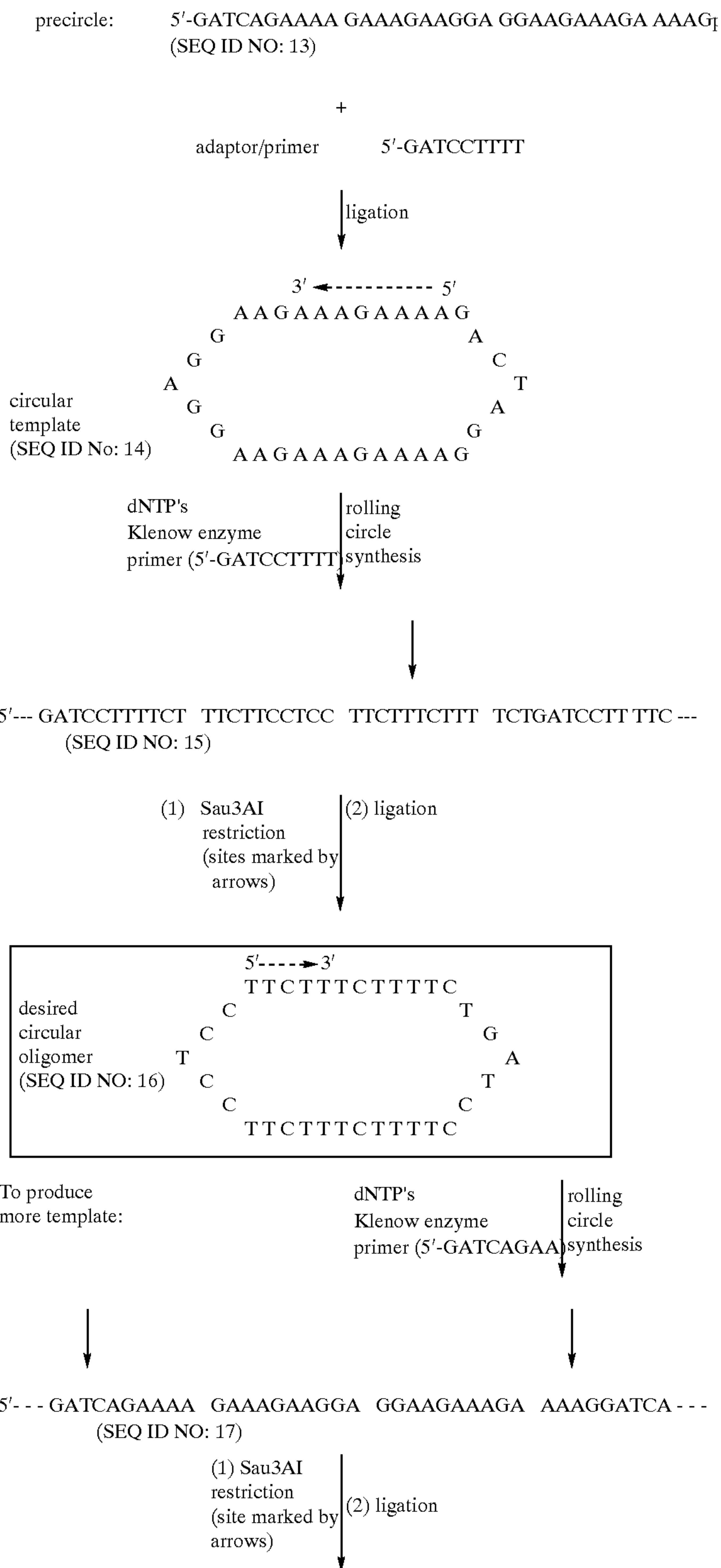
Scheme III
