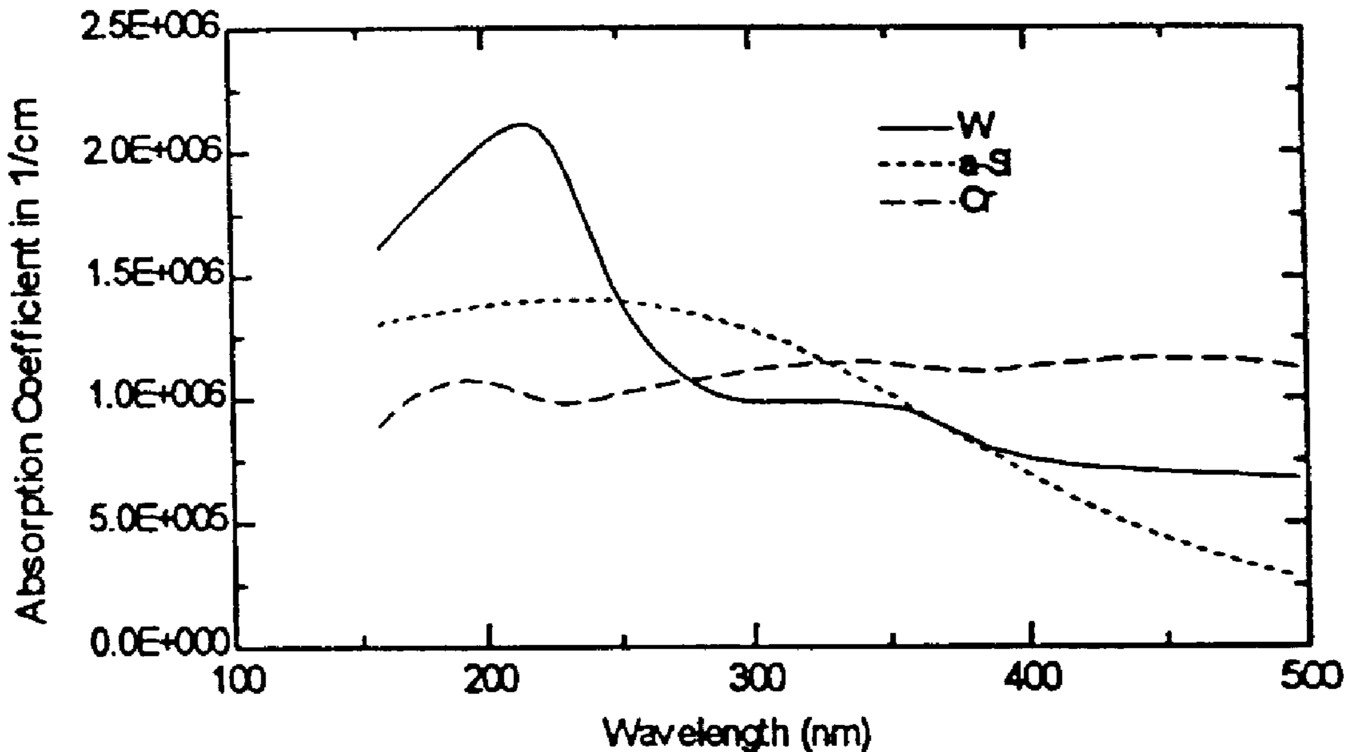
Absorption coefficients of W, Cr, and a-Si
