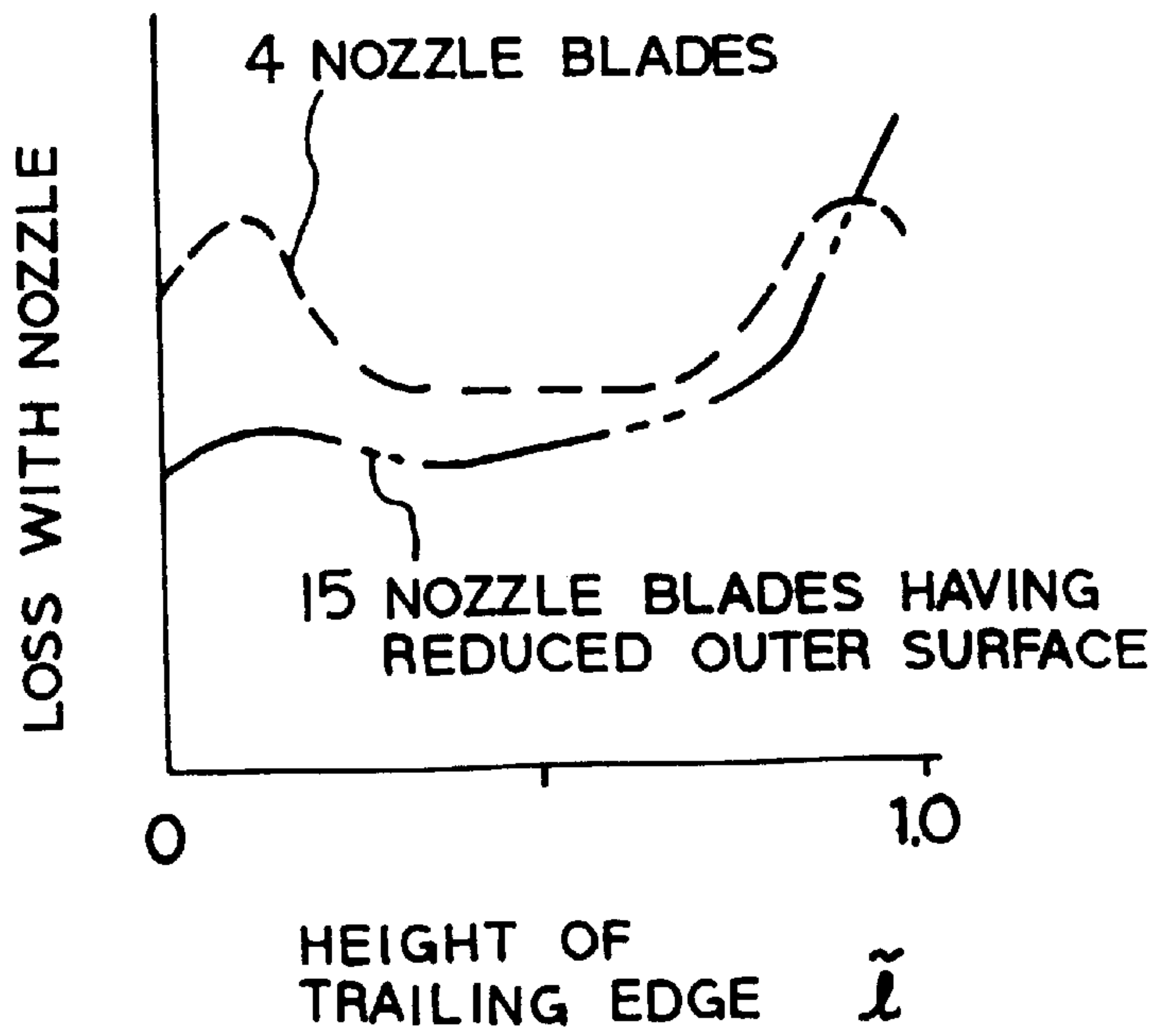
FIG. 25 PRIOR ART
