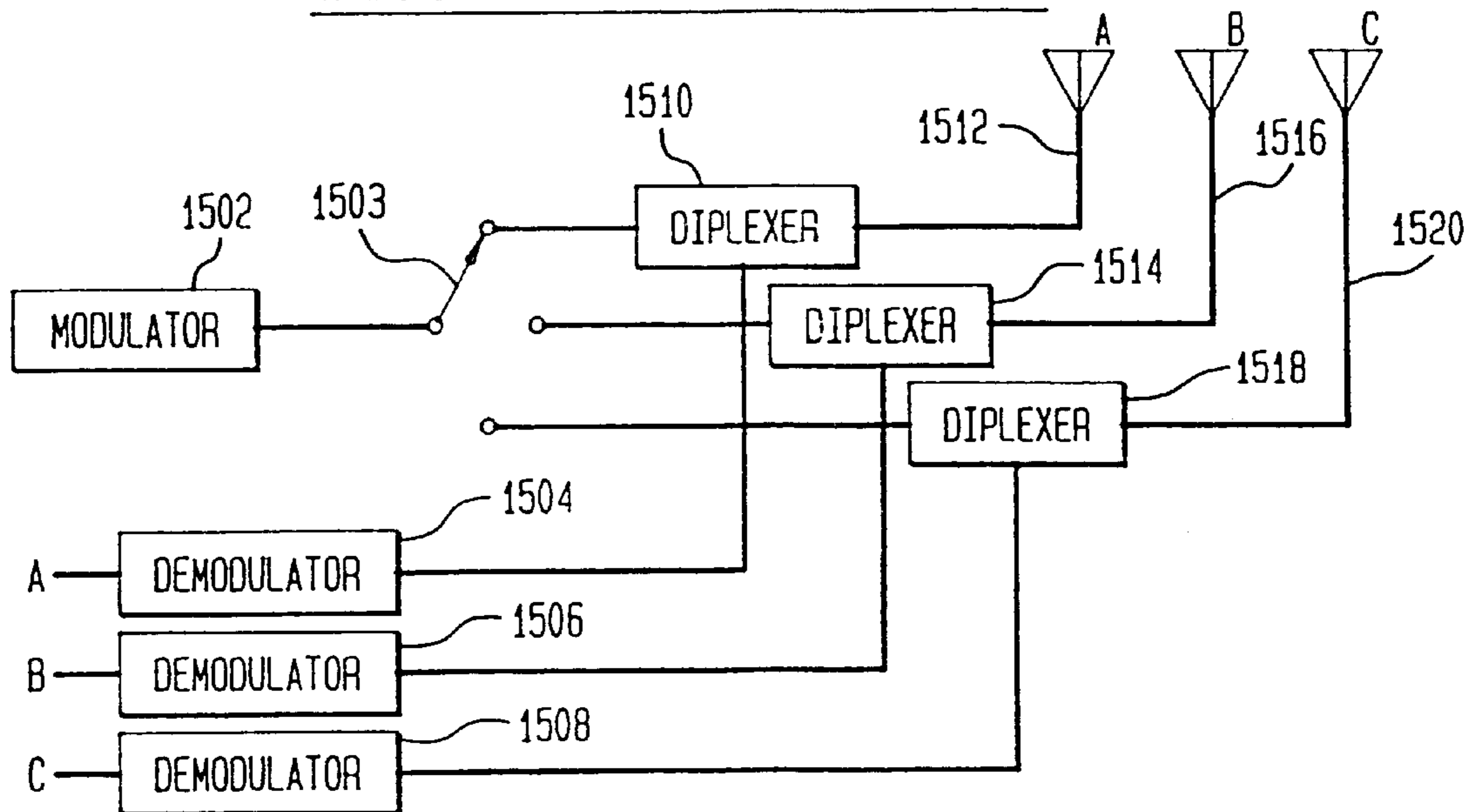
TRANSFER STATION ANTENNA IMPLEMENTATION
