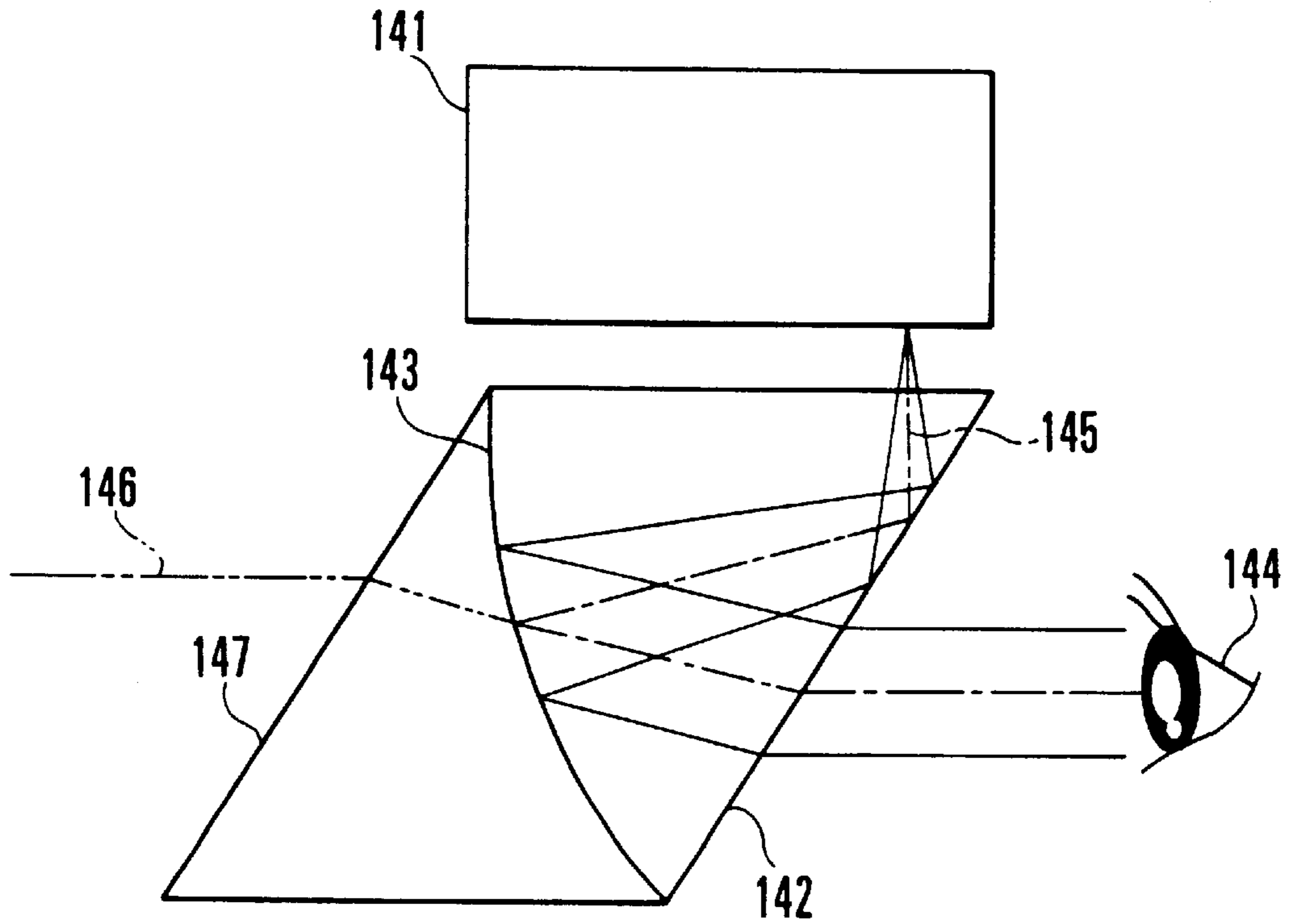
FIG. 27 PRIOR ART
