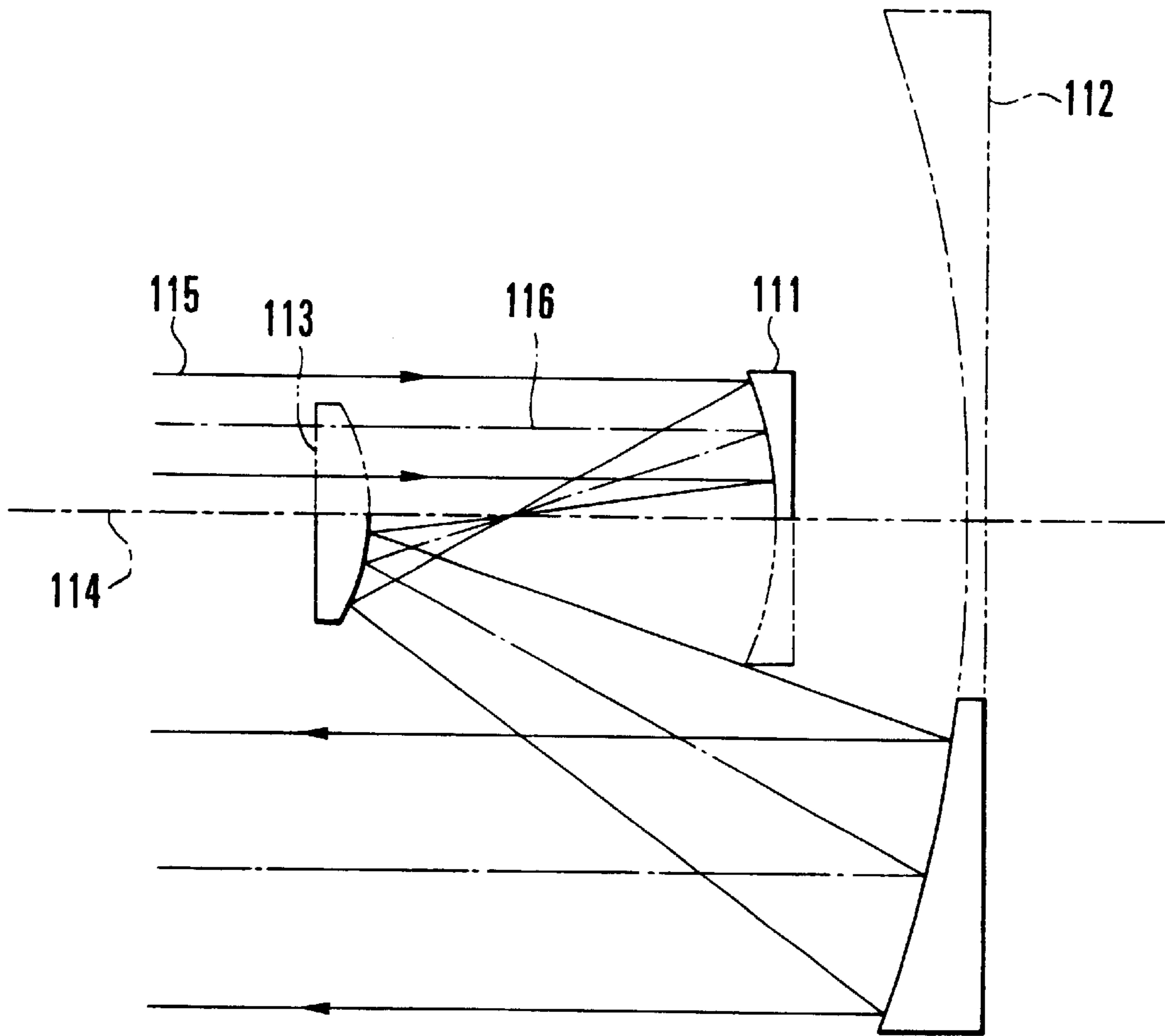
FIG. 25 PRIOR ART
