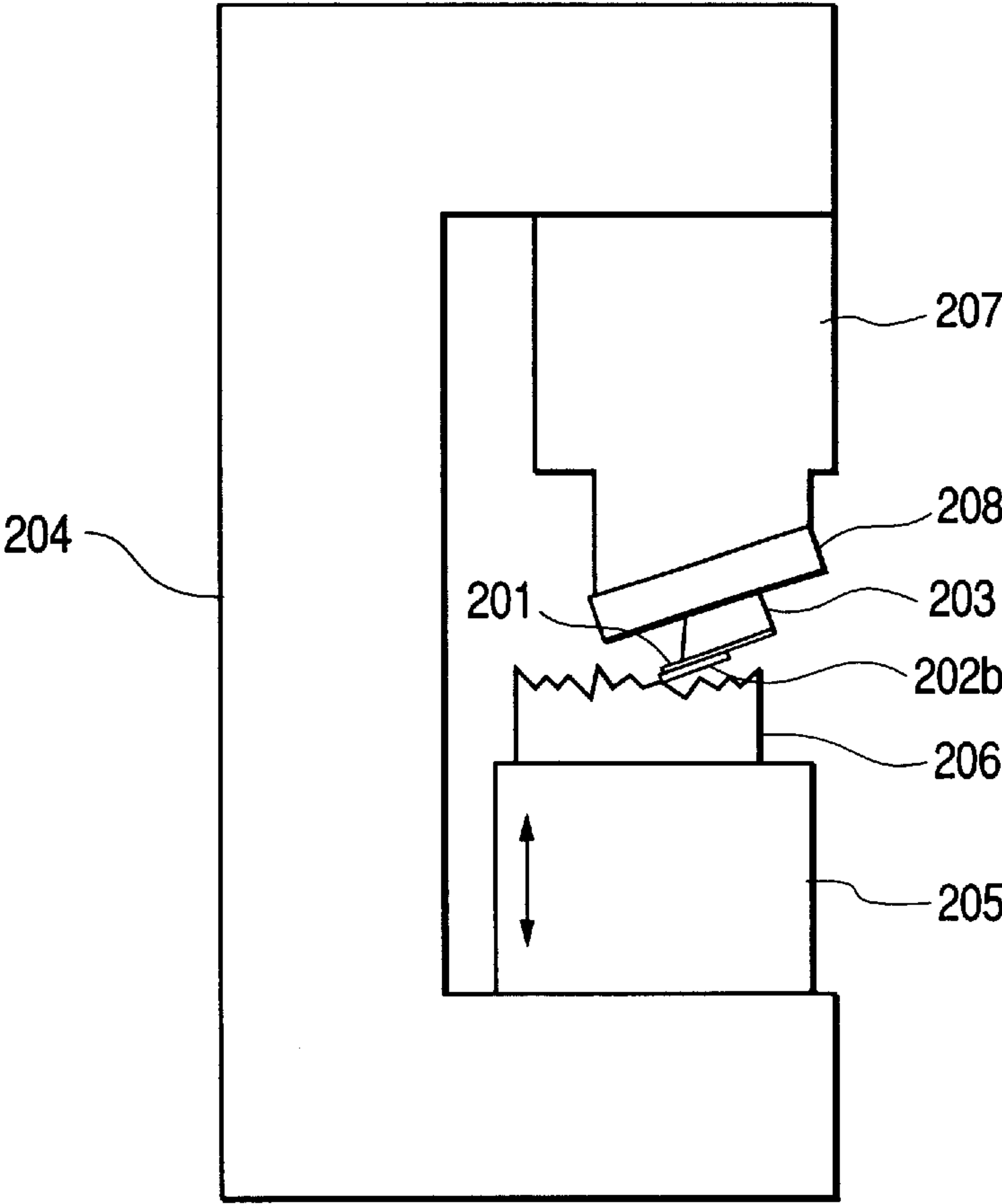
FIG. 19 PRIOR ART
