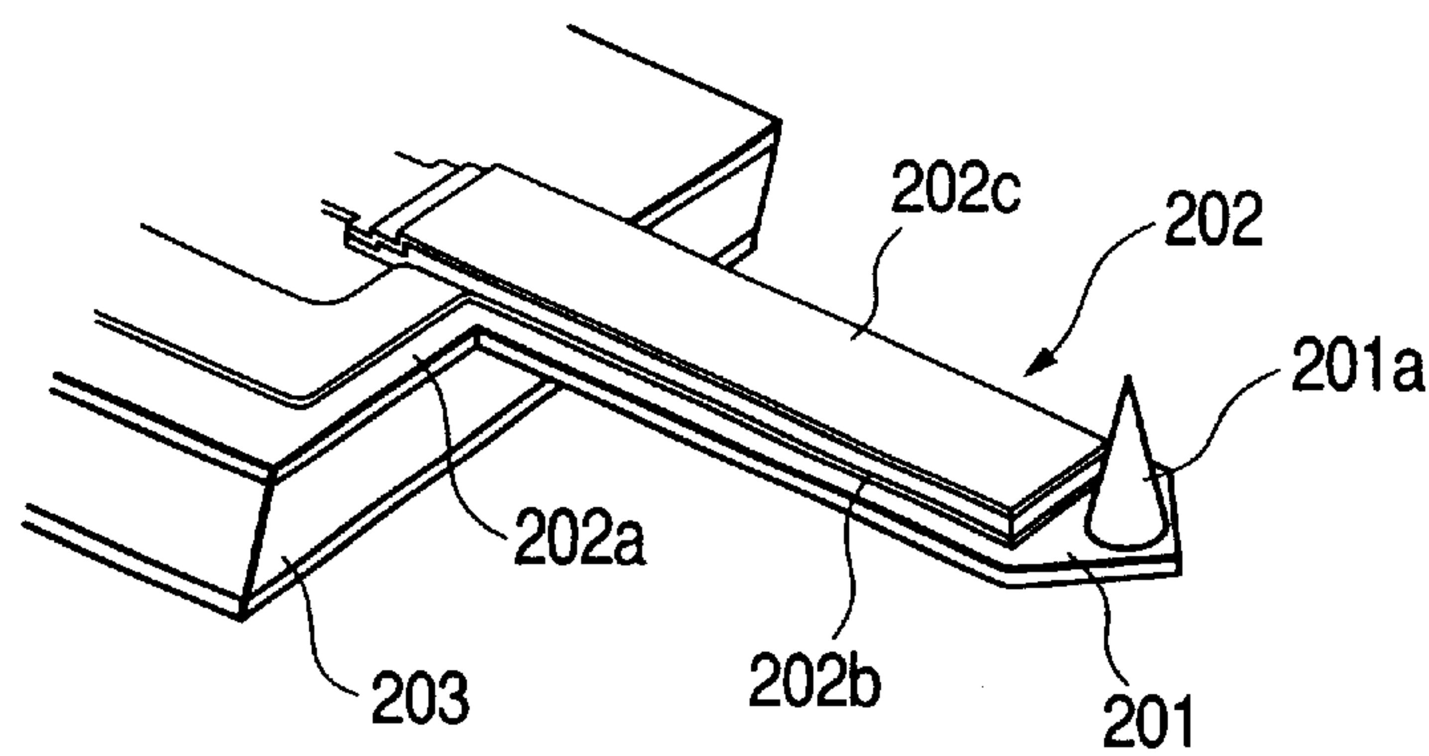
FIG. 18 PRIOR ART
