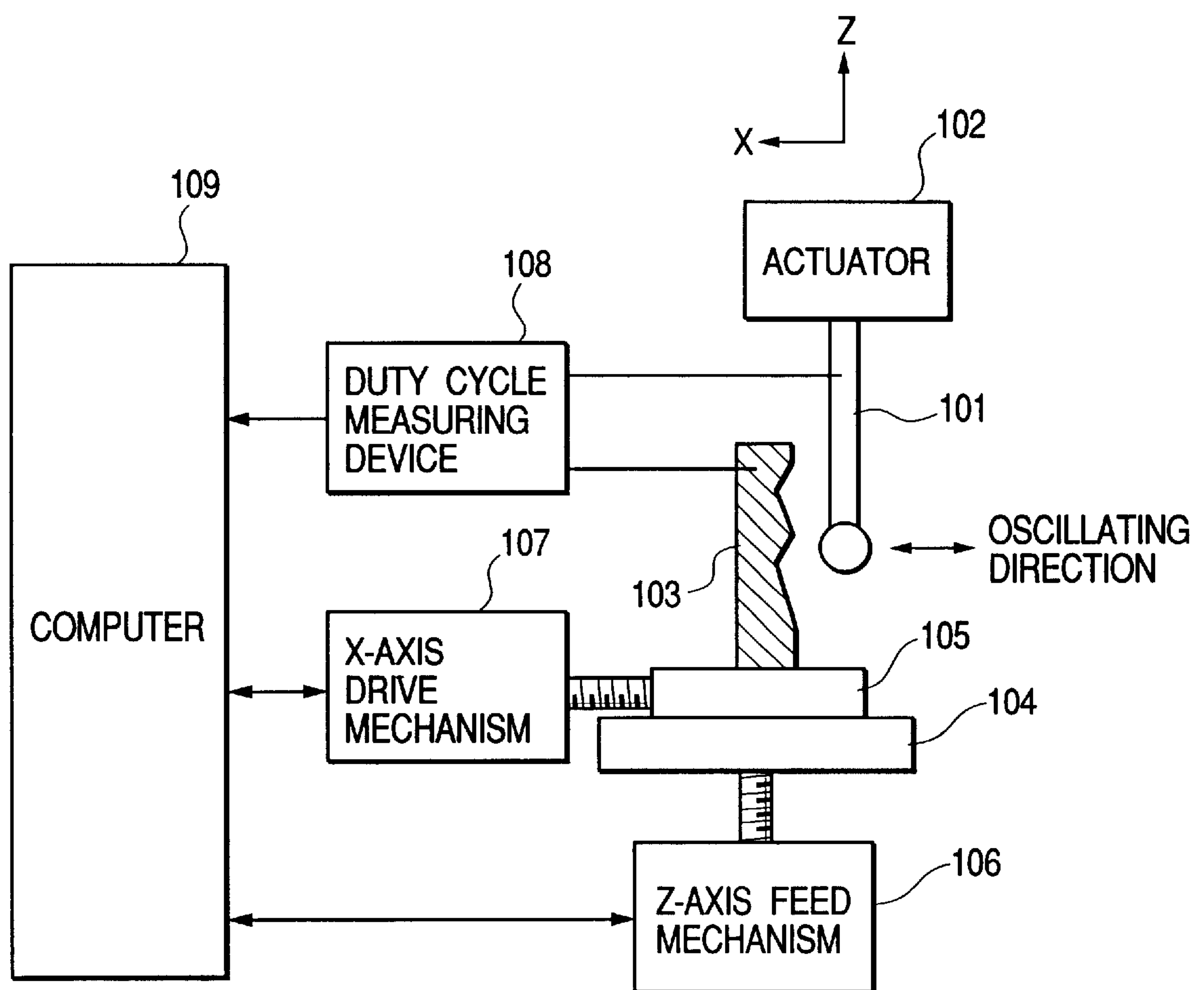
FIG. 15 PRIOR ART
