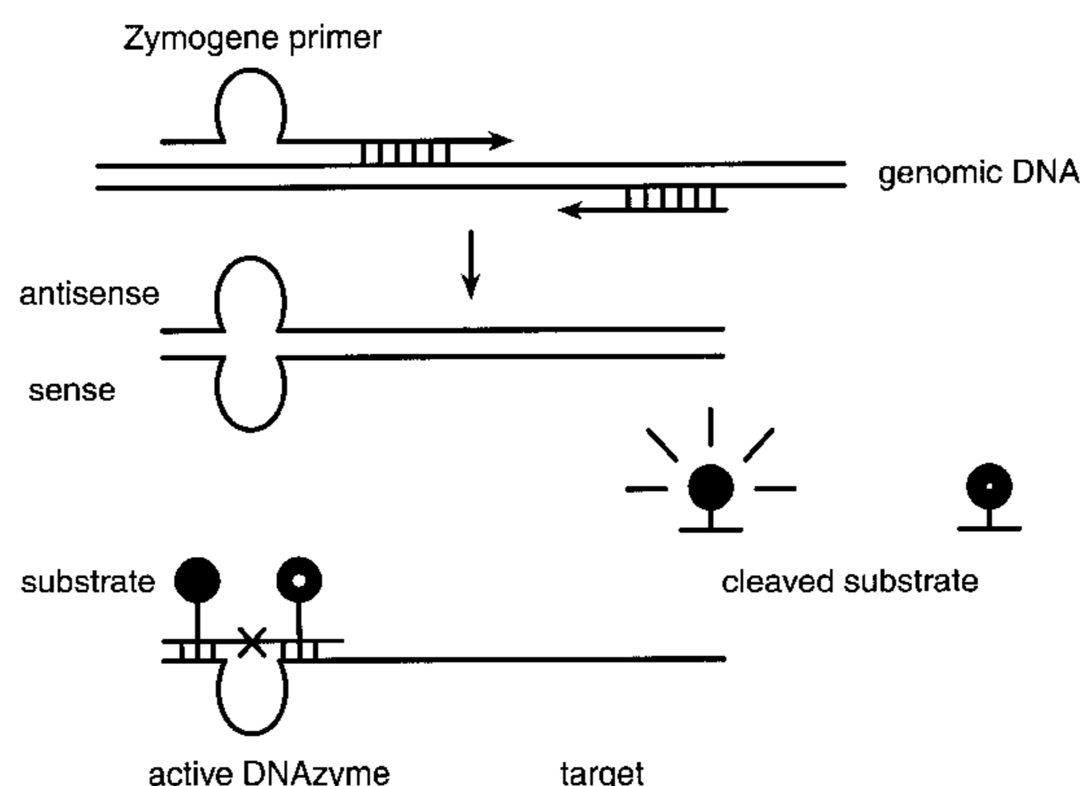
Homogeneous PCR amplification and detection
