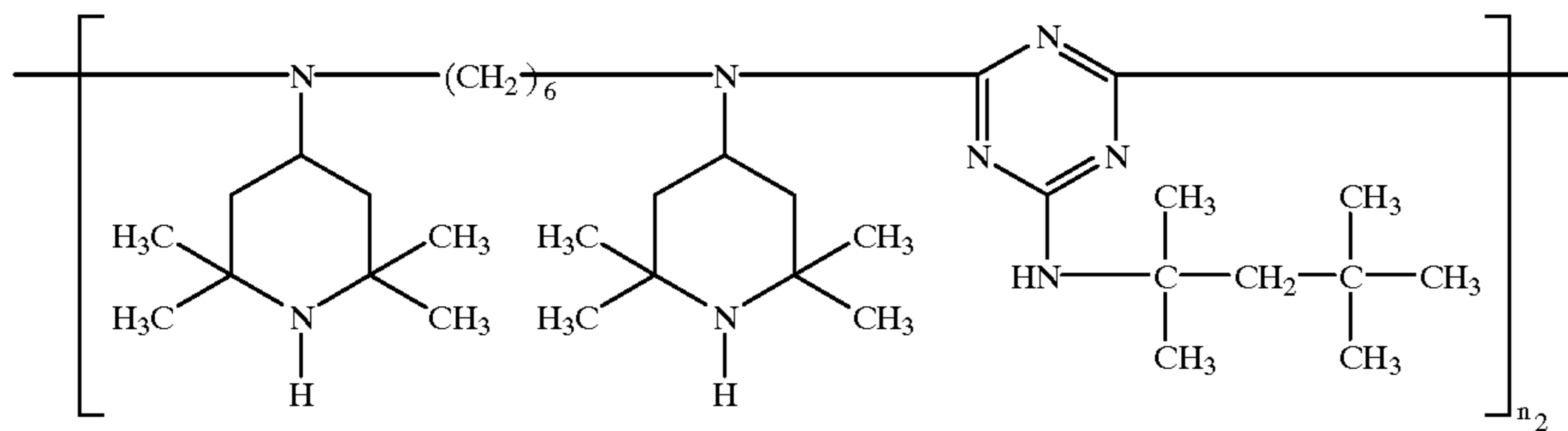
Compound E
