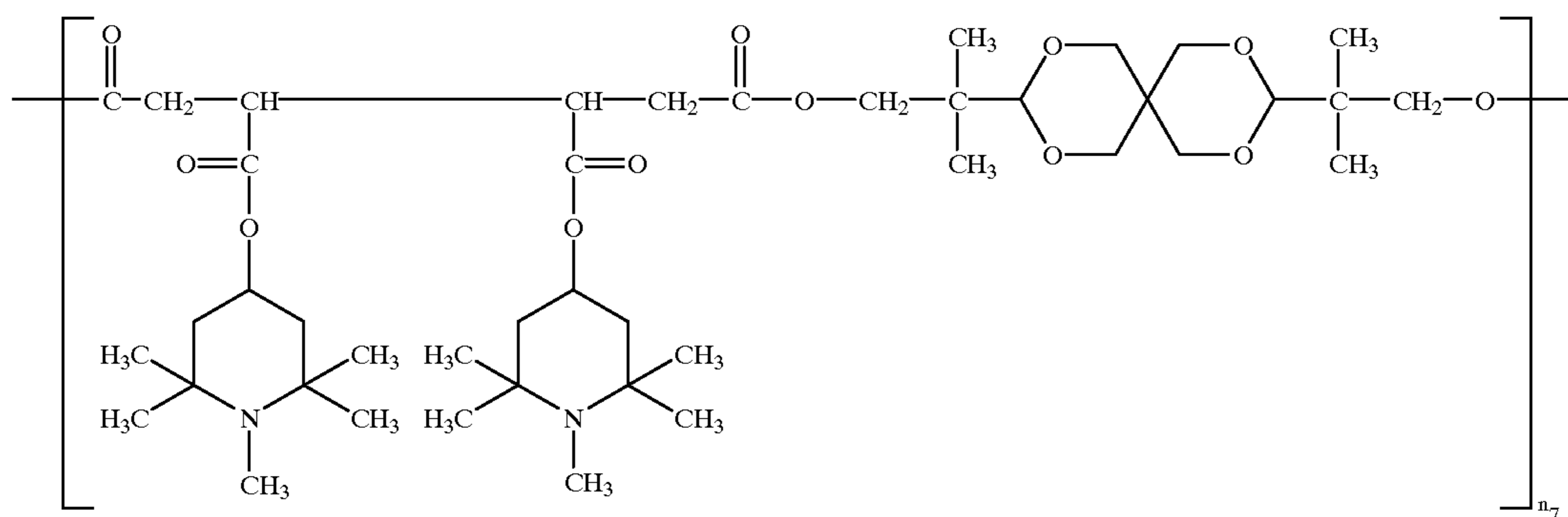
Compound G-1
