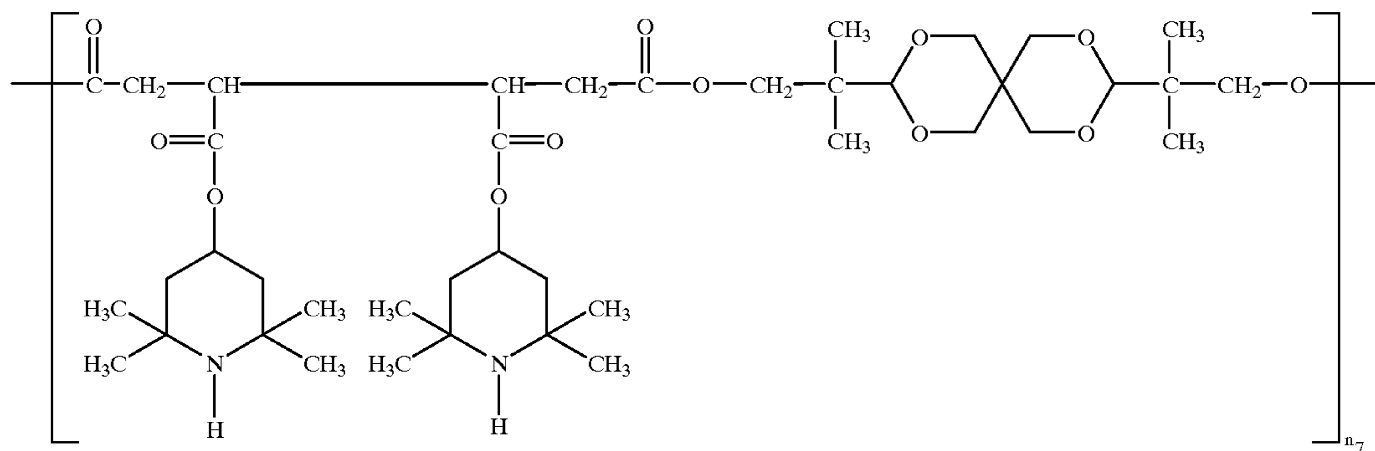
Compound G-2
