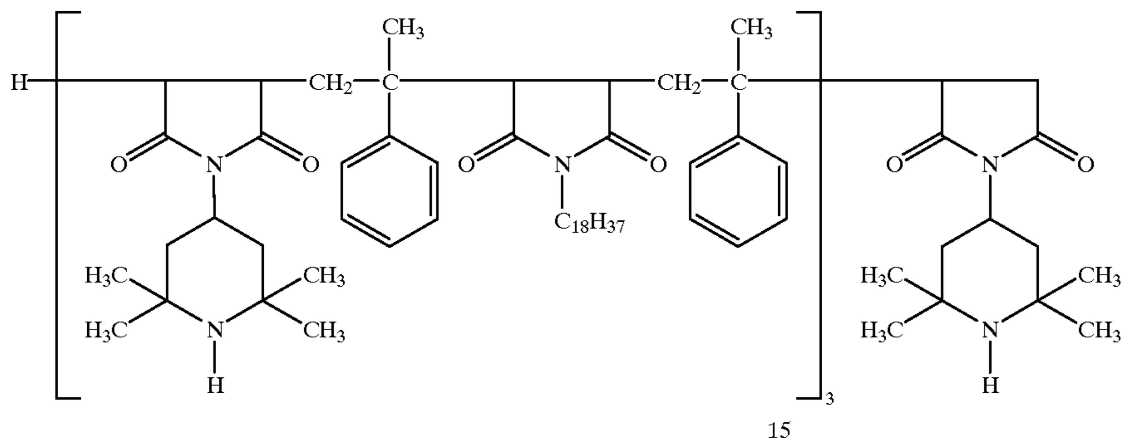
Compound G-1
