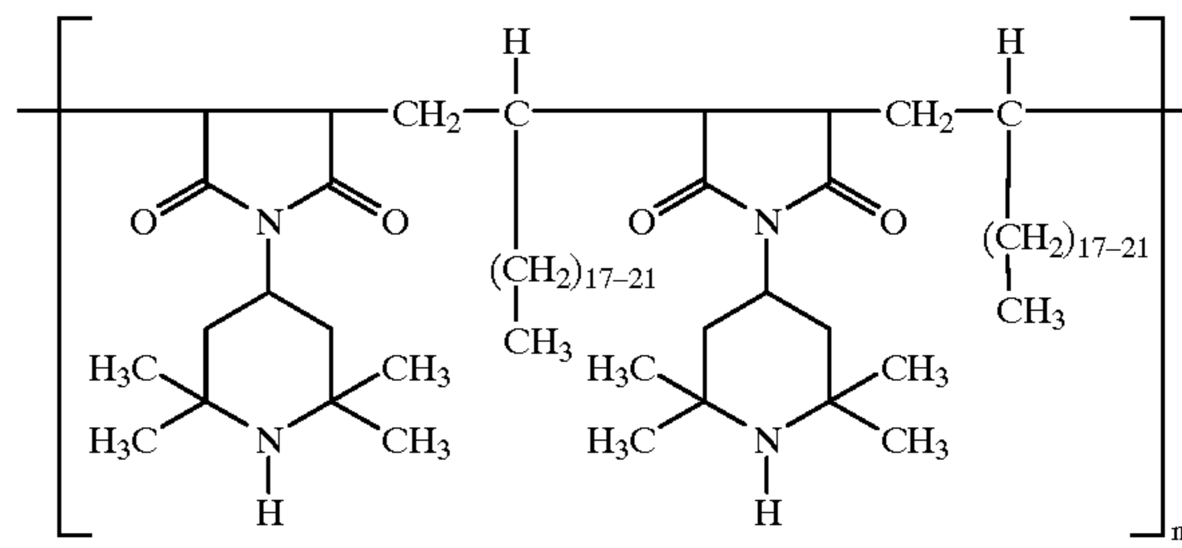
Compound F-1
