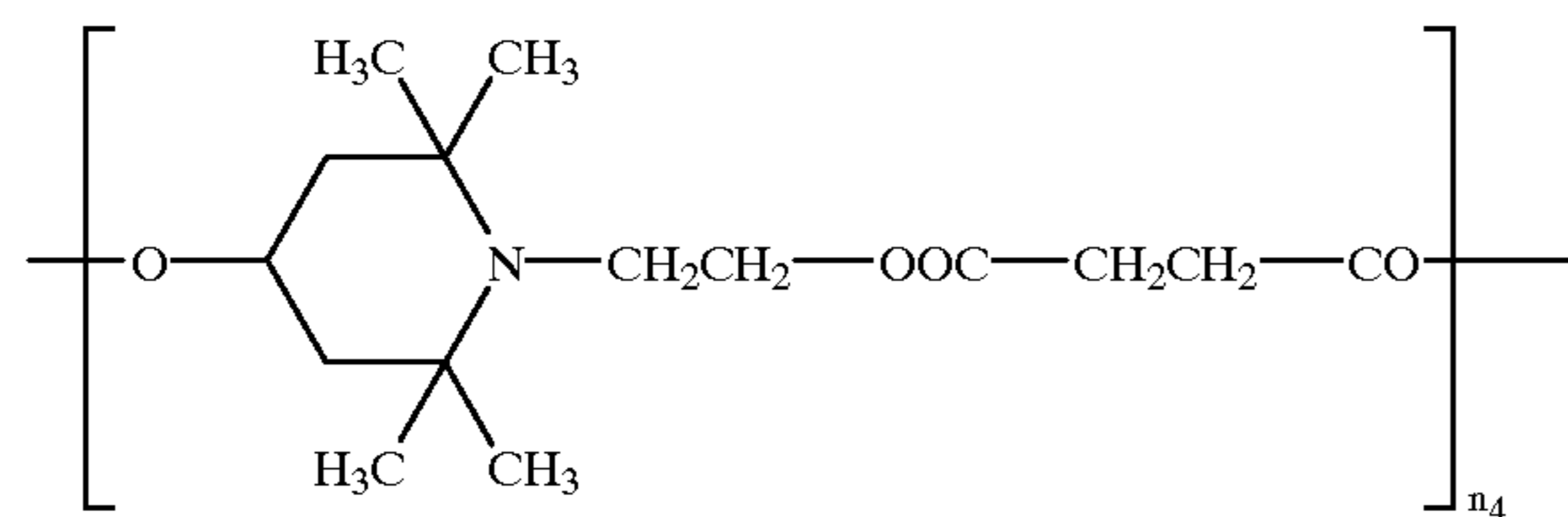
Compound D
