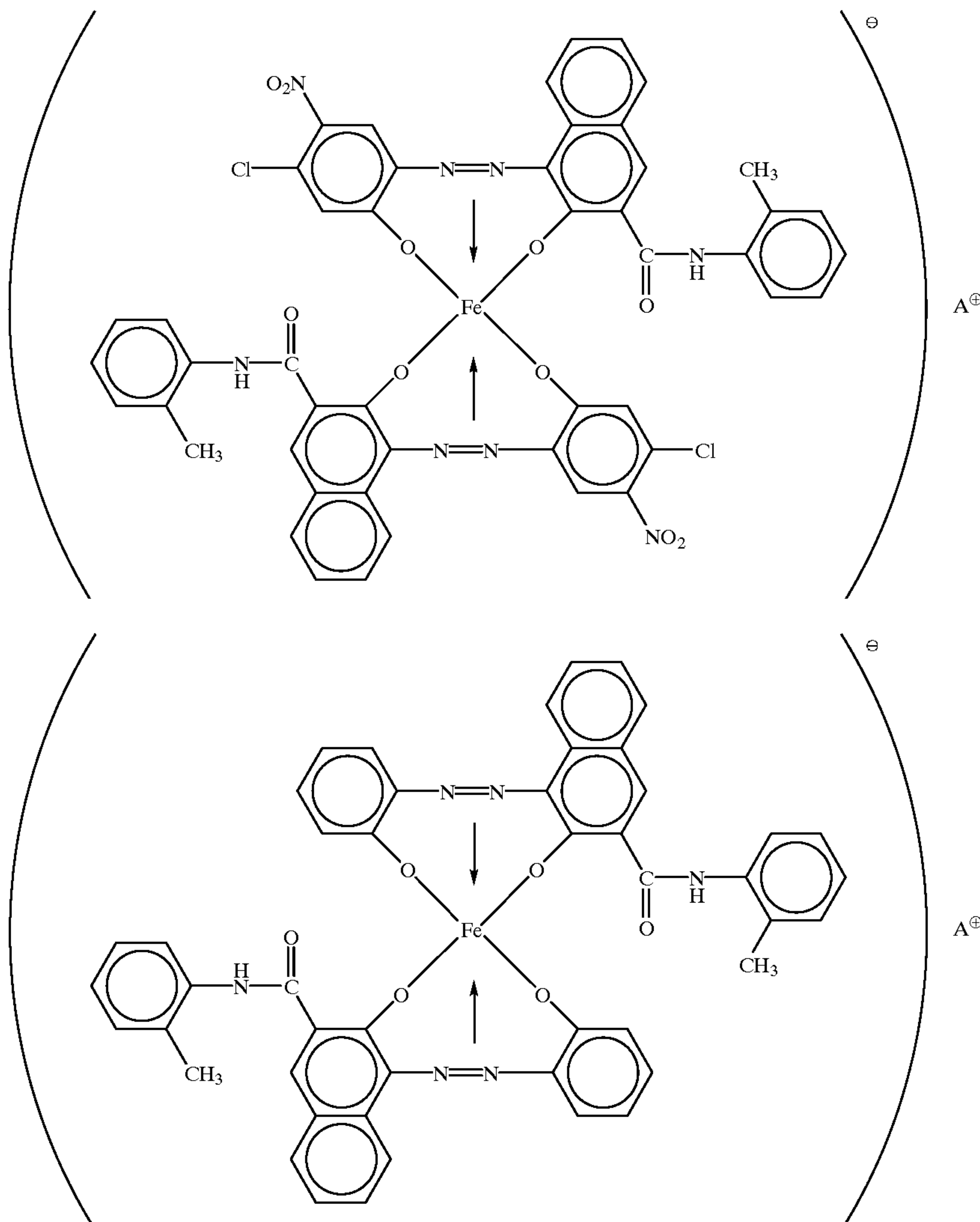
Iron Complex (6)
