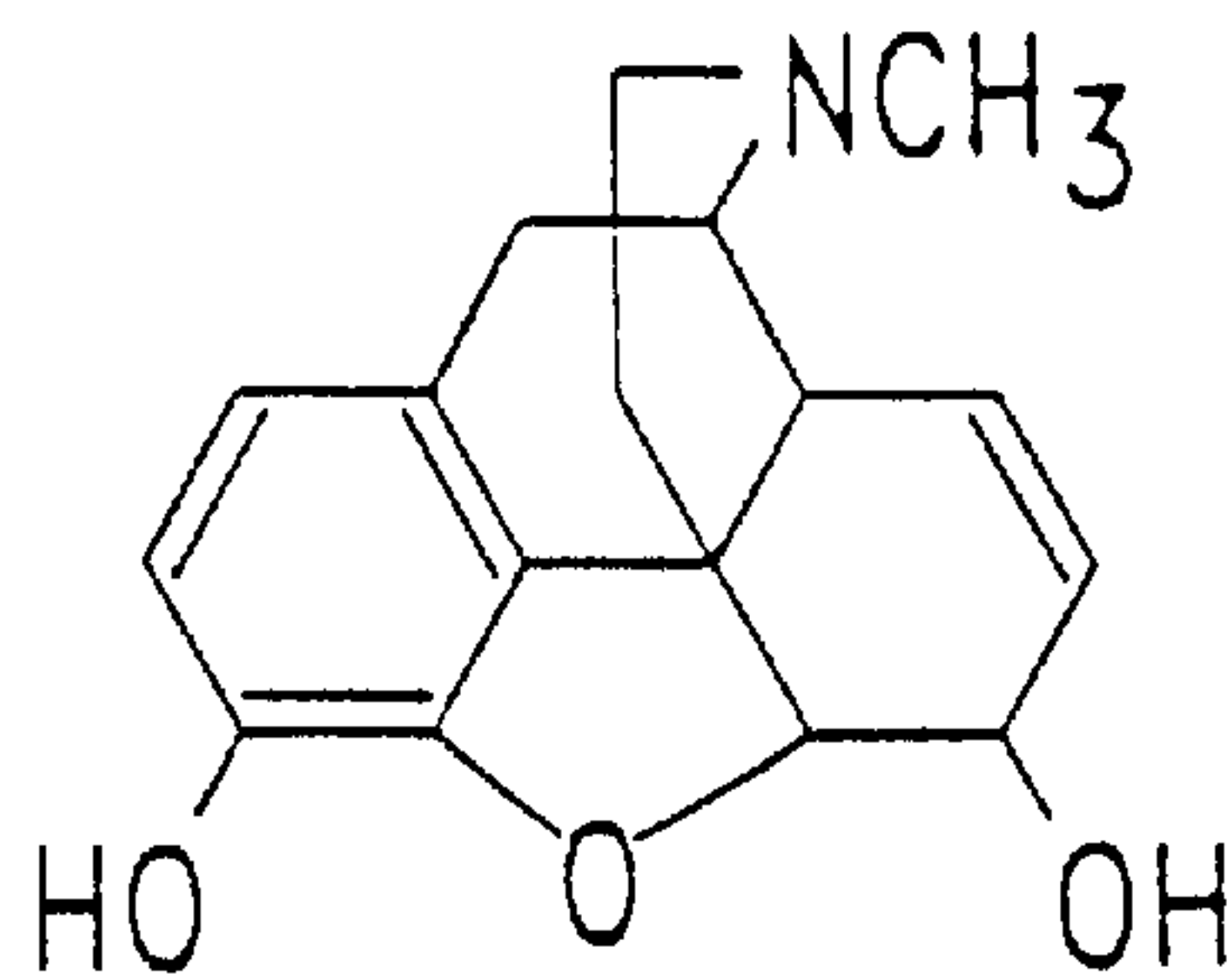
Morphine
