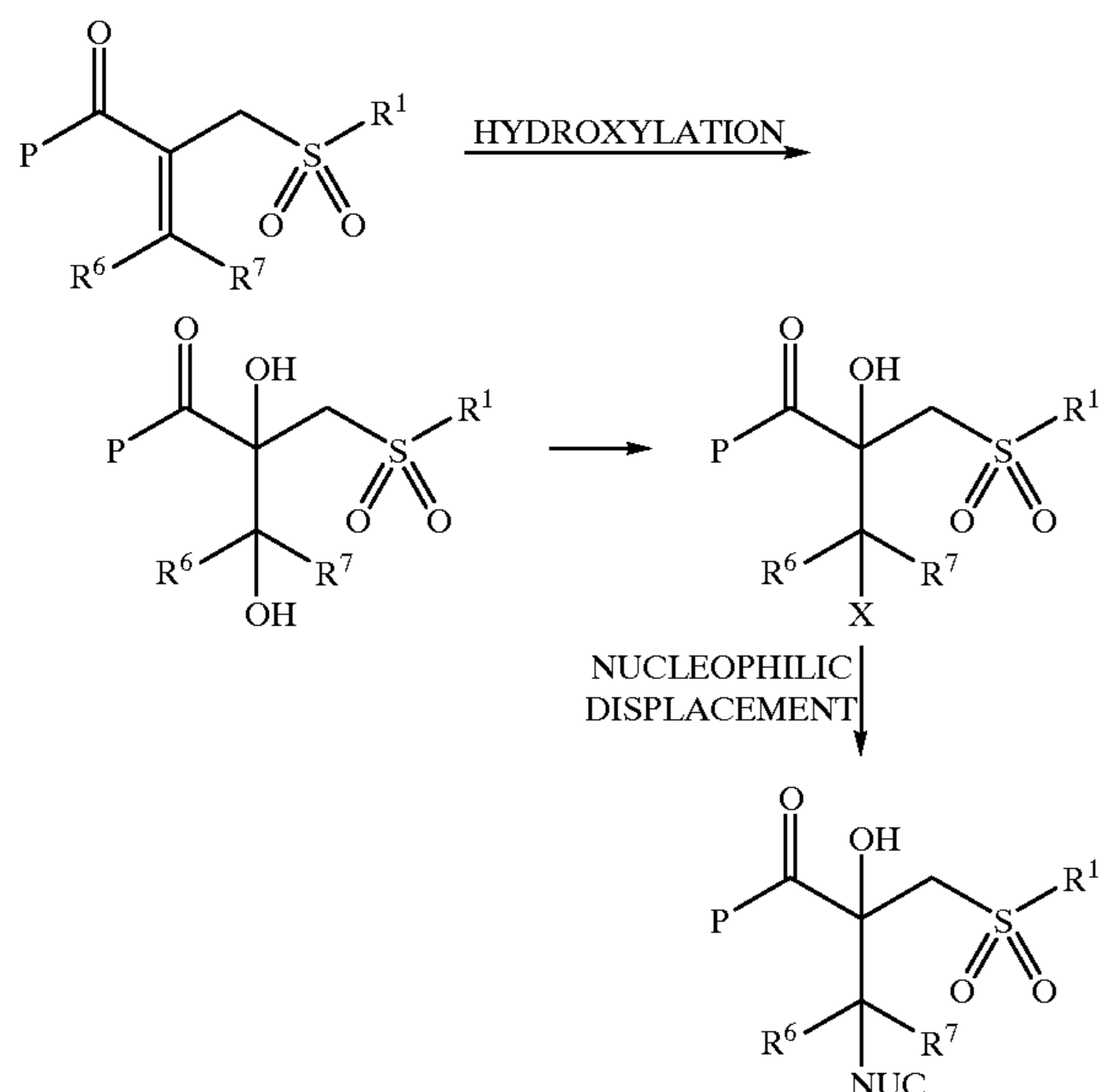
SCHEME IV
