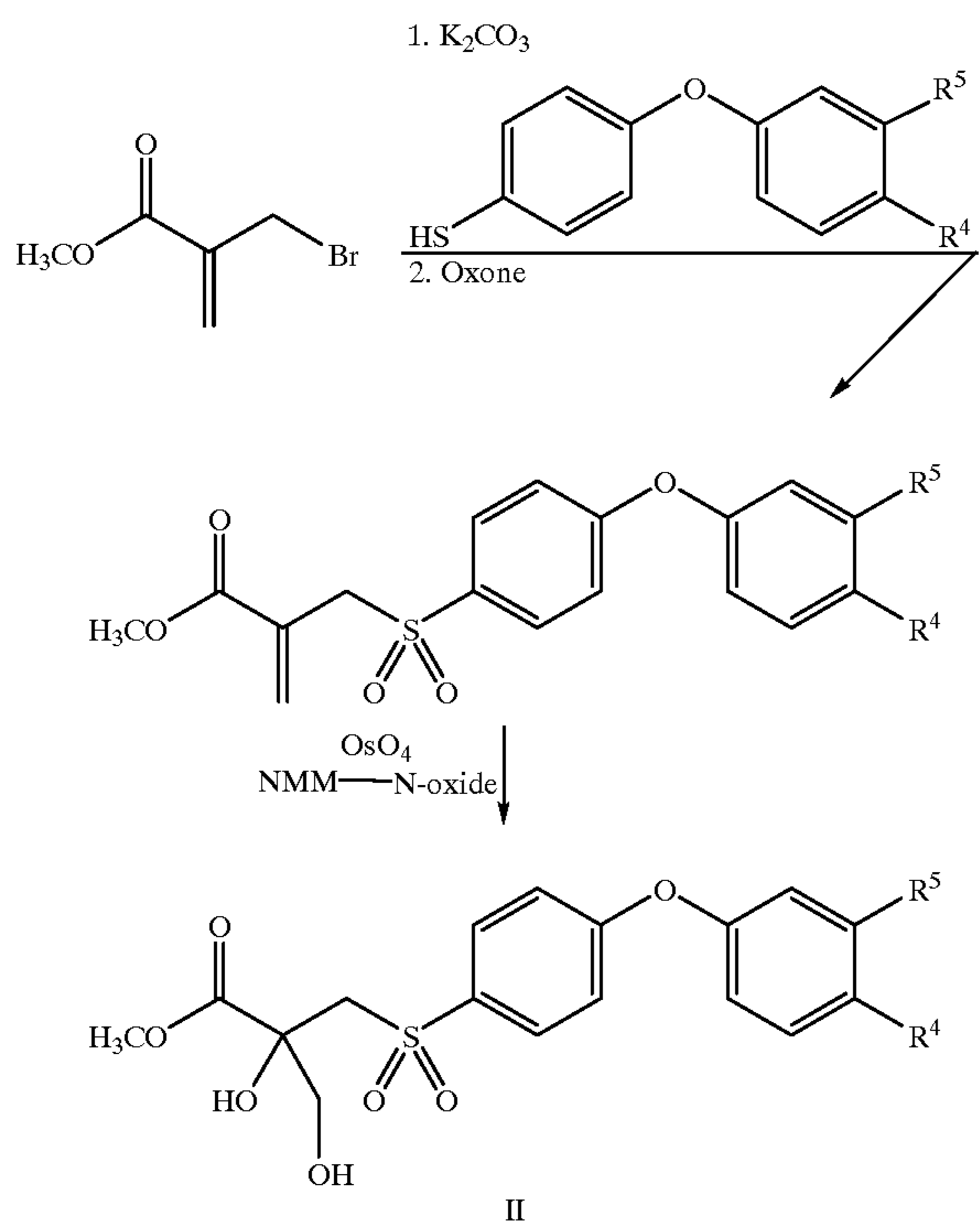
SCHEME 2 Examples 2-4, 6 and 7
