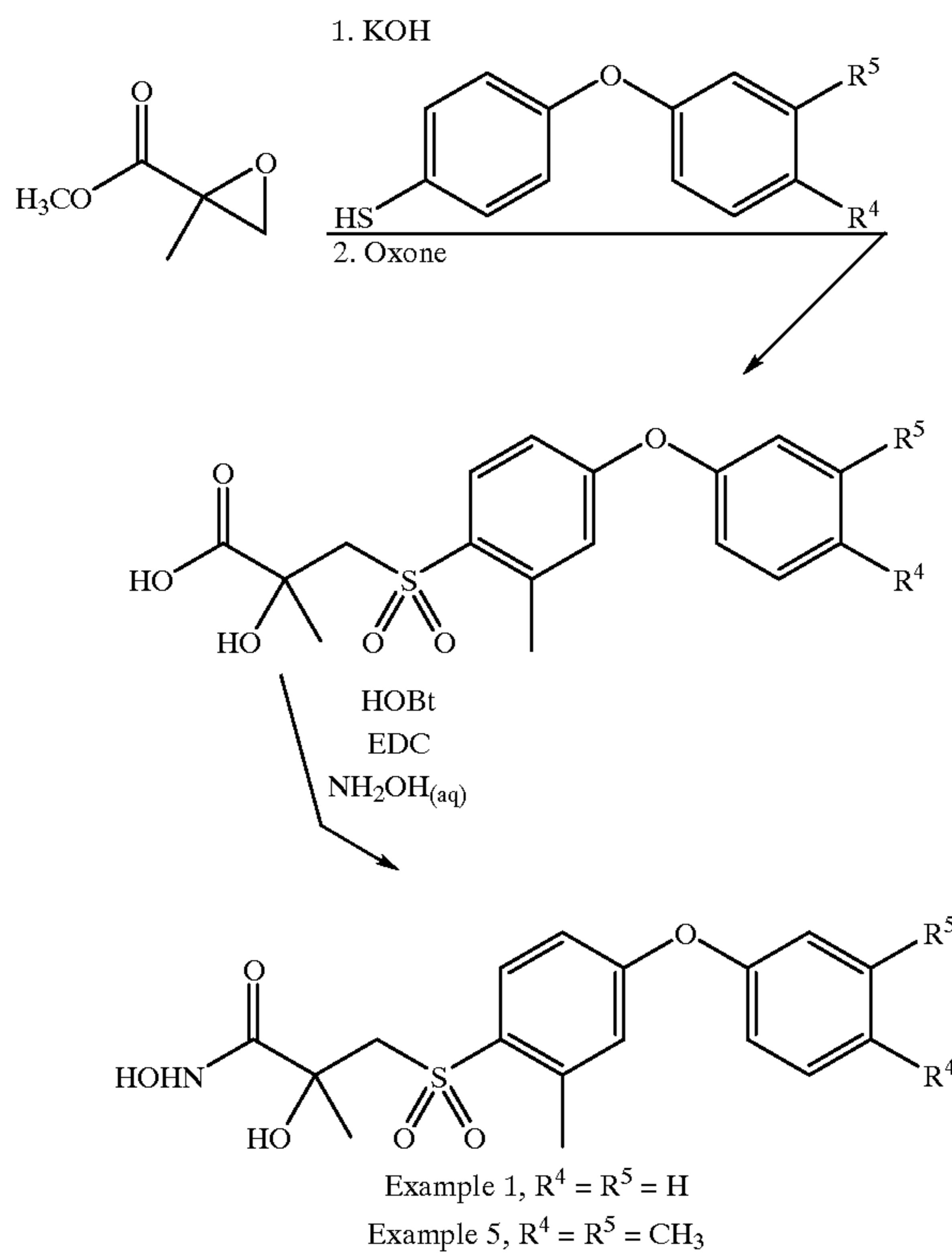
SCHEME 1 Examples 1 and 5
