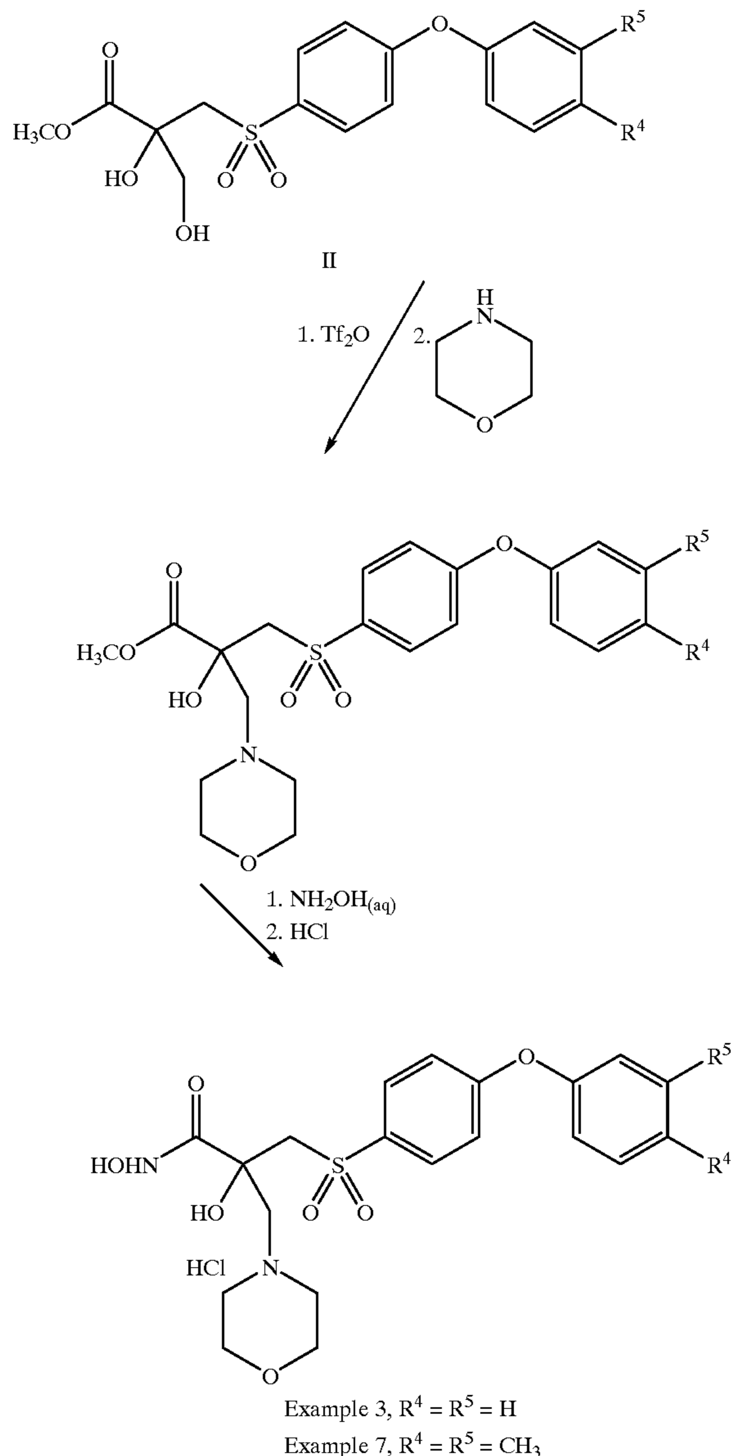
SCHEME 2C Examples 2-4, 6 and 7
