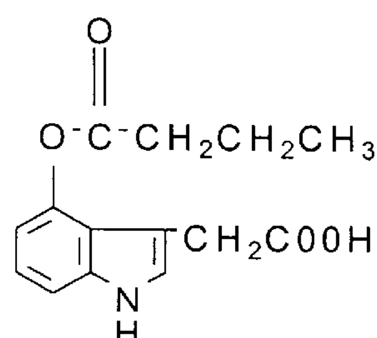
4-butyryloxy-IAA
