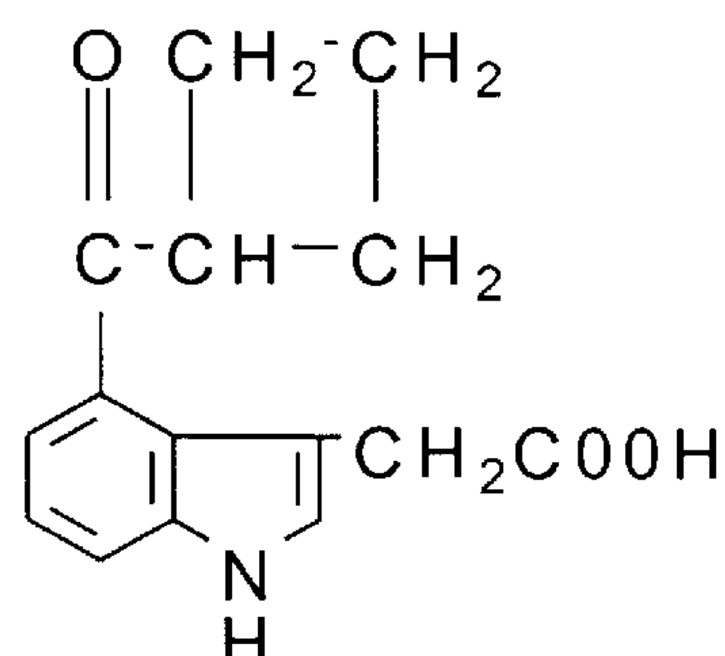
4-cyclovaleryl-IAA
