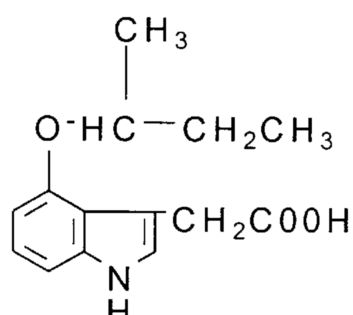
4-sec-butoxy-IAA
