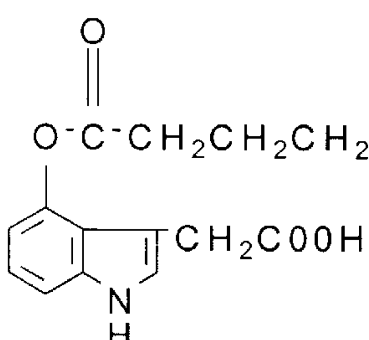
4-valeryloxy-IAA
