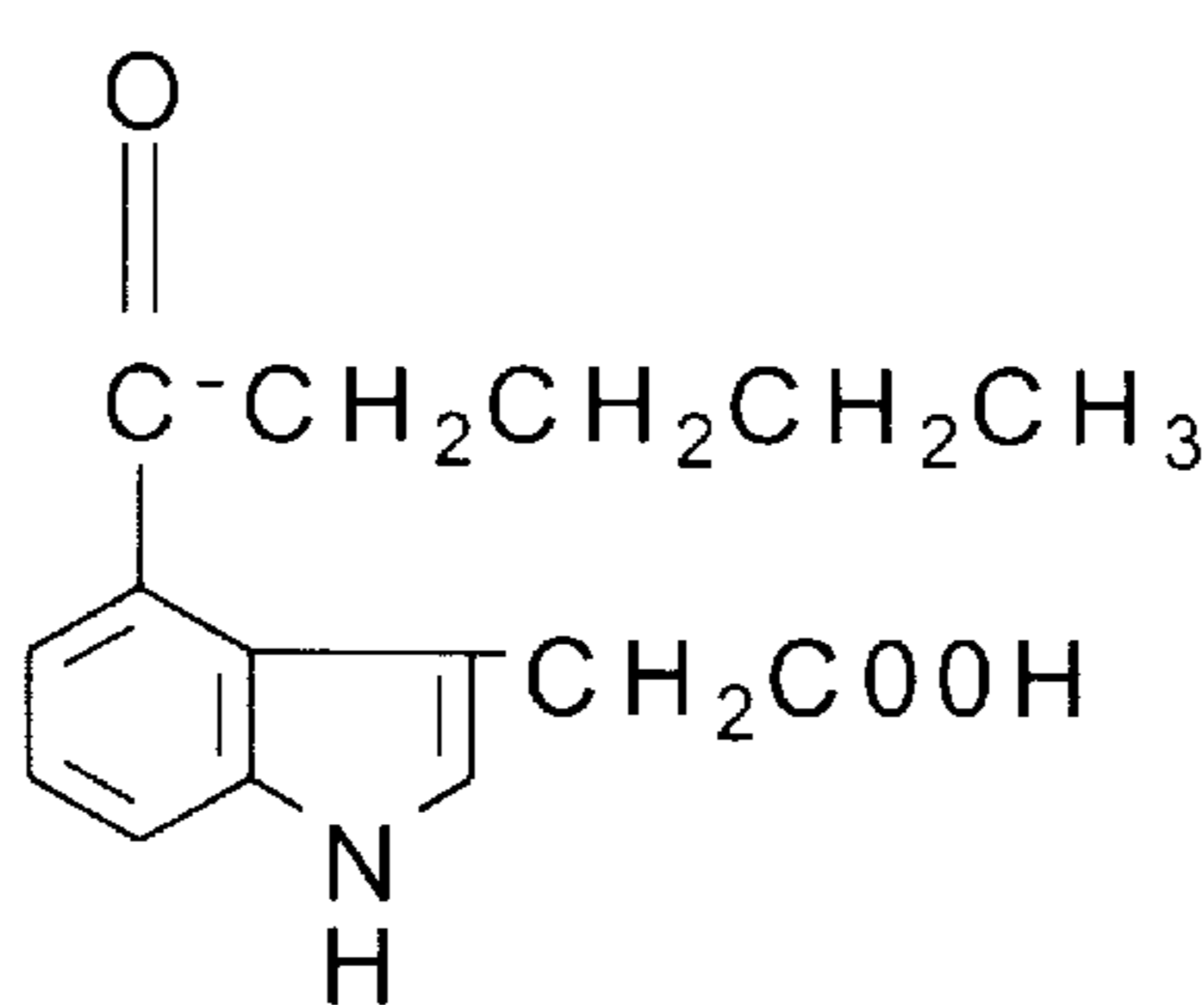
4-valeryl-IAA
