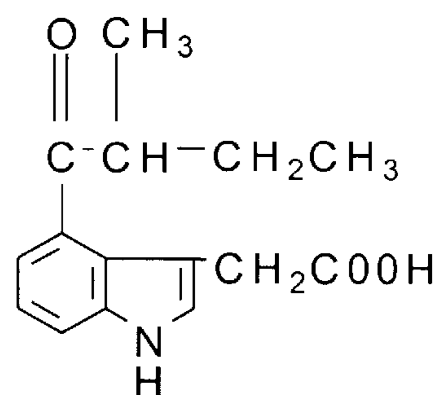
4-sec-valeryl-IAA
