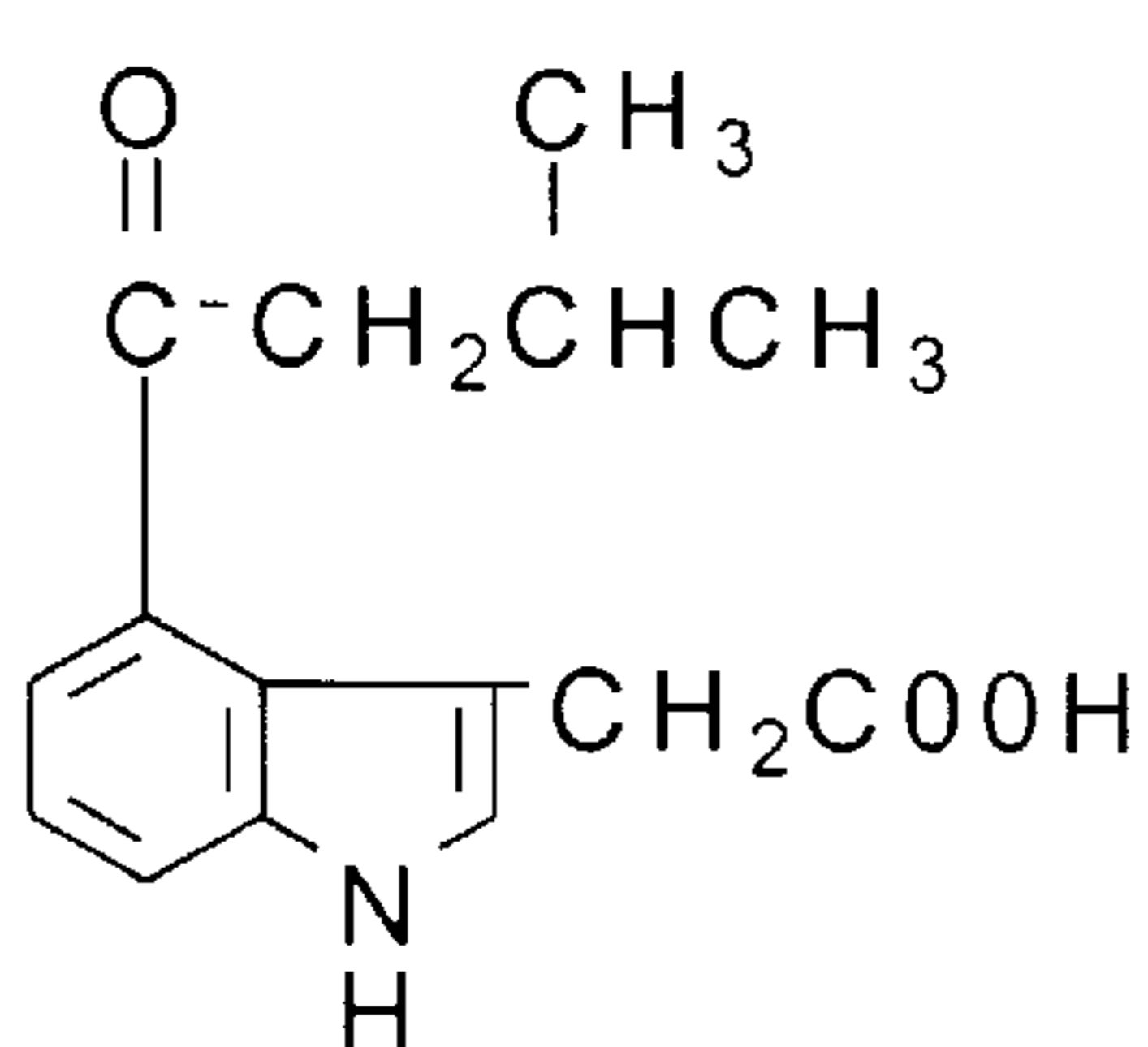
4-iso-valeryl-IAA
