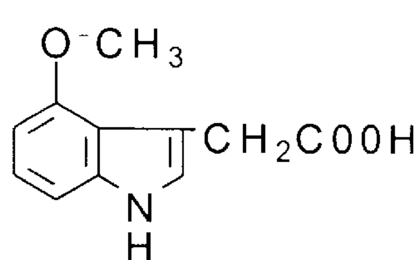
4-methoxy-IAA
