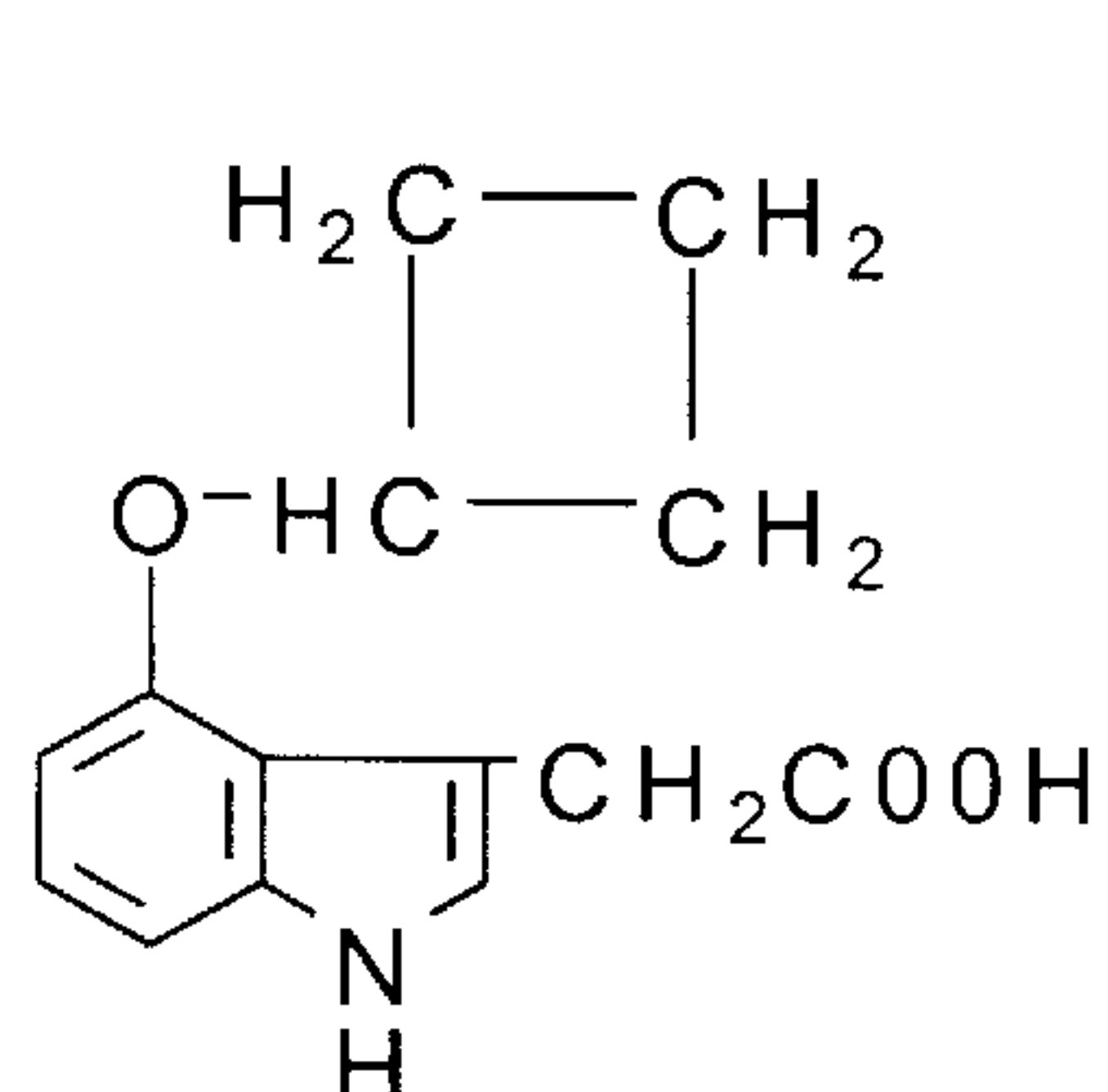
4-cyclobutoxy-IAA
