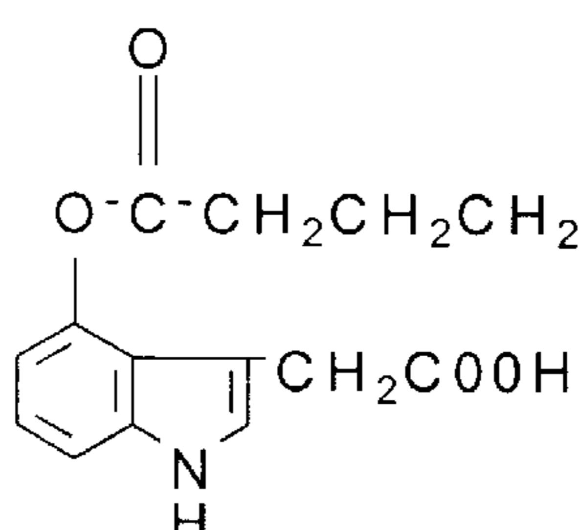
4-valeryloxy-IAA
