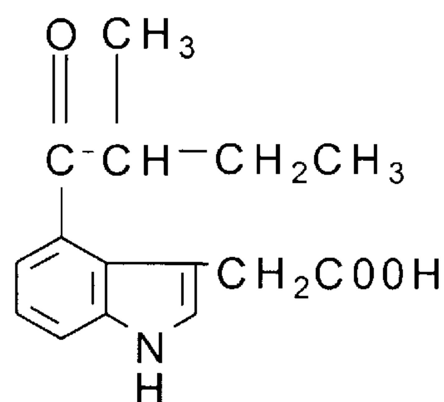
4-sec-valeryl-IAA
