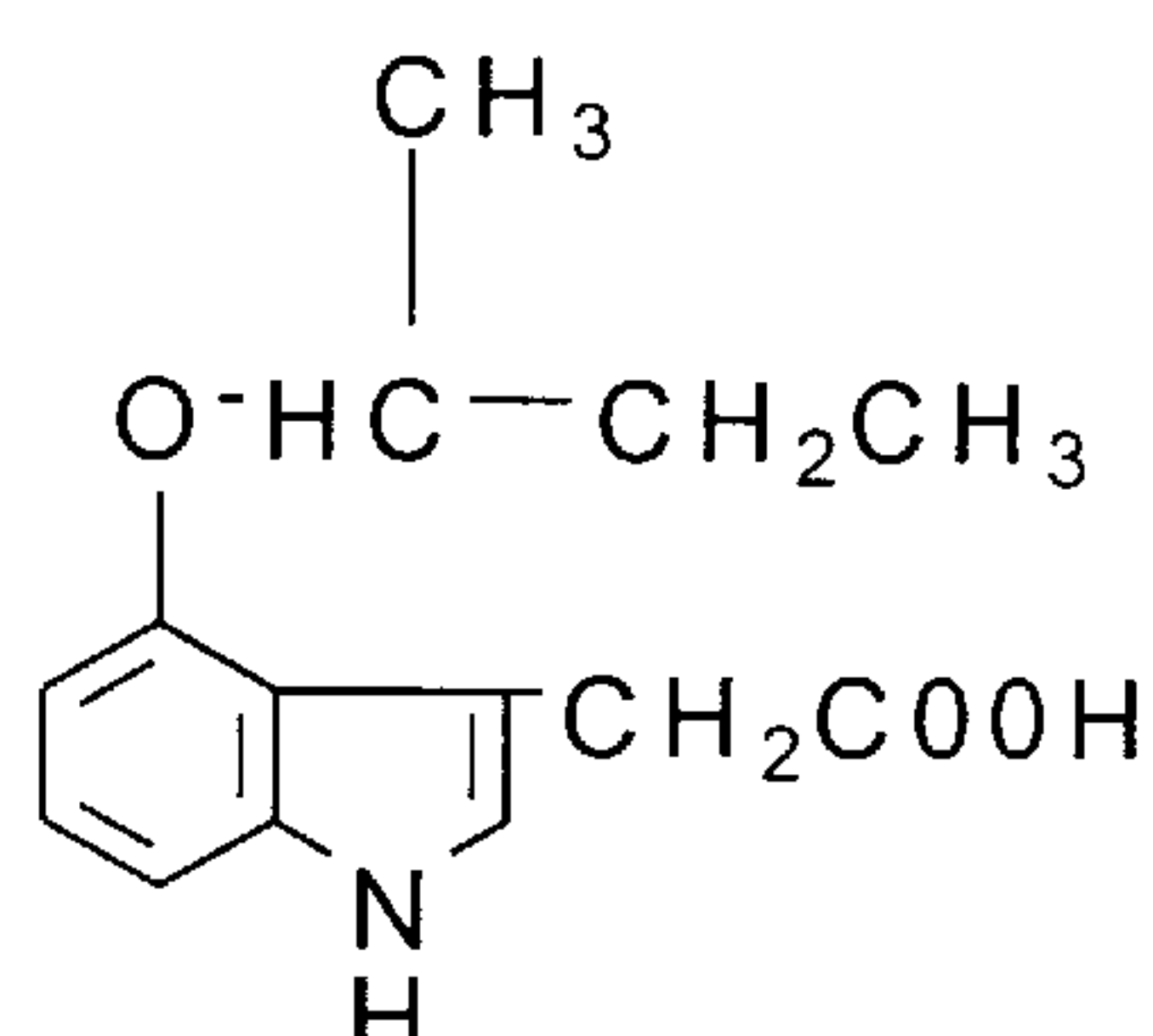
4-sec-butoxy-IAA
