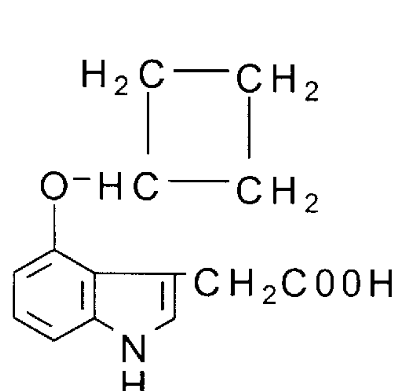
4-cyclobutoxy-IAA
