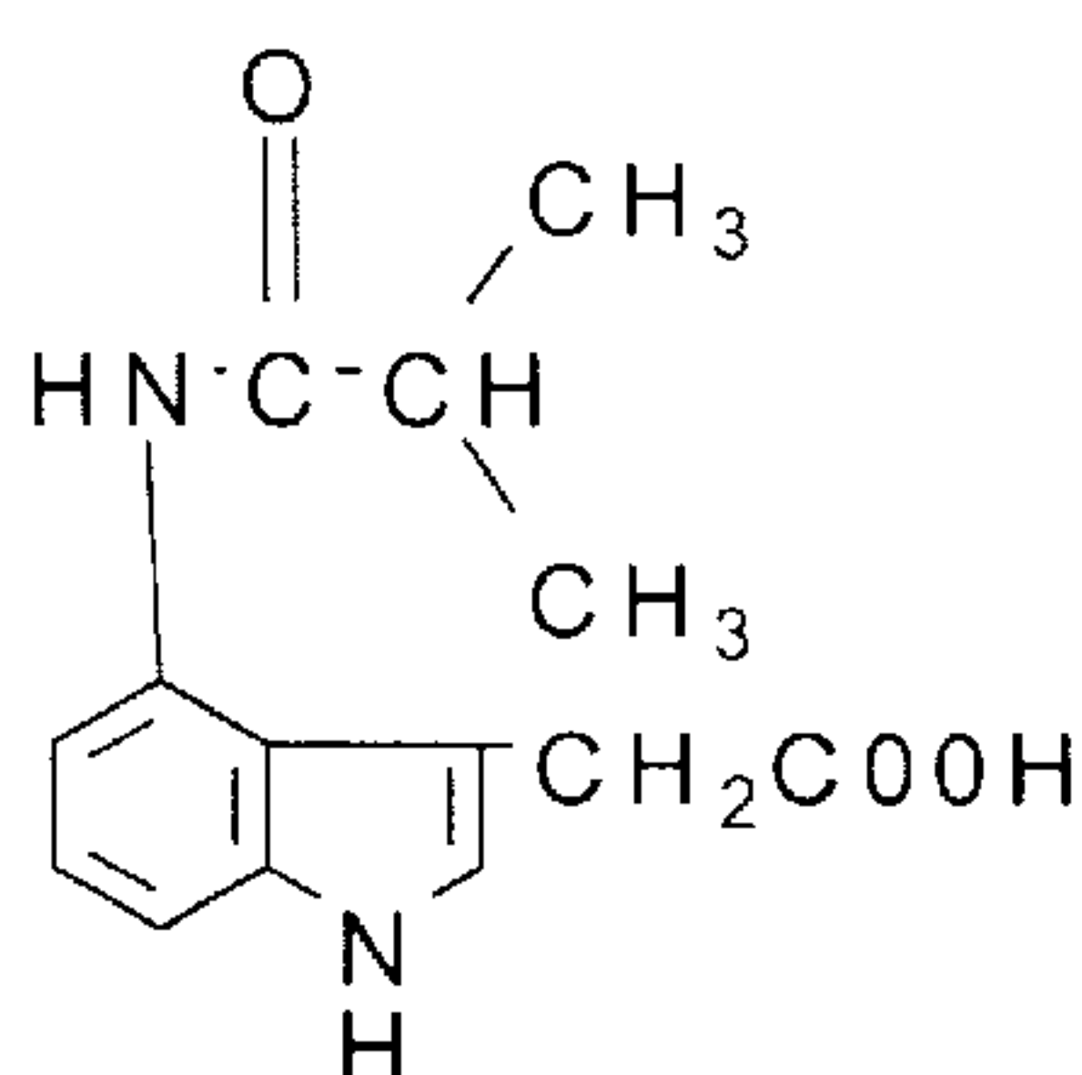
4-isobutyrylamido-IAA
