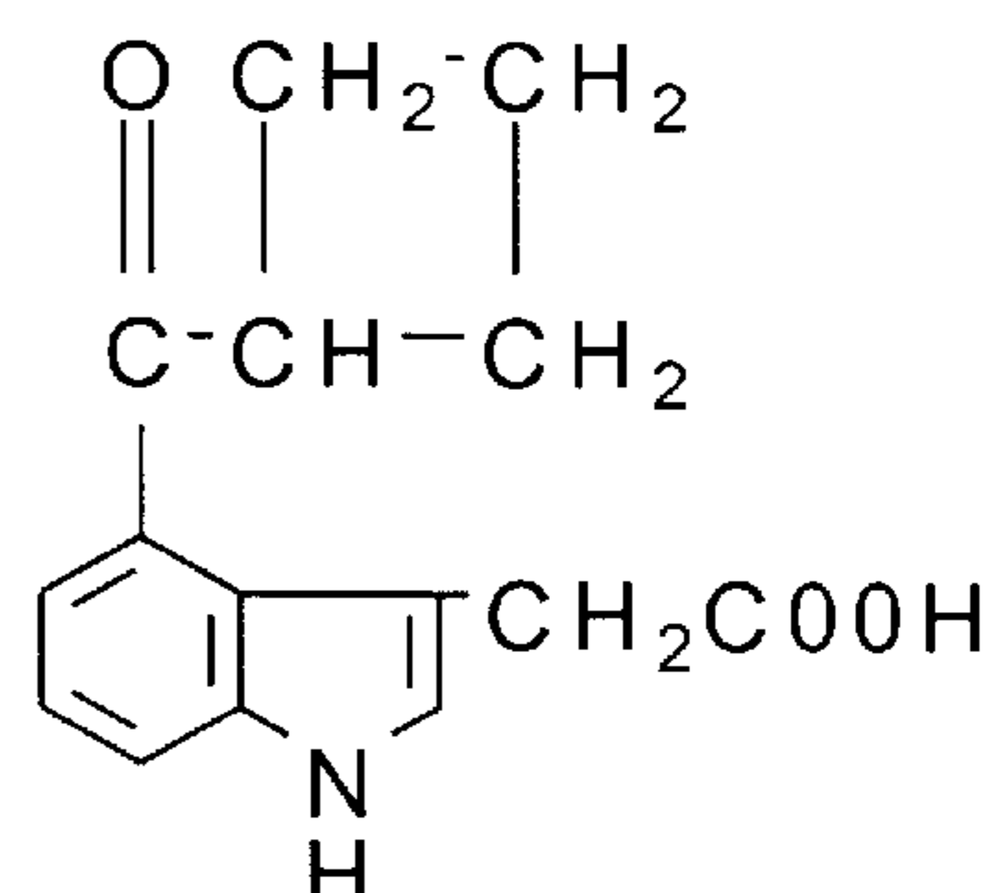
4-cyclovaleryl-IAA
