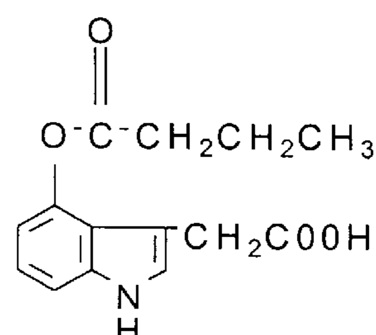
4-butyryloxy-IAA
