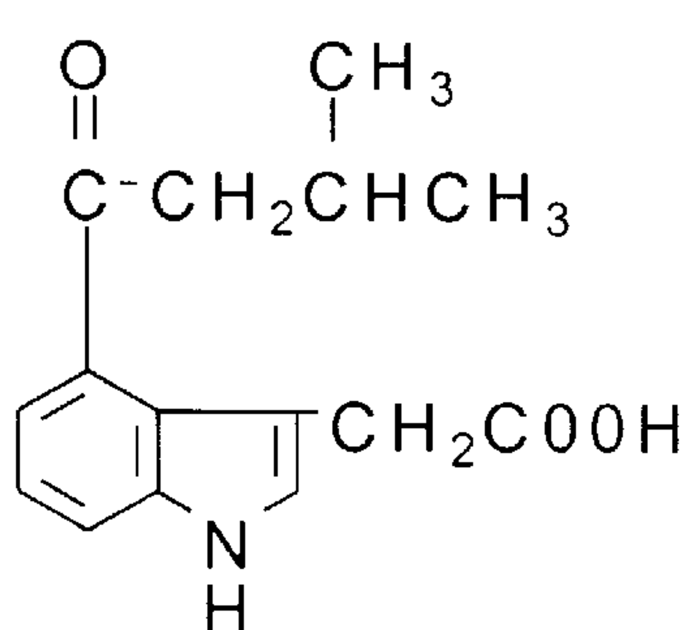
4-iso-valeryl-IAA
