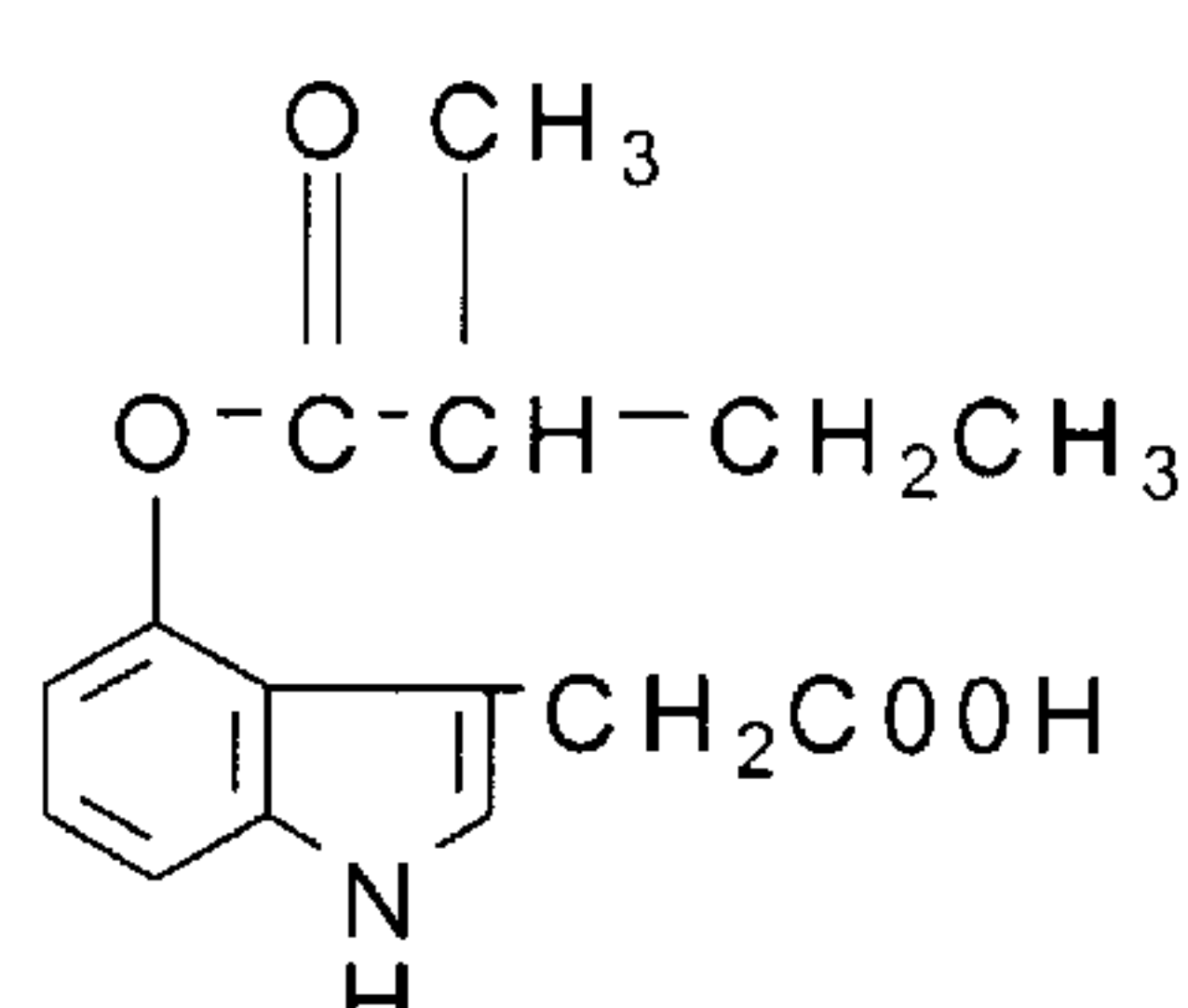
4-sec-valeryloxy-IAA
