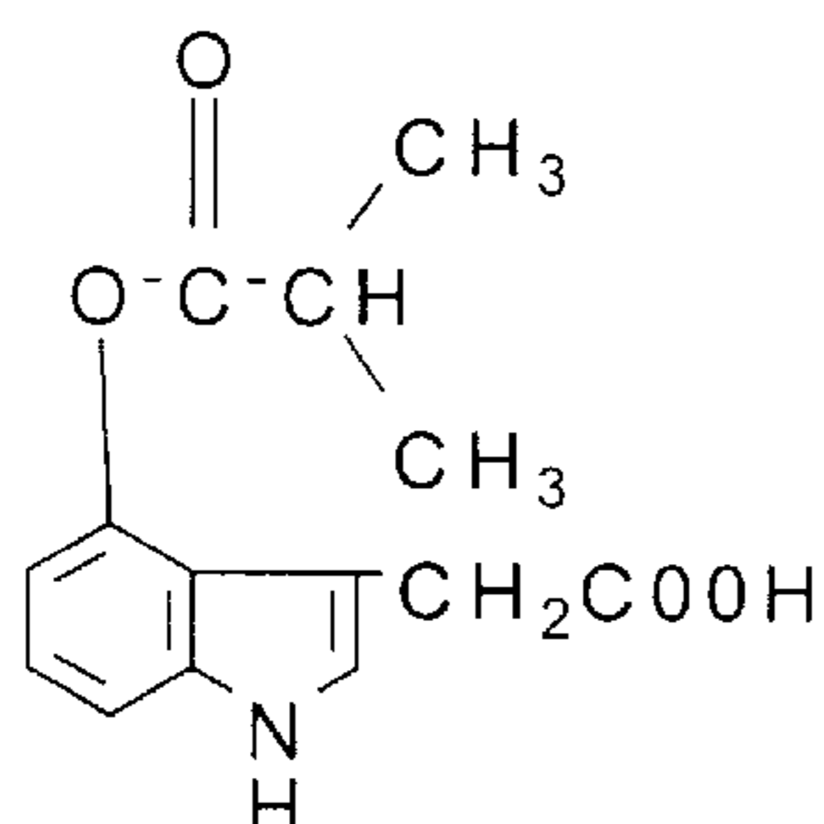
4-isobutyryloxy-IAA
