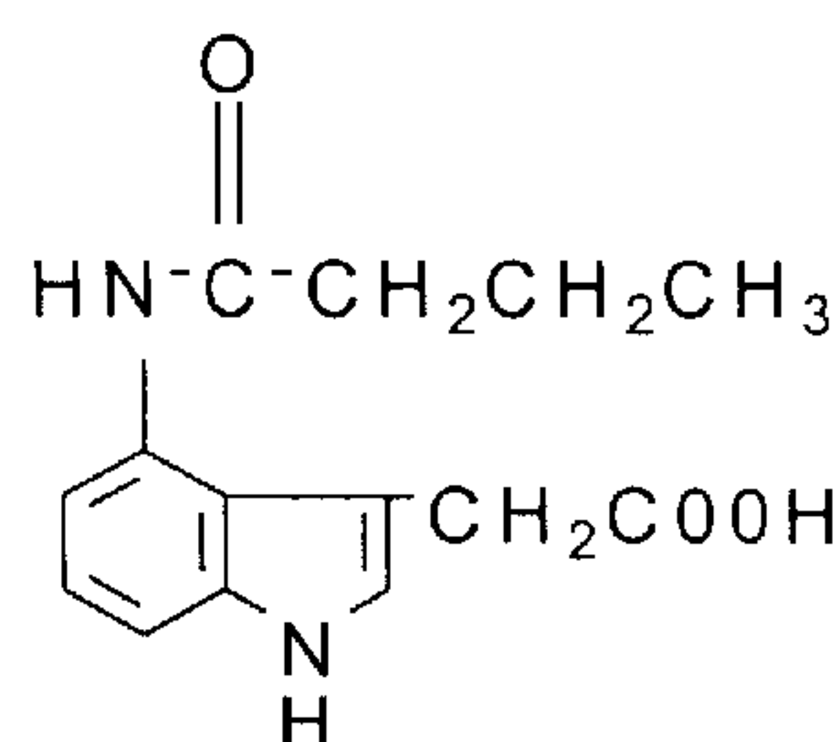
4-butyrylamido-IAA
