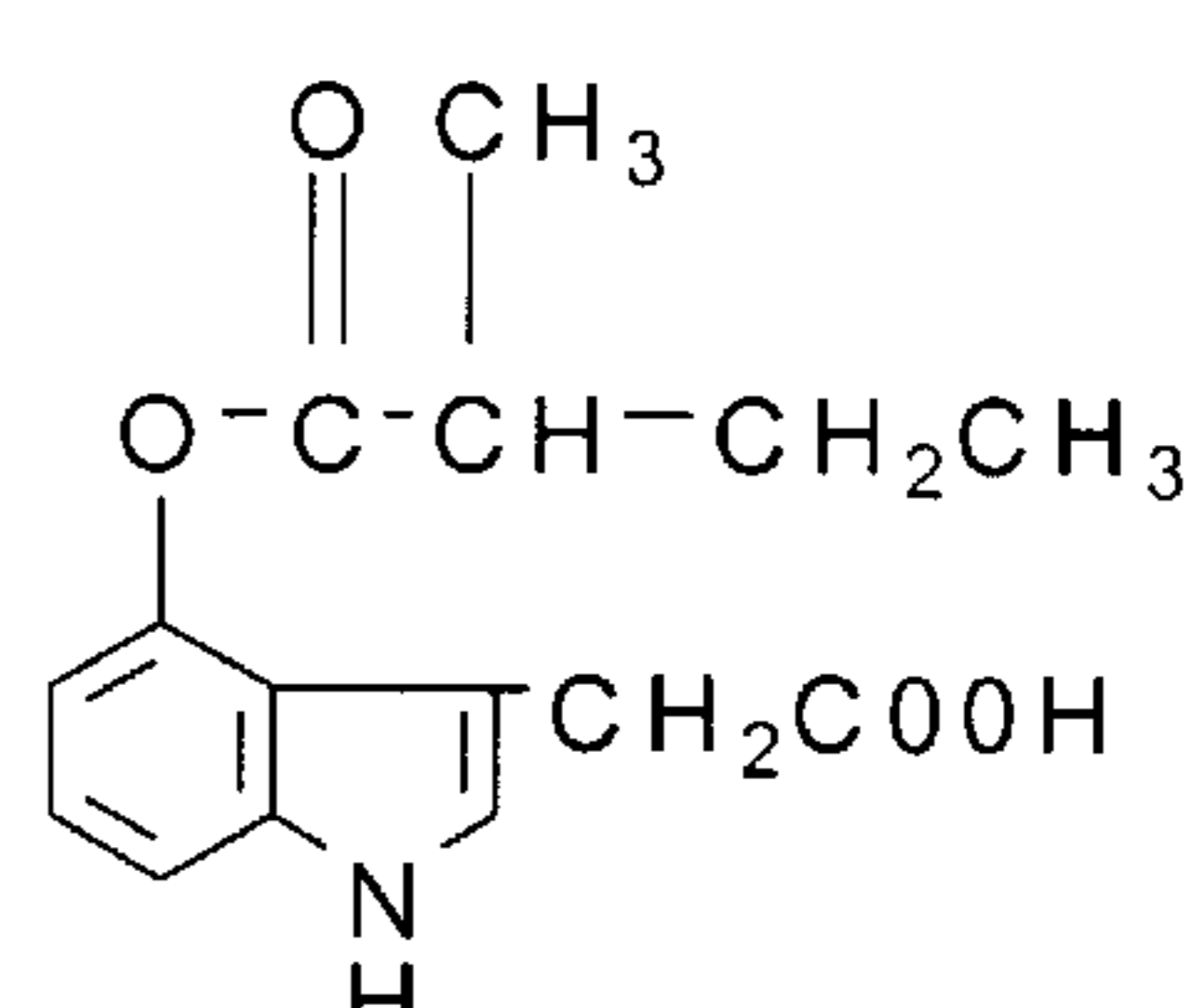
4-sec-valeryloxy-IAA
