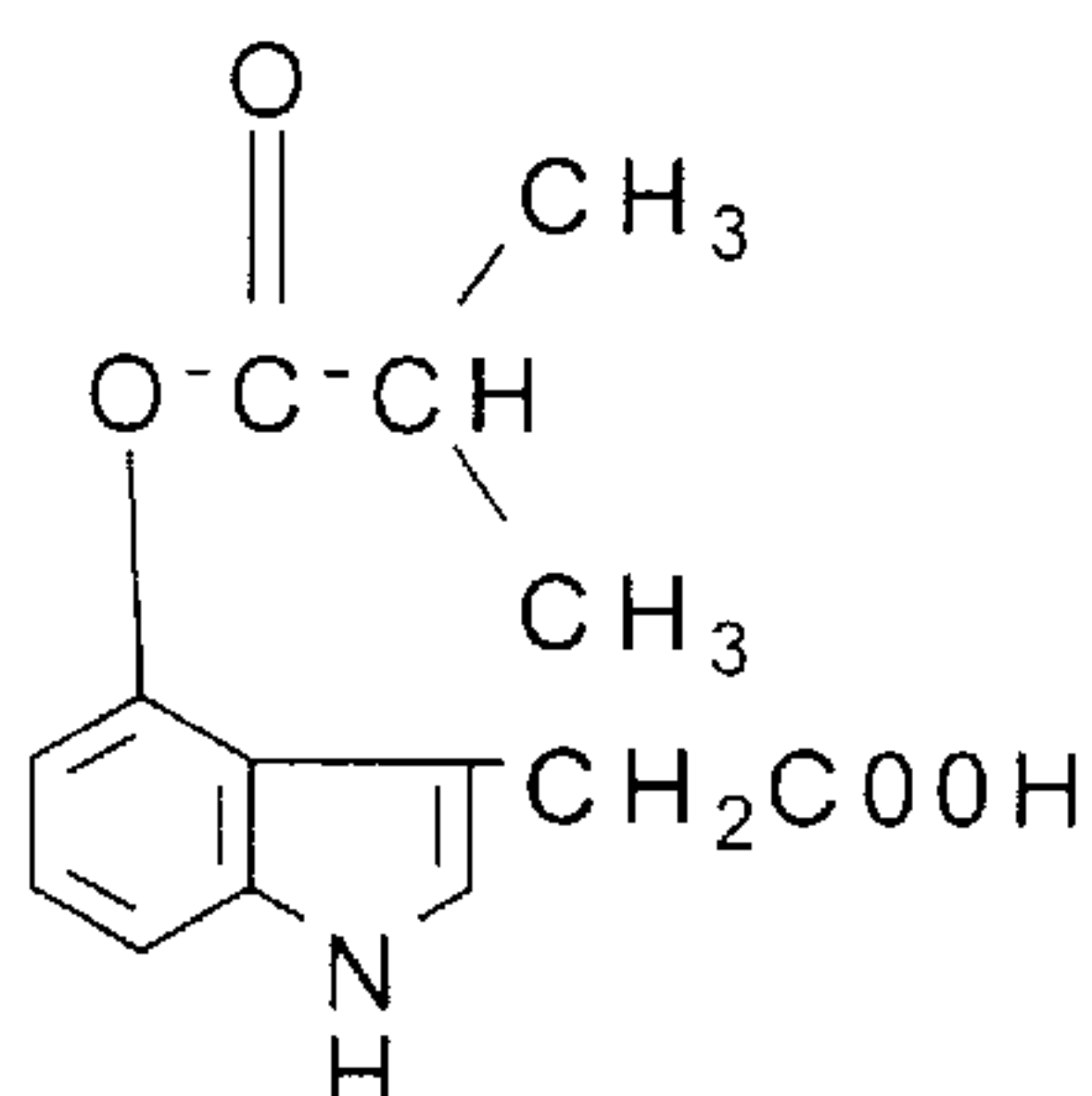
4-isobutyryloxy-IAA
