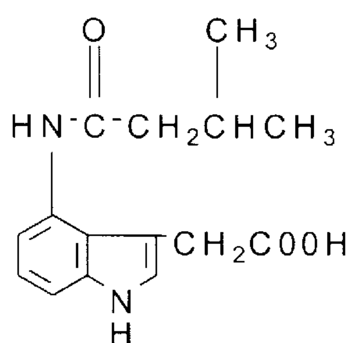
4-isovalerylamido-IAA
