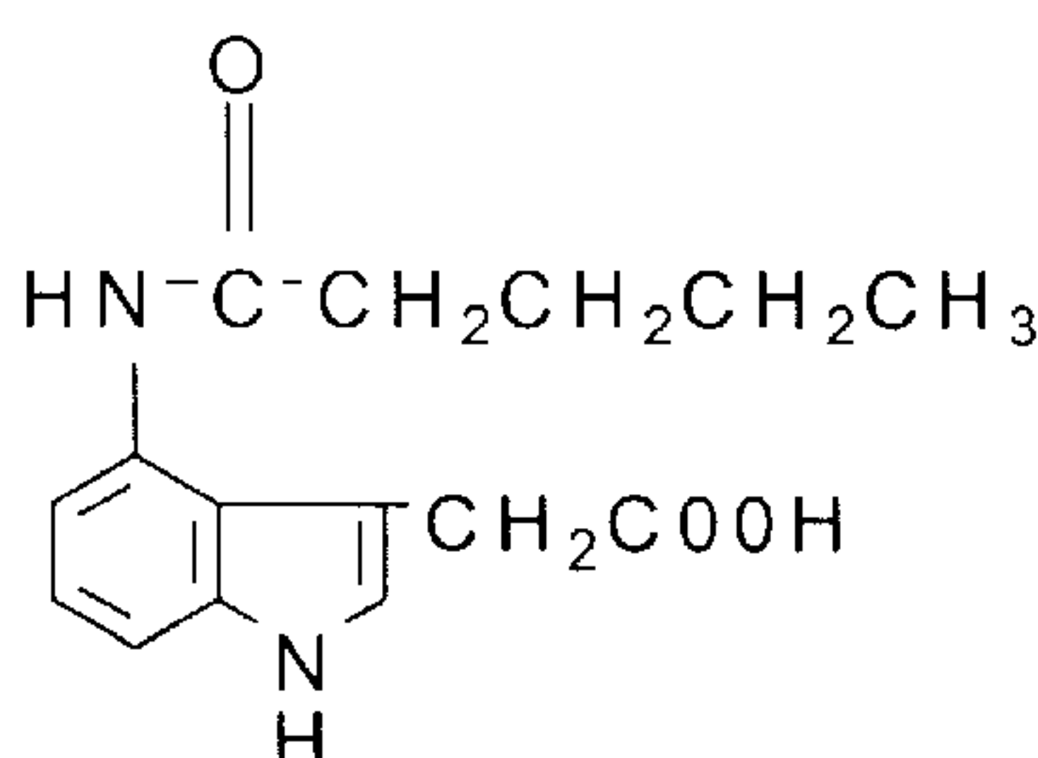
4-valerylamido-IAA
