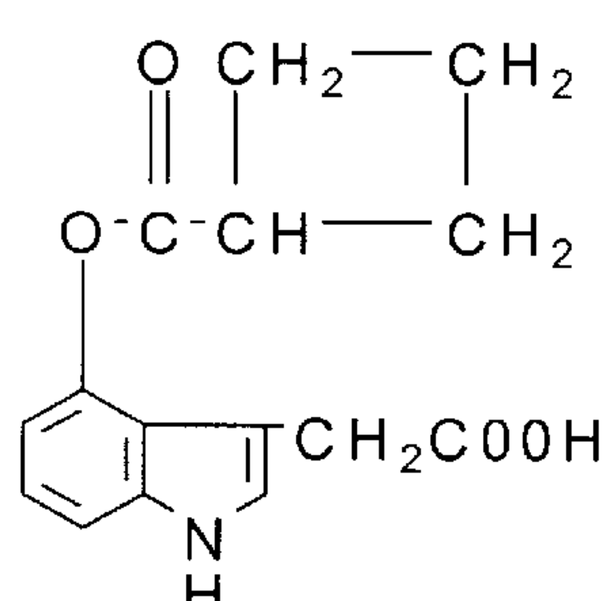
4-cyclovaleryloxy-IAA
