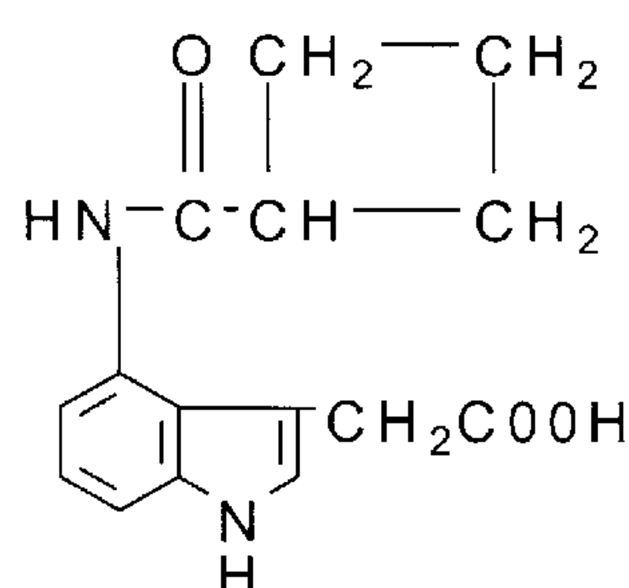
4-cyclovalerylamido-IAA
