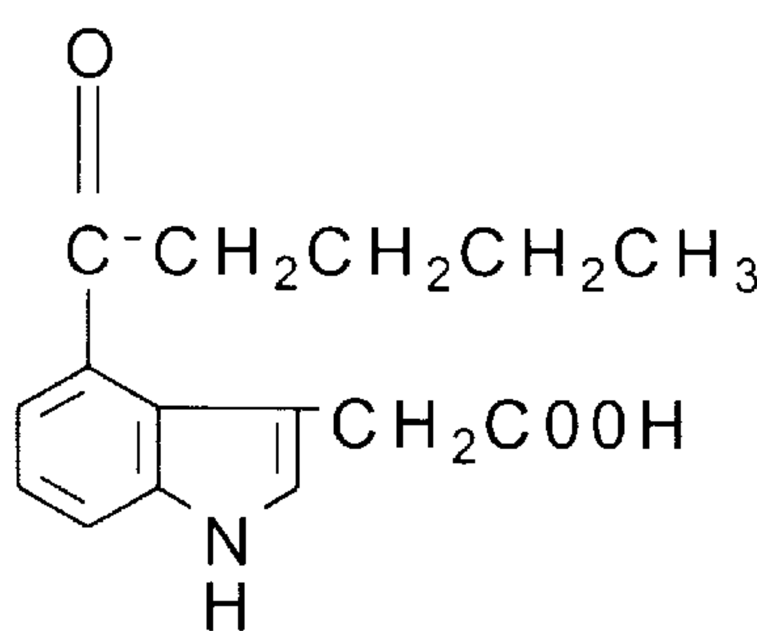
4-valeryl-IAA
