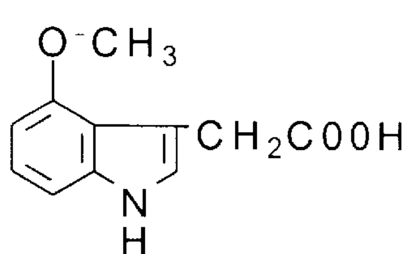
4-methoxy-IAA
