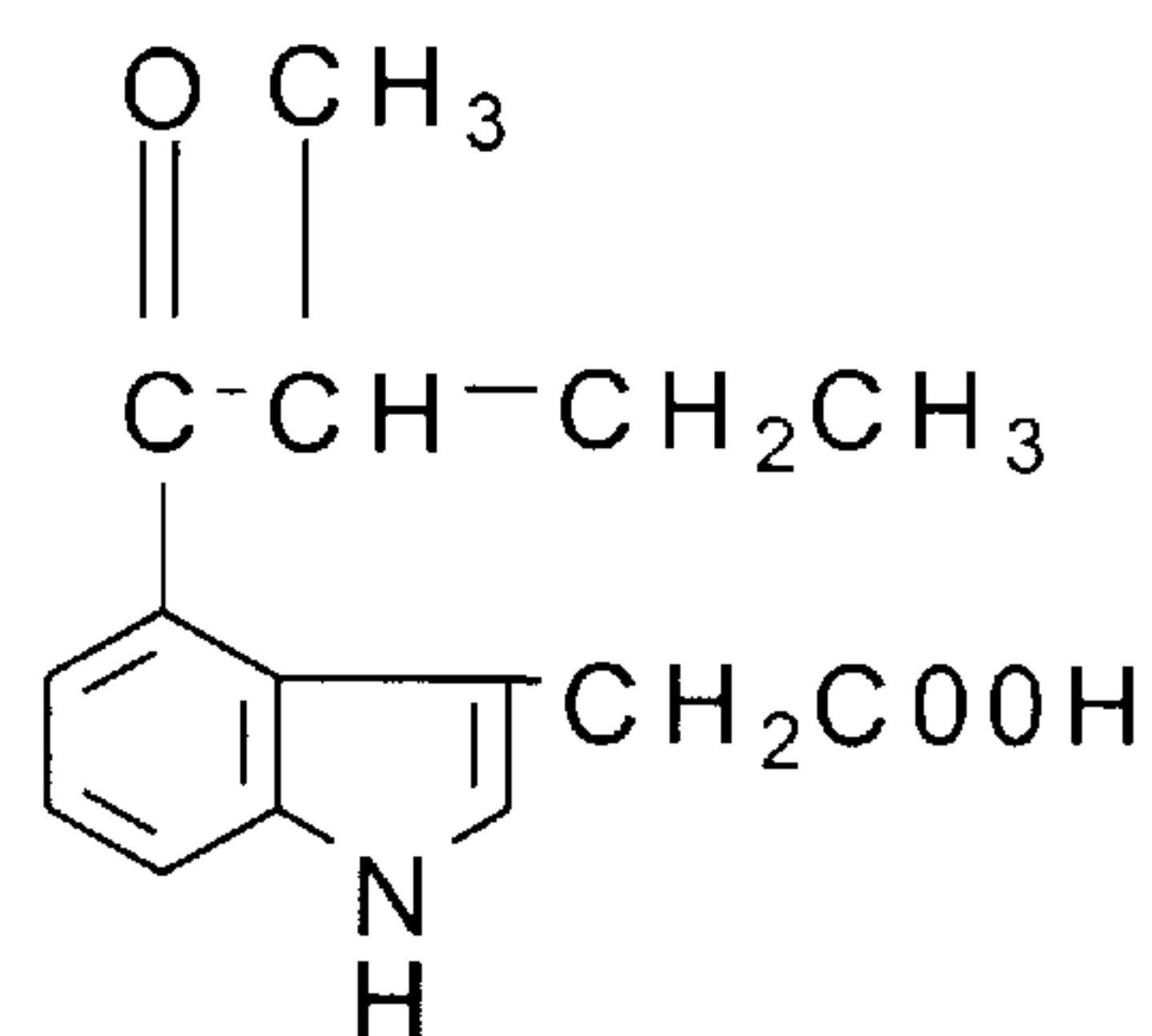
4-sec-valeryl-IAA
