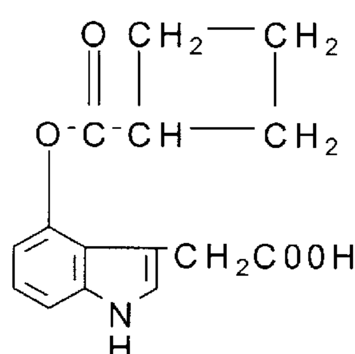
4-cyclovaleryloxy-IAA
