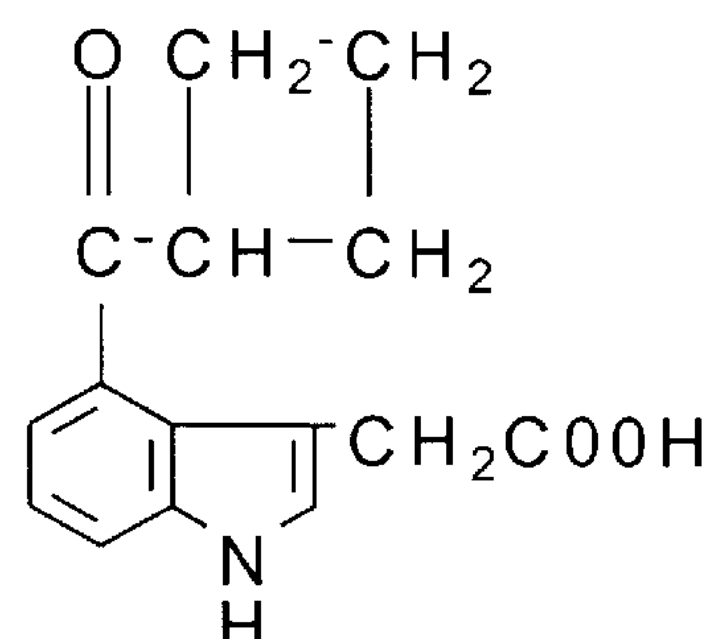
4-cyclovaleryl-IAA
