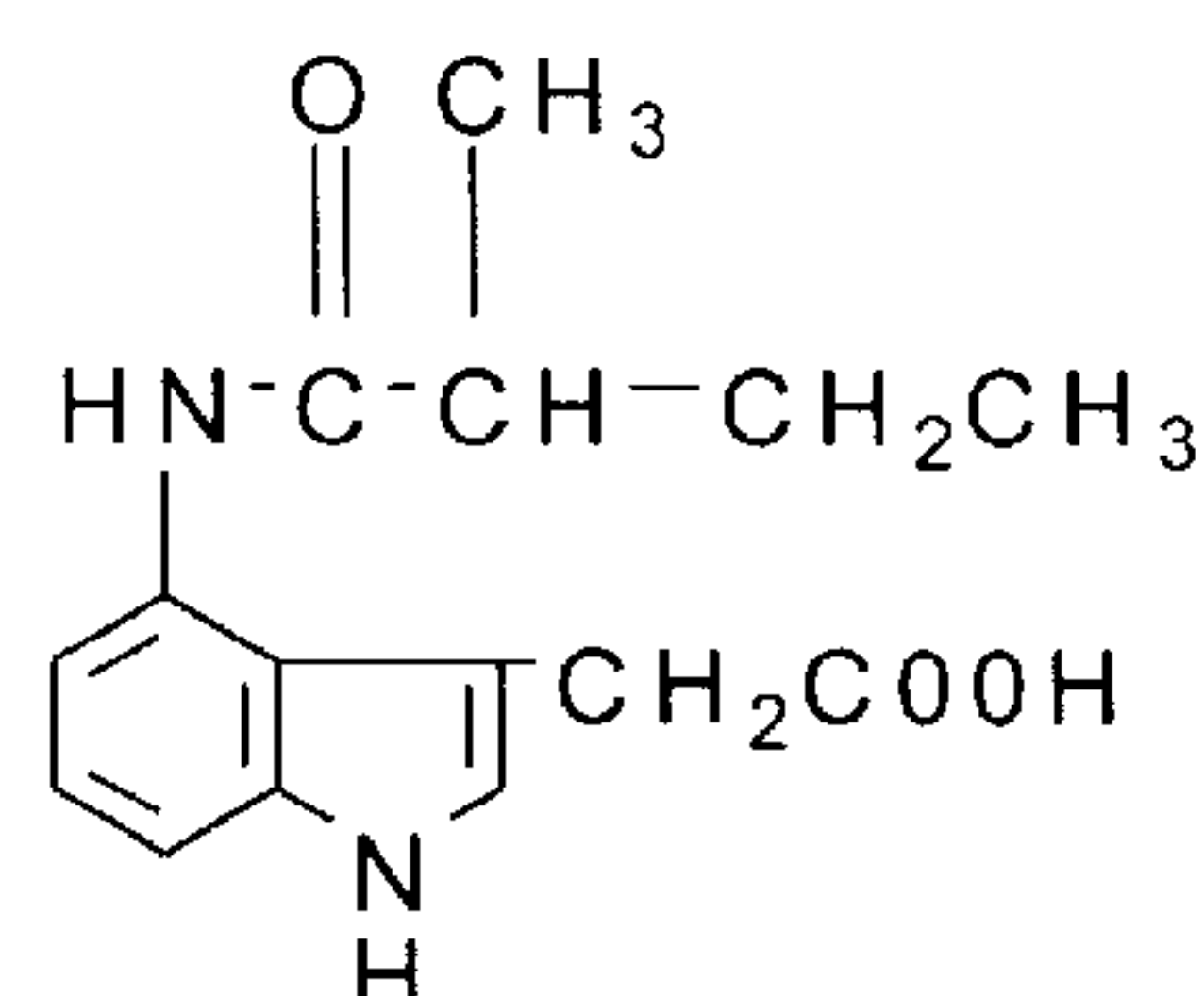
4-sec-valerylamido-IAA
