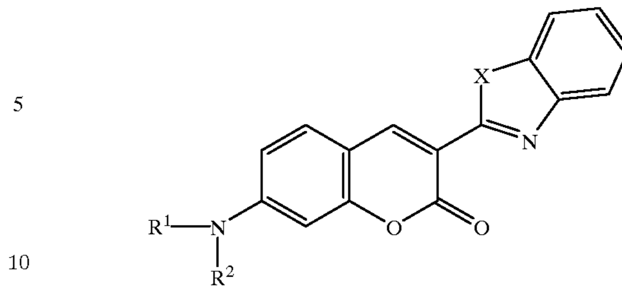
FD8 X = O, R 1 = R 2 = Alkyl
