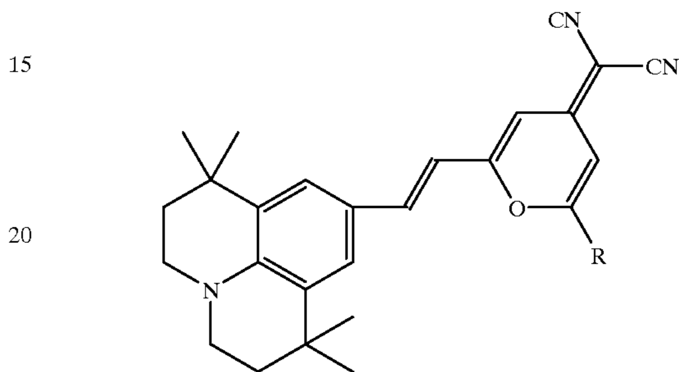
FD10 R = Ph
