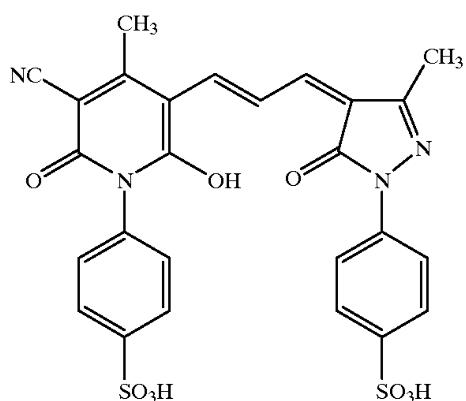
6-Hydroxy-4-methyl-5-(3-(3-methyl-5-oxo-1-(4-sulfophenyl)-1,5-dihydropyrazol-4-yliden)-propenyl)-2-oxo-1-(4-sulfophenyl)-1,2-dihydropyridin-3-carbonitrile (18)
