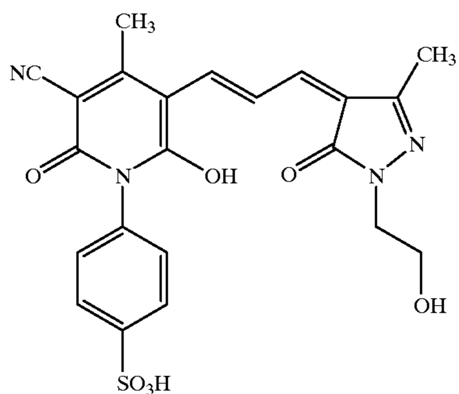
6-Hydroxy-5-(3-(1-(2-hydroxyethyl)-3-methyl-5-oxo-1,5-dihydro-pyrazol-4-yliden)-propenyl)-4-methyl-2-oxo-1-(4-sulfophenyl)-1,2-dihydro-pyridin-3-carbonitrile (17)
