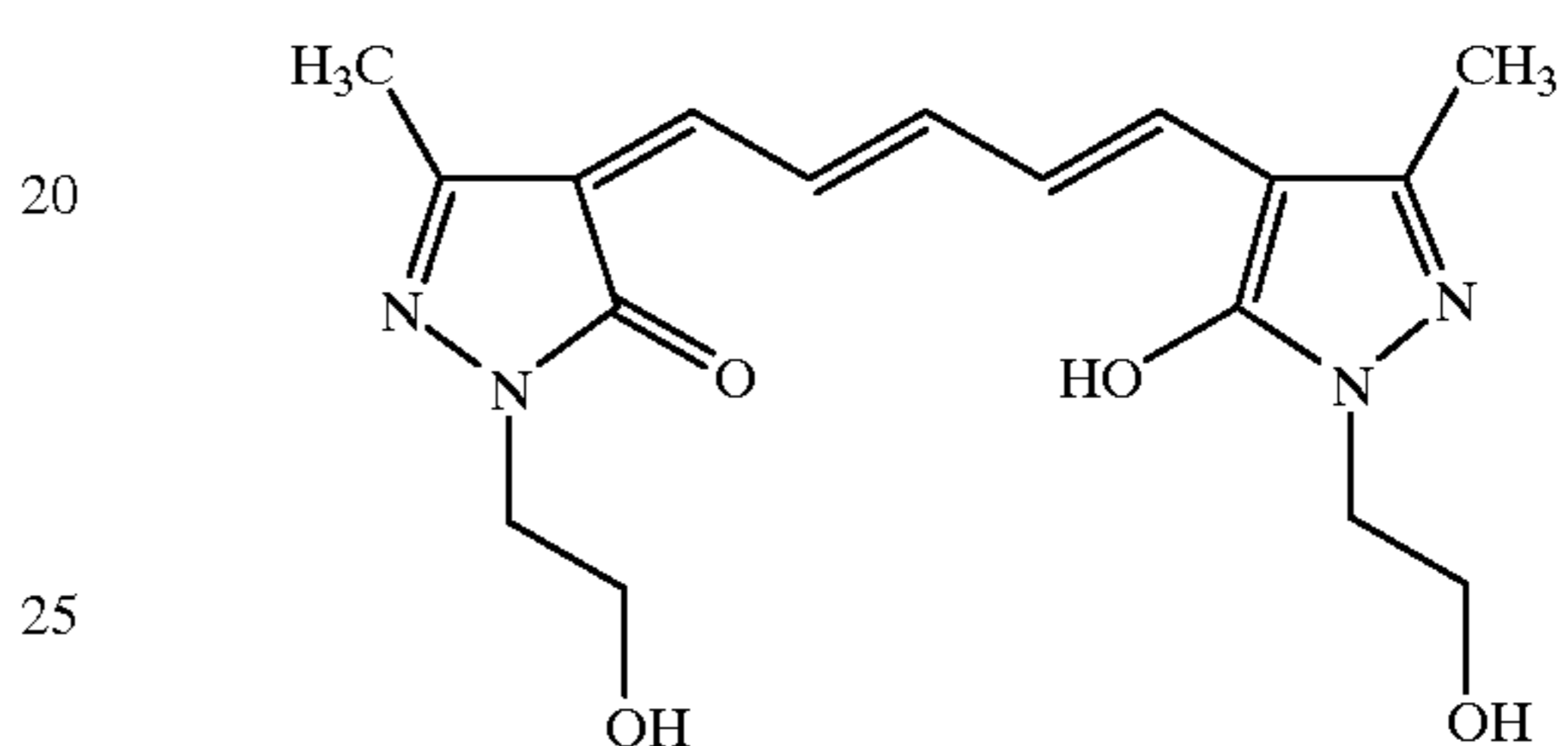
2-(2-Hydroxyethyl)-4-(5-(5-hydroxy-1-(2-hydroxyethyl)-3-methyl-1H-pyrazol-4-yl)-penta-2,4-dienylidene)-5-methyl-2,4-dihydropyrazol-3-one (13)
