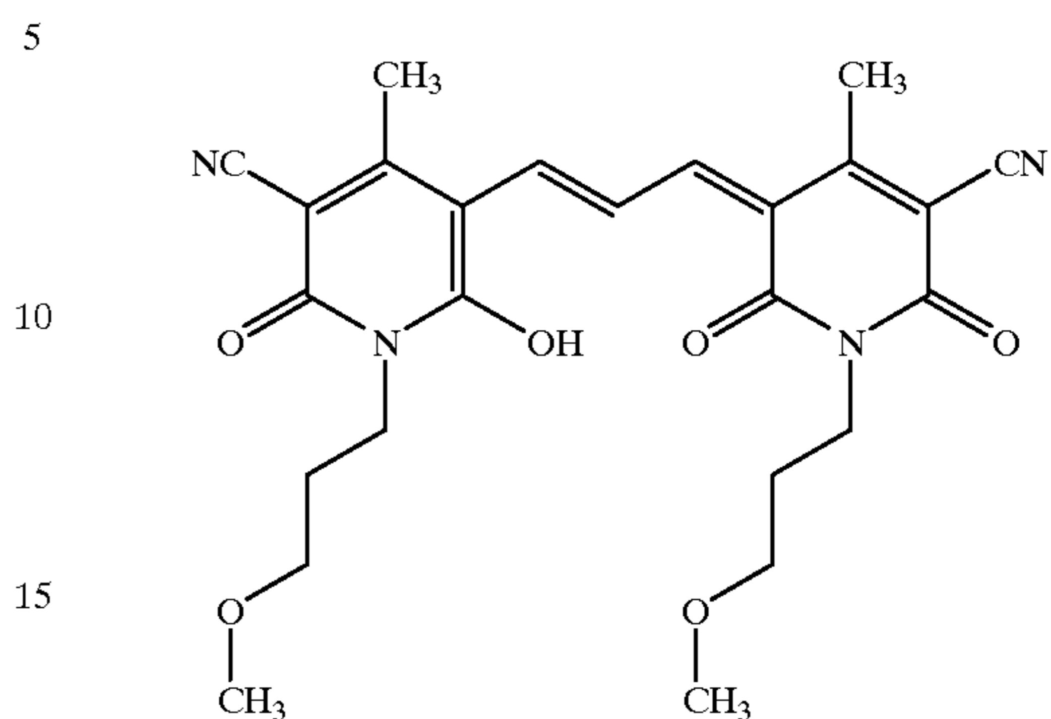
5-(3-(5-Cyano-1-ethyl-4-methyl-2,6-dioxo-1,6-dihydro-2H-pyridin-3-yliden)-propenyl)-1-ethyl-6-hydroxy-4-methyl-2-oxo-1,2-dihydropyridin-3-carbonitrile (24)
