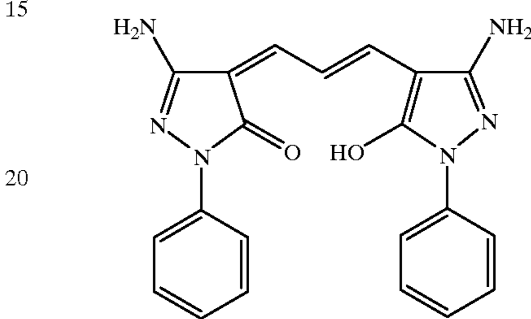
5-Amino-4-(3-(3-amino-5-hydroxy-1-phenyl-1H-pyrazol-4-yl)-allylidene)-2-phenyl-2,4-dihydropyrazol-3-one (5)
