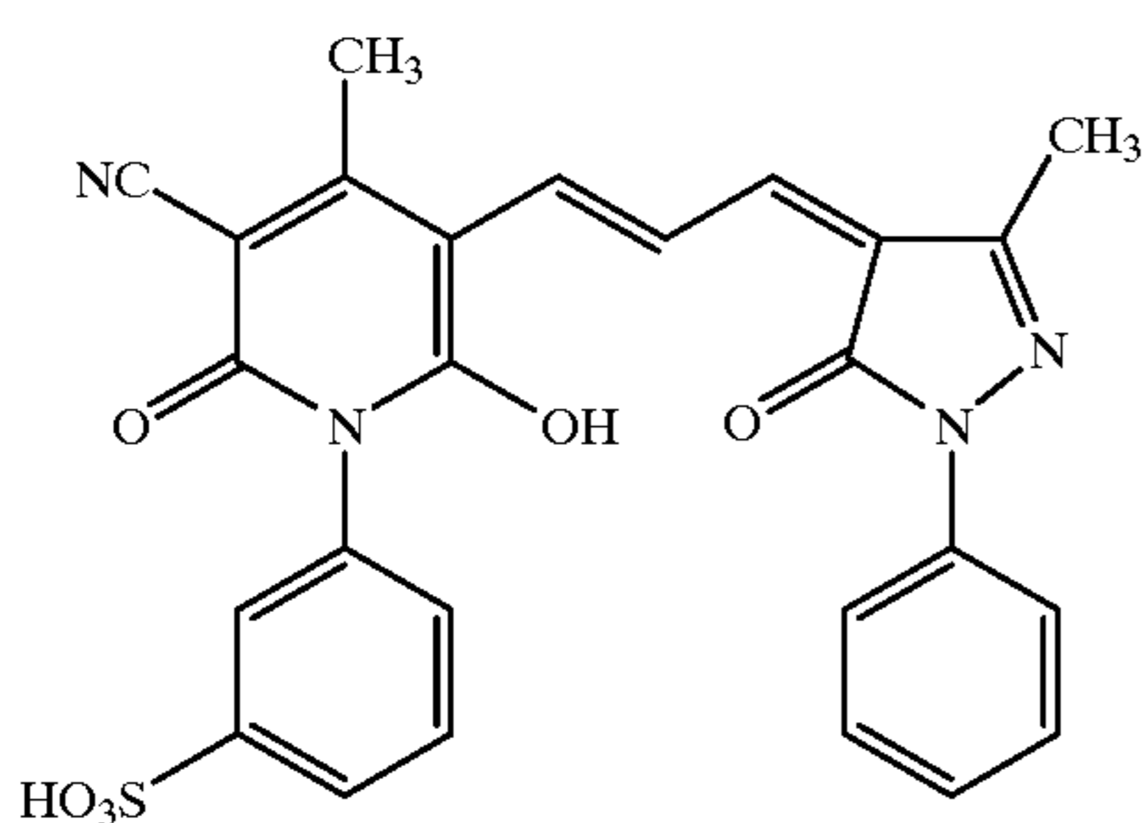
6-Hydroxy-4-methyl-5-(3-(3-methyl-5-oxo-1-(4-sulfophenyl)-1,5-dihydropyrazol-4-yliden)-propenyl)-2-oxo-1-(4-sulfophenyl)-1,2-dihydropyridin-3-carbonitrile (18)
