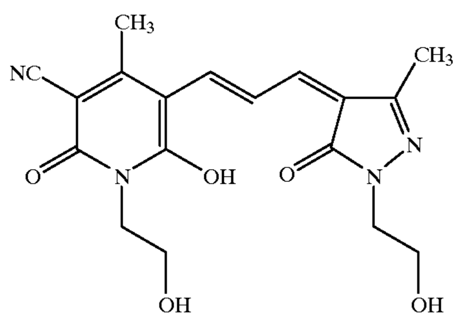
6-Hydroxy-1-(2-hydroxyethyl)-5-(3-(1-(2-hydroxyethyl)-3-methyl-5-oxo-1,5-dihydro-pyrazol-4-yliden)-propenyl)-4-methyl-2-oxo-1,2-dihydro-pyridin-3-carbonitrile (16)
