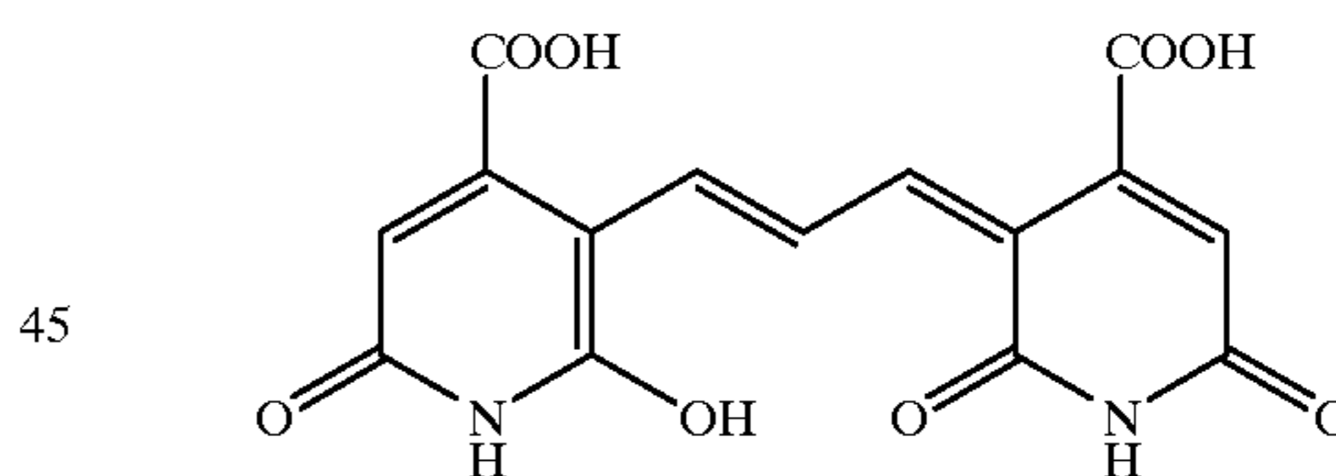
5-(3-(4-Carboxy-2,6-dioxo-1,6-dihydro-2H-pyridin-3-yliden)-propenyl)-6-hydroxy-2-oxo-1,2-dihydropyridin-4-carboxylic acid (22)
