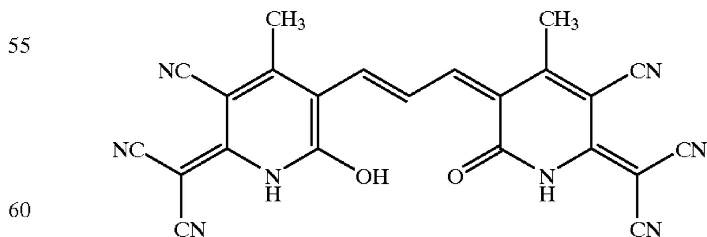
2-(3-Cyano-5-(3-(5-cyano-6-dicyanomethylen-4-methyl-2-oxo-1,6-dihydro-2H-pyridin-3-yliden)-propenyl)-6-hydroxy-4-methyl-1H-pyridin-2-yliden)-malononitrile (23)
