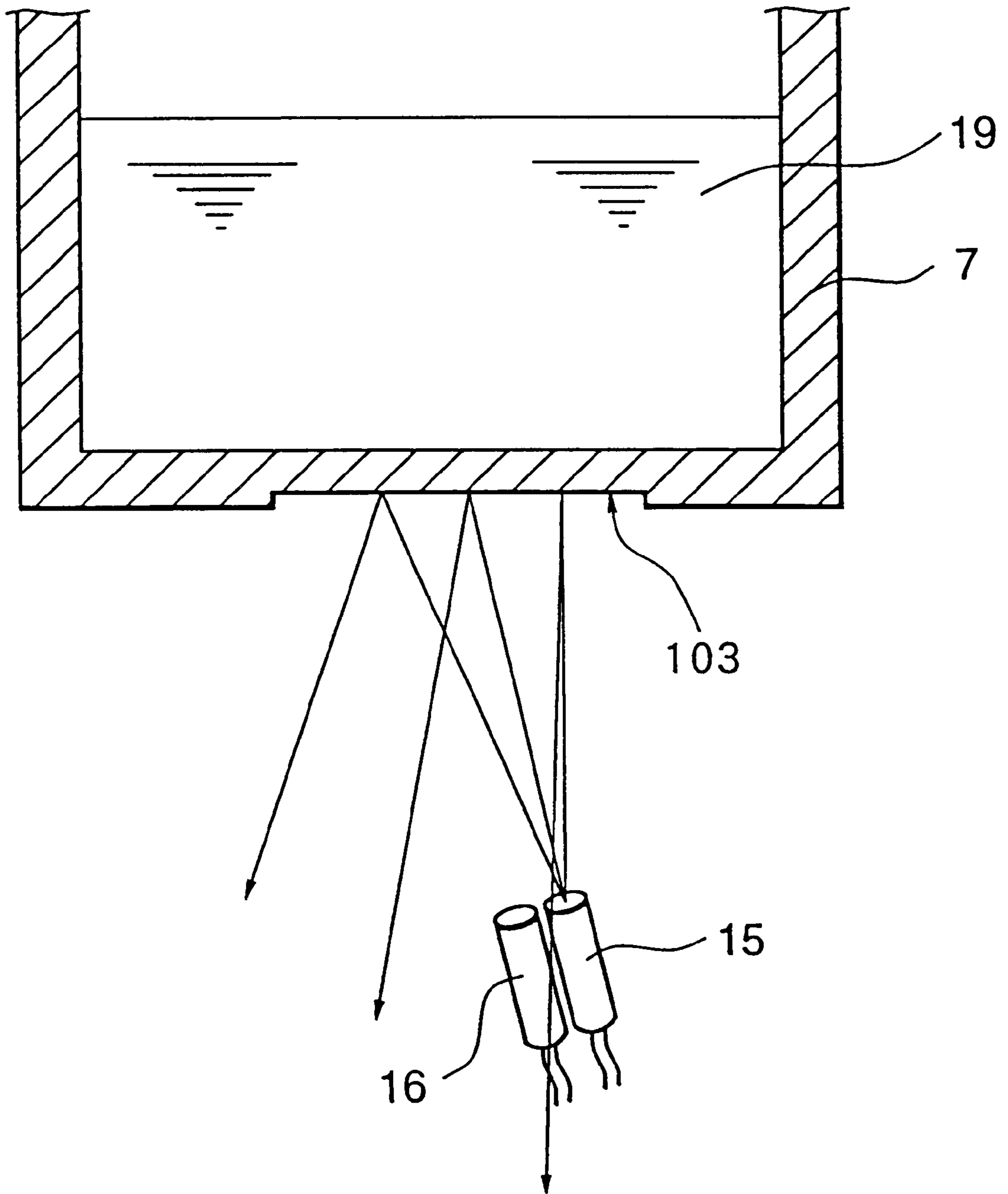
FIG. 10C PRIOR ART
