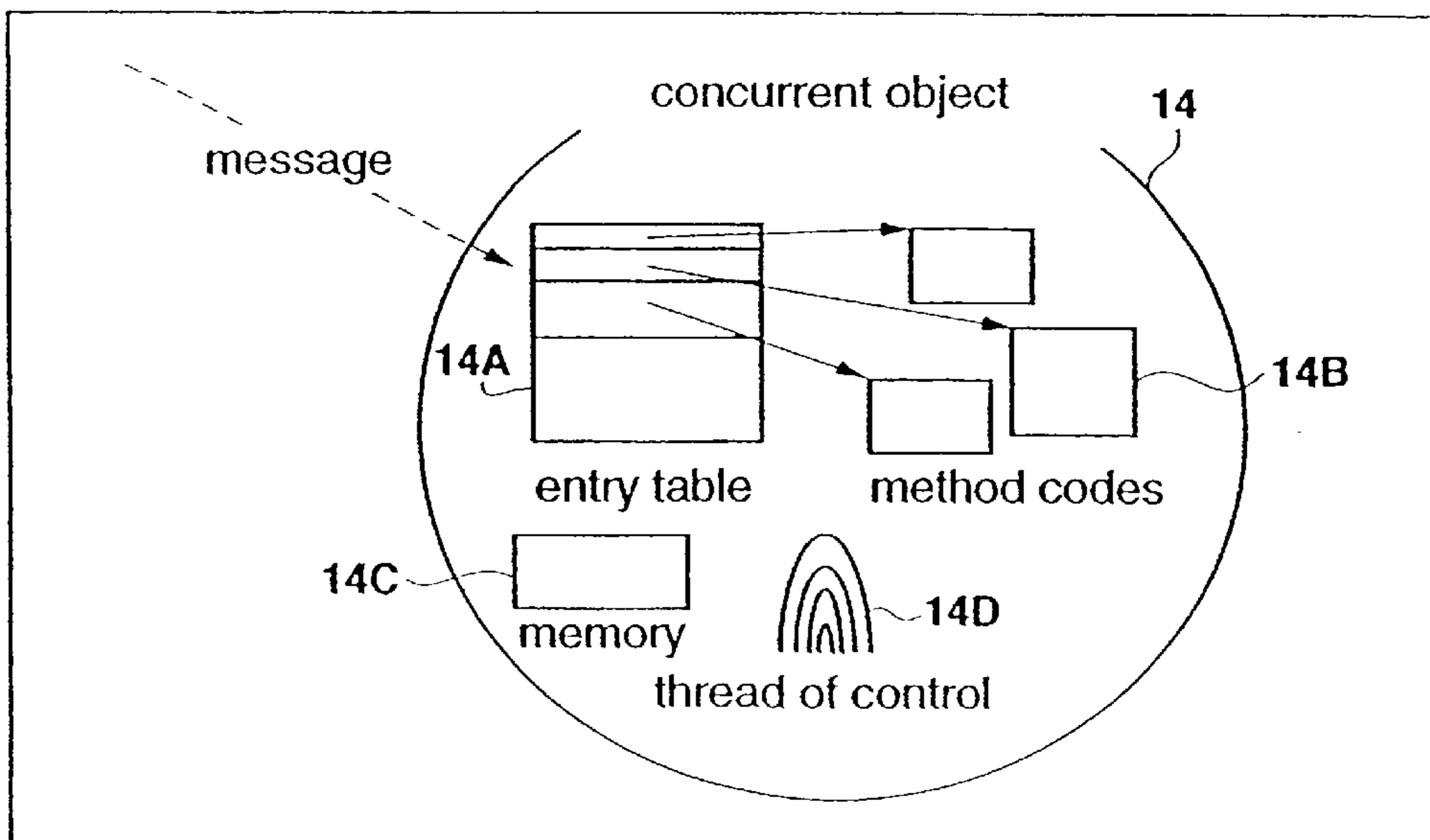
concurrent object structure
