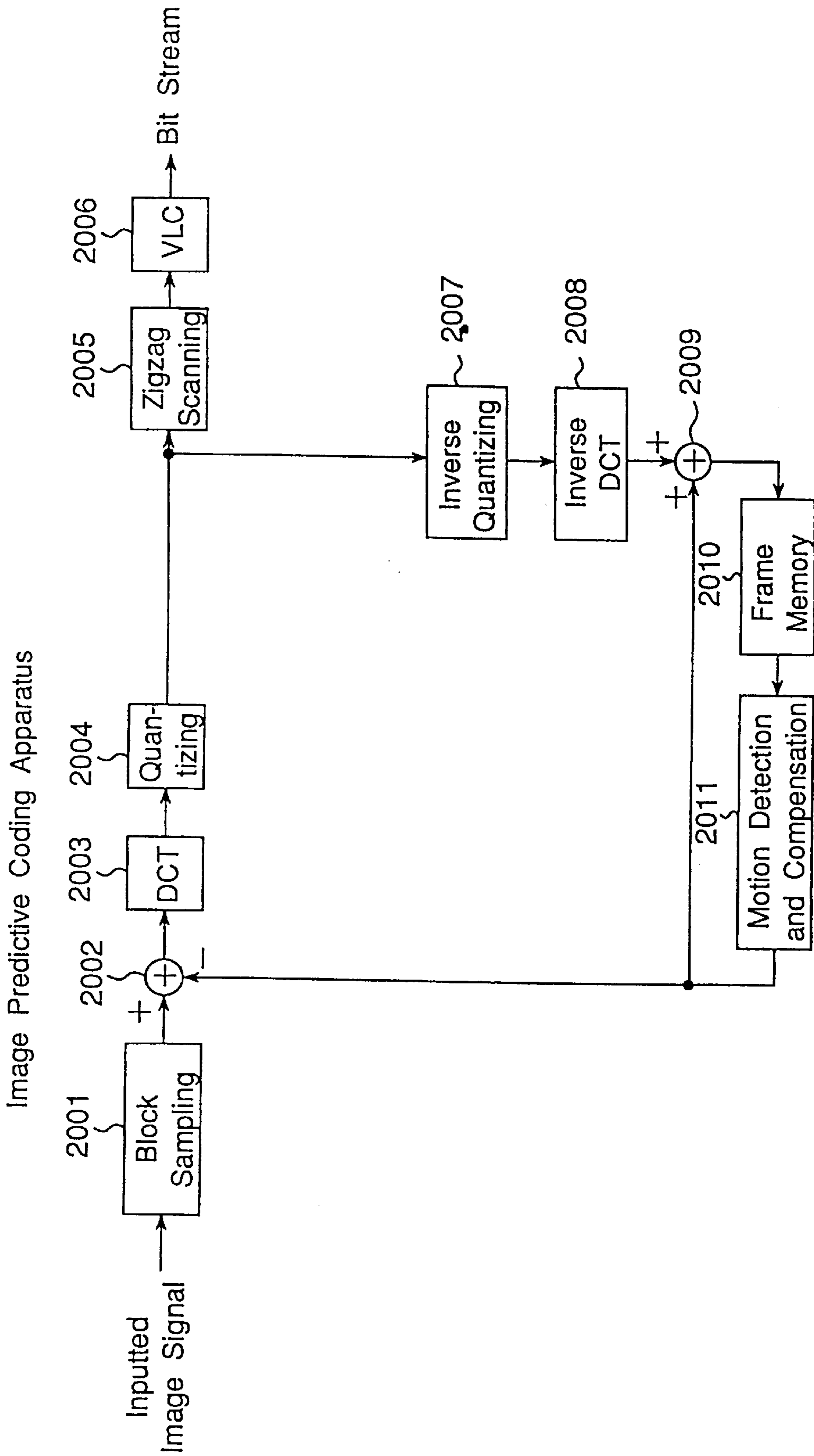
Fig.22 PRIOR ART
