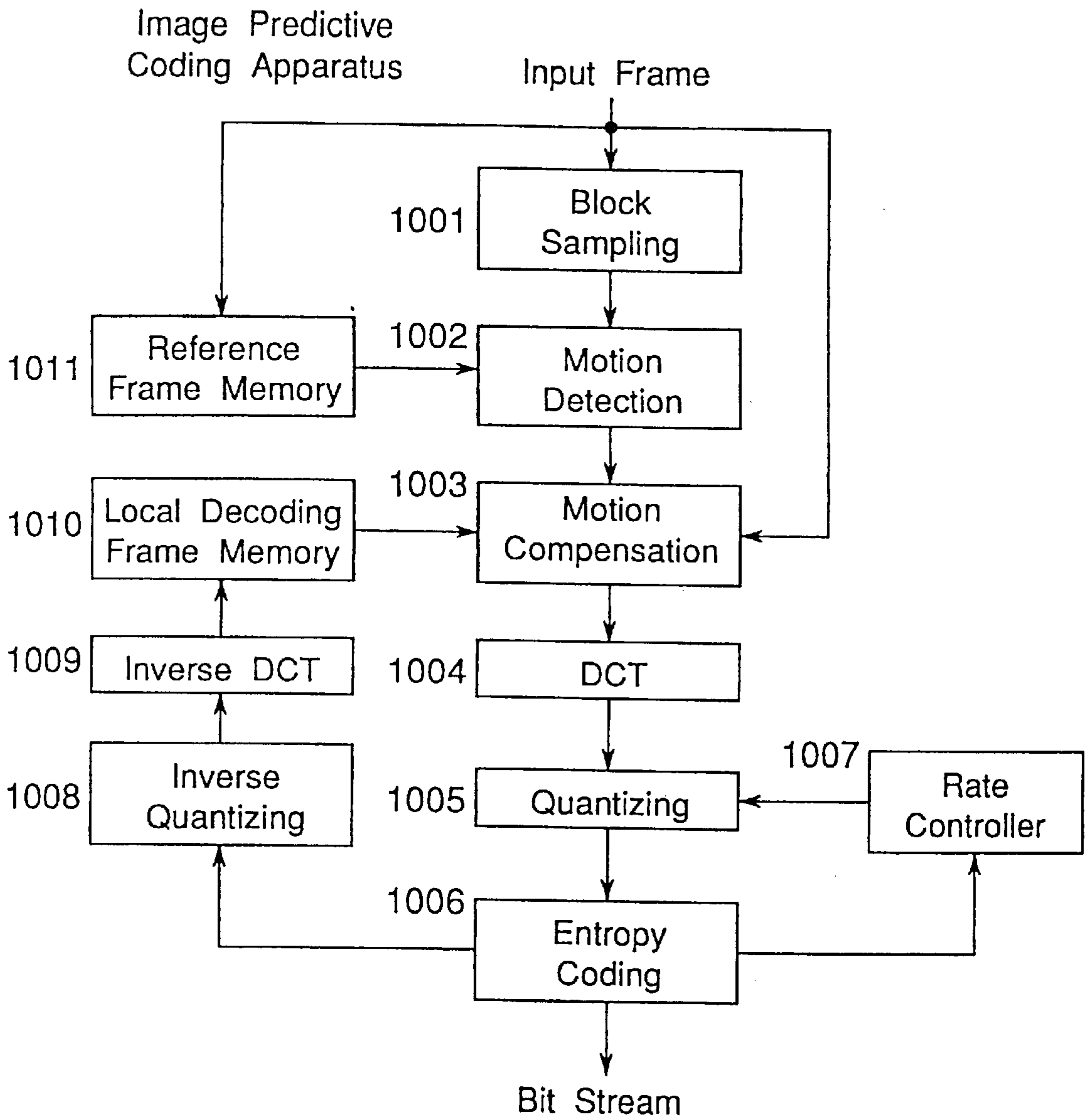
Fig.14 PRIOR ART
