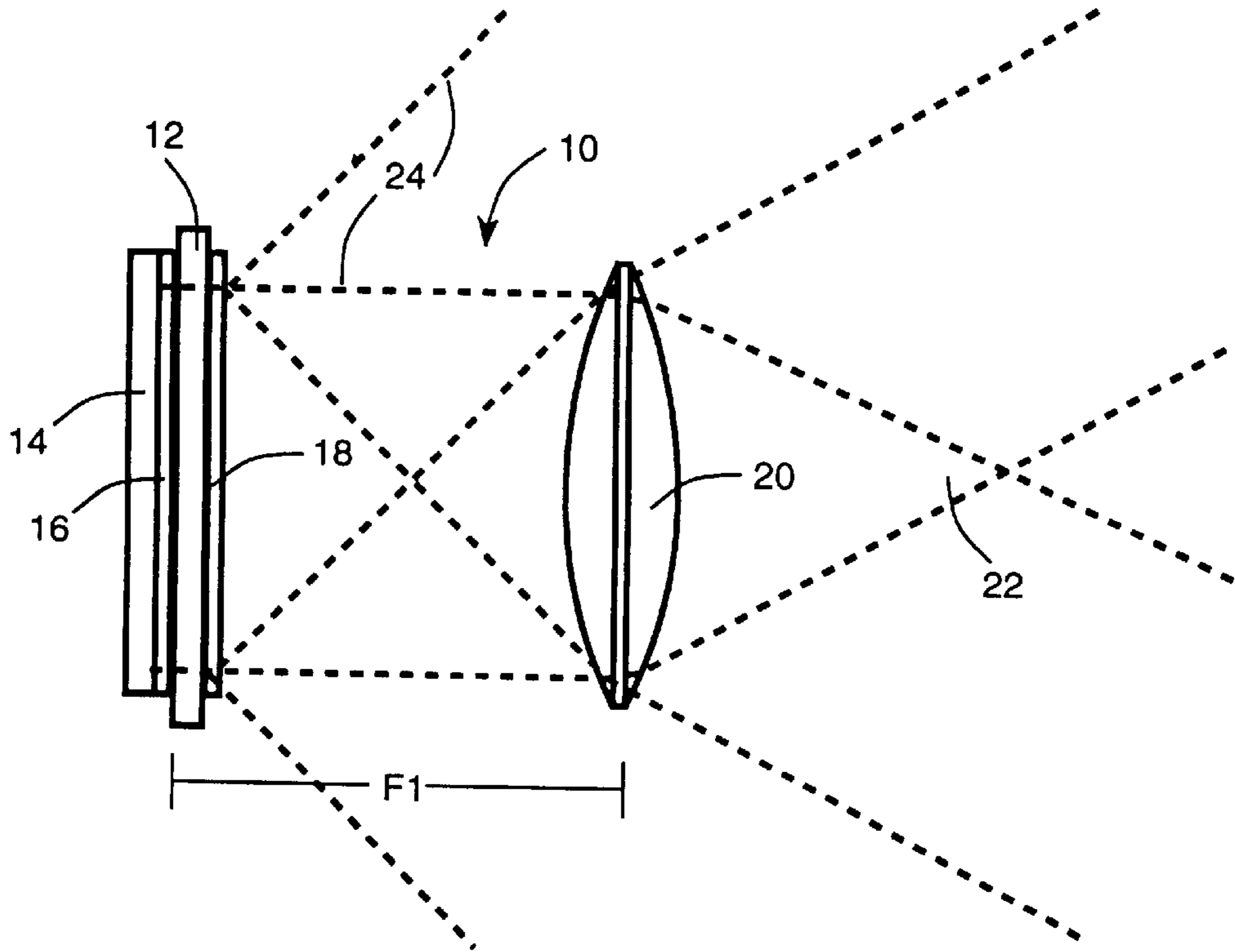
Figure 1 (Prior Art)
