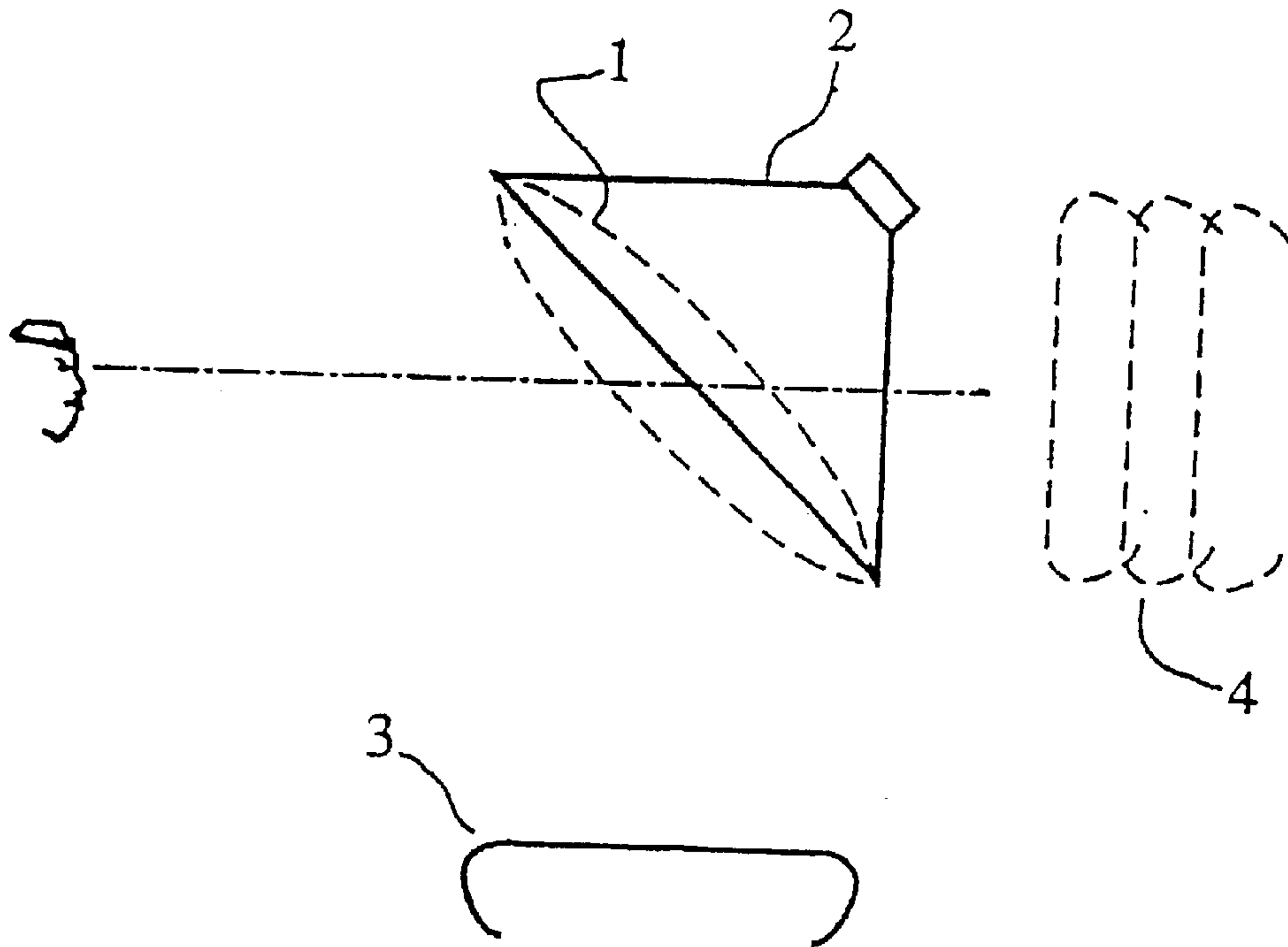
FIG. 1 (PRIOR ART)
