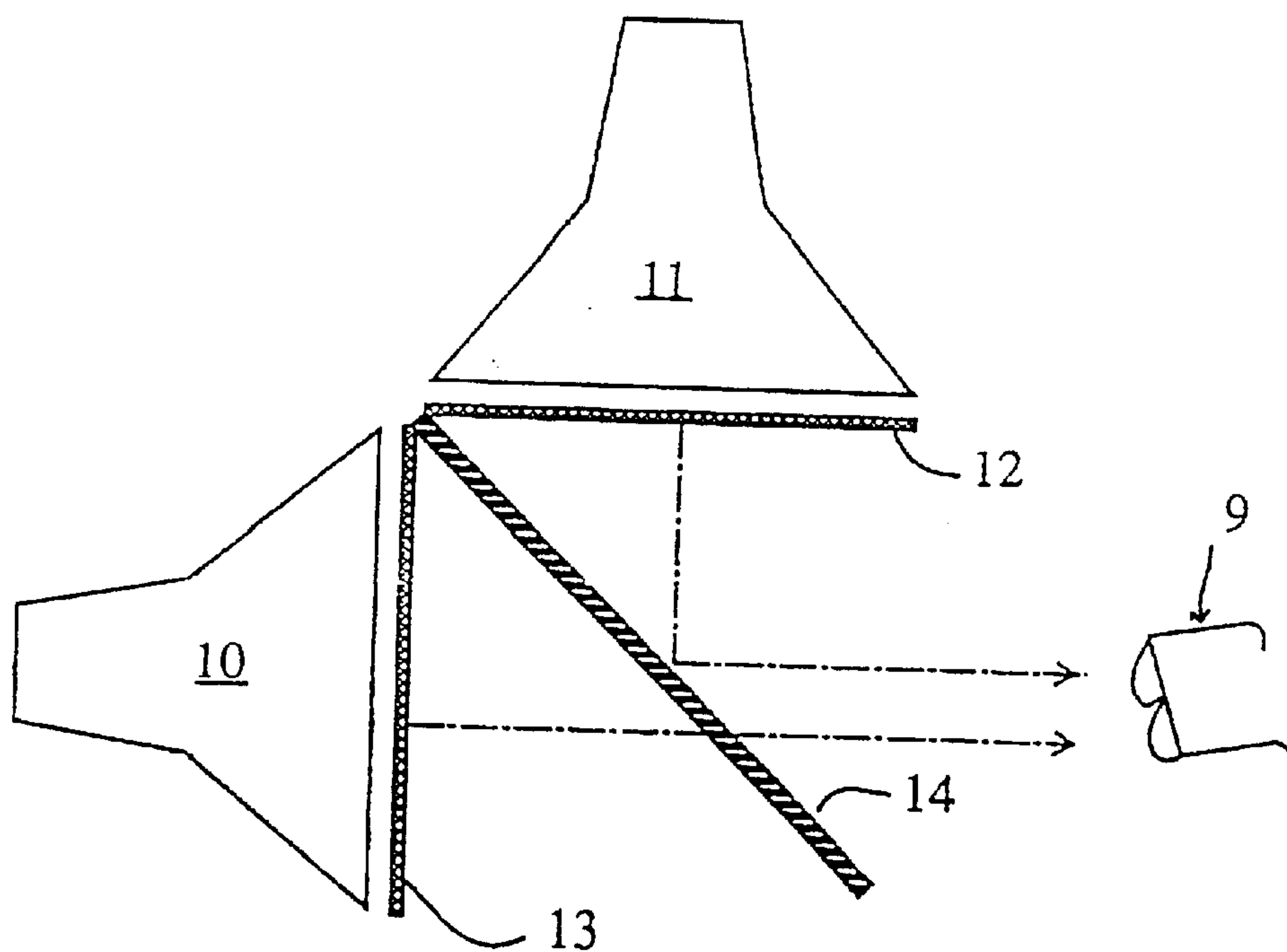
FIG. 3 (PRIOR ART)
