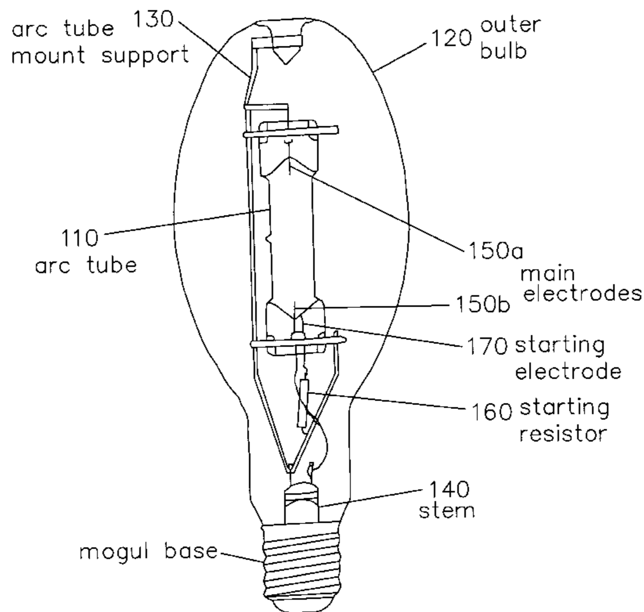
High-pressure mercury-vapor lamp
