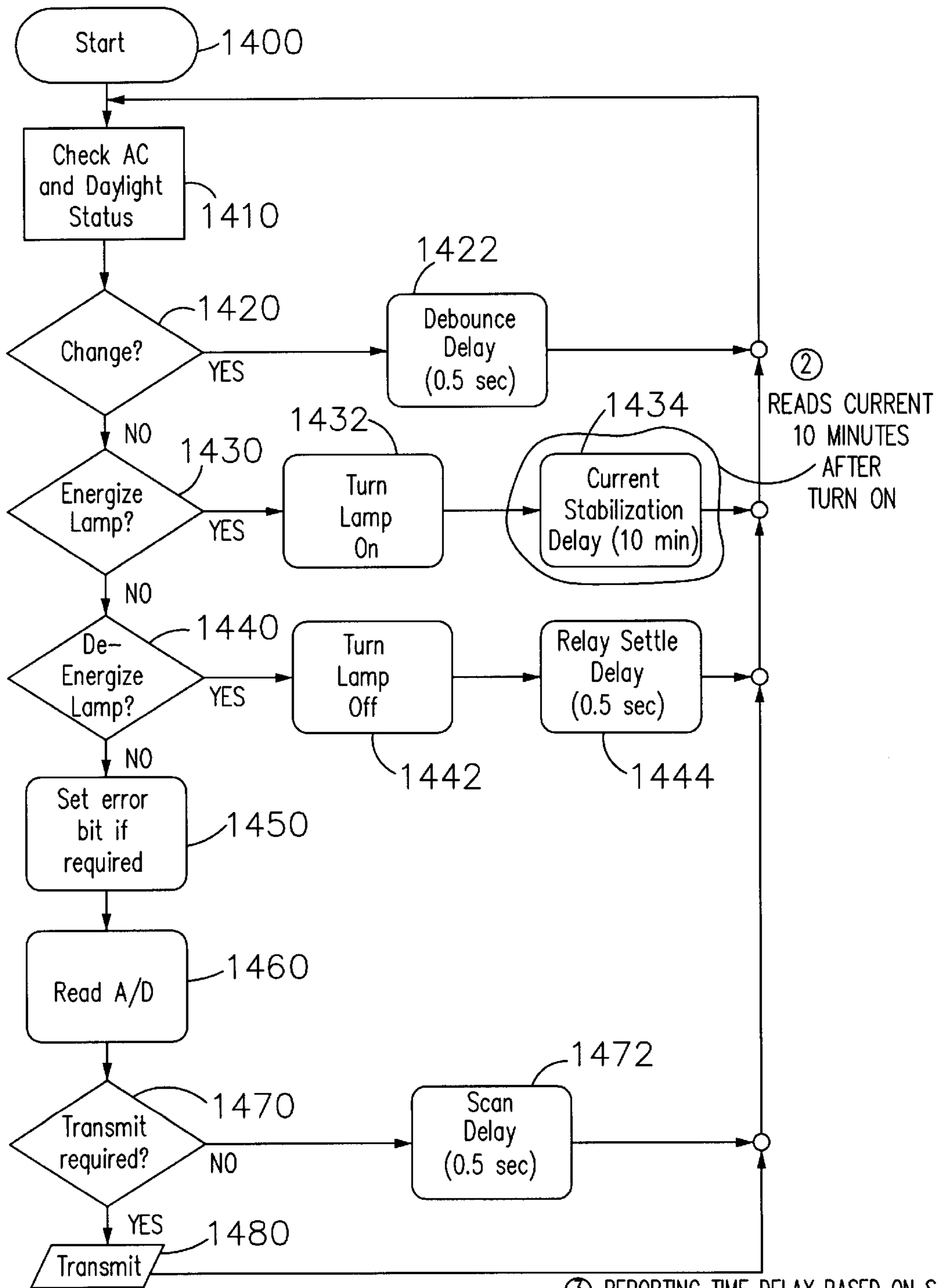
FIG. 14A (3) REPORTING TIME DELAY BASED ON S
